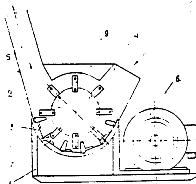
Structural-Technological Diagram for an IRM-50 Milling Unit
