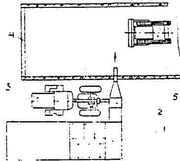
Technological Line for Processing Corn Ears and Leaf and Stalk Bulk Using an IRM-50 Milling Unit
