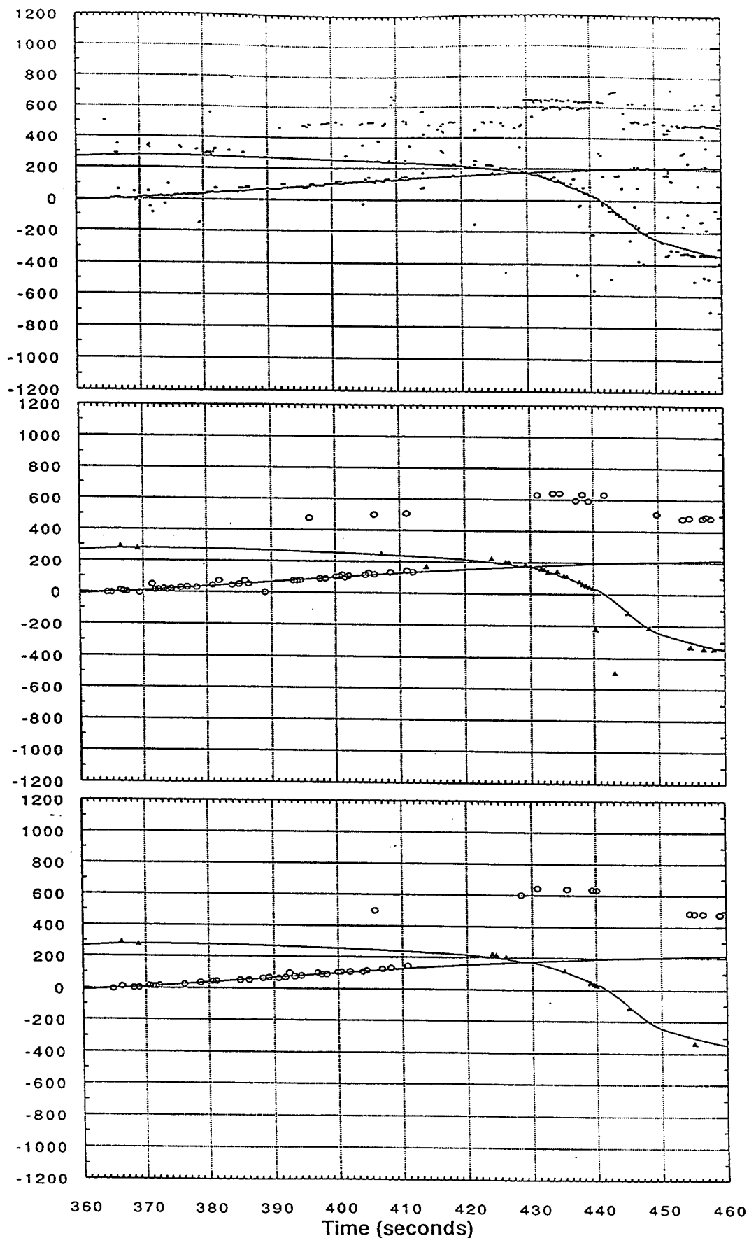
Figure E-2. Correlation of DTOAs (Delta - Stouffers) to predictions.
