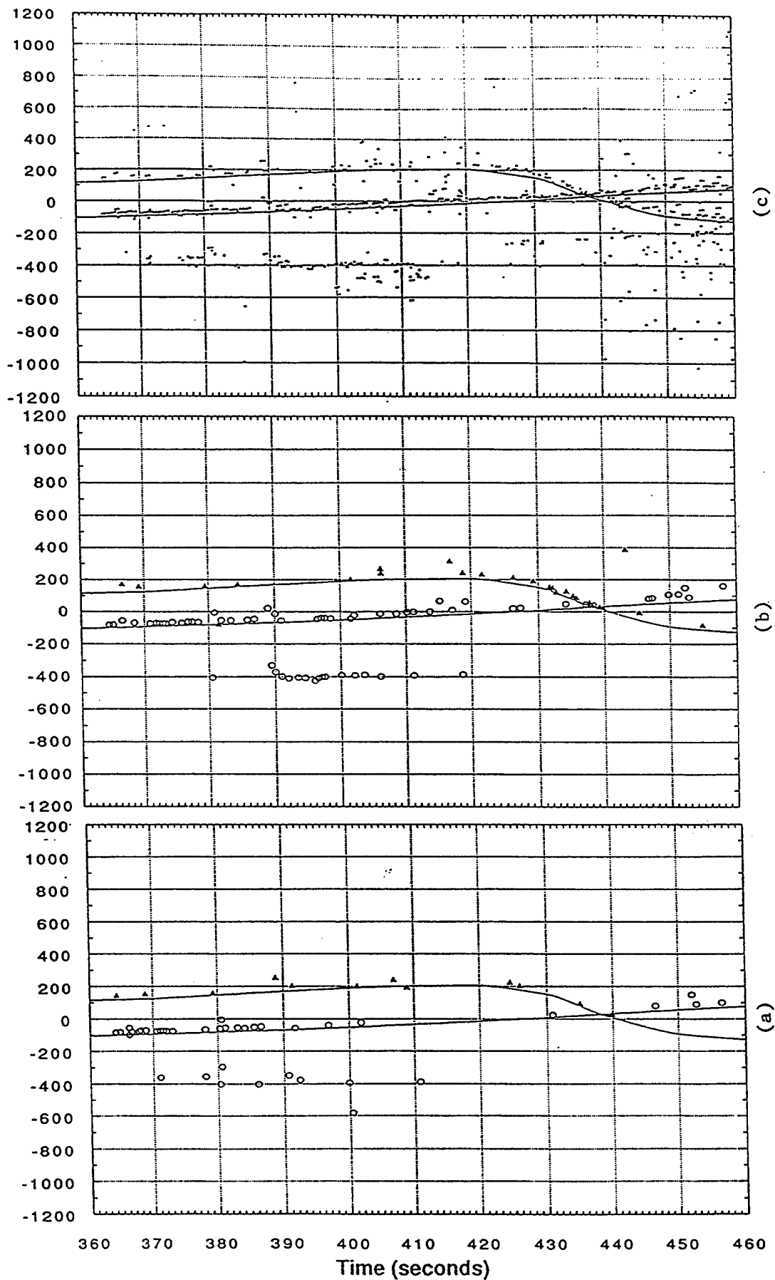
Figure 5-18. Correlation of DTOAs (Stouffers - Terminal C) to predictions.
