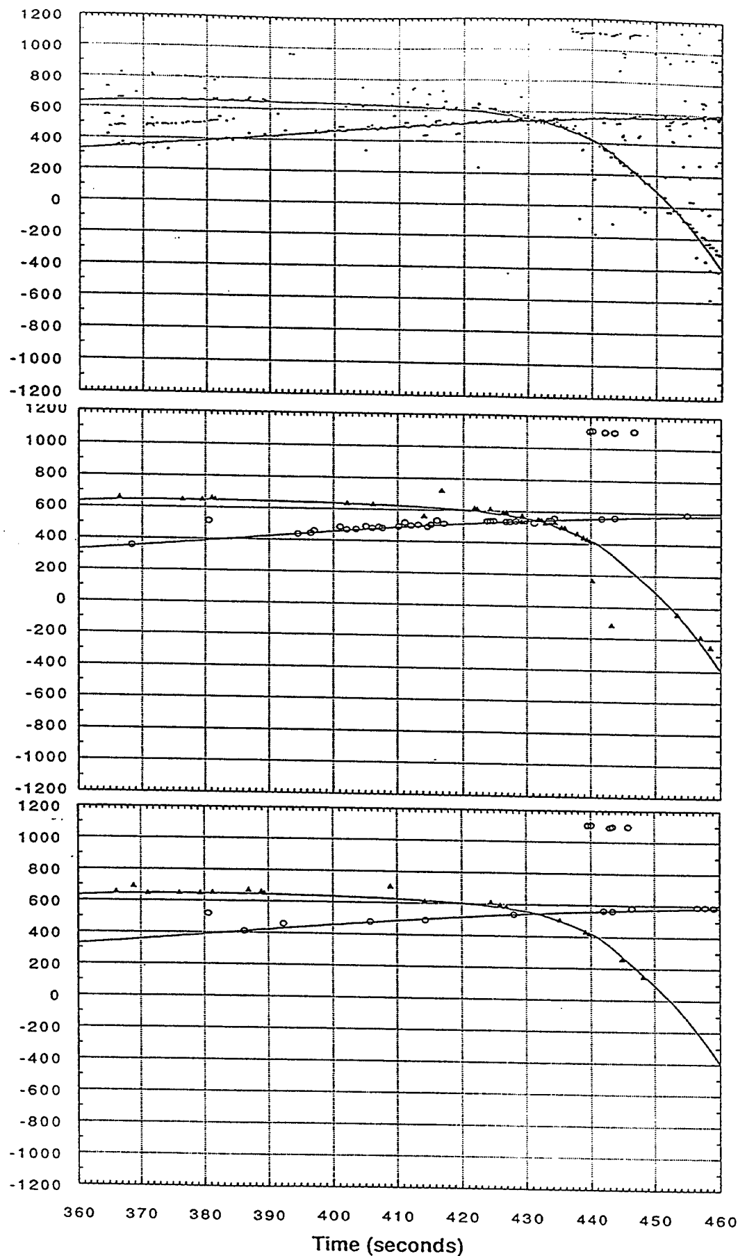
Figure E-5. Correlation of DTOAs (Ford - Stouffers) to predictions.
