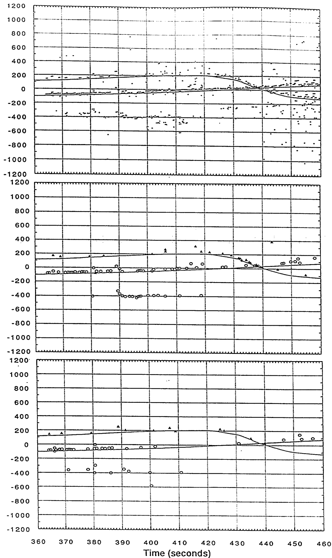
Figure E-9. Correlation of DTOAs (Stouffers - Terminal C) to predictions.
