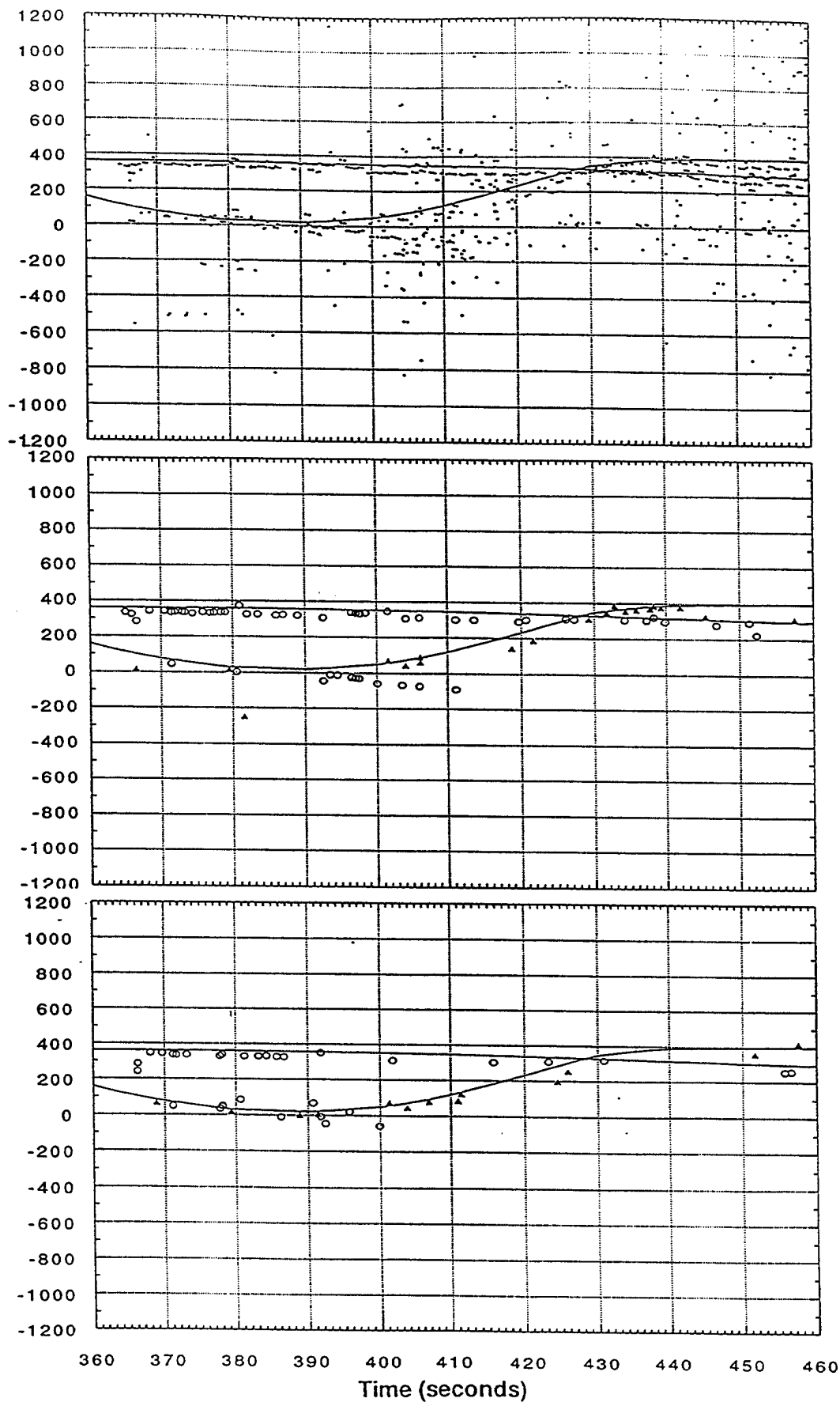
Figure E-10. Correlation of DTOAs (Region - Terminal C) to predictions.
