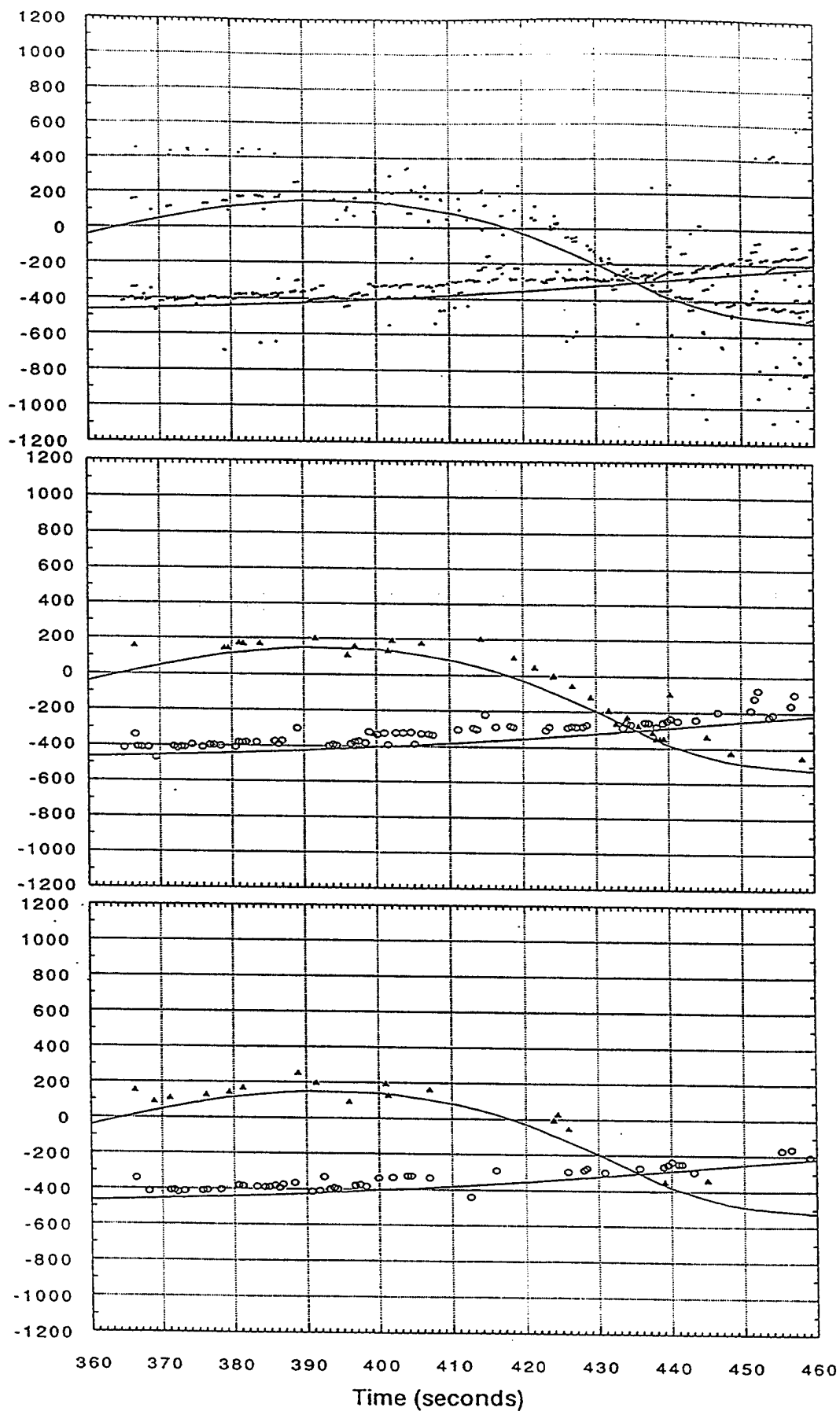
Figure E-8. Correlation of DTOAs (Stouffers - Region) to predictions.
