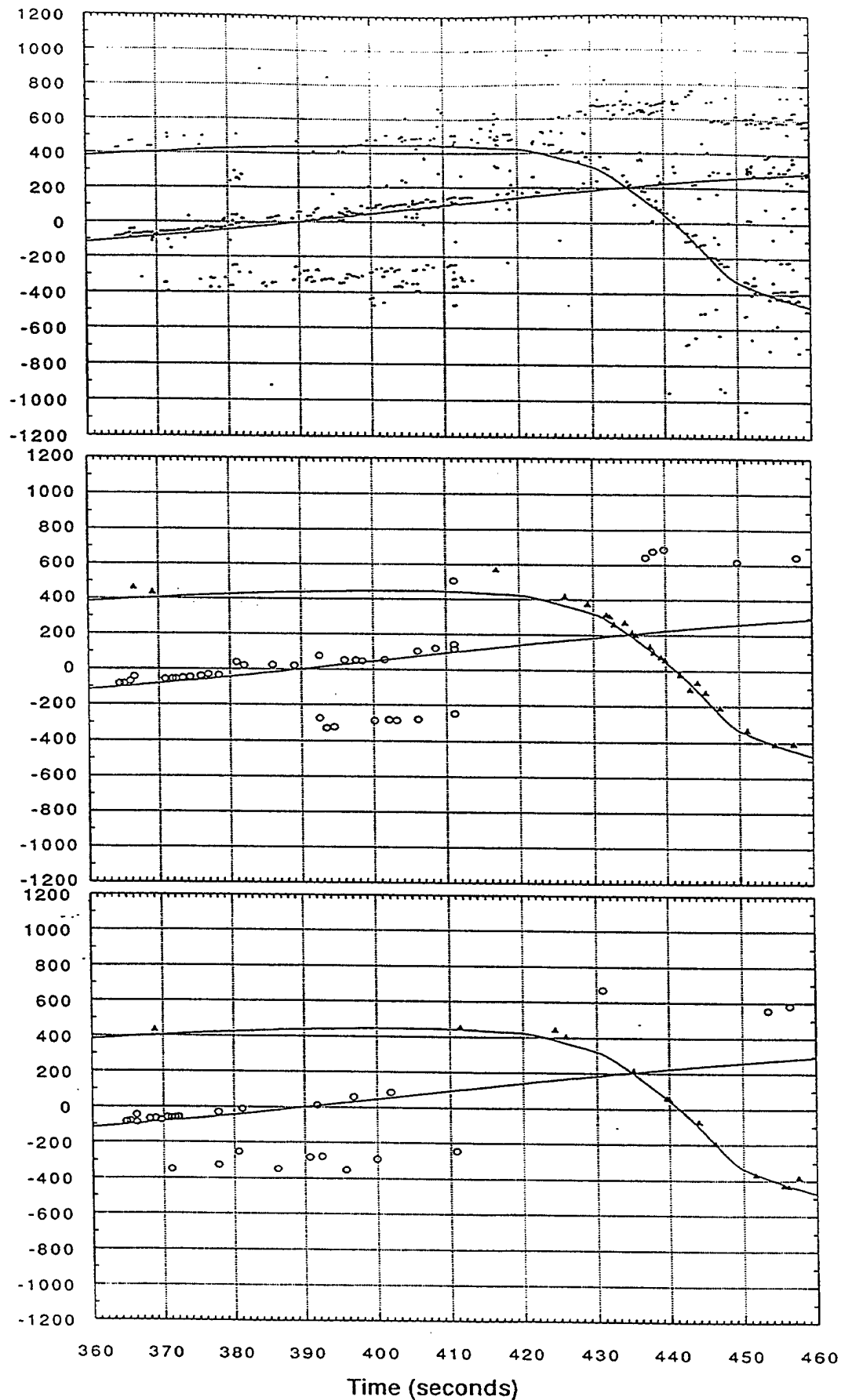
Figure E-4. Correlation of DTOAs (Delta - Terminal C) to predictions.
