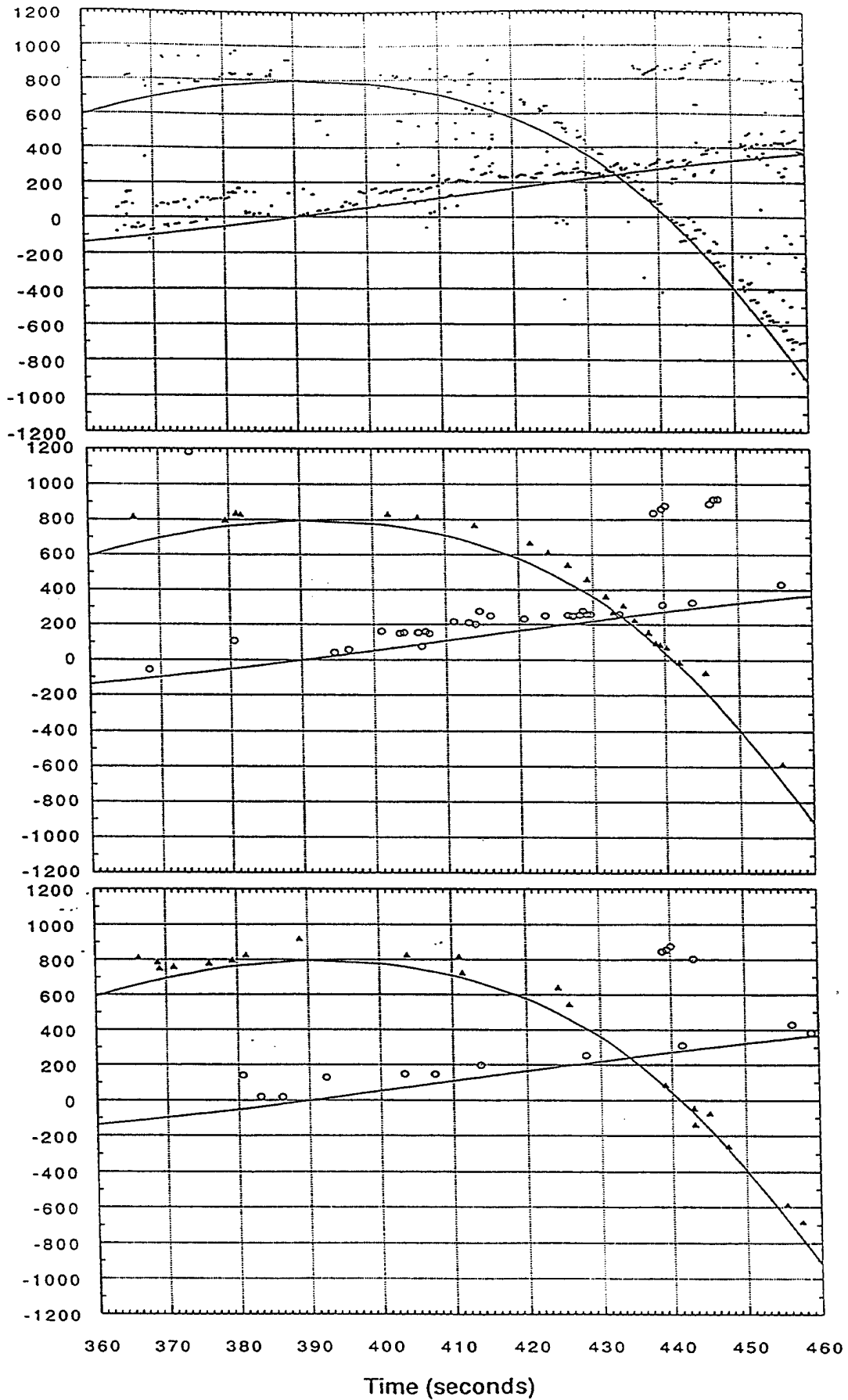
Figure E-6. Correlation of DTOAs (Ford - Stouffers) to predictions.
