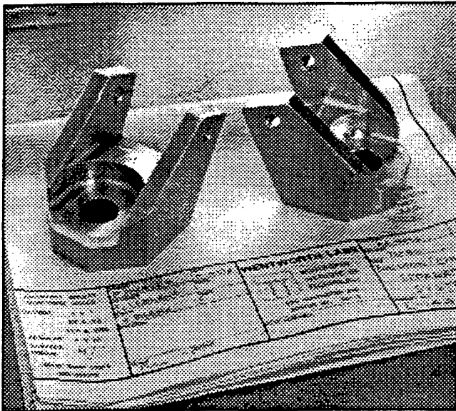
Figure 3 HABE Chute Bracket
