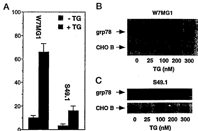
FIG. 9. Effect of TG on grp78 mRNA levels and viability in lymphoma cells. A , exponentially growing cells were incubated for 24 h in the presence or absence of 100 nM TG. The percentage of trypan blue-positive cells was measured 24 h after TG addition. Error bars represent the mean of duplicate determinations in multiple experiments. B , exponentially growing W7.MG1 cells were diluted to a concentration of 0.5 \times 10^6 /ml in fresh culture medium 7 h before adding 100 nM TG. RNA was isolated 7 h after TG addition and analyzed by Northern hybridization using radiolabeled grp78 and CHO-B cDNA probes. C , exponentially growing S49.1 cells were diluted to a concentration of 0.5 \times 10^6 /ml in fresh culture medium 7 h before adding 100 nM TG. RNA was isolated 7 h after TG addition and analyzed by Northern hybridization using radiolabeled grp78 and CHO-B cDNA probes.
