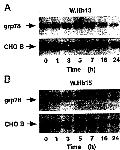
FIG. 3. Effect of TG treatment on grp78 mRNA levels in W.Hb13 and W.Hb15 cells. Exponentially growing cells were diluted to a concentration of 1 \times 10^6 /ml with fresh culture medium before adding 100 nM TG. RNA was isolated at the indicated times following TG addition and analyzed by Northern hybridization using radiolabeled grp78 and CHO-B cDNA probes. Representative blots for W.Hb13 cells (A) and W.Hb15 cells (B) are shown.
