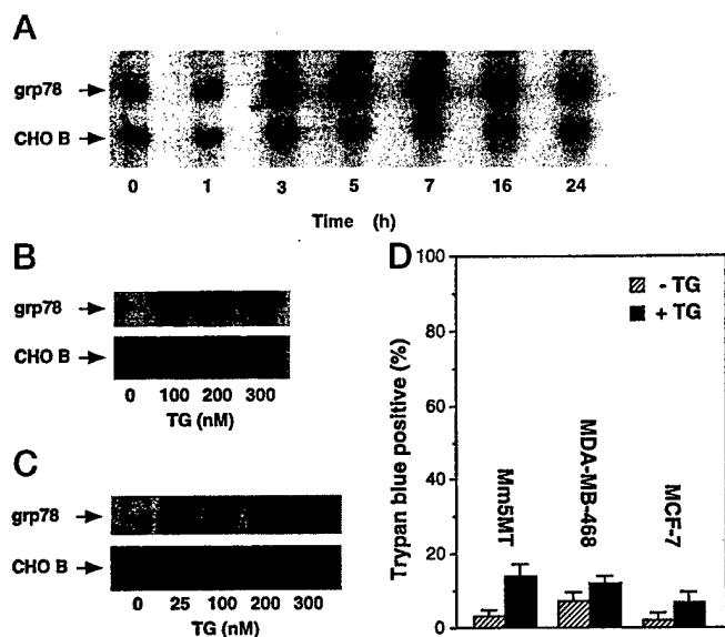
FIG. 8. Effect of TG on grp78 mRNA levels and viability in breast cancer cells. A , exponentially growing Mm5MT cells were treated with 100 nM TG. RNA was isolated at the indicated times following TG addition and analyzed by Northern hybridization using radiolabeled grp78 and CHO-B cDNA probes. B , exponentially growing MDA-MB-468 cells were treated with multiple concentrations of TG. RNA was isolated 7 h after TG addition and analyzed by Northern hybridization using radiolabeled grp78 and CHO-B cDNA probes. C , exponentially growing MCF-7 cells were treated with multiple concentrations of TG. RNA was isolated 7 h after TG addition and analyzed by Northern hybridization using radiolabeled grp78 and CHO-B cDNA probes. D , exponentially growing cells were incubated for 24 h in the presence or absence of 100 nM TG. The percentage of trypan blue-positive cells was measured 24 h after TG addition. Error bars represent the mean of duplicate determinations in multiple experiments.
