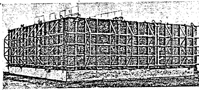
Large-panel formwork for poured-in-situ farmstead house.
