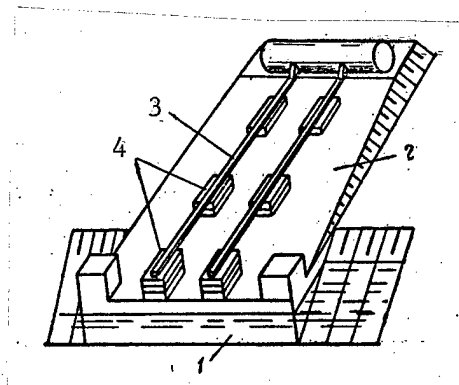
Figure 3. Berth for the Unloading of Heavy Equipment
