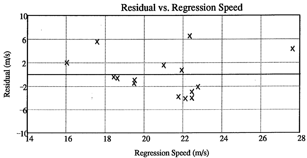
Figure 18. Residual Plot for Equation (38).
