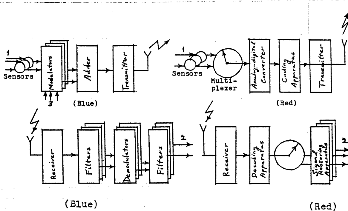
Fig. 2. Diagram of the analog (with frequency condensed channels) and digital (with time condensed channels) telemetric systems: 1 - Value measured; 2 - Measurement result; 3 - Subcarrier oscillations.
