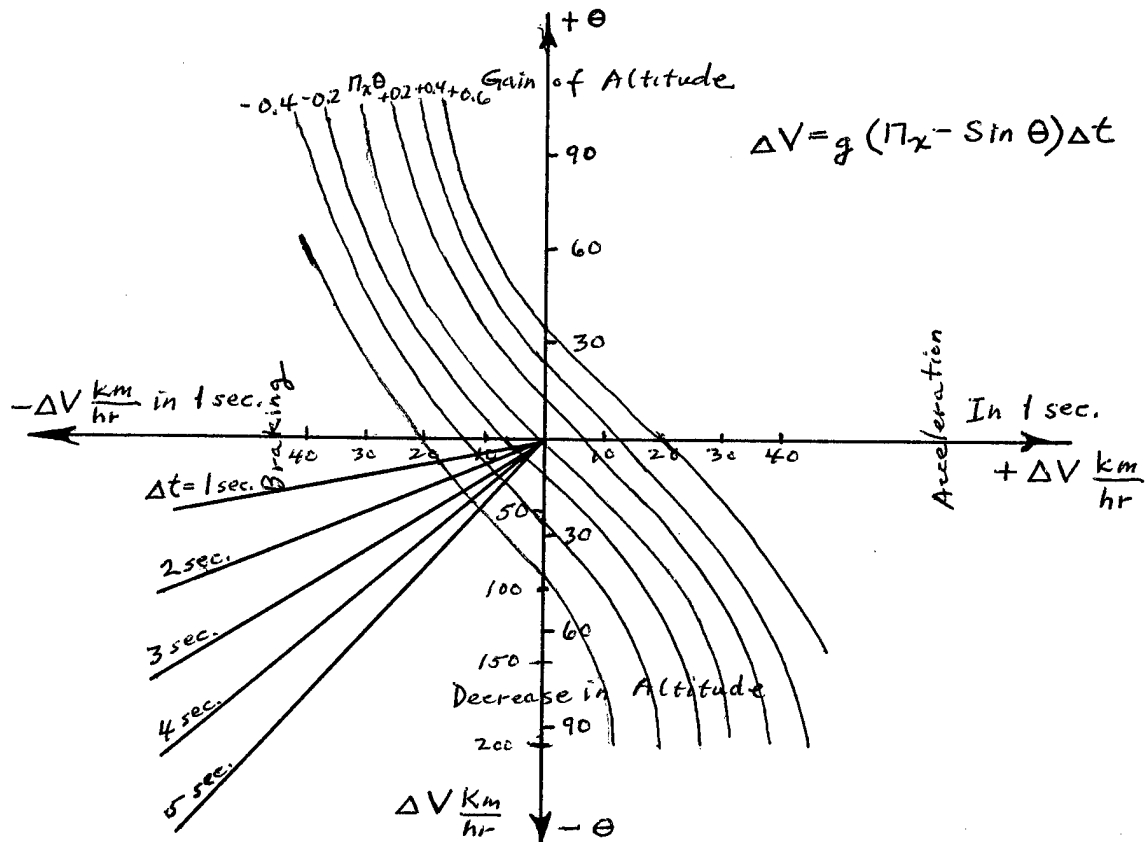
Fig. 2. Nomogram for Evaluating the Value of the Change in Velocity Excess from Angle 0 and Overload.
