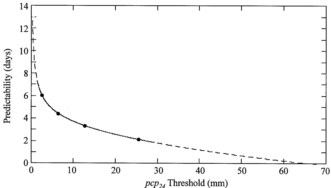
Figure 38. Limit of predictability as a function of pcp_{24} threshold. Results from skill score analysis are plotted as dots ( \bullet ). The solid line part of the curve shows the more credible results while the dashed parts of the curve are less credible extrapolations.
