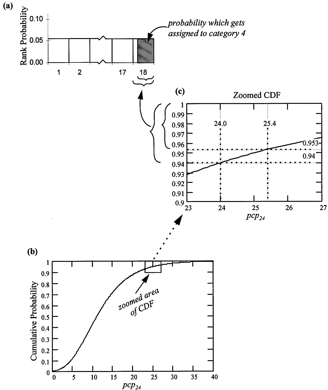
Figure 12. Determination of probability for a category whose threshold exceeds the highest ensemble member. (a) Verification rank probabilities for uniform ranks method. The fraction of rank #18 probability for category 4 is determined on the CDF. (b) Full view of the fitted Gumbel CDF for the sample ensemble forecast, ENS . (c) Zoomed view of CDF with markers for highest forecast pcp_{24} value (24.0) and category 4 threshold (25.4), and corresponding quantiles, 0.94 and 0.953. The ratio (1 - 0.953) / (1 - 0.94) \approx 0.8 , so 4/5 of the probability of rank #18 is the PQPF for category 4.
