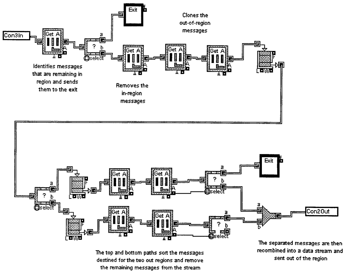
Figure C.1g – Message Routing Block
