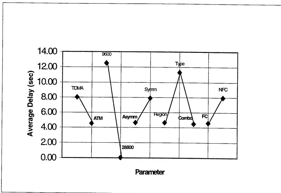
Figure 7.1 - Average Delay Optimization Plot
