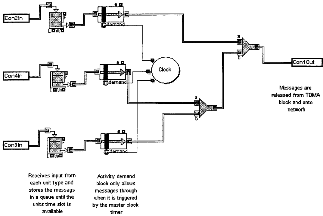
Figure C.1e – TDMA Block
