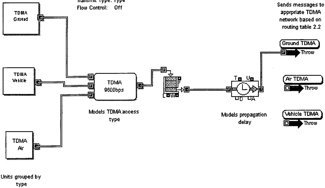
Figure C.3a – Top Layer of Model #3
