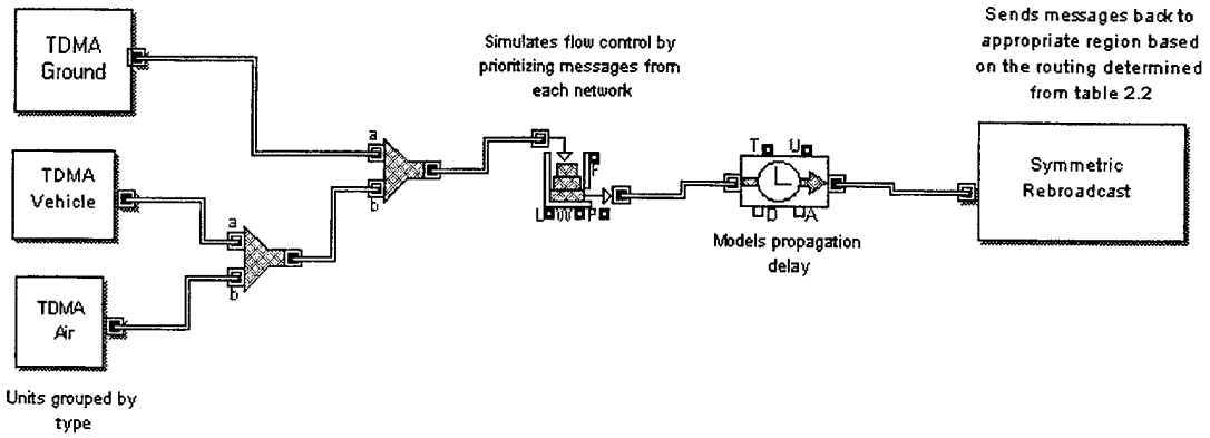
Figure C.6a – Top Layer of Model #6
