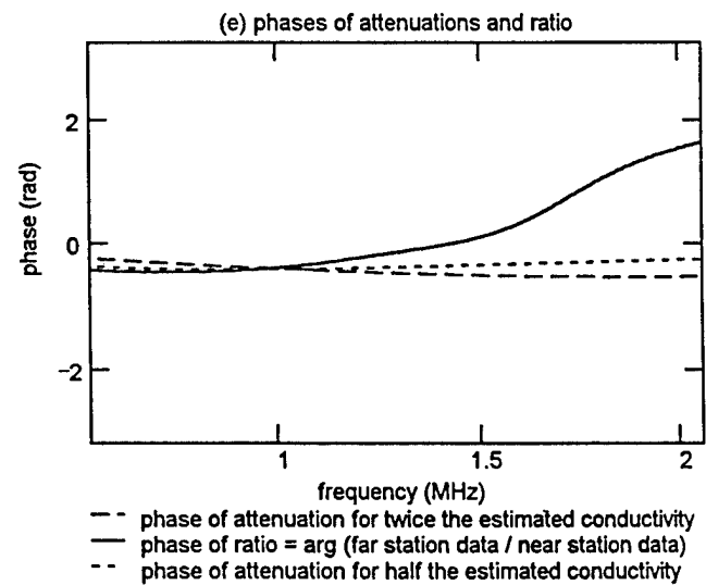
Fig 4. (a): Window showing subwindow limits, near station data, far station data, and estimate; (b) magnitudes of corresponding spectra; (c) phase shifts of spectra; (d) magnitudes of ratio of far station data to near station data and theoretical attenuation for twice the conductivity and half the conductivity; and (e) phase shifts of ratio and theoretical attenuation. System time tag = ( 1761.009 -1992 -254 -20 -31 -43 -608 -17 ) (Thomson, et al., 1994); station 2 time_tag = 499 ; near_station = 5 ; propagation distance to near station over land = 6147 m., far station = 3 ; difference in propagation distances over ground = 7223 m., and \sigma = 0.0058 S/m. All vectors were padded. This solution included data from all five stations.
