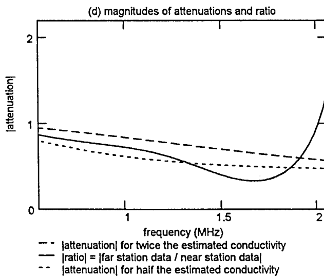
Fig 4. (a): Window showing subwindow limits, near station data, far station data, and estimate; (b) magnitudes of corresponding spectra; (c) phase shifts of spectra; (d) magnitudes of ratio of far station data to near station data and theoretical attenuation for twice the conductivity and half the conductivity; and (e) phase shifts of ratio and theoretical attenuation. System time tag = ( 1761.009 -1992 -254 -20 -31 -43 -608 -17 ) (Thomson, et al., 1994); station 2 time_tag = 499 ; near_station = 5 ; propagation distance to near station over land = 6147 m., far station = 3 ; difference in propagation distances over ground = 7223 m., and \sigma = 0.0058 S/m. All vectors were padded. This solution included data from all five stations.
