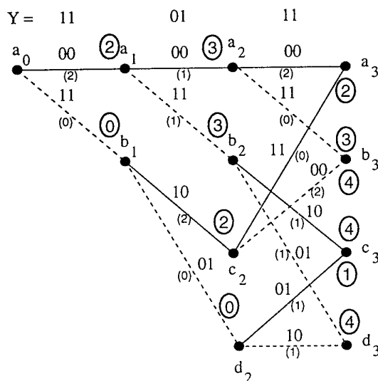
Figure 3.11: Example of a received Viterbi Code
