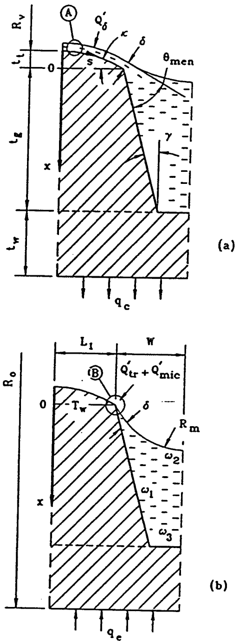
Figure 2.1: Cross sections of the characteristic elements of an axially grooved heat pipe: (a) condenser; (b) evaporator.
