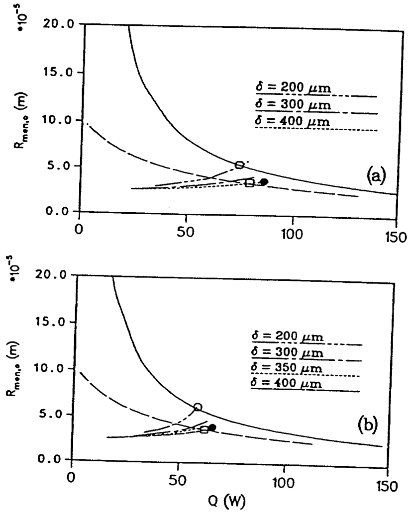
Figure 2.33: Variation of the driving meniscus radius and thickness of the vapor blanket at the fin top with heat input ( K = 1.0 \times 10^{-12} \text{ m}^2 ): (a) T_v = 110^\circ\text{C} ; (b) T_v = 100^\circ\text{C} .
