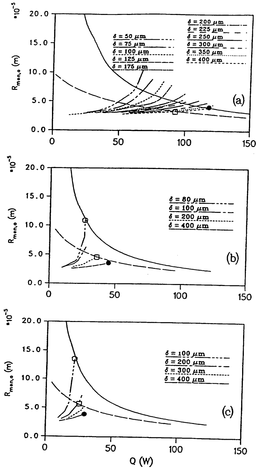
Figure 2.32: Variation of the driving meniscus radius and thickness of the vapor blanket at the fin top with heat input: (a) T_v = 120^\circ\text{C} , K = 1.0 \times 10^{-12} \text{ m}^2 ; (b) T_v = 90^\circ\text{C} , K = 1.0 \times 10^{-12} \text{ m}^2 ; (c) T_v = 90^\circ\text{C} , K = 0.5 \times 10^{-12} \text{ m}^2 .
