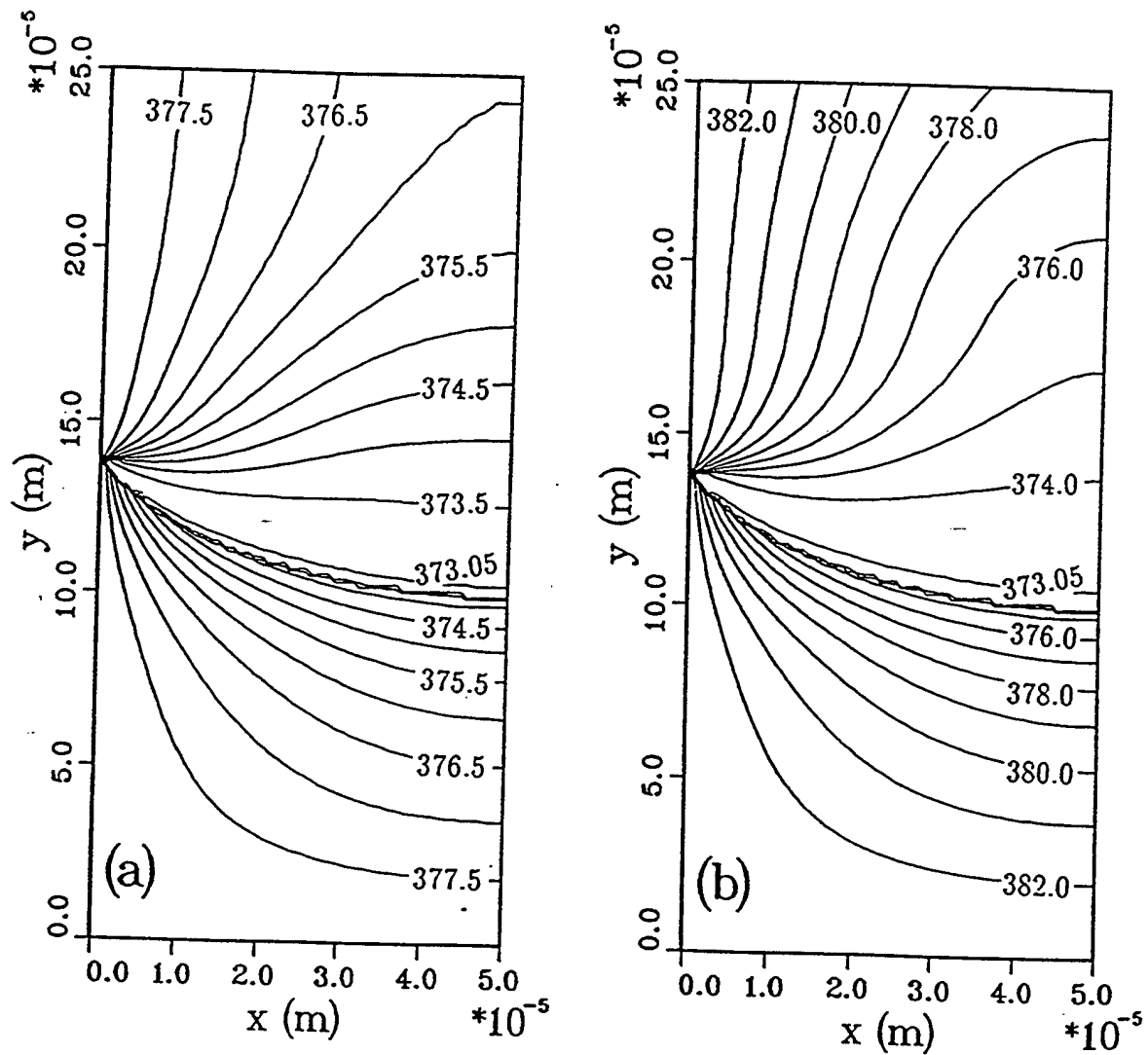
Figure 2.11: Temperature contours in the liquid and vapor (a) T_w - T_{\text{sat}} = 5 \text{ K} (b) T_w - T_{\text{sat}} = 10 \text{ K}
