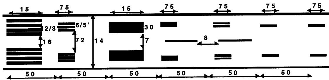
Figure 1. Standard Runway Markings for Instrument Runway.
