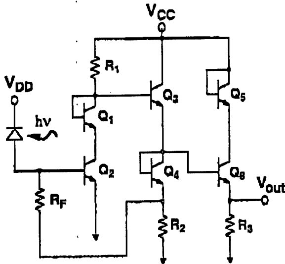
Fig. 6.6. Circuit diagram of the fabricated photoreceiver
