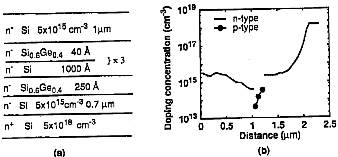
Figure 7.6: (a) Design of ideal heterostructure for SiGe/Si quantum well modulator, and (b) doping profile of heterostructure grown by Molecular beam epitaxy as measured by SRA.
