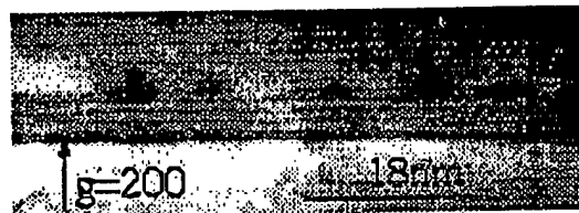
Figure 8.1. Cross-section TEM of InGaAs/GaAs multi-layer quantum dots
