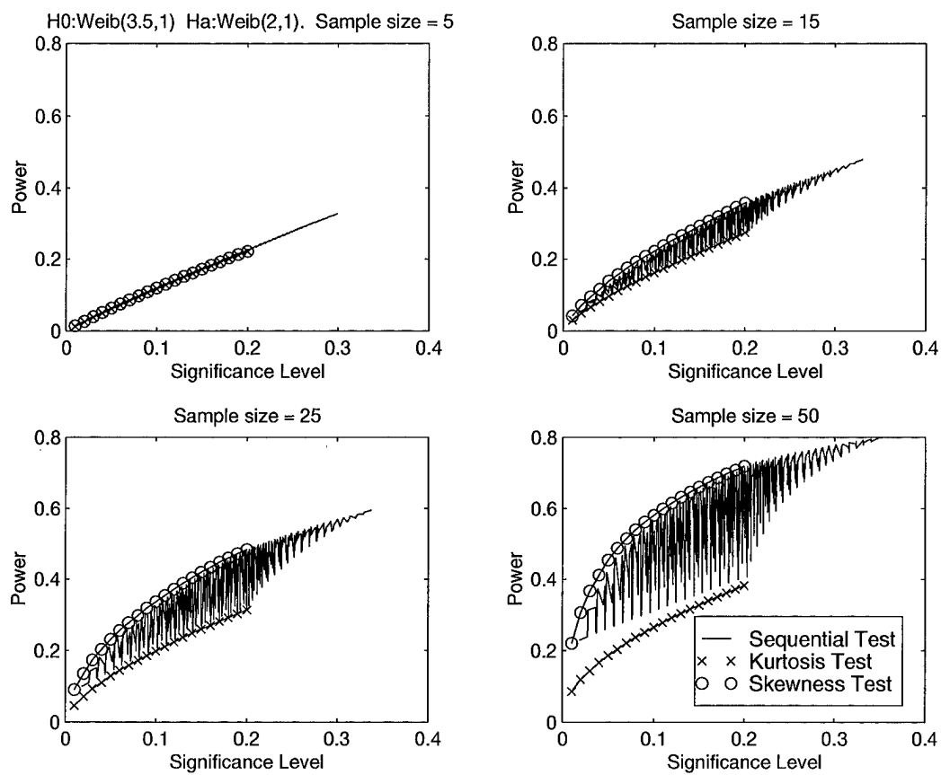
Figure D.25 Individual vs. Sequential Power: H_0: \text{Weibull}(\beta = 3.5) ; H_a: \text{Weibull}(\beta = 2) .
