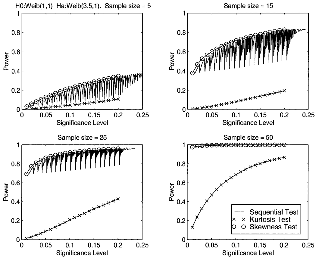
Figure D.11 Individual vs. Sequential Power: H_0 :Weibull( \beta = 1 ); H_a :Weibull( \beta = 3.5 ).
