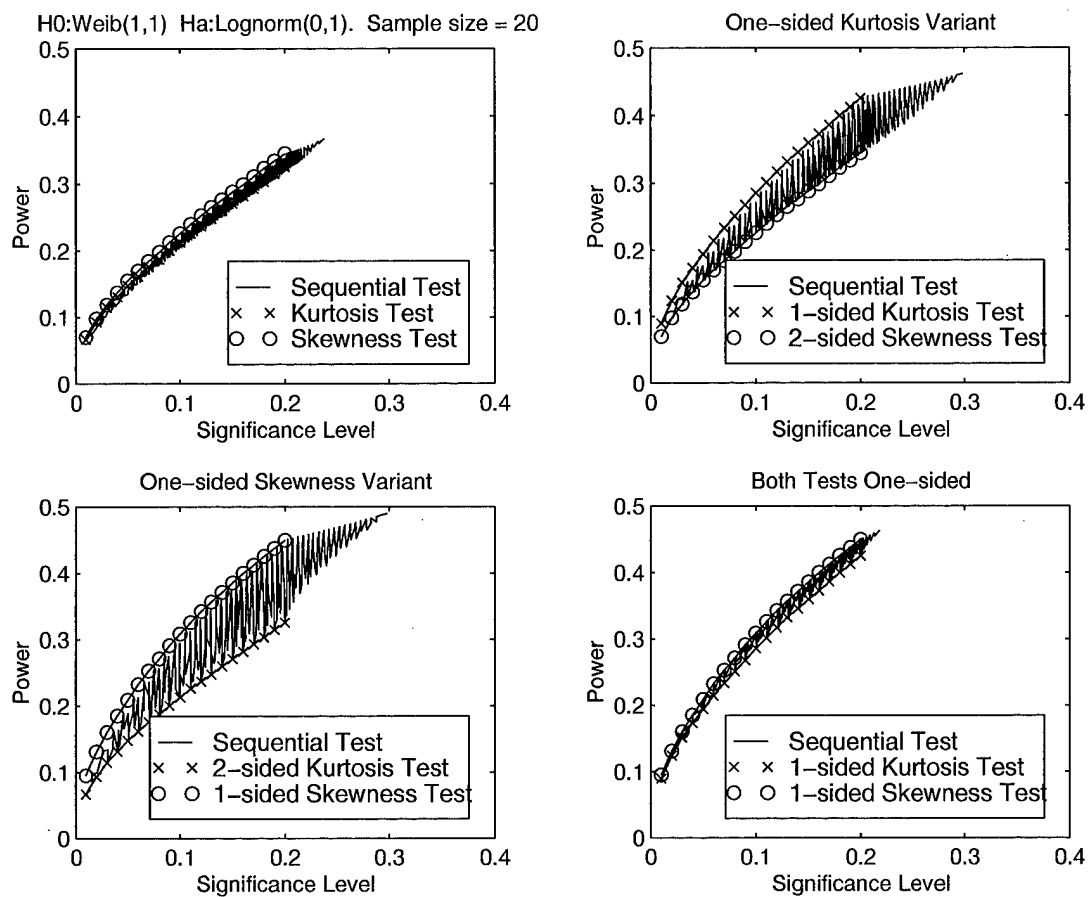
Figure G.1 Power of One-Sided Variants: H 0 : Weibull( \beta = 1 ); H a : Lognormal(0,1), n = 20 .
