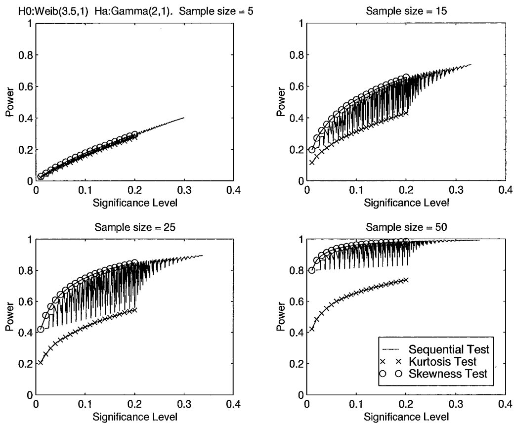
Figure D.23 Individual vs. Sequential Power: H_0: \text{Weibull}(\beta = 3.5) ; H_a: \text{Gamma}(2, 1) .
