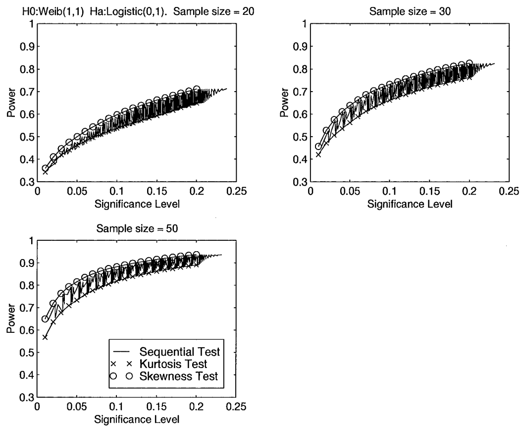
Figure D.15 Individual vs. Sequential Power: H_0: \text{Weibull}(\beta = 1) ; H_a: \text{XLogistic}(0,1) .
