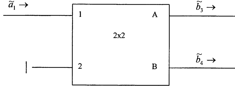
Figure 2.3 Single Input 2x2 Coupler
