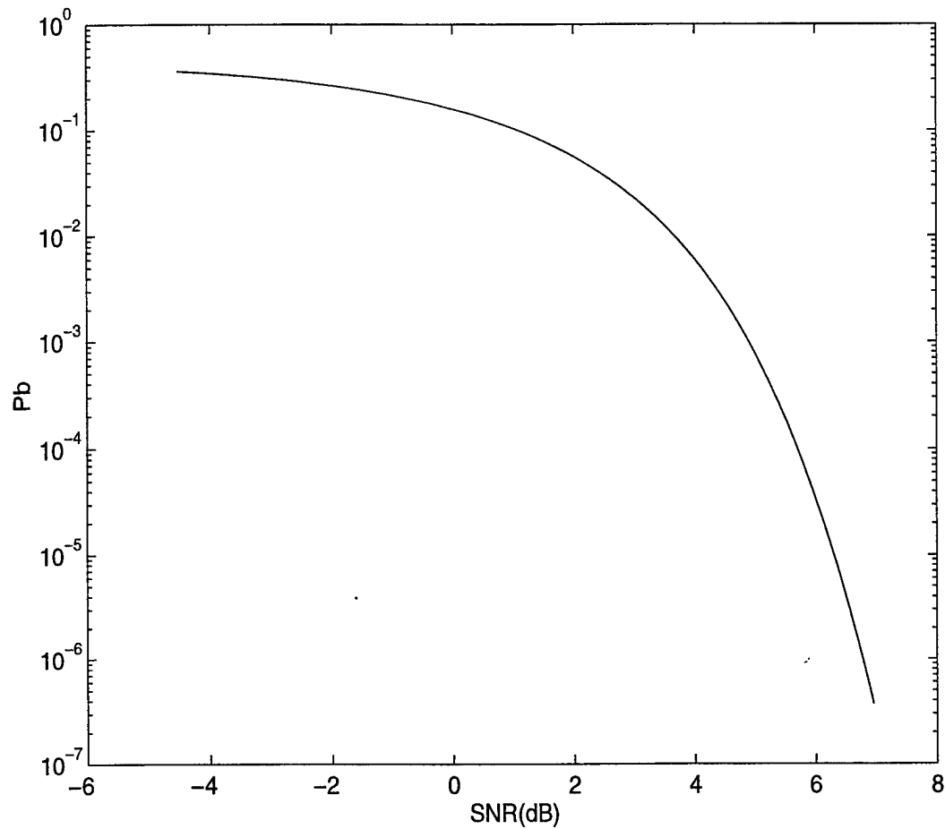
Figure 3.2 P_b vs. SNR
