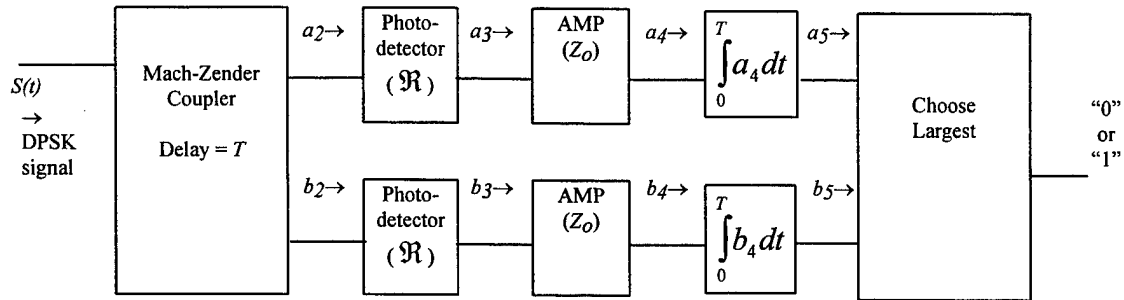
Figure 3.1 Optical DPSK Receiver
