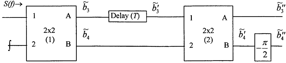
Figure 2.6 Input Signal Through Mach-Zender Coupler
