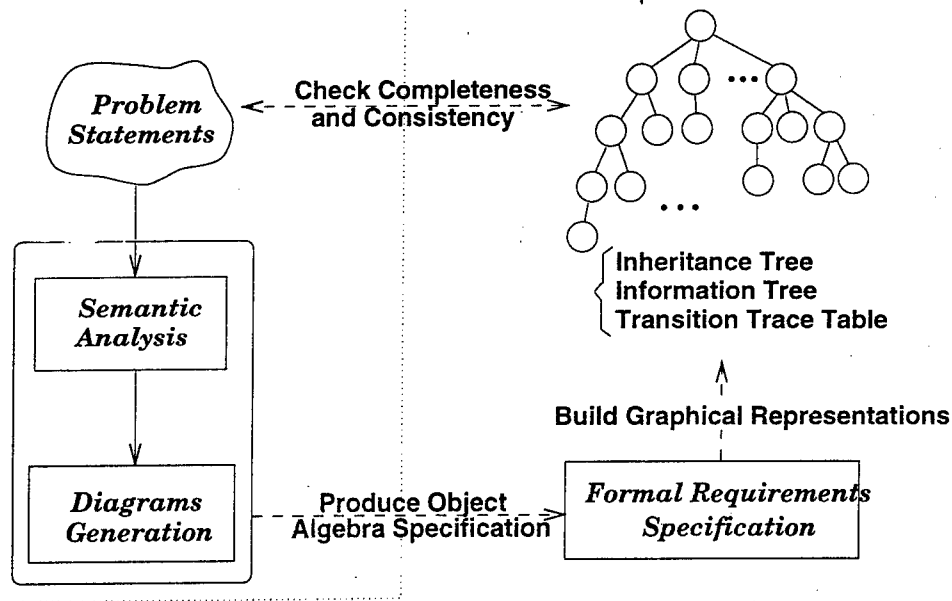
Figure 3.5: OOA verification.
