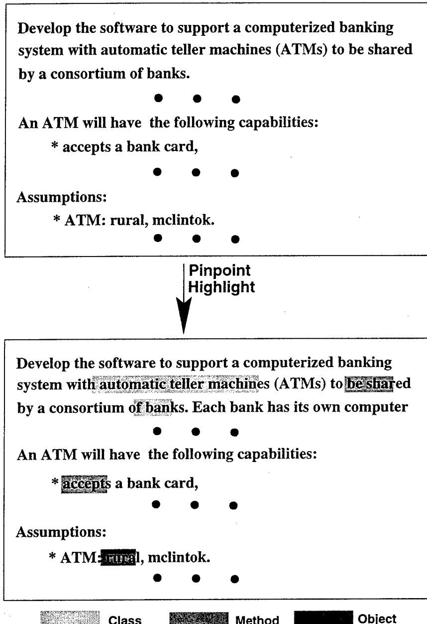
Figure 3.3: Our process for semantic analysis.
