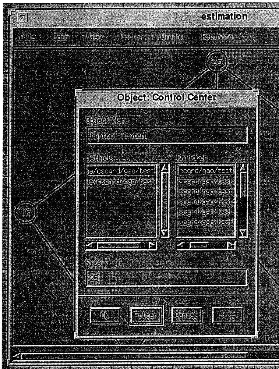
Figure 4.5: An example of the interface for modifying the object "Control Center" (25).
