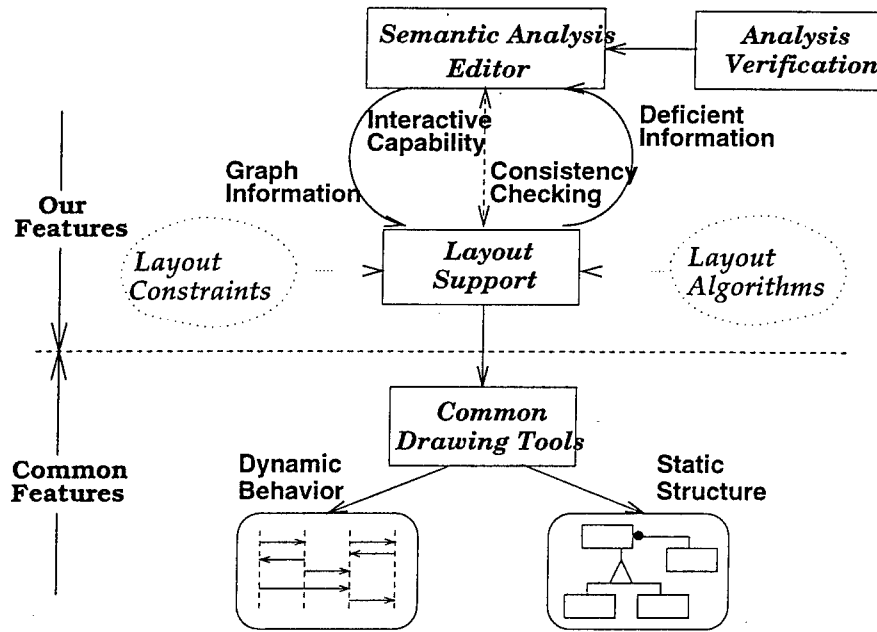
Figure 3.2: Our approach.
