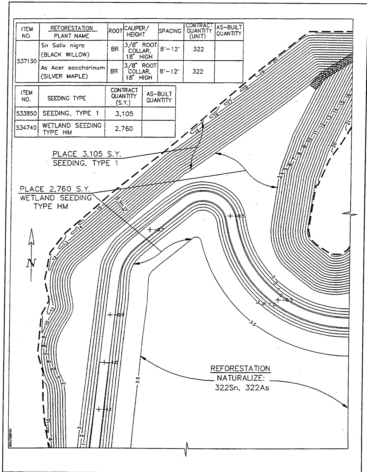
Figure 3. Segment of landscape plan with pay items
