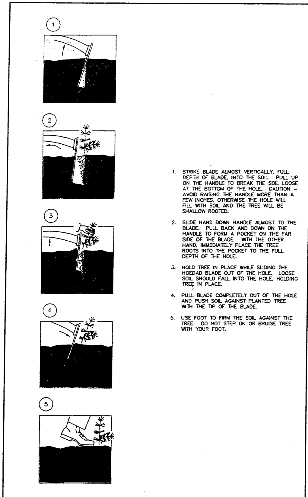
Figure H3. Reforestation planting procedure with hoedad
