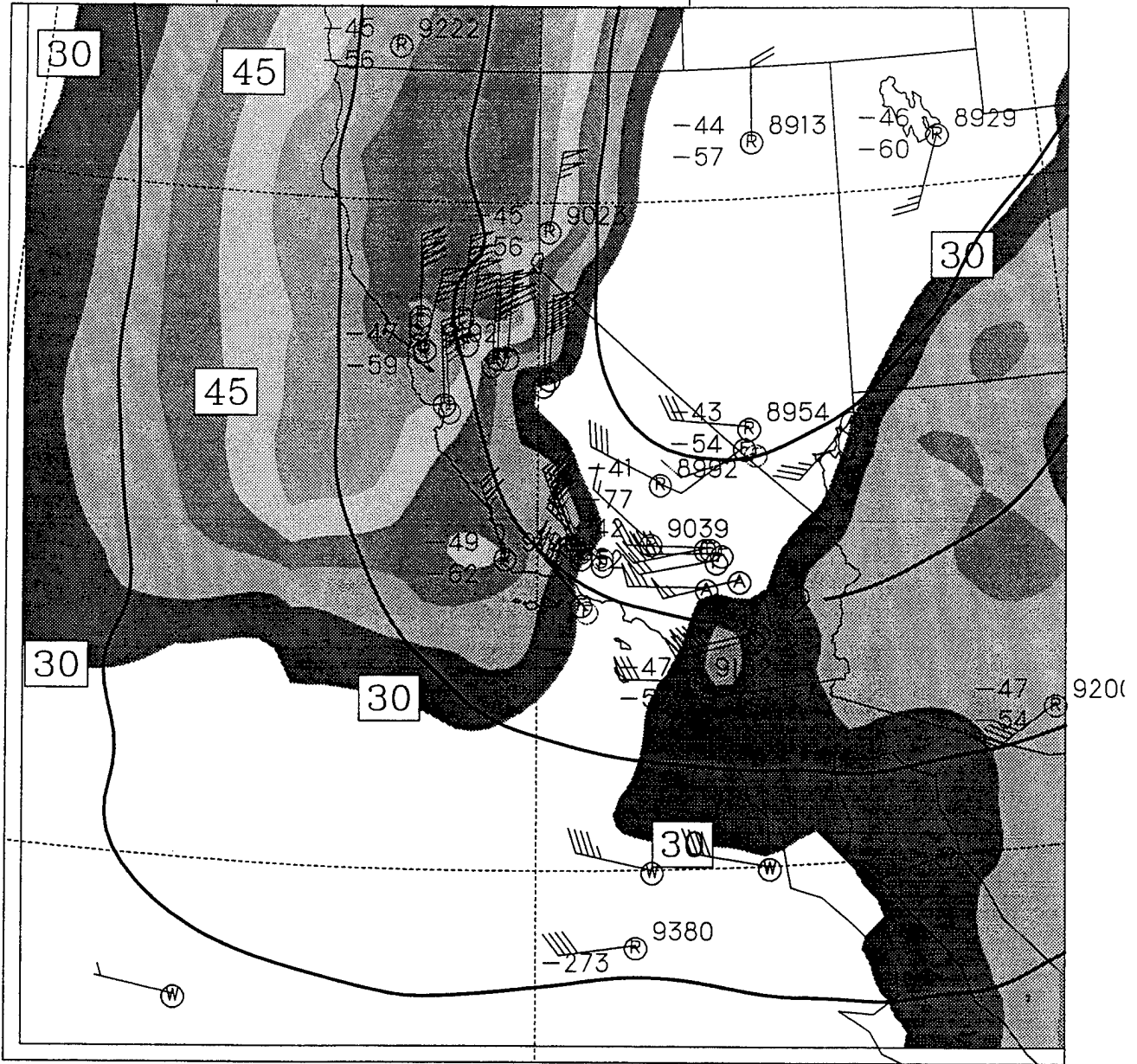
Fig. 32. Same as Fig. 28 except for 0000 UTC 2 April 1997.
