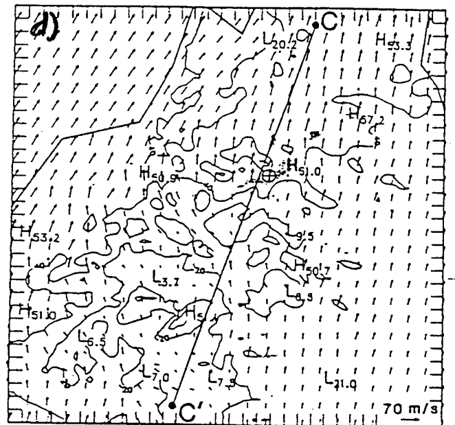
Fig. 43. Diagrams from Doyle et al. 1995. a) is isentropic cross section, b) is topographic and COAMPS grid map, c) is cross section of horizontal wind speed in m/s; d) is plan view of cross sectional plane C to C'.
