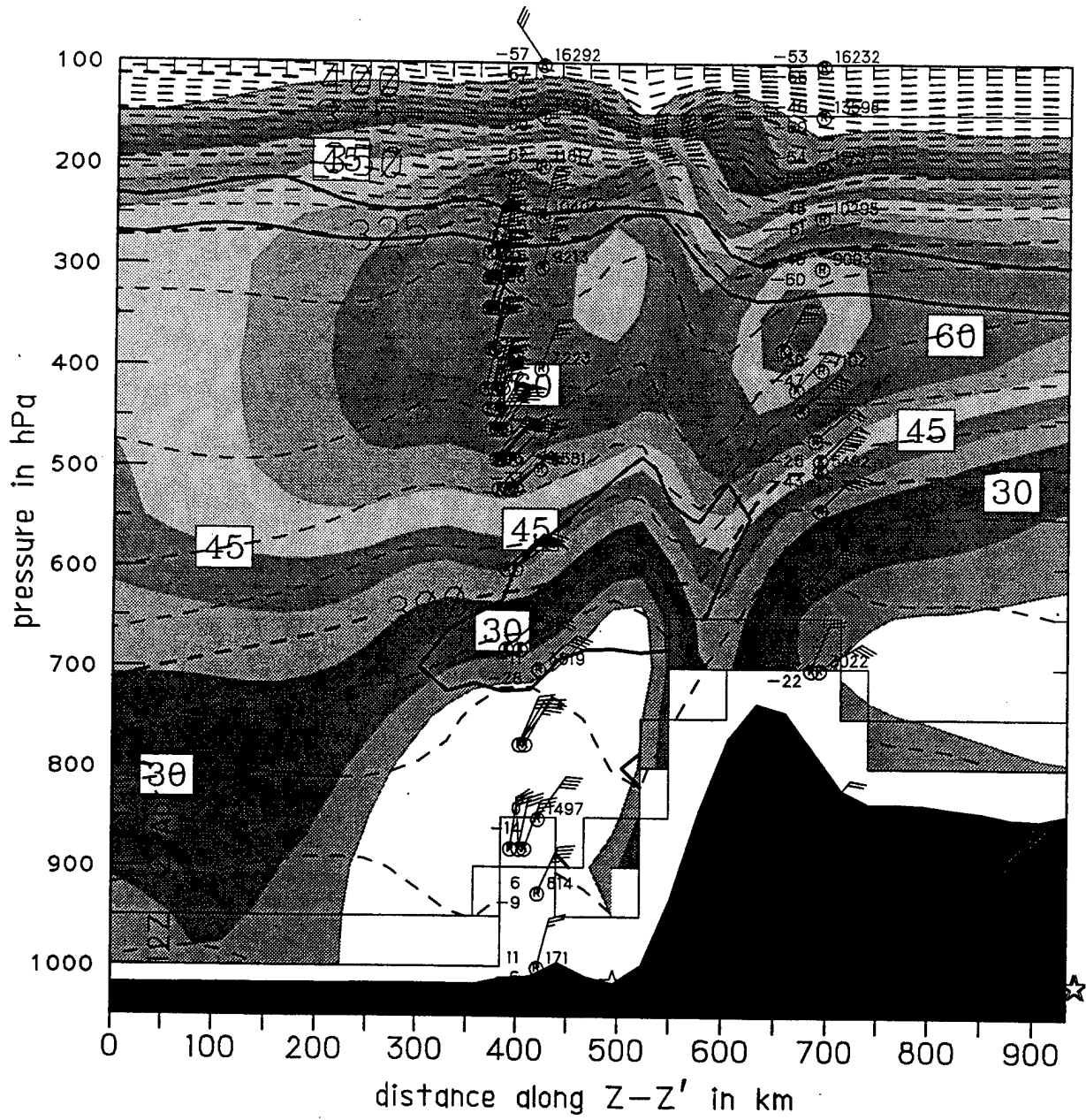
Fig. 41. COAMPS cross section at 1200 UTC 2 April 97 through the Z to Z' plane identified in Fig. 40. Cross section details same as in Fig. 4.
