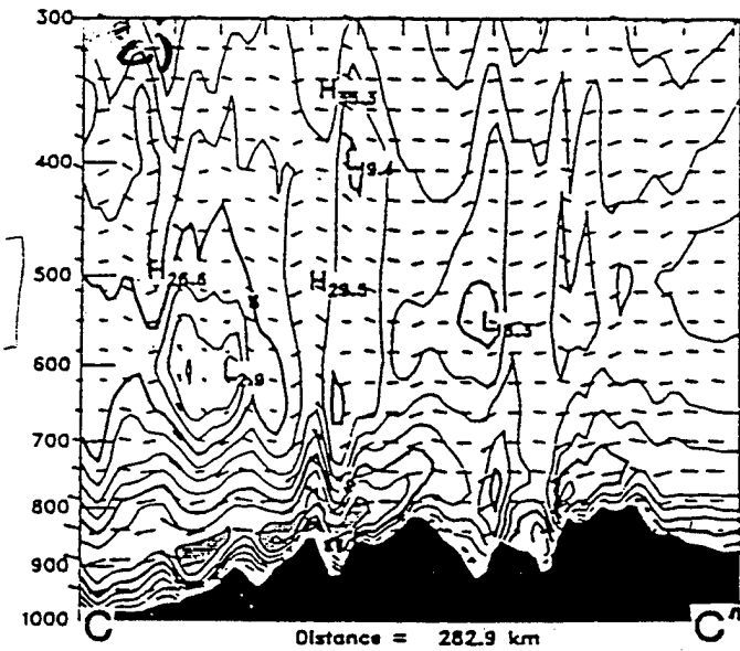
Fig. 43. Diagrams from Doyle et al. 1995. a) is isentropic cross section, b) is topographic and COAMPS grid map, c) is cross section of horizontal wind speed in m/s; d) is plan view of cross sectional plane C to C'.
