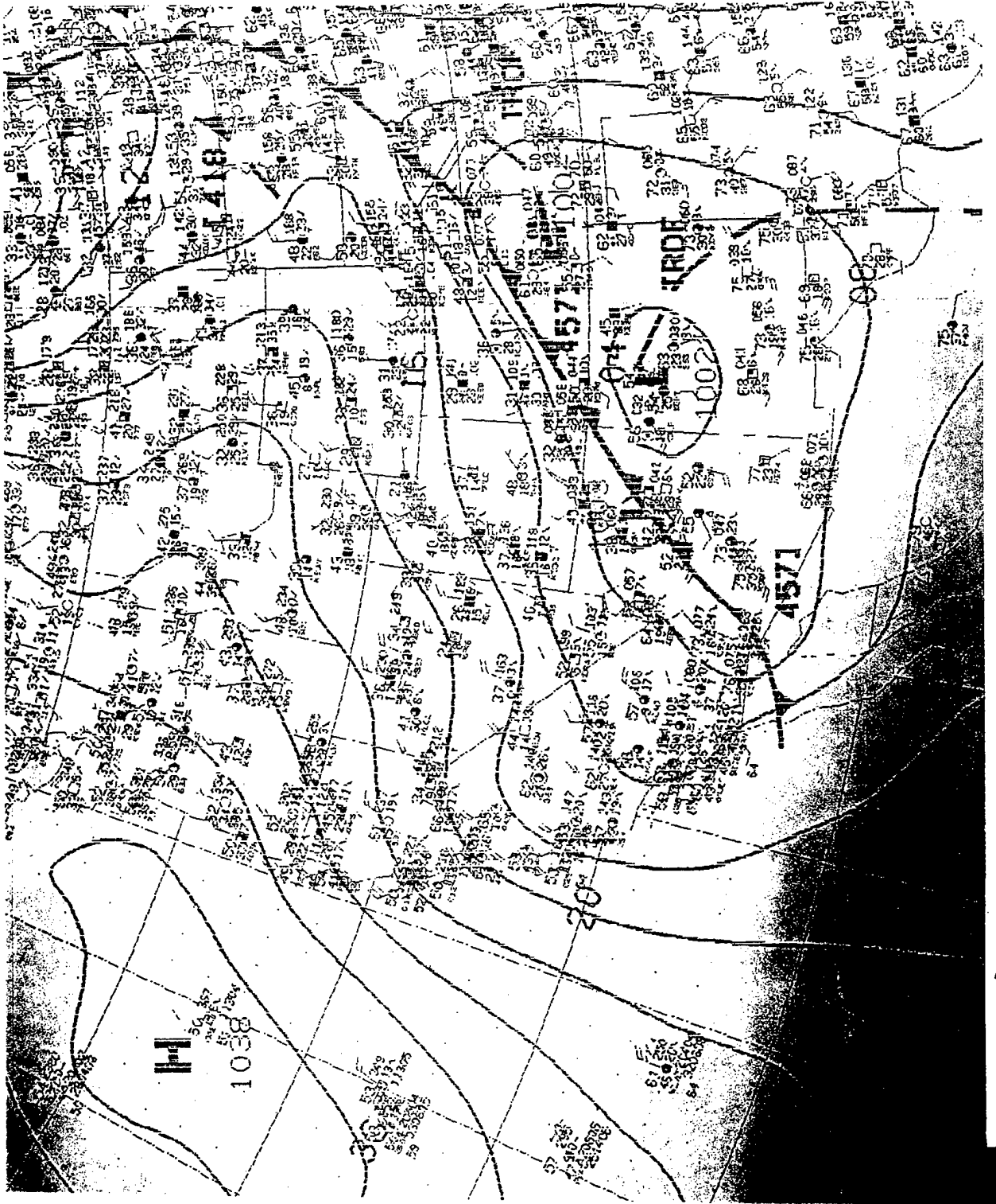
Fig. 19. Same as Fig. 11 but at 0000 UTC 2 April 1997.
