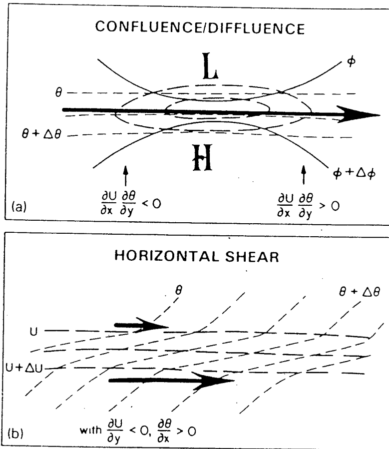
Fig. 1. Schematic depictions on a constant pressure surface, of straight frontal zones characterized by (a) confluence and diffuence associated with a jet maximum, and (b) horizontal shear in the presence of a positive along-front thermal gradient. Geopotential height contours, thick solid lines; isotachs of the along-front geostrophic wind component U , thick dashed lines; isentropes, thin dashed lines. Heavy arrows indicate the jet axis in (a) and the sense of cross-front shear of the along-front wind component in (b). (from Shapiro and Keyser 1990, Fig. 10.6)
