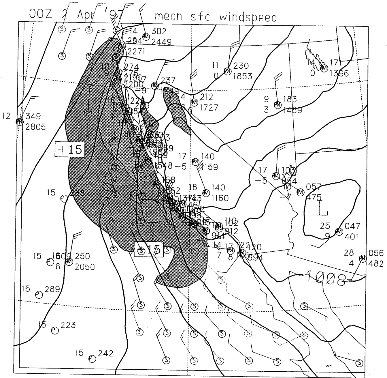
Fig. 33. Same as Fig. 29 except for 0000 UTC 2 April 1997.
