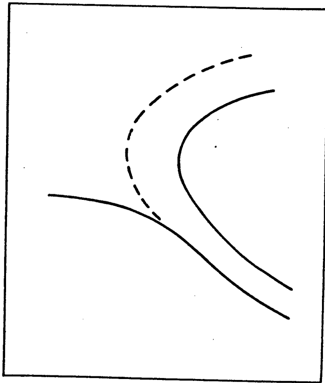
Fig. 3. Schematic diagram of the present-day model for analyzing upper-level fronts and tropopauses. Solid lines denote frontal and tropopause boundaries; dashed line depicts the boundary of cyclonic shear zone in the lower stratosphere. (from Keyser and Shapiro 1986, Fig. 6)
