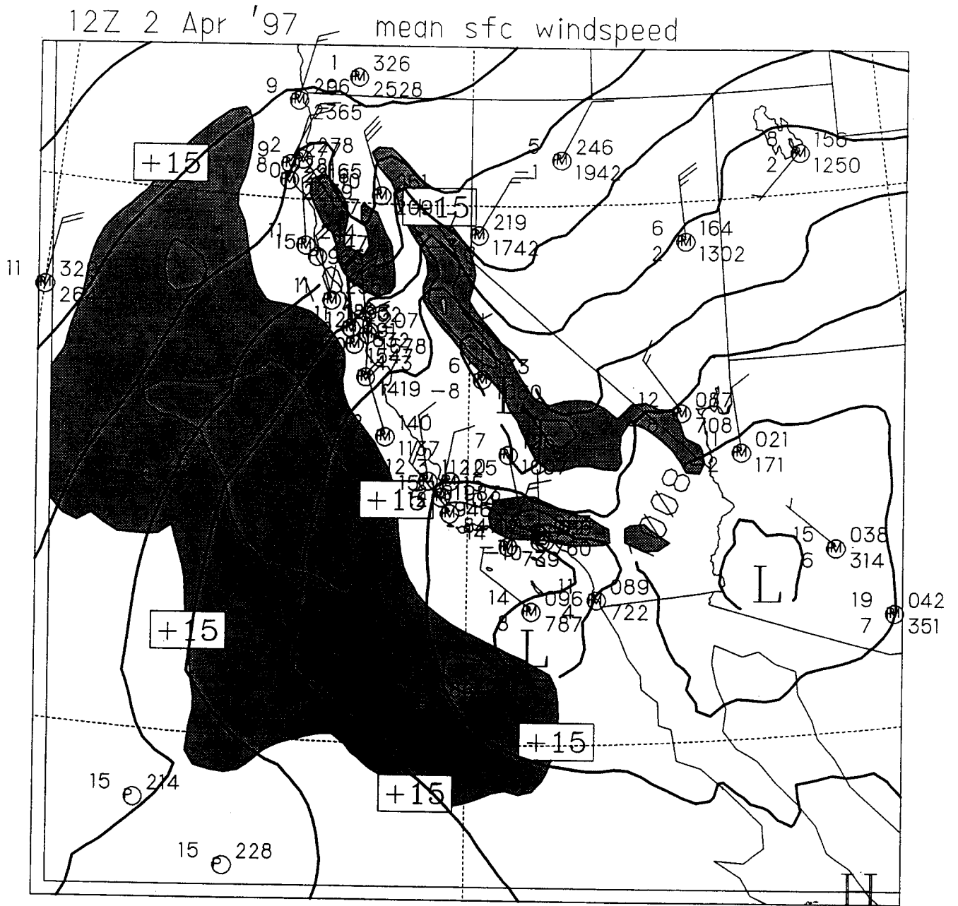
Fig. 36. Same as Fig. 29 except for 1200 UTC 2 April 1997.
