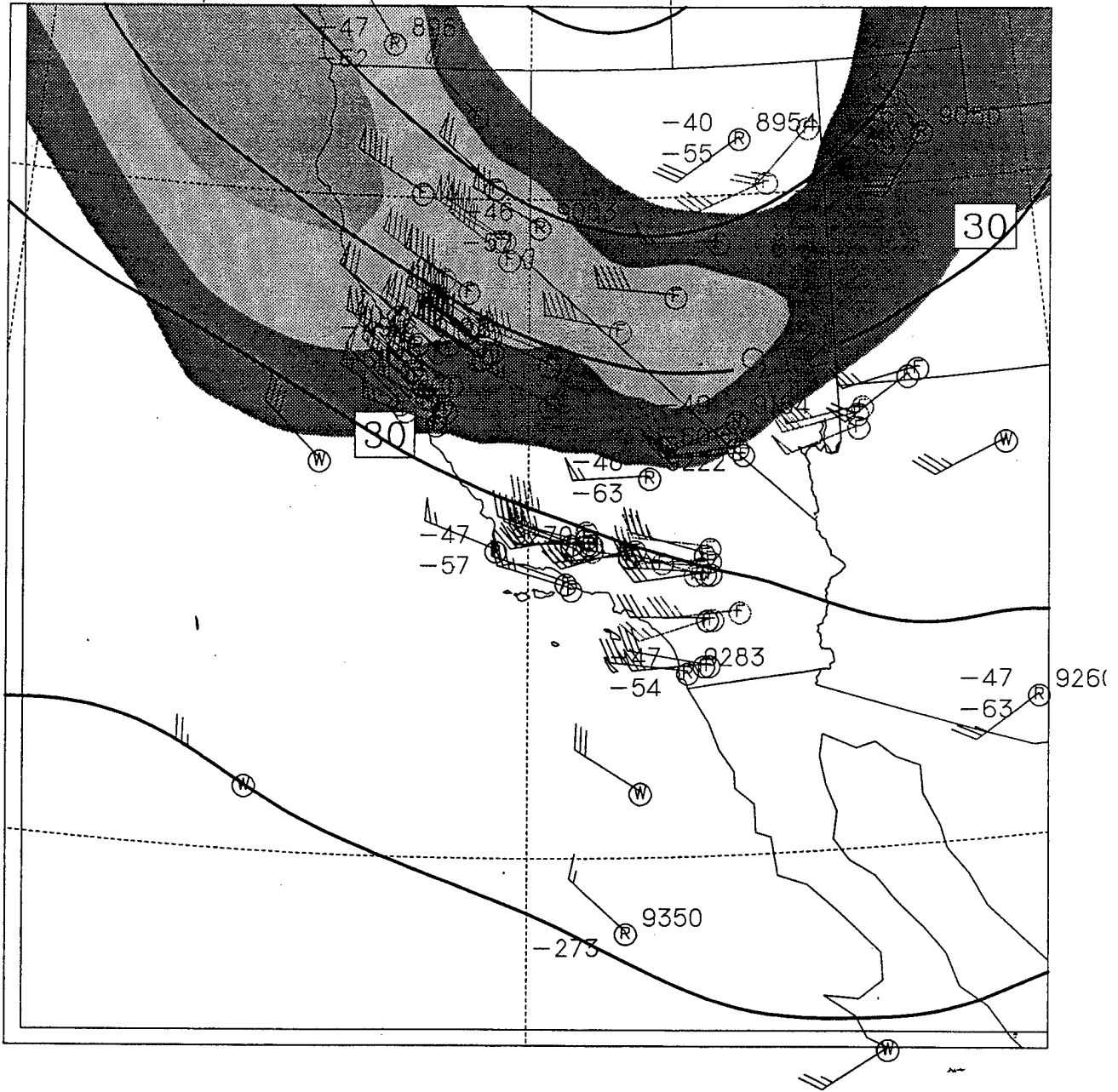
Fig. 28. COAMPS 300 mb chart at 0000 UTC 1 April 1997. Height contours are solid lines (12 dm increment), isotachs are shaded at 5 m/s increments starting at 30 m/s. Observations are in m/s: flag = 25 m/s, full barb = 5 m/s, and half barb = 2.5 m/s.
