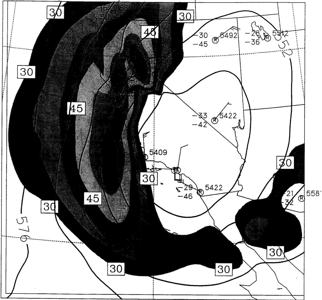
Fig. 35. COAMPS 500 mb chart at 1200 UTC 2 April 1997. Height contours are solid lines (6 dm increment). Other fields as described in Fig. 28.
