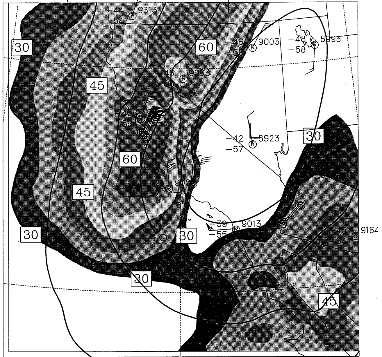
Fig. 34. Same as Fig. 28 except for 1200 UTC 2 April 1997.
