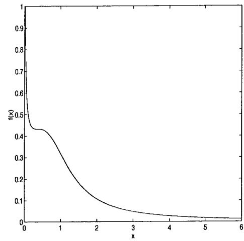
Figure 3.14 Log-Cauchy(0,1) PDF
