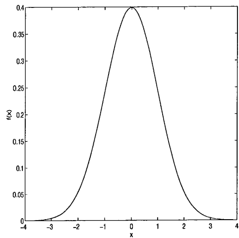
Figure 3.6 Normal(0,1) PDF
