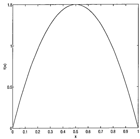
Figure 3.8 Beta(2,2) PDF
