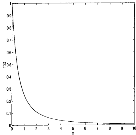
Figure 3.13 Log-logistic(0,1) PDF
