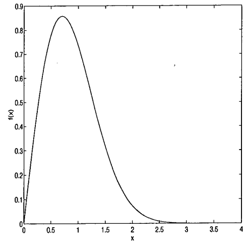
Figure 3.3 Weibull(0,1,2) PDF
