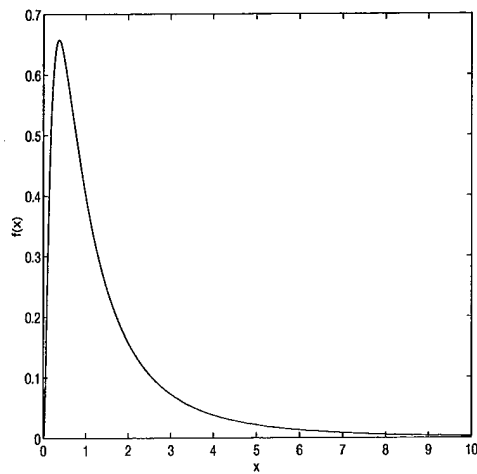
Figure 3.12 Log-normal(0,1) PDF
