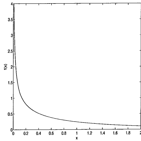
Figure 3.10 Chi-square(1) PDF
