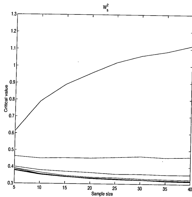
Figure 4.3 W_s^2 Critical Values vs. Sample Size, \alpha = 0.05
