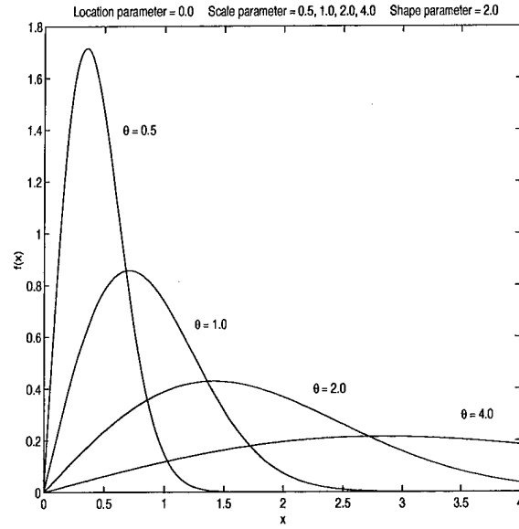
Figure 2.3 Weibull Distributions with Various Scale Parameters
