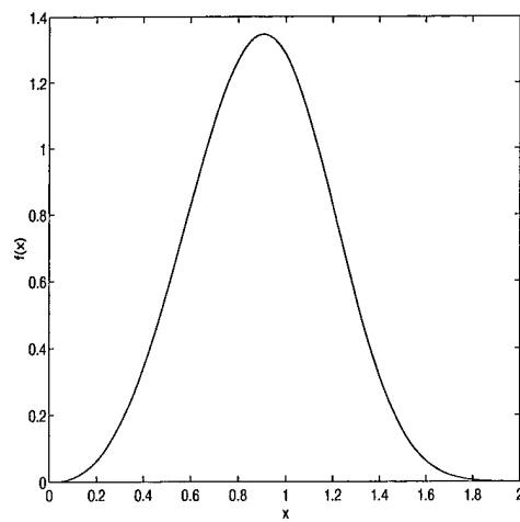
Figure 3.4 Weibull(0,1,3.5) PDF
