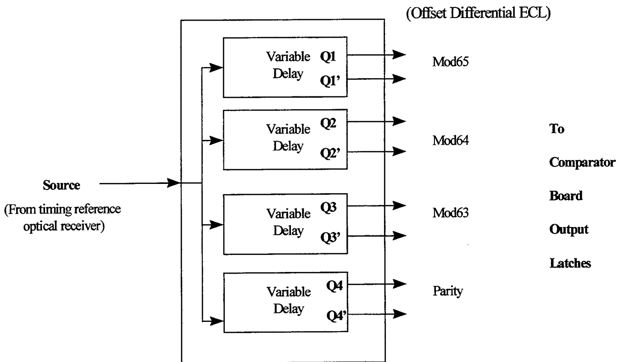
Figure (18): Adjustable delay trigger circuit block diagram
