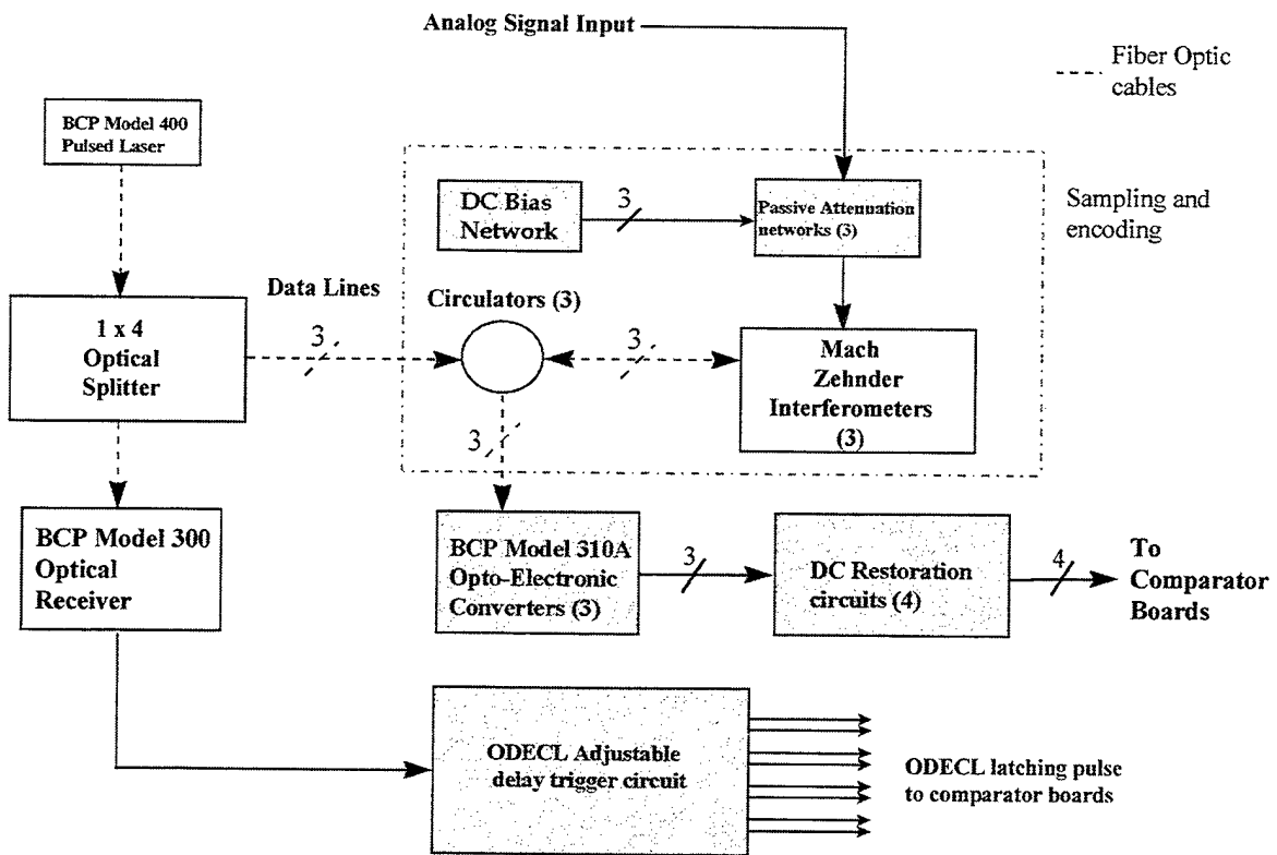
Figure (11): Analog electronic subsystem block diagram
