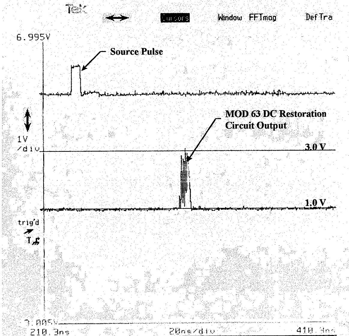
Figure (23): Mod 63 DC restoration circuit output
