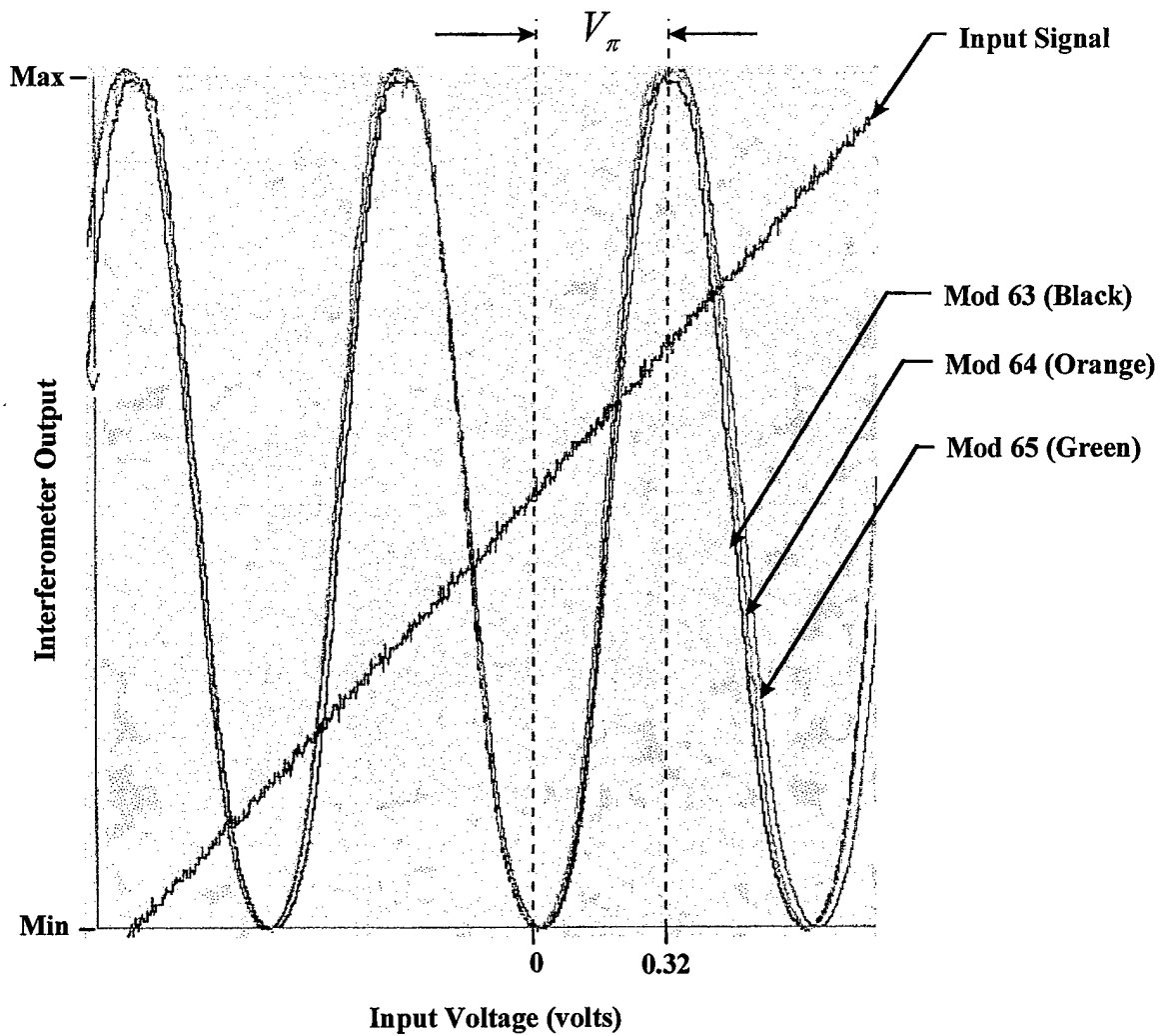
Figure (7): Interferometer outputs for a given input voltage
