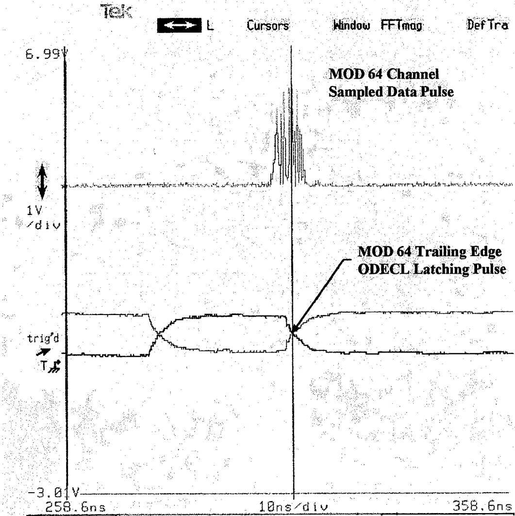
Figure (28): Mod 64 ODECL trigger alignment with data pulse
