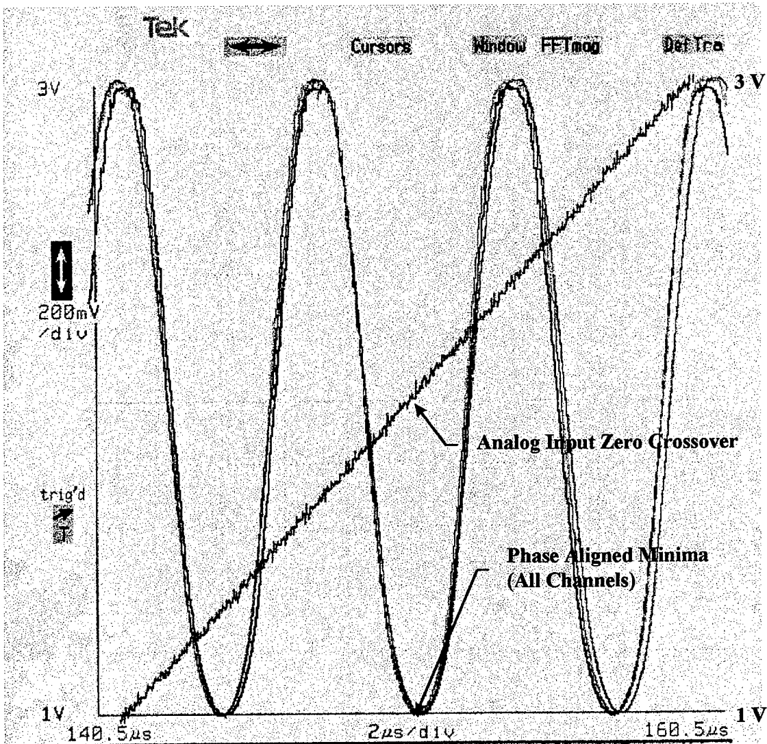
Figure (34): Combined, phase adjusted outputs versus analog input
