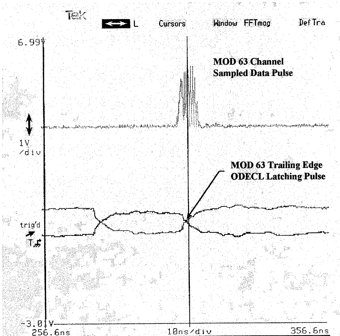
Figure (27): Mod 63 ODECL trigger alignment with data pulse
