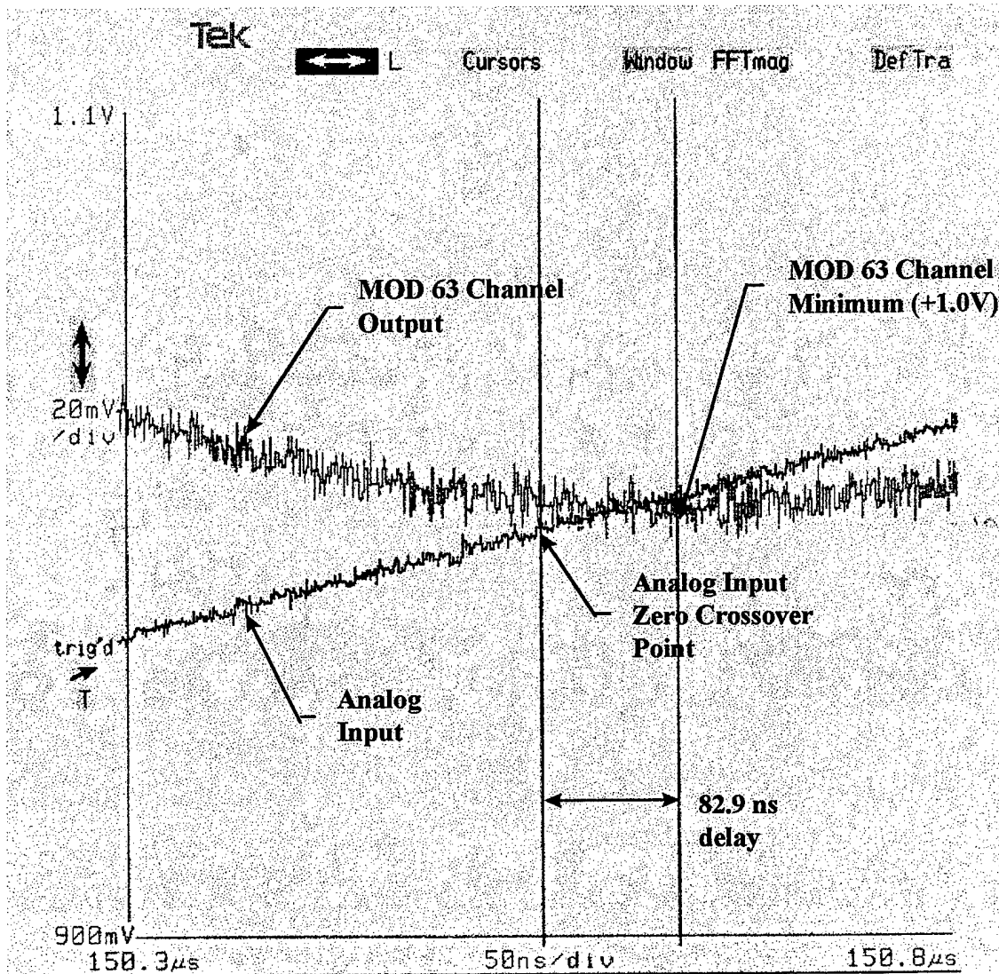
Figure (31): Phasing of Mod 63 minimum and zero crossover point
