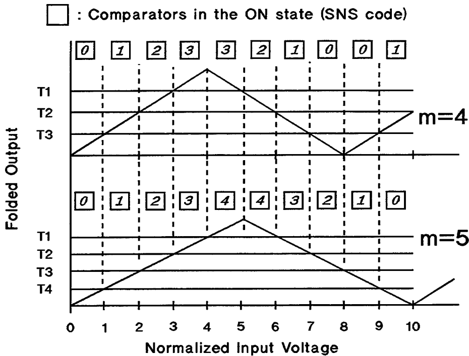
Figure (5): OSNS folding waveforms and output codes for m_1 = 4 and m_2 = 5 .
