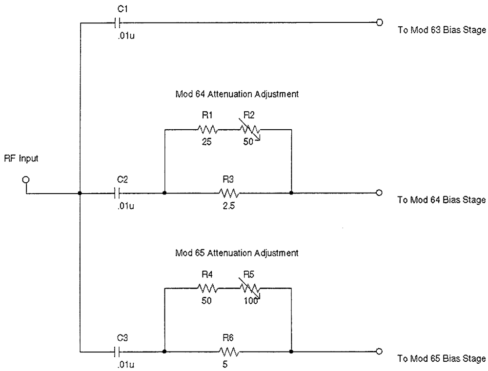
Figure (15): Attenuation network schematic diagram
