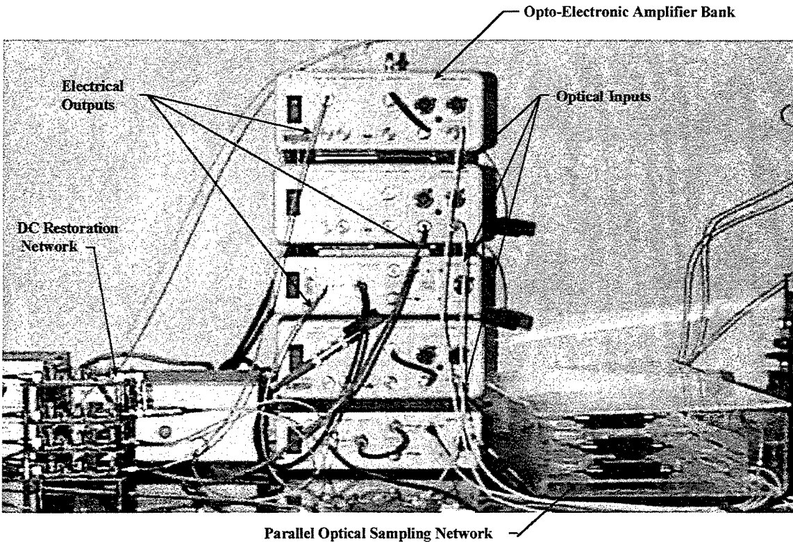
Figure (10): Laboratory configuration of opto-electronic converter/amplifier bank
