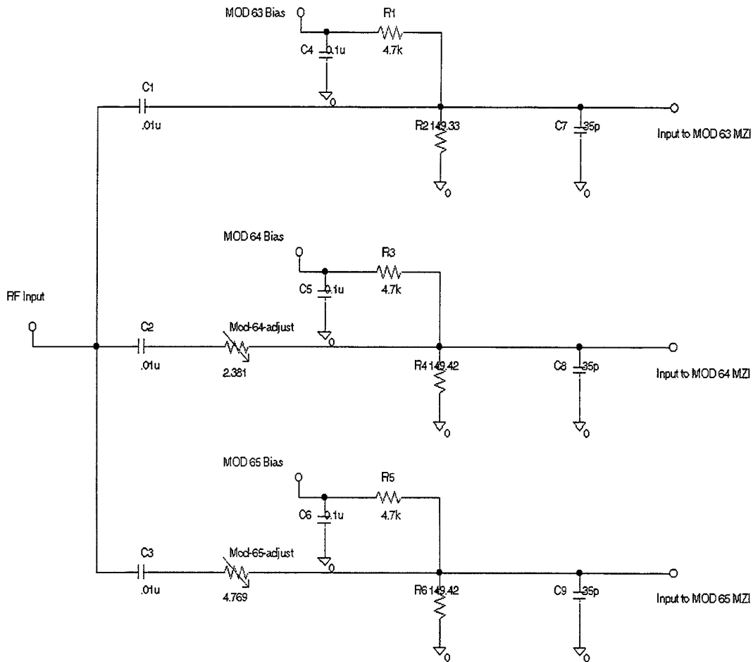
Figure (12): DC bias network schematic
