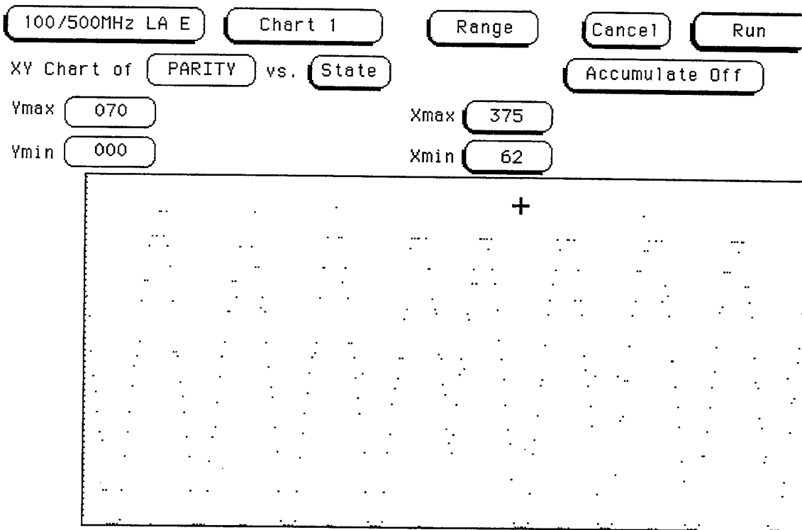
Figure (35): Digital output of Parity channel for a triangle wave antenna input
