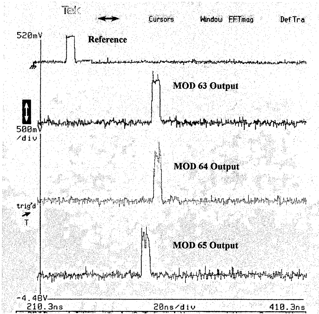
Figure (22): Comparison of interferometer outputs with the reference pulse
