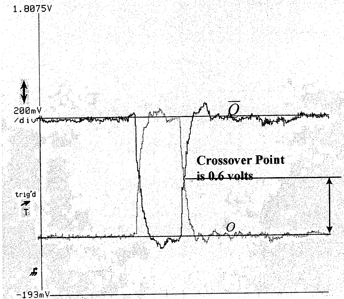
Figure (21): Offset differential emitter coupled logic latching pulse
