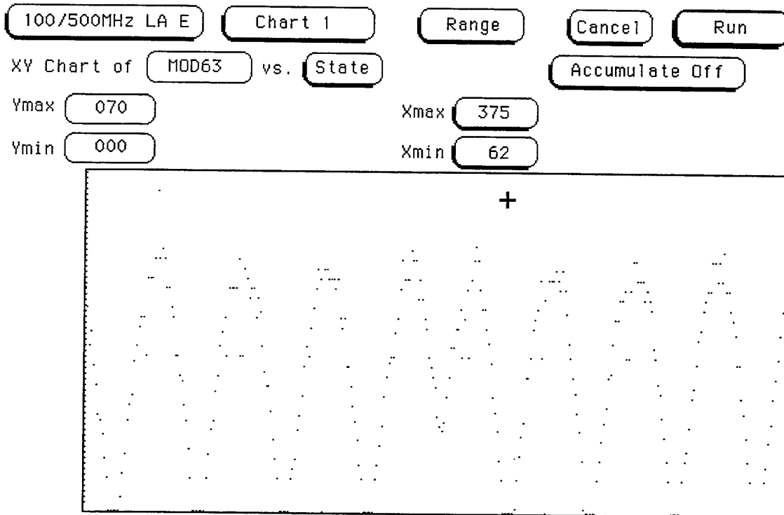
Figure (37): Digital output of Mod 63 channel for triangle wave antenna input
