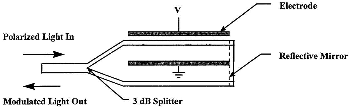
Figure (6): Mach-Zehnder interferometer
