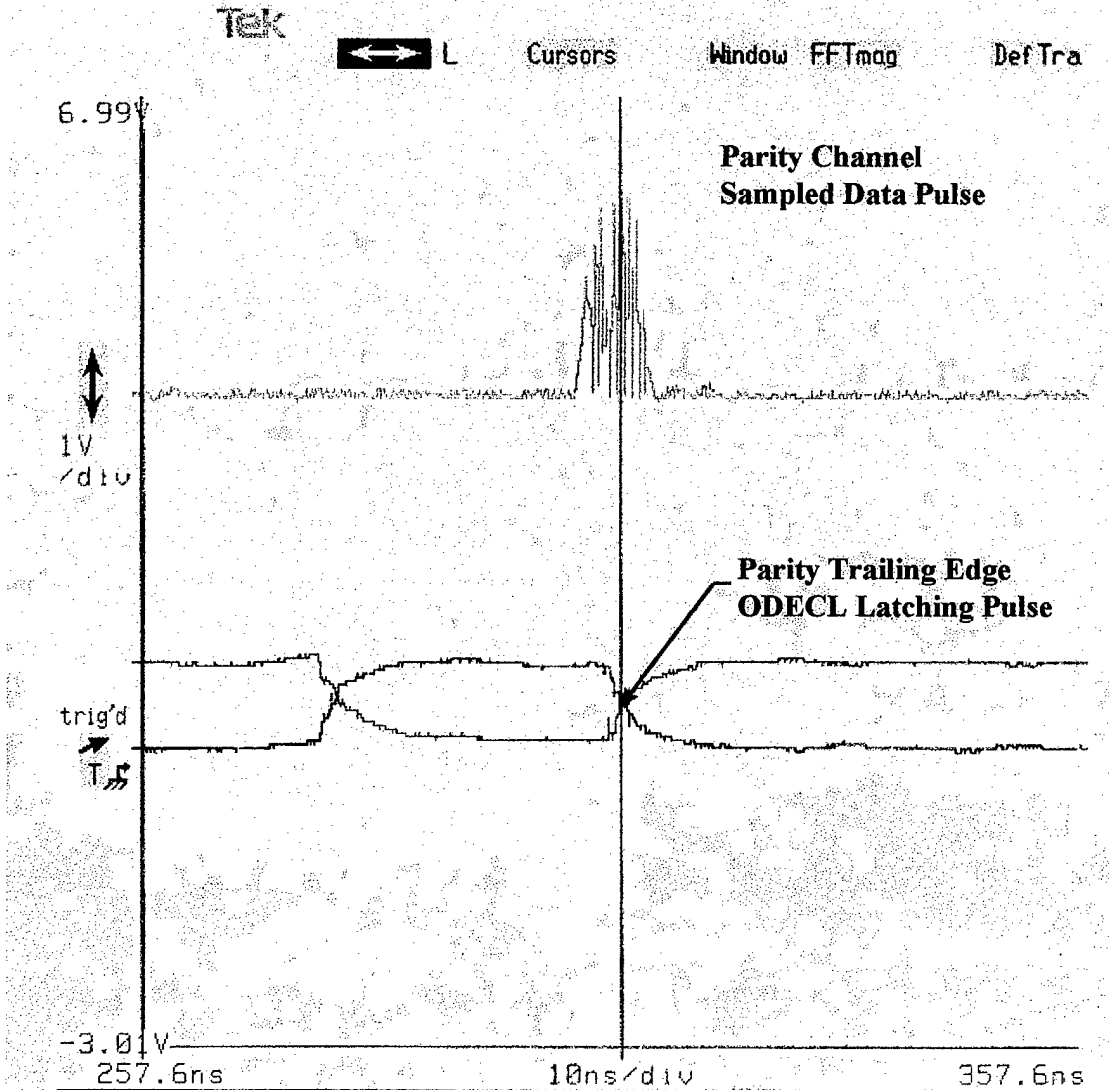
Figure (26): ODECL trigger circuit alignment with data pulse
