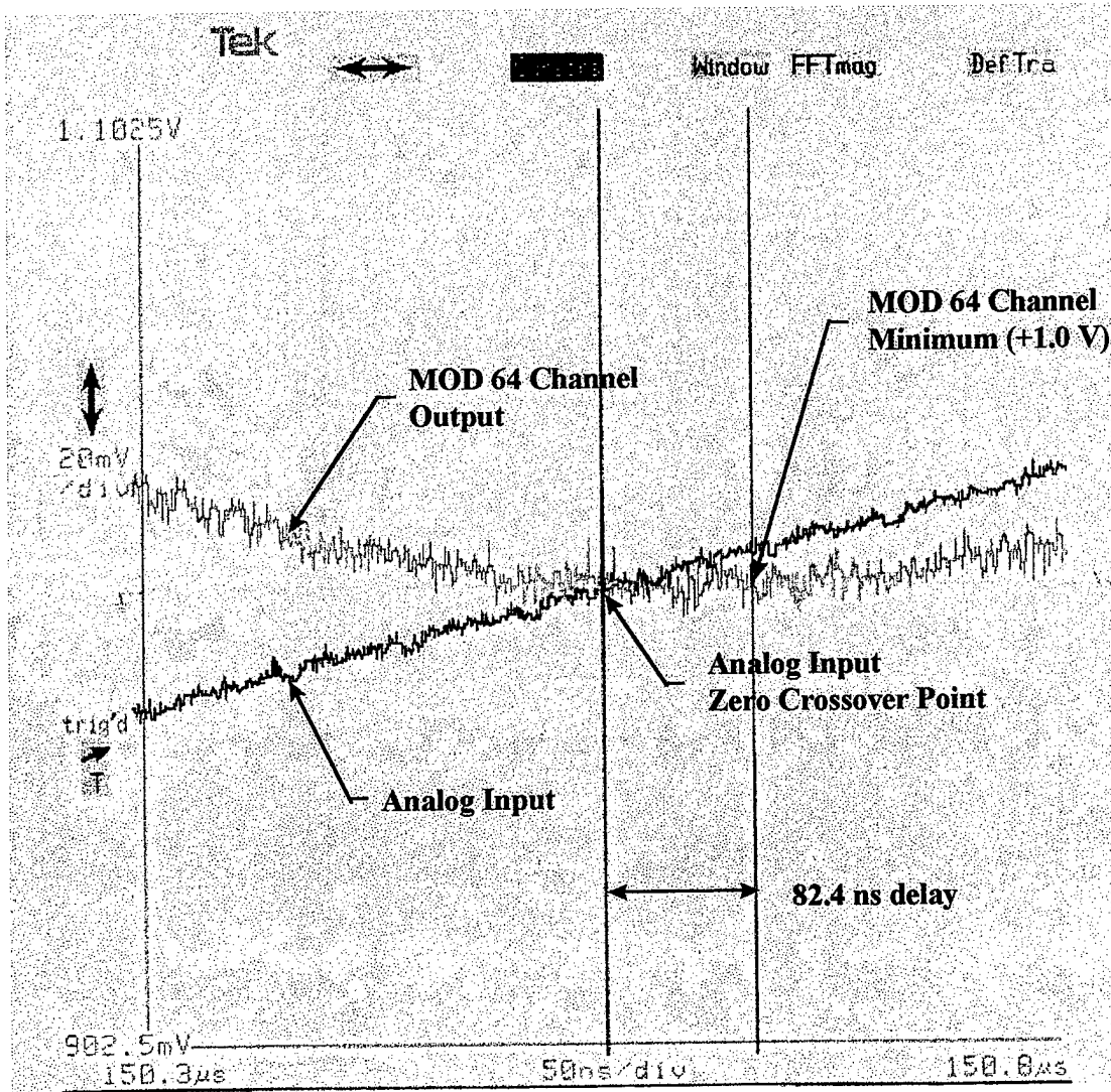
Figure (32): Phasing of the Mod 64 minimum and the zero crossover point
