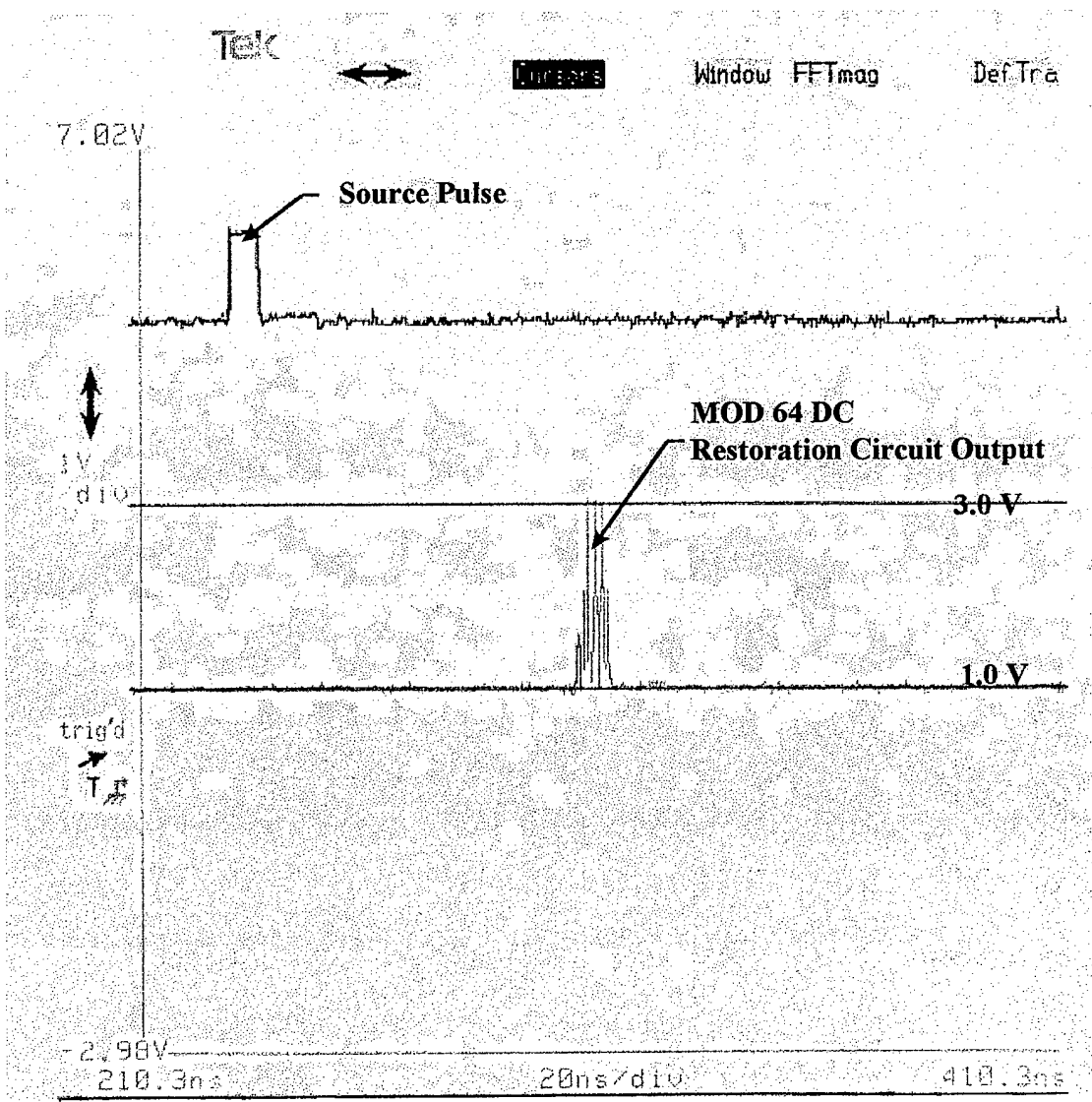
Figure (24): Mod 64 DC restoration circuit output
