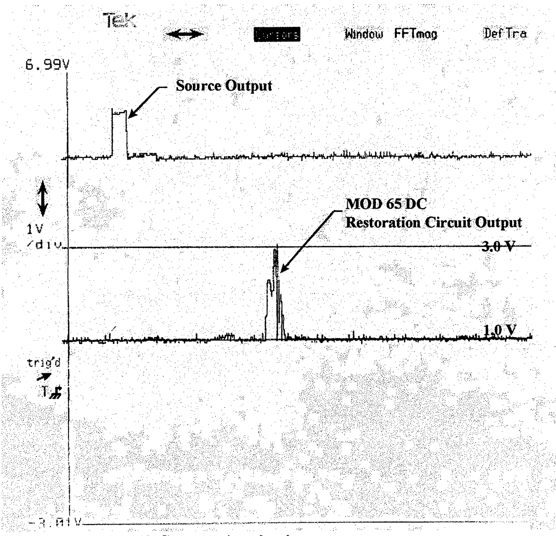
Figure (25): Mod 65 DC restoration circuit output
