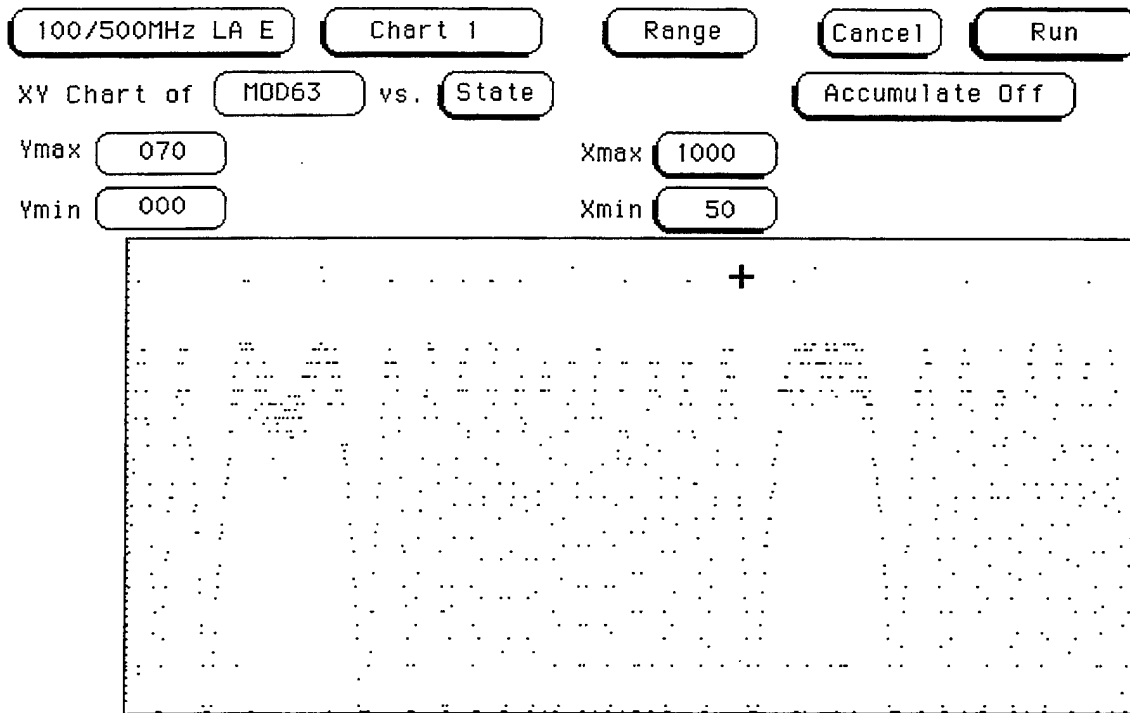
Figure (38): Digital code output of Mod 63 channel for sinusoidal antenna input
