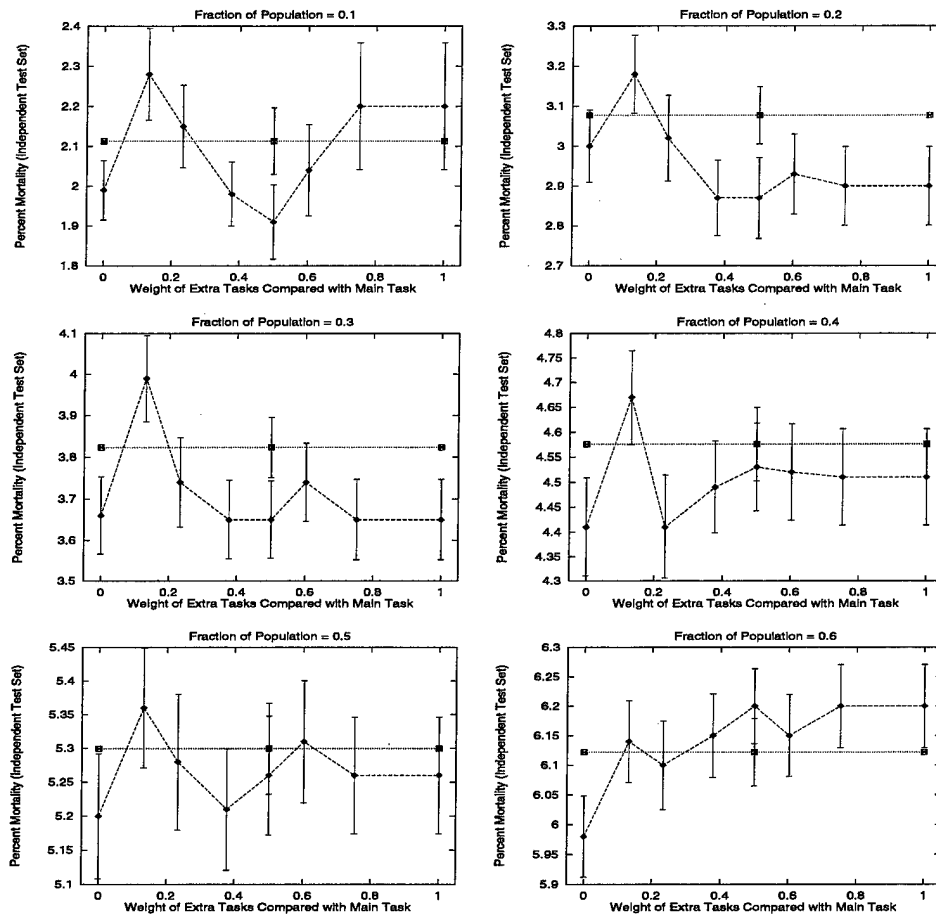
Figure 7.9: Performance on Different Fractions of the Population as \lambda Varies using the Attributes as the Extra MTL Tasks (Train = 500; Halt = 500)
