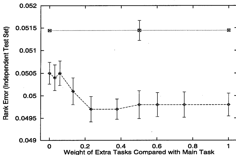
Figure 7.5: Rank Sum Error as a Function of \lambda During MTL (Train = 1000; Halt = 1000; RunTime = 1000+1000)
