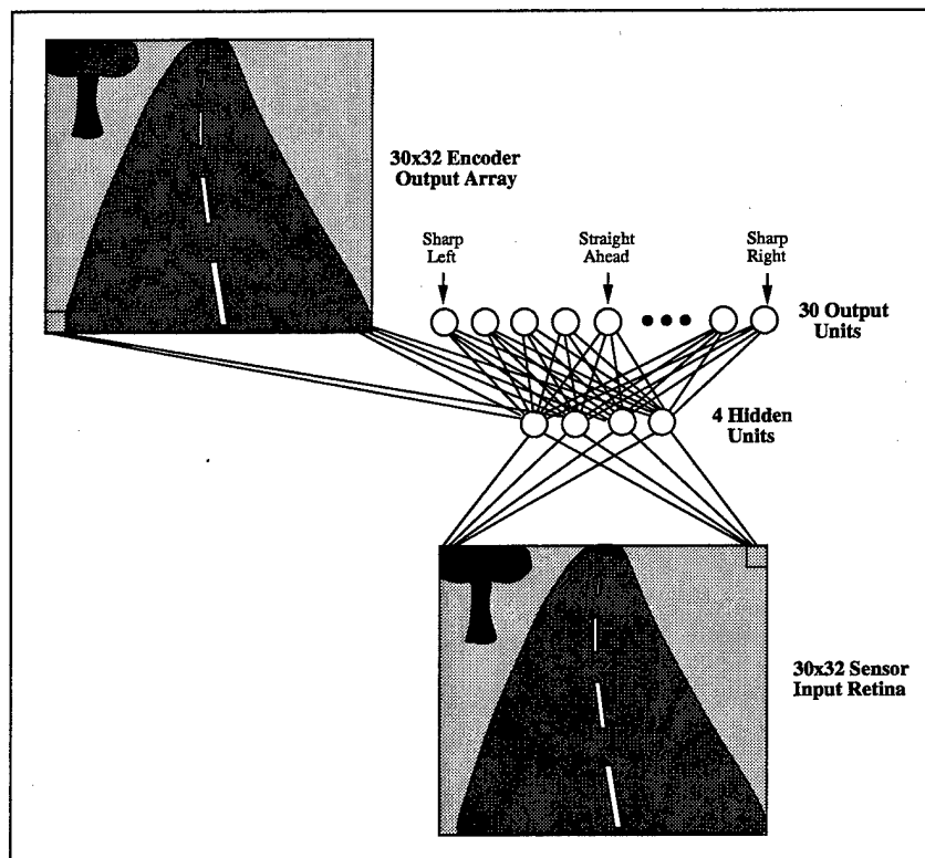
Figure 8.3: IRE Net for Assessing Prediction Confidences in ALVINN (courtesy Dean Pomerleau).
