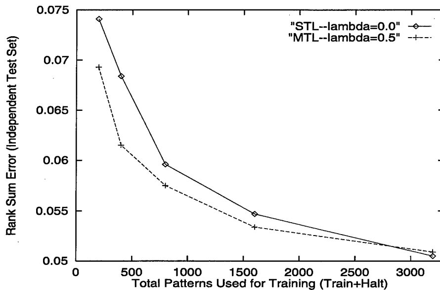
Figure 7.7: Rank Sum Error of STL ( \lambda = 0 ) and MTL ( \lambda = 0.5 ) as a Function of the Size of the Training+Halt Sets
