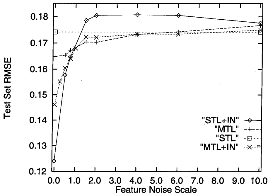
Figure 5.13: Performance on F3(A,B) of STL with the regular inputs, STL with the extra input for EF(A) and EF(B), and MTL with extra output tasks for EF(A) and EF(B).
