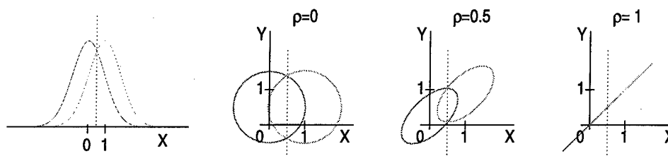
Figure 5.7: Two overlapped Gaussian classes (left), and an extra feature (y-axis) correlated different amounts ( \rho = 0 : no correlation, \rho = 1 : perfect correlation) with the unencoded version of the regular input (x-axis)
