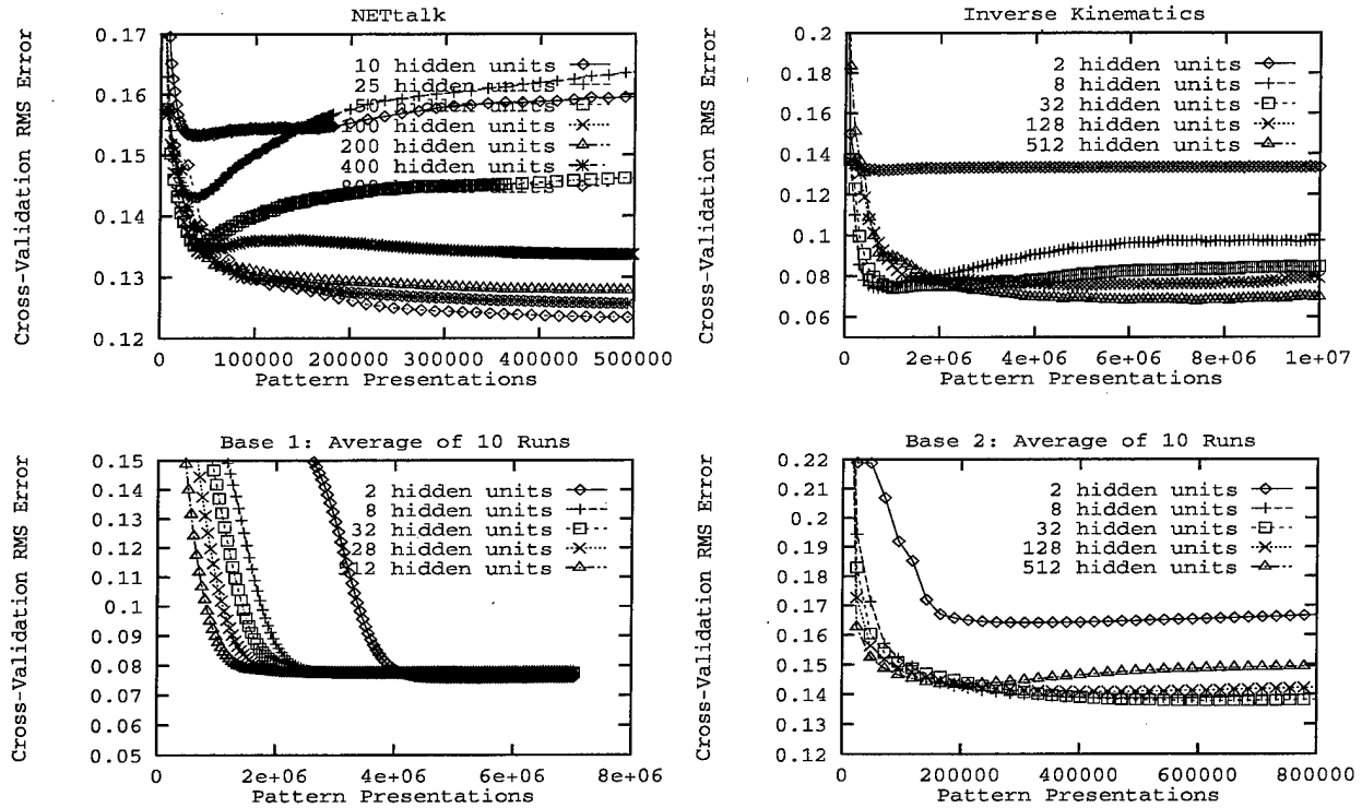
Figure A.1: Generalization Performance vs. Network Size for Four of the Test Problems
