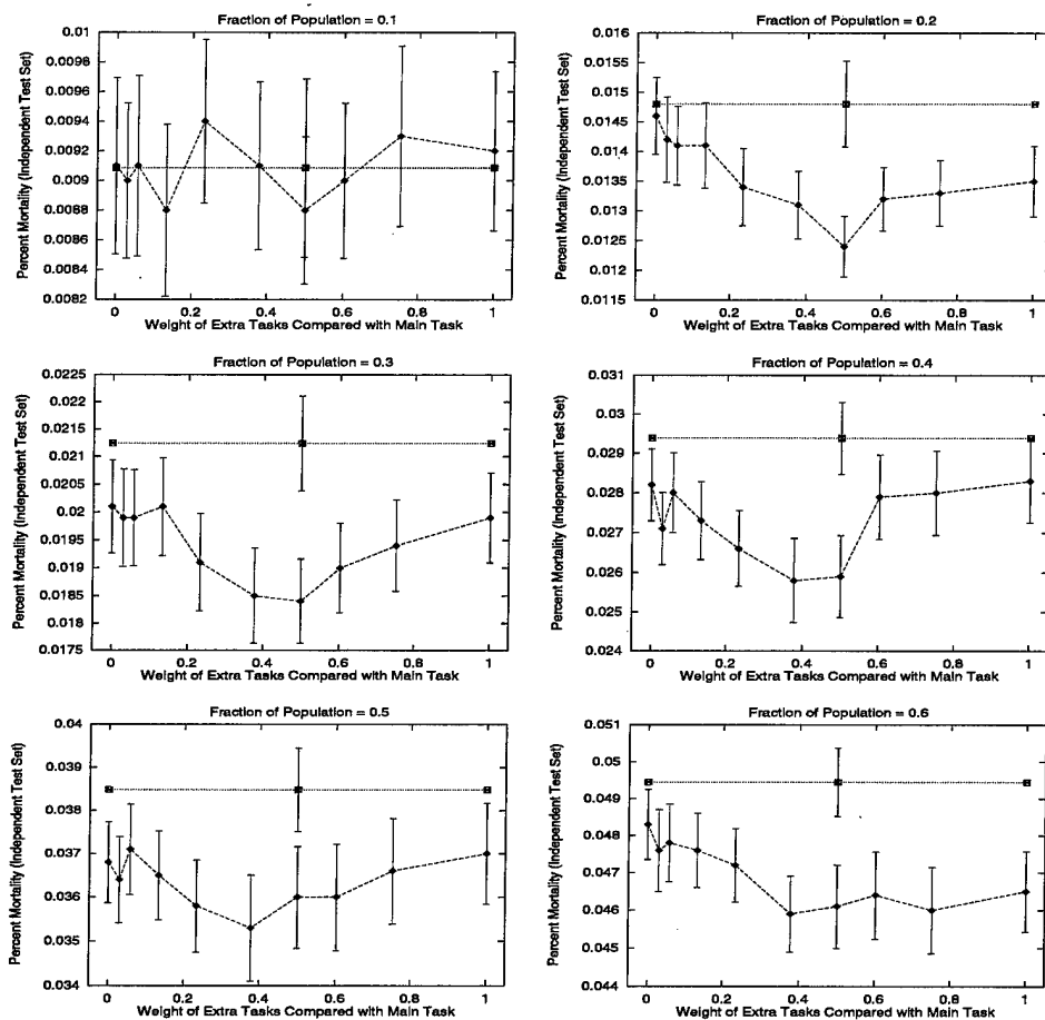
Figure 7.6: Performance on Different Fractions of the Population as \lambda Varies (Train = 1000; Halt = 1000; RunTime = 1000+1000)
