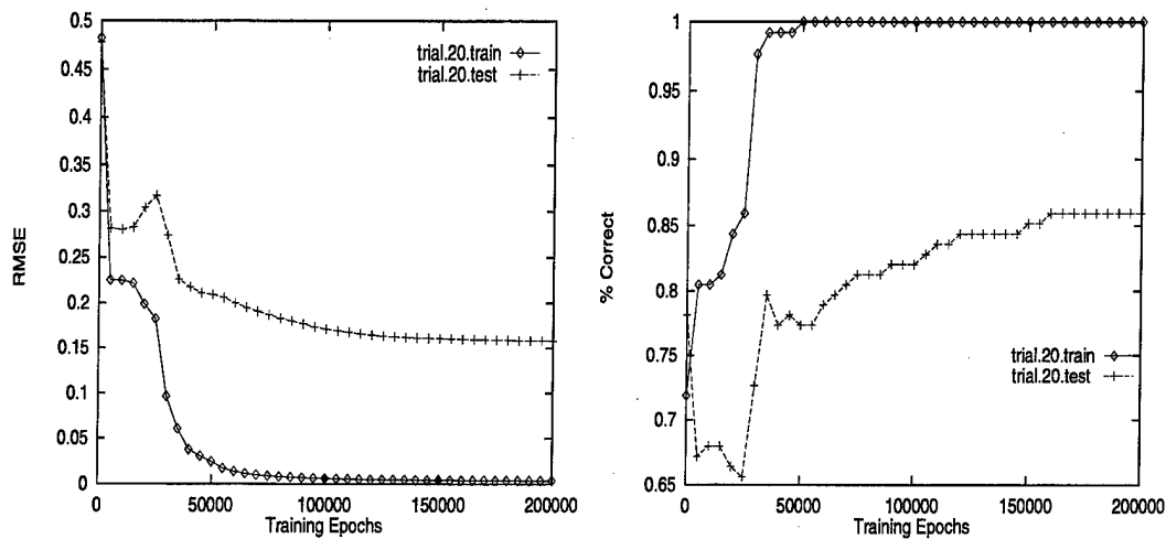
Figure 1.4: Training curves for one run of backprop STL on Task 1
