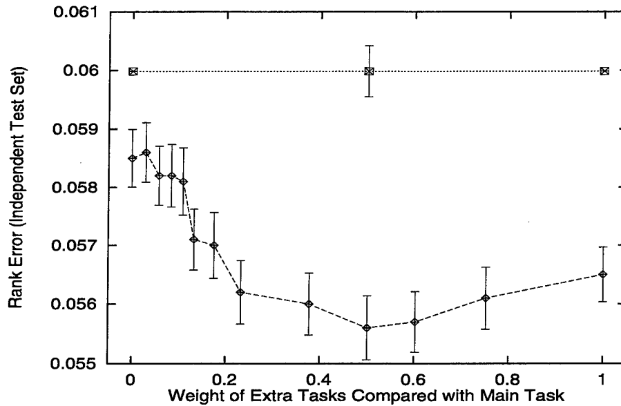
Figure 7.1: Rank Sum Error as a function of MTL's \lambda (Train = 500 cases; Halt = 500 cases). \lambda = 0 is STL; the extra tasks are ignored. The horizontal line near the top of the graph is the performance before feature weights are trained. This is the performance of simple, unweighted Euclidean distance.
