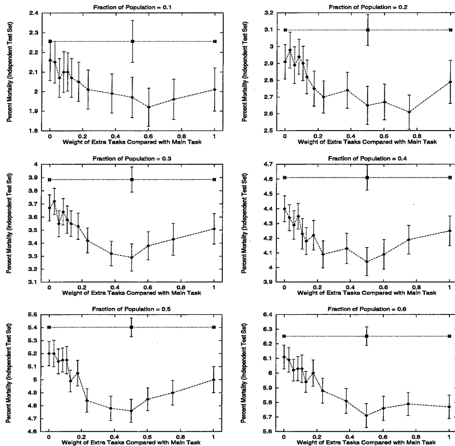
Figure 7.2: Performance on Different Fractions of the Population as \lambda Varies (Train = 500; Halt = 500)
