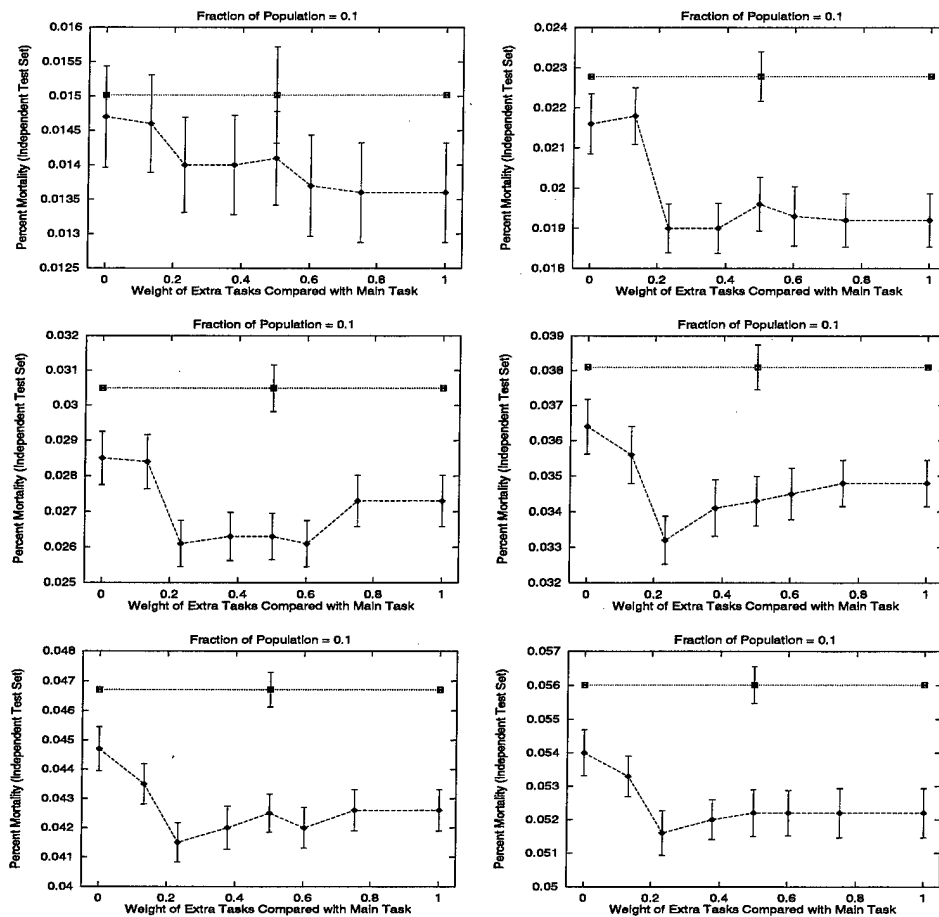
Figure 7.4: Performance on Different Fractions of the Population as \lambda Varies (Train = 1000; Halt = 1000)
