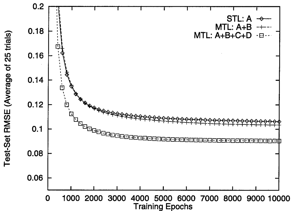
Figure 1.8: RMSE Test-set Performance of Three Different Nets on Task A.
