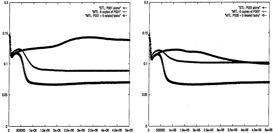
Figure 3.3: Generalization performance of STL, MTL with six copies of the same task, and MTL with six strongly related tasks on P001 (left) and P005 (right). The vertical axis is the RMS error on the test set. Lower error indicates better performance. The horizontal axis is the number of backprop passes. In each graph the best performing curve is for MTL with six strongly related tasks. In the left graph MTL with six copies of P001 performs better than STL of P001, but in the right graph STL of P005 performs slightly better than six copies of P005.
