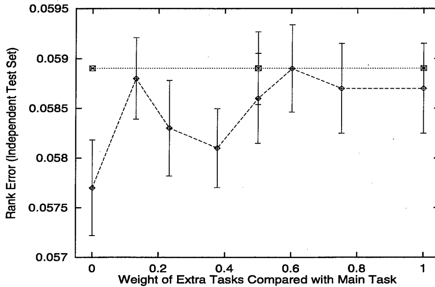
Figure 7.8: Rank Sum Error as a Function of \lambda During MTL using the Attributes as the Extra Tasks (Train = 500; Halt = 500) The horizontal line is the baseline performance with all weights initialized to 1. The lower curve is the performance of the weights trained with MTL as a function of \lambda . As before, \lambda = 0 ignores the extra tasks completely and is thus equivalent to STL.
