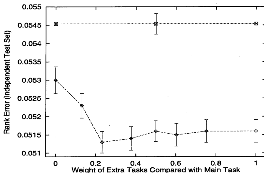
Figure 7.3: Rank Sum Error as a Function of \lambda During MTL (Train = 1000; Halt = 1000)
