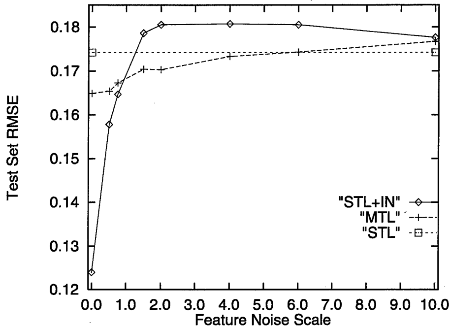
Figure 5.6: Performance on F3(A,B) of STL with the regular inputs, STL with the extra input for EF(A) and EF(B), and MTL with extra output tasks for EF(A) and EF(B).
