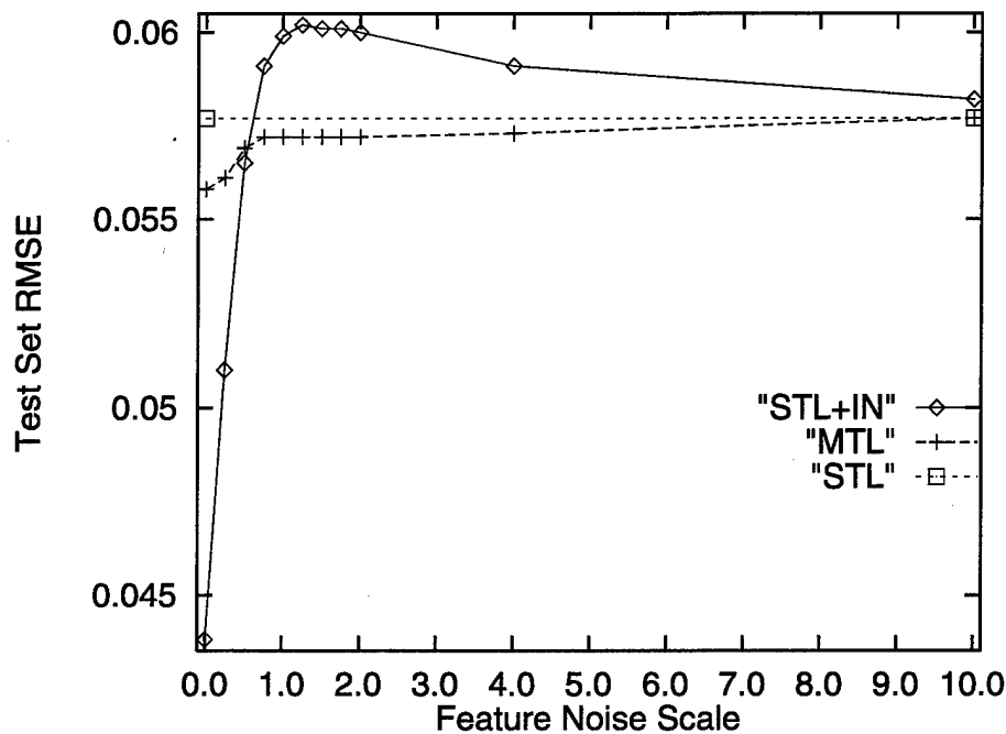
Figure 5.5: Performance on F1(A,B) of STL with the regular inputs, STL with the extra input for F2(A,B) , and MTL with the extra output task for F2(A,B) .
