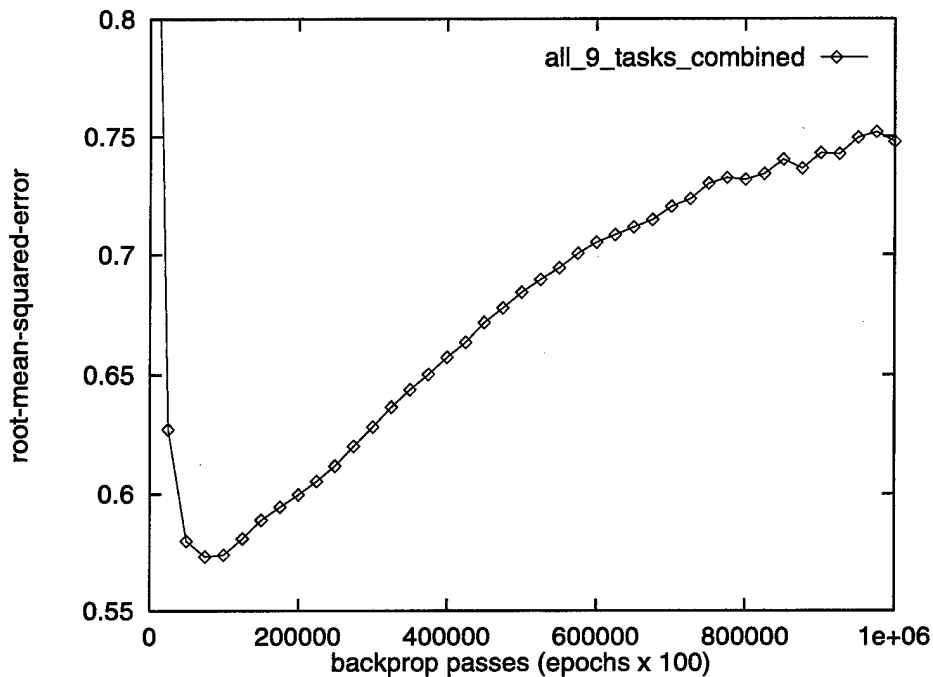
Figure 6.2: Combined Test-Set Performance on all 1D-ALVINN Tasks.
