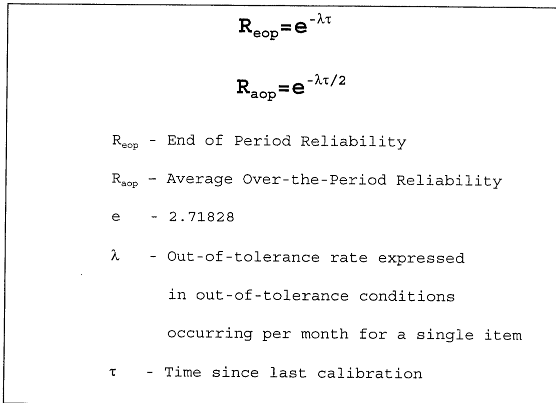
Figure 3. Exponential Distribution Probability Model (Dwyer, 1997)
