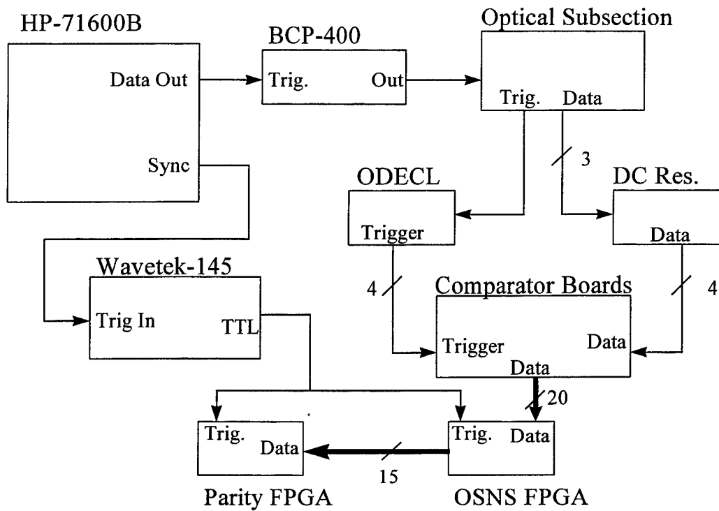
Figure 26 Trigger diagram.
