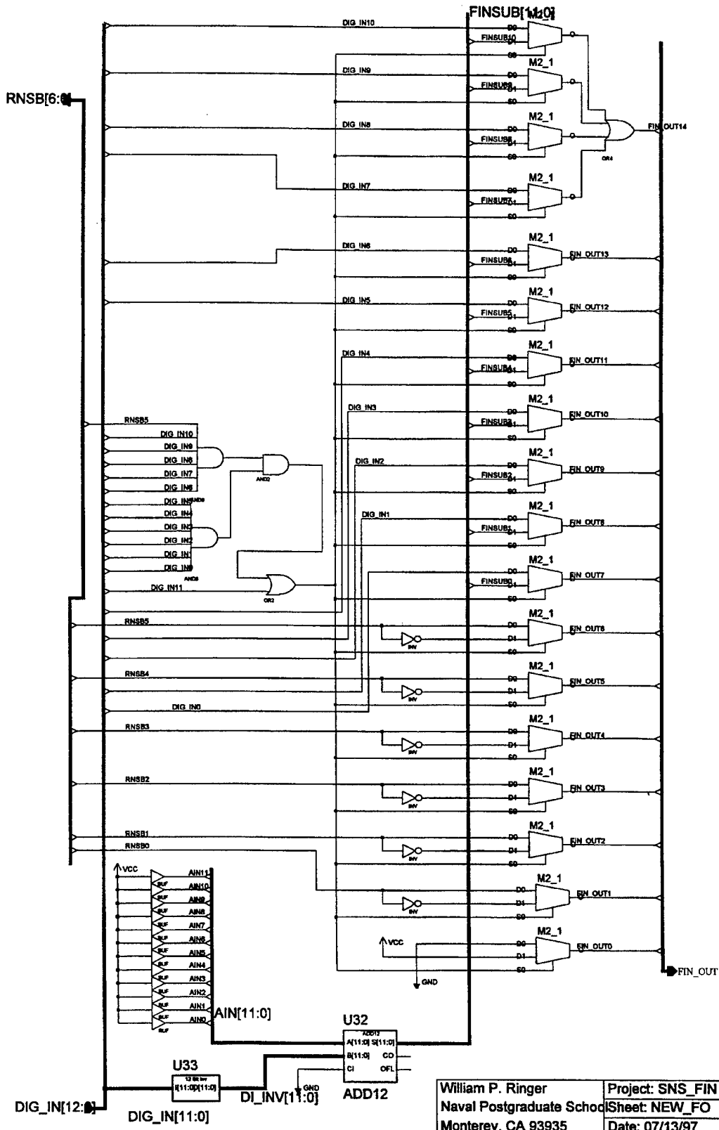
Figure 80 NEWFO schematic.
