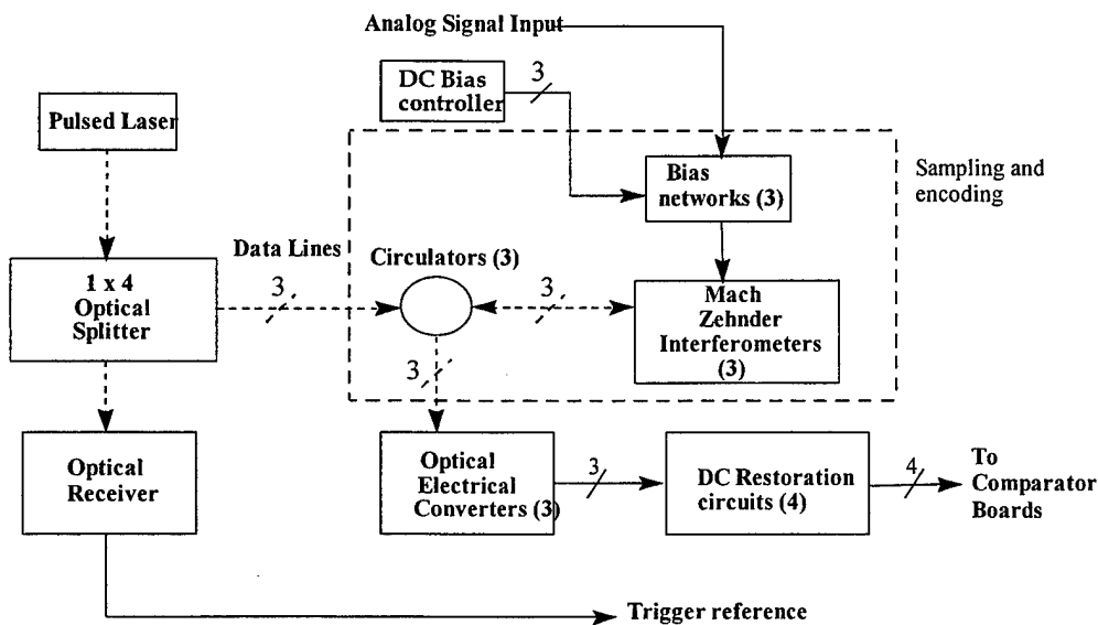
Figure 3 Optical Subsection.
