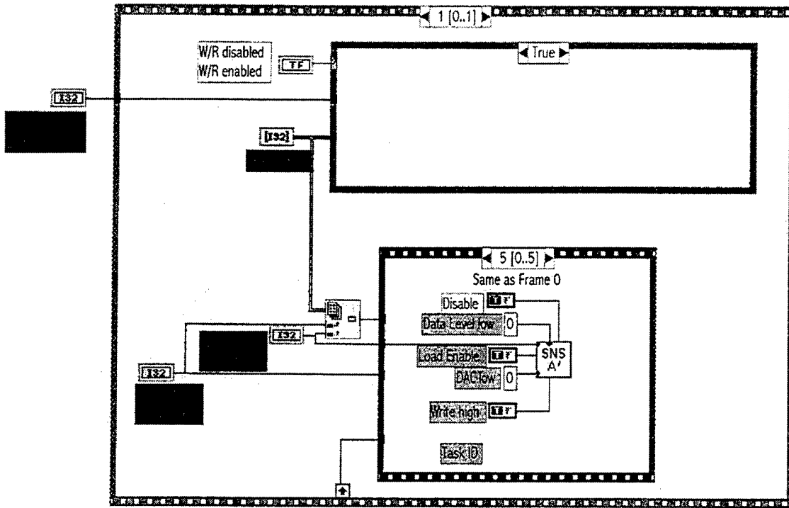
Figure 50 SNS_Control4g vi internal diagram (1 of 7).
