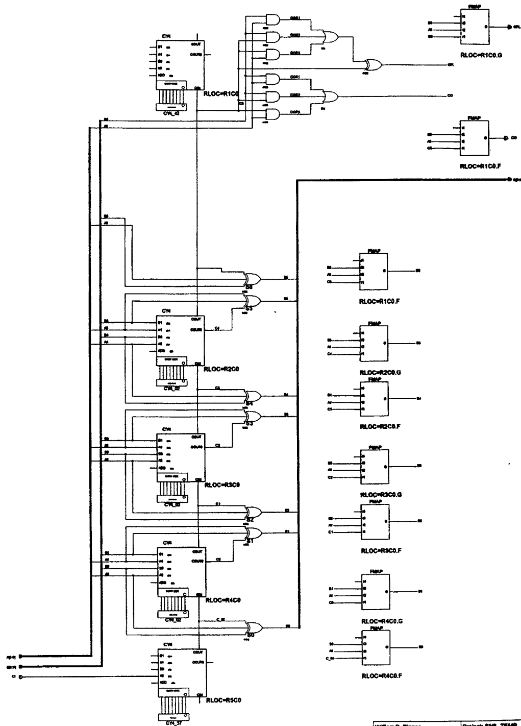
Figure 70 ADD7 schematic
