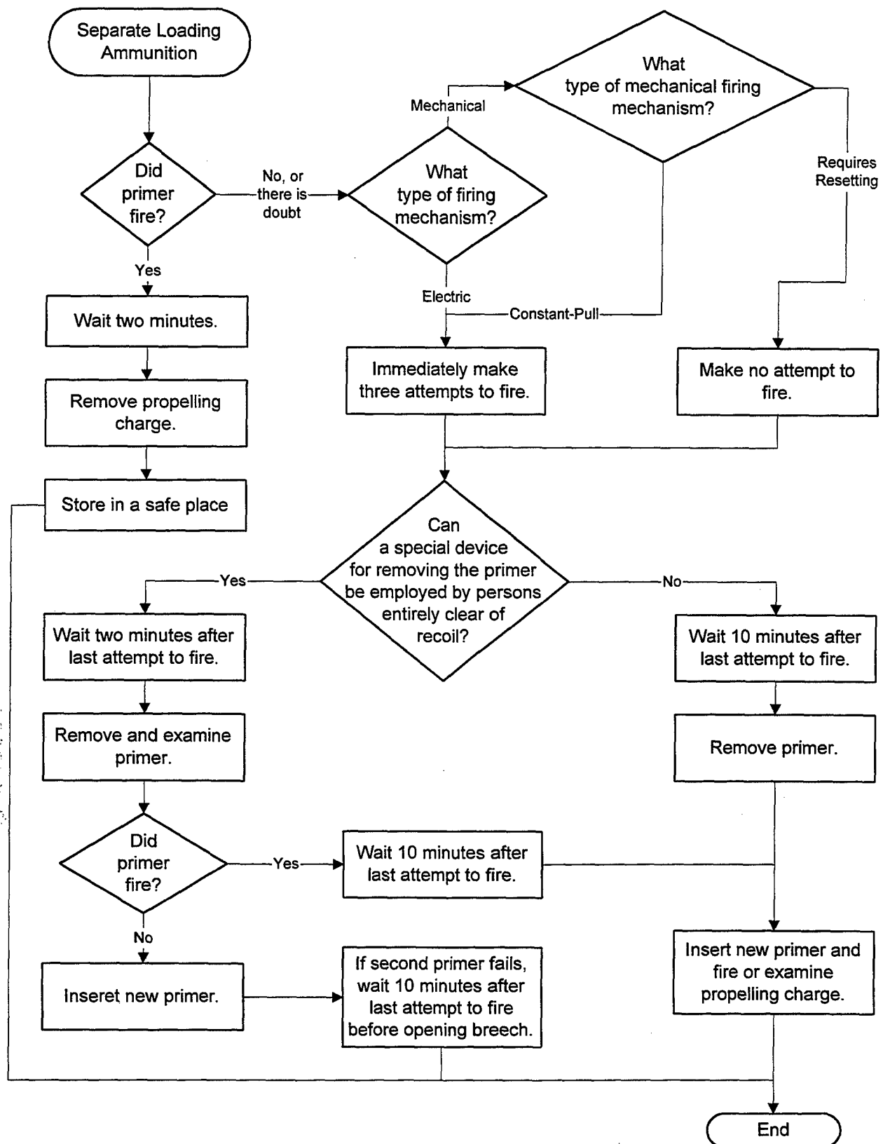
Figure 14-8. Misfire of Separate Loading Ammunition.
