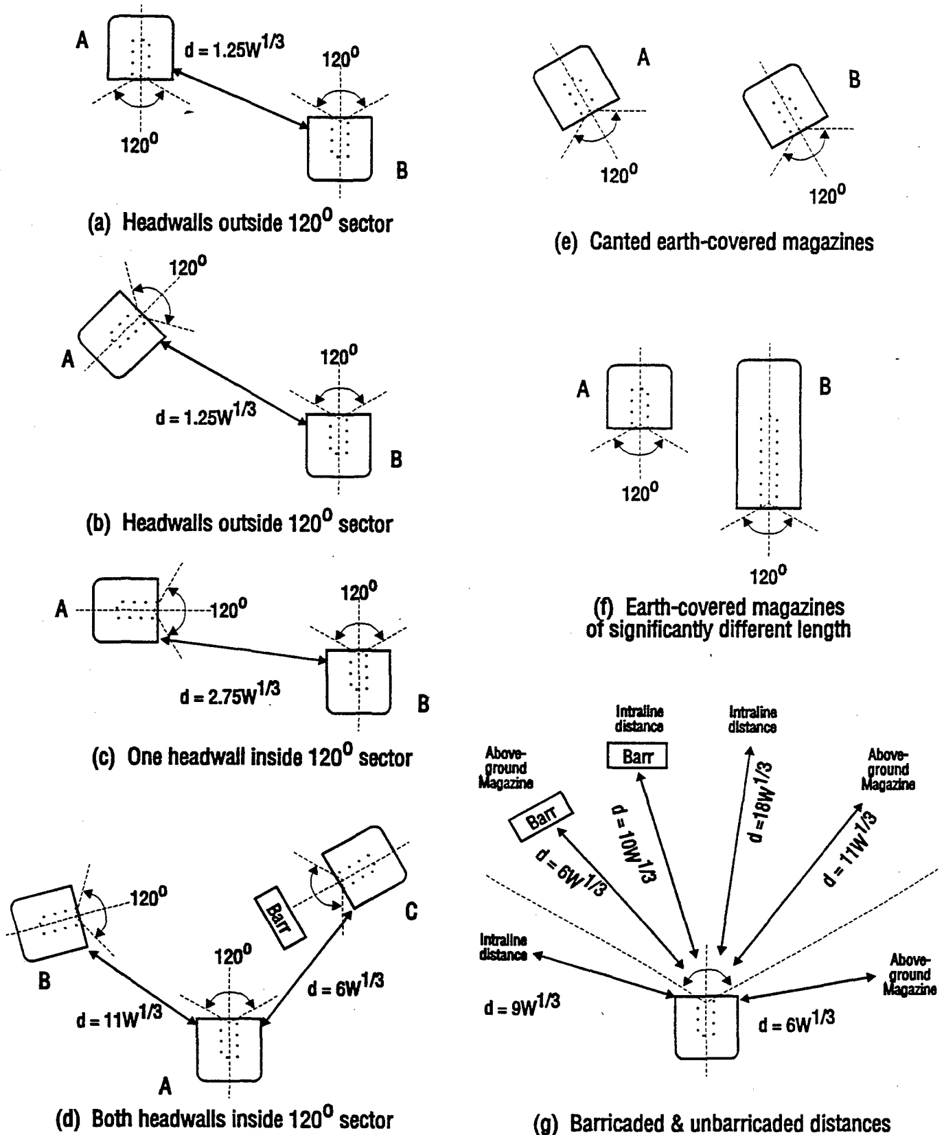
Figure 6-1. Effects of Magazine Orientation on Q-D.
