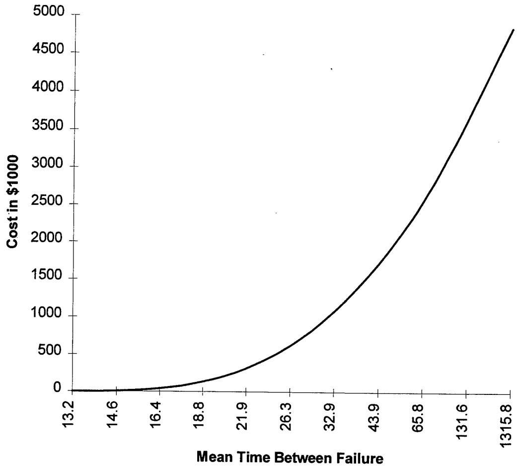
Figure 4.4. Reliability Improvement Cost Function
