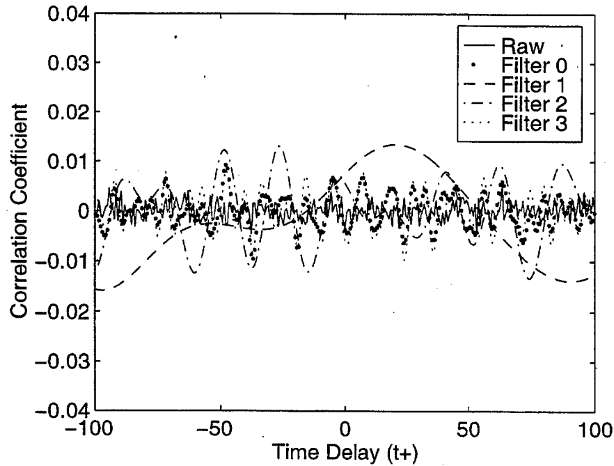
Figure 3.9: The effects of band-pass filtering on the cross-correlation function between two independently obtained white noise signals
