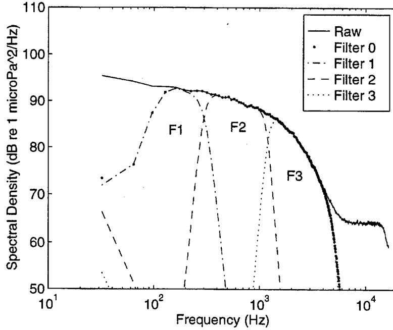
Figure 3.1: The spectral effects of band-pass filters on typical wall pressure signal ( U_0 = 15.3 m/s)
