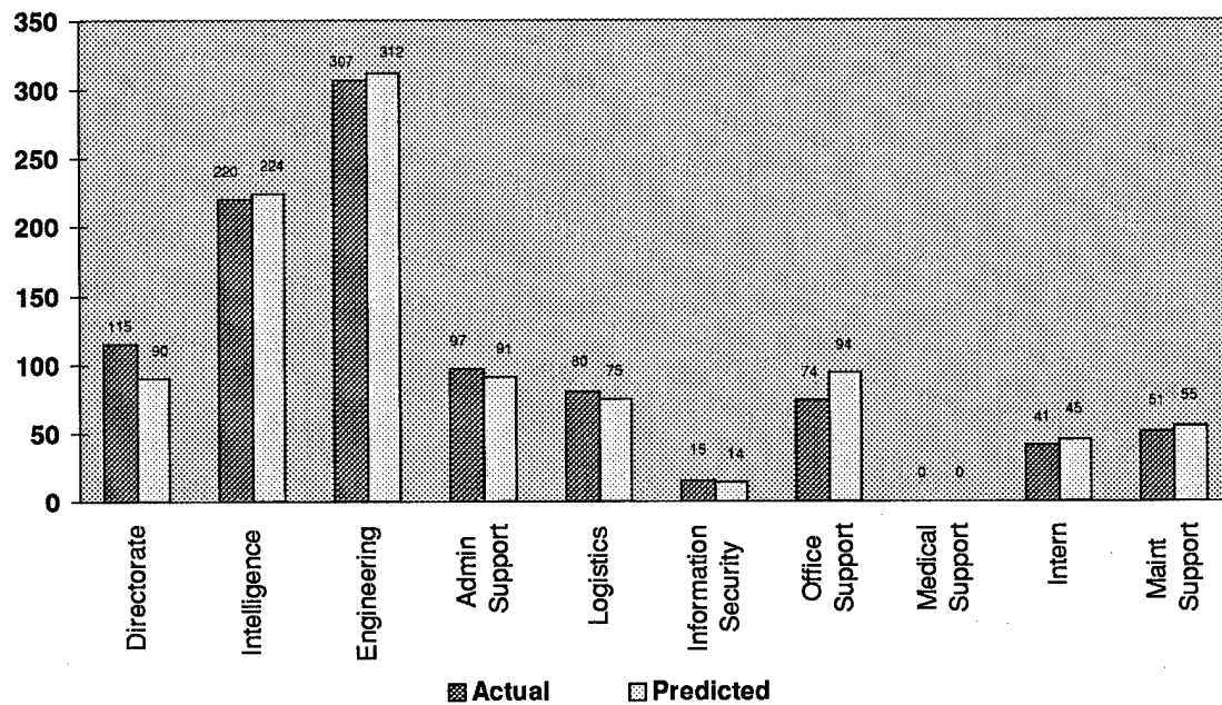
Figure 8. Validation Results for Migrations Model
