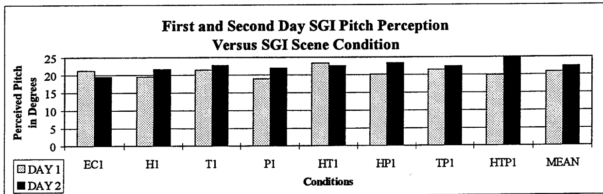
Figure 5. Graph of the first and second day means (N=16) of the somatogravic perceived pitch plotted against the various scene conditions.
