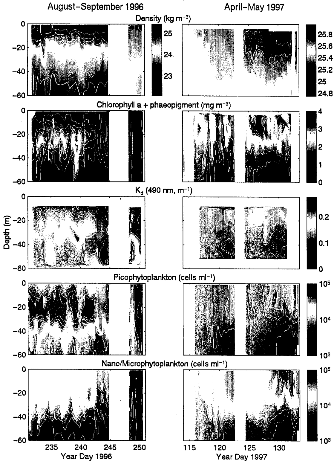
Figure 1. Time series of depth profiles observed during intensive sampling conducted at 40^\circ 30' \text{ N } 70^\circ 30' \text{ W} during late summer 1996 (left panels) and spring 1997 (right panels). Panels top to bottom: Density, chlorophyll a + phaeopigment concentration (data provided by Dr. Collin Roesler, U. Conn.), diffuse attenuation for downwelling irradiance at 490 nm, picophytoplankton (genus Synechococcus ) cell concentration, nano/microphytoplankton cell concentration.
