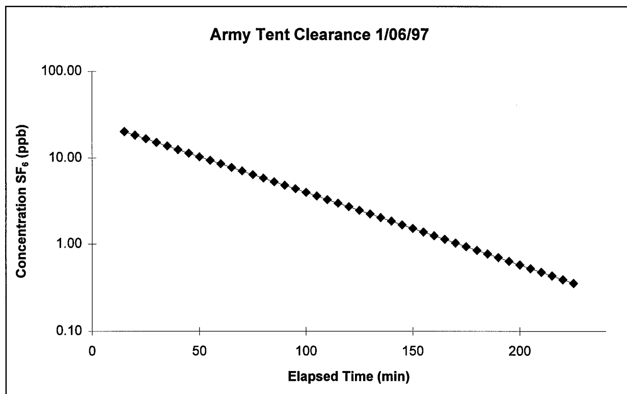
Figure 4 \text{SF}_6 Concentration decay as a function of time
