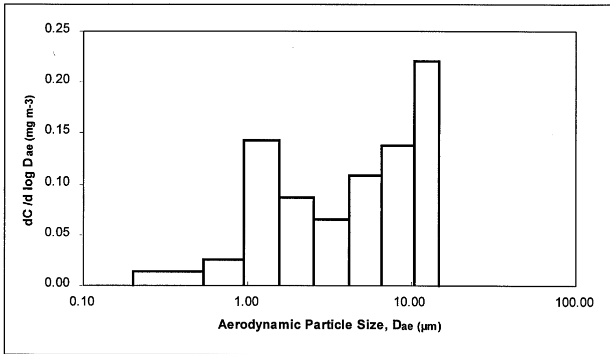
Figure 10. Particle size distribution from LMJ impactor
