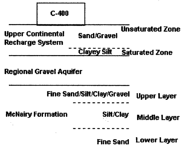
Figure 3-5 Subsurface Formations
