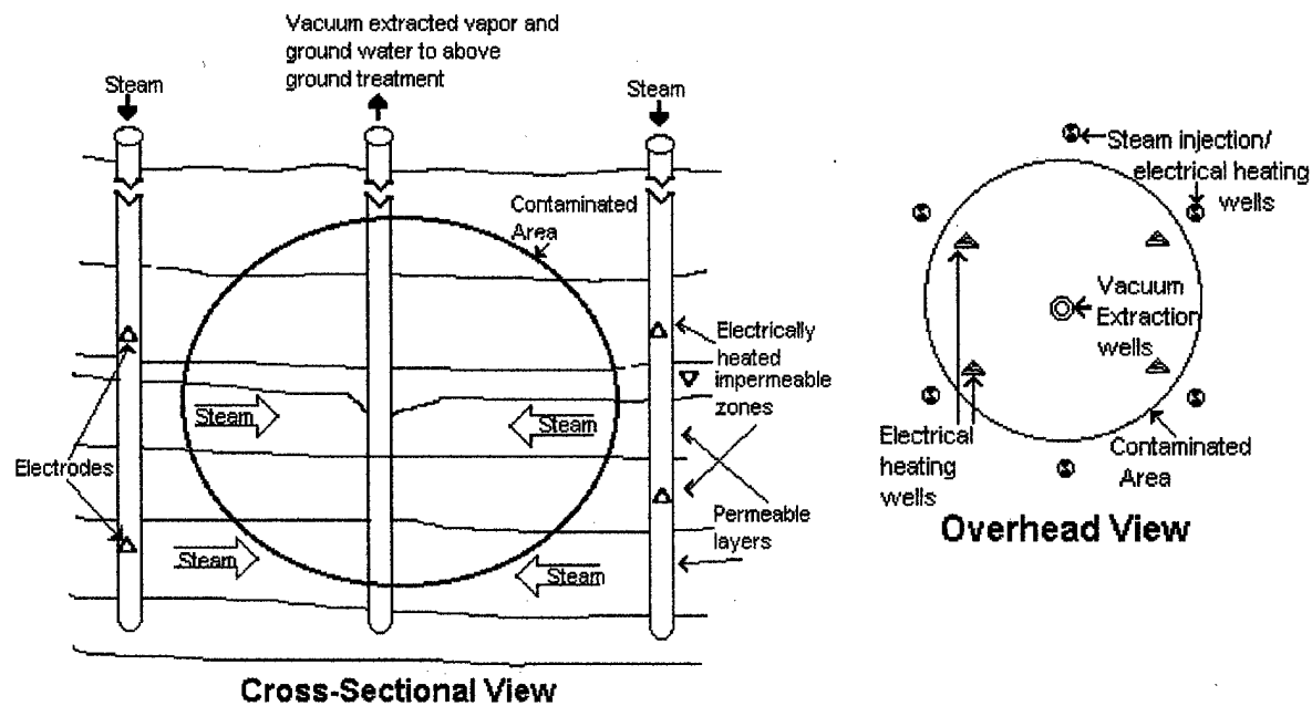
Figure 2-3 Dynamic Underground Stripping [DOE/EM/0271, 1995: 1]
