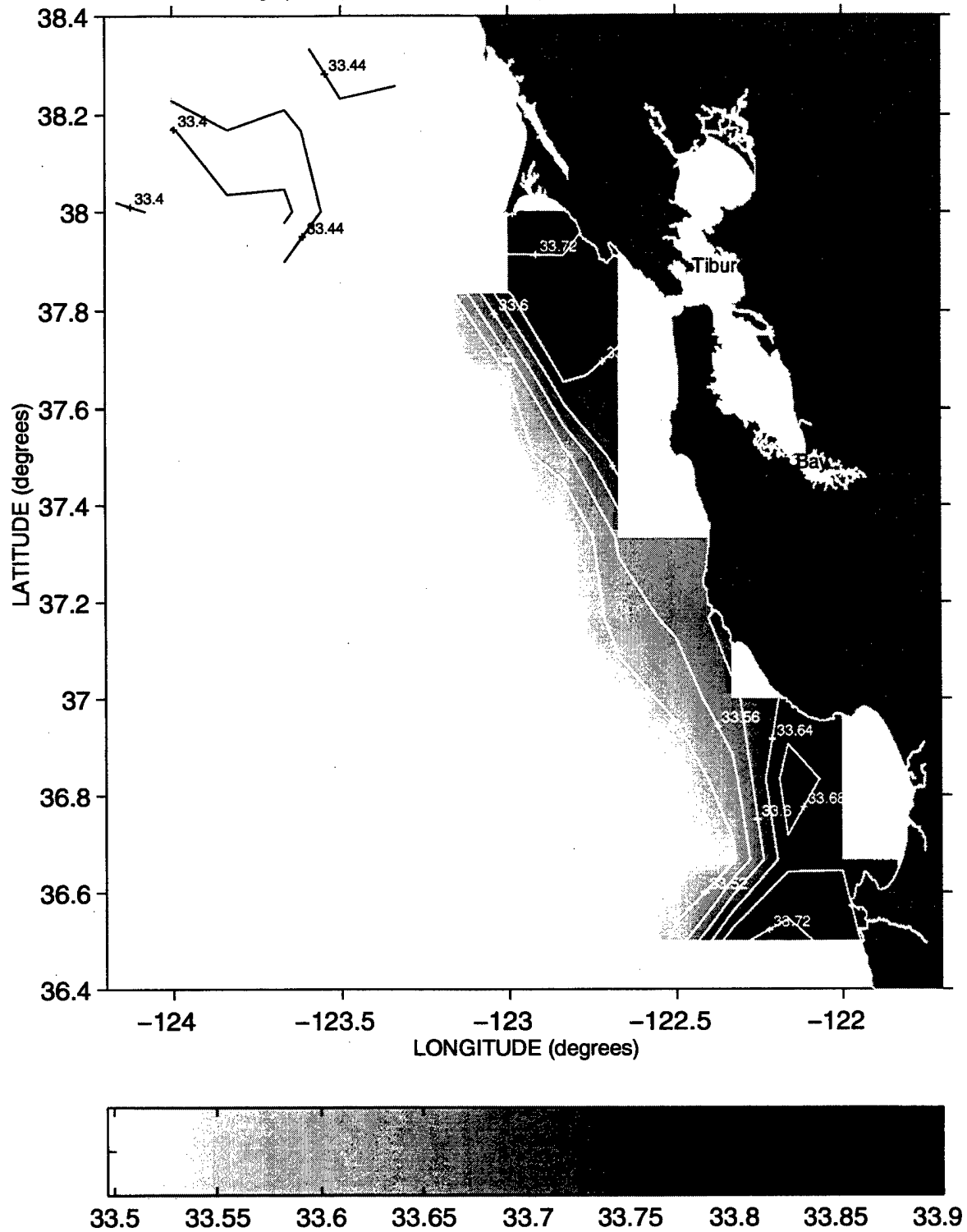
Salinity (PSS) at the 25.8 Isopycnal during Sweep 1, 1994
