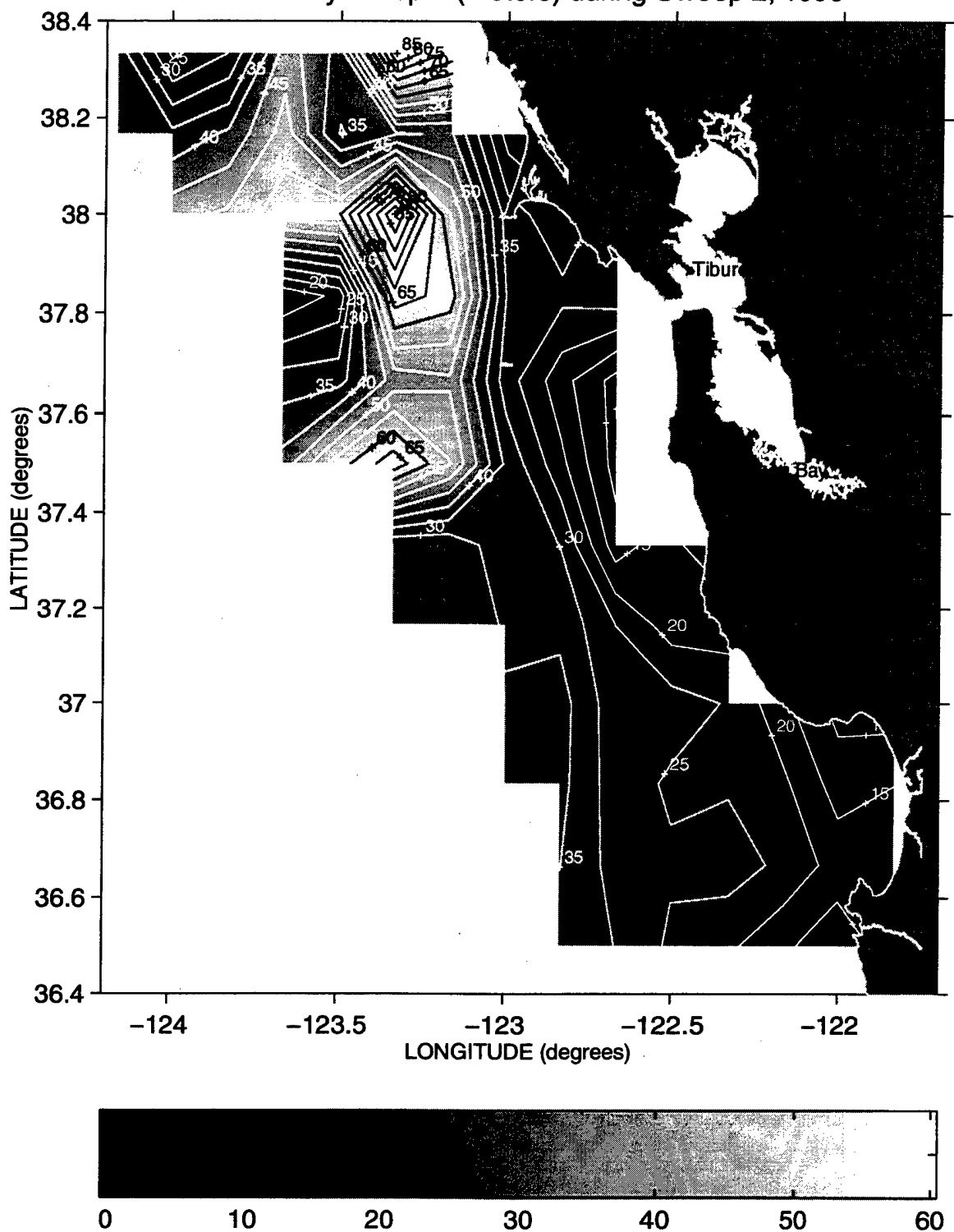
Mixed Layer Depth (meters) during Sweep 2, 1996
