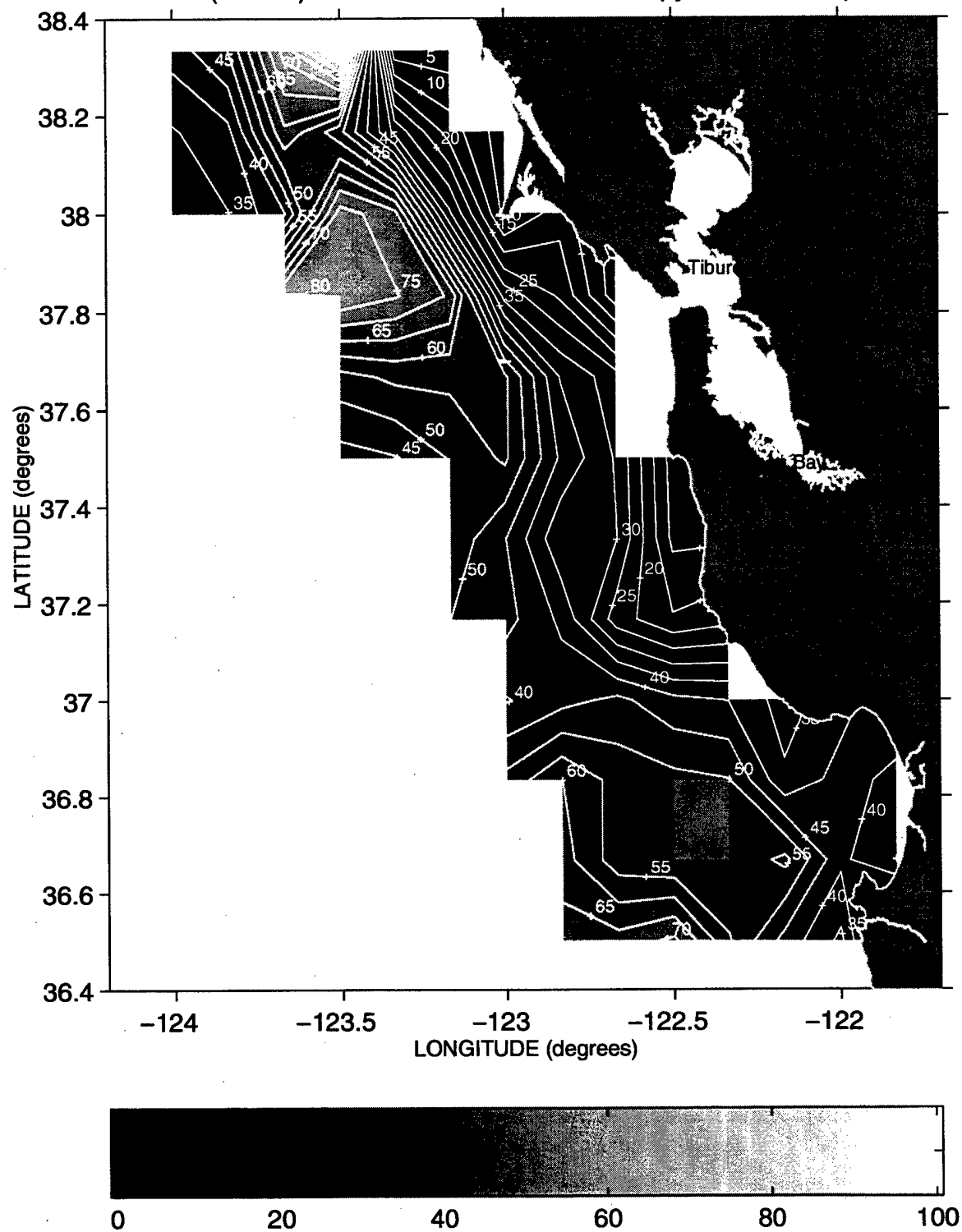
Thickness(meters) between the 25.8 and 26.2 isopycnals ~ Sweep 3, 1994
