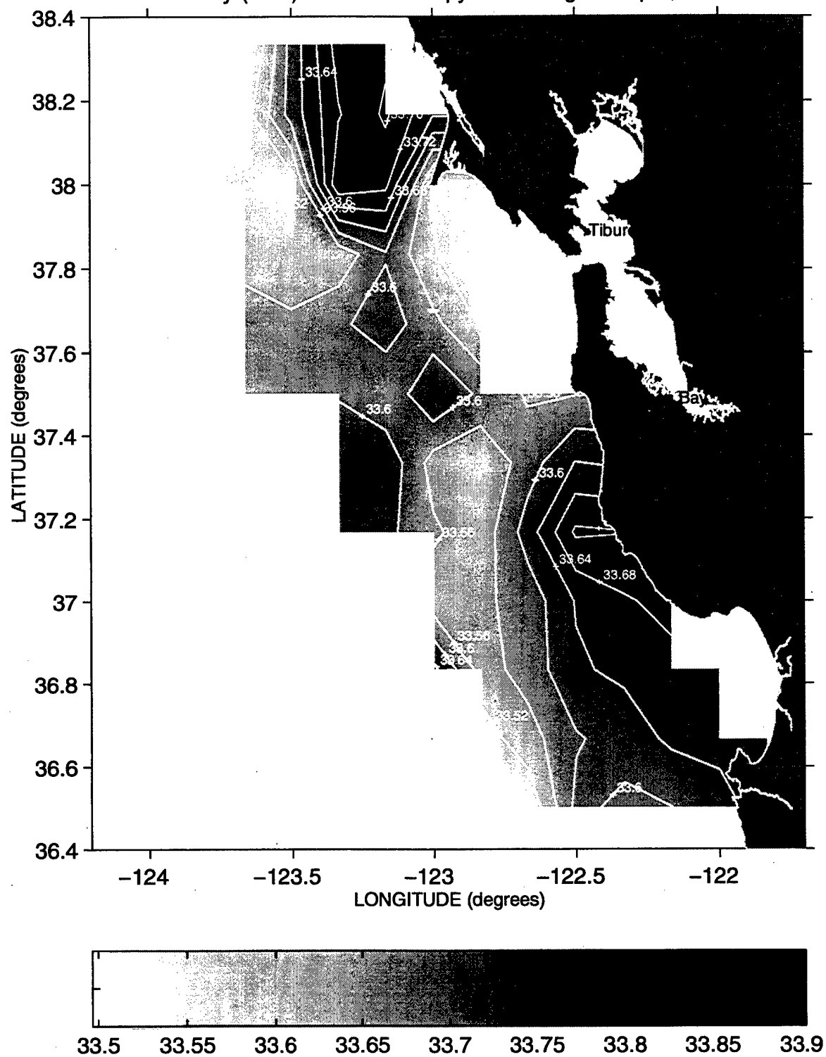
Salinity (PSS) at the 25.8 Isopycnal during Sweep 1, 1996
