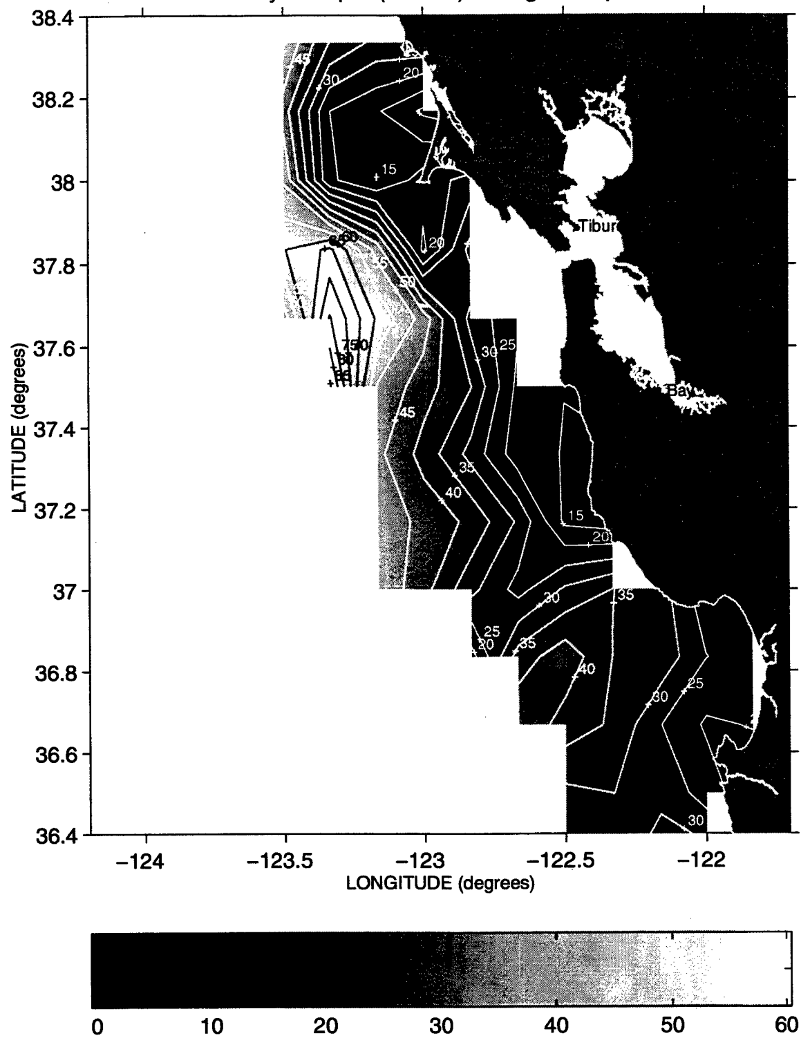
Mixed Layer Depth (meters) during Sweep 1, 1990
