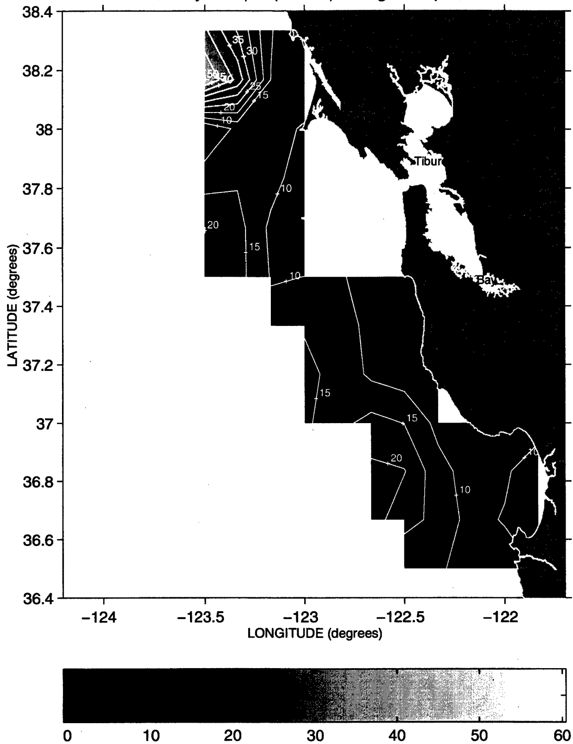
Mixed Layer Depth (meters) during Sweep 2, 1987
