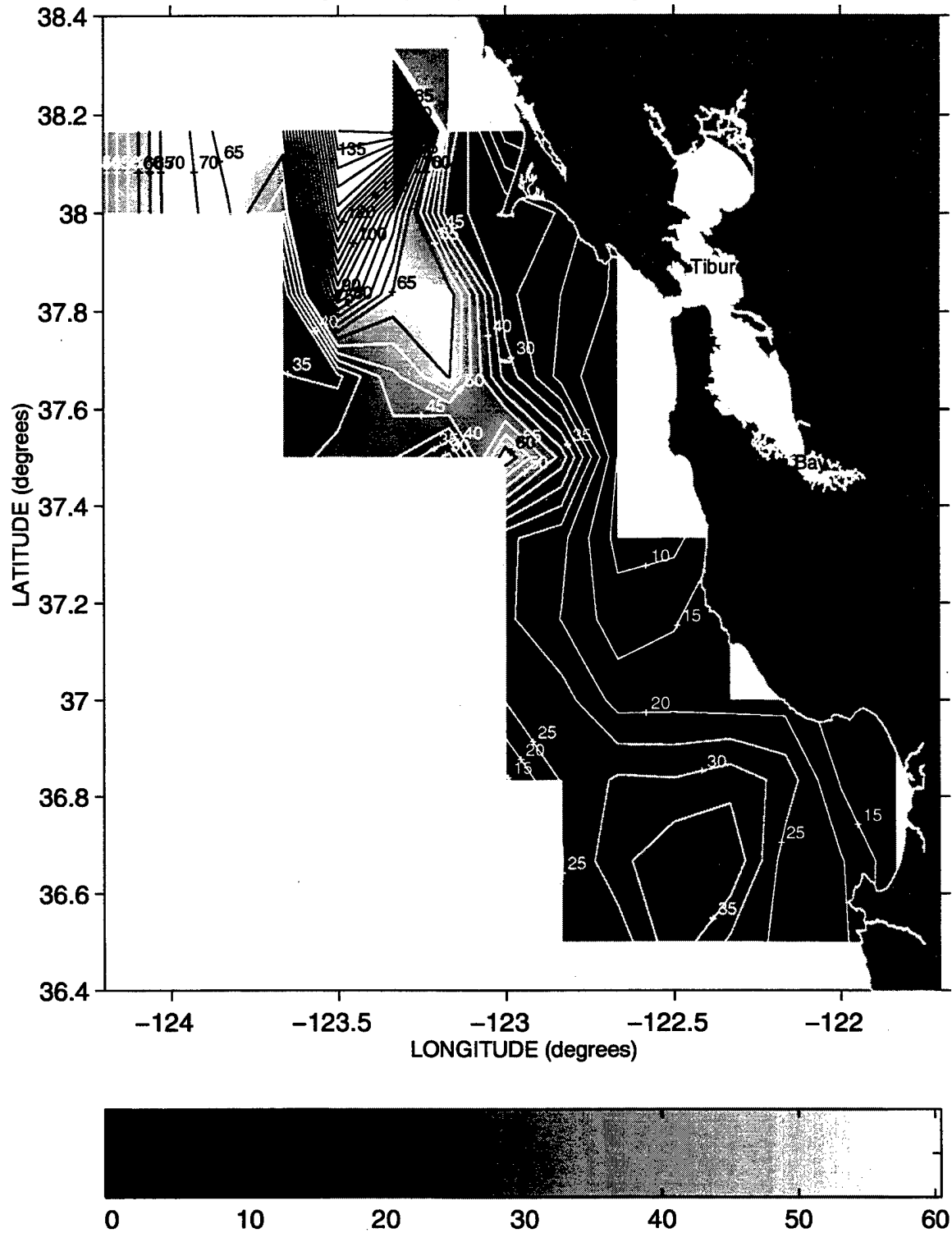
Mixed Layer Depth (meters) during Sweep 3, 1996
