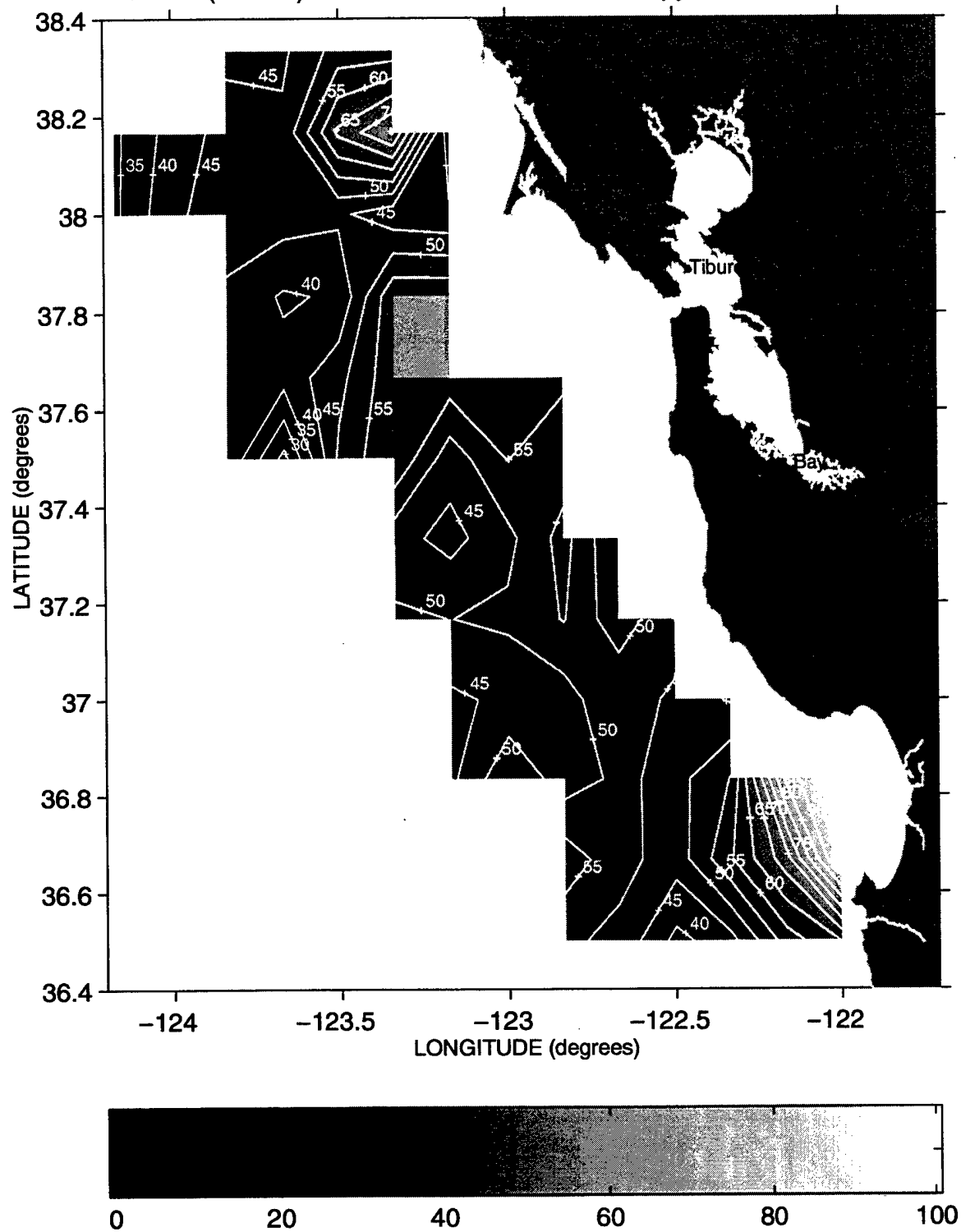
Thickness(meters) between the 25.8 and 26.2 isopycnals ~ Sweep 1, 1992
