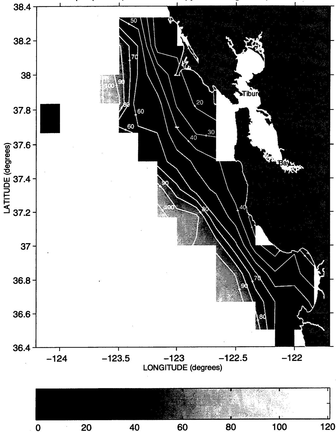
Depth (meters) of the 26.2 Isopycnal during Sweep 3, 1989
