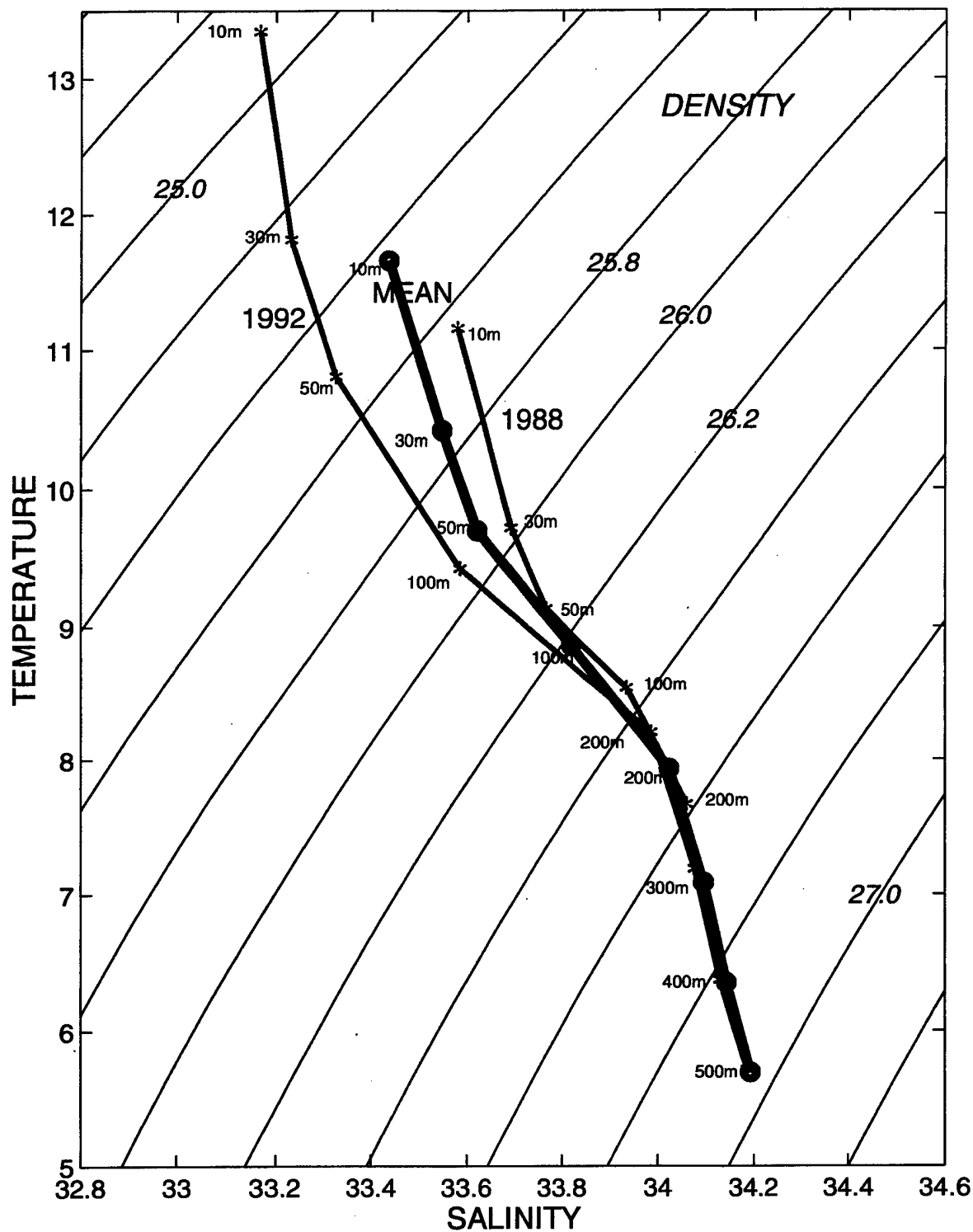
Figure 7. TS Diagrams for the 10 year mean (1987-1996) along with the two contrasting years of 1988 and 1992. Bold circles and asterisks along the TS curves denote the values at discrete depths from 10 to 500 meters.
