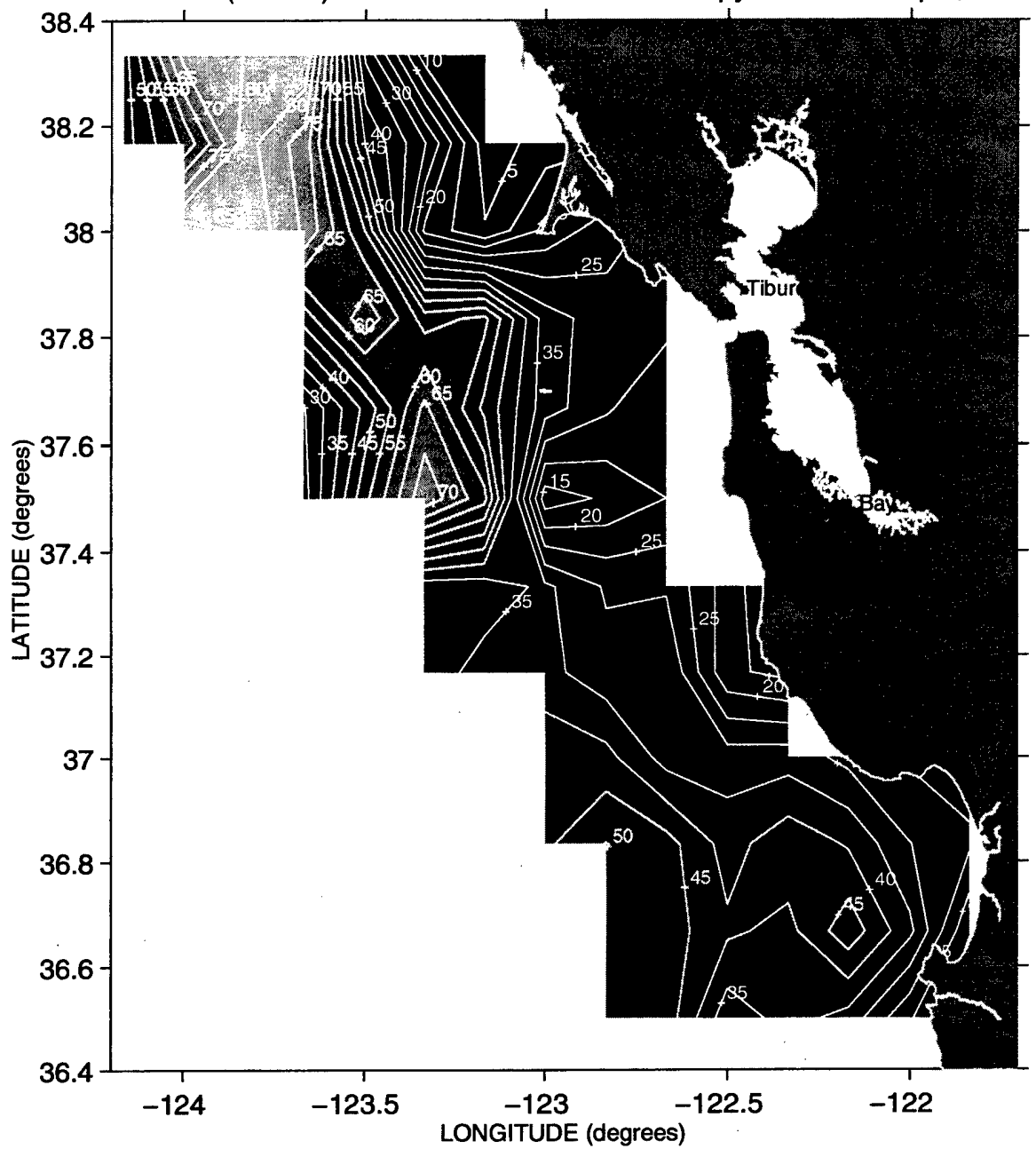
Thickness(meters) between the 25.8 and 26.2 isopycnals ~ Sweep 2, 1996
