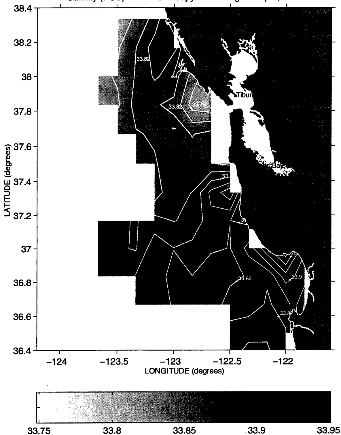
Salinity (PSS) at the 26.2 Isopycnal during Sweep 1, 1989
