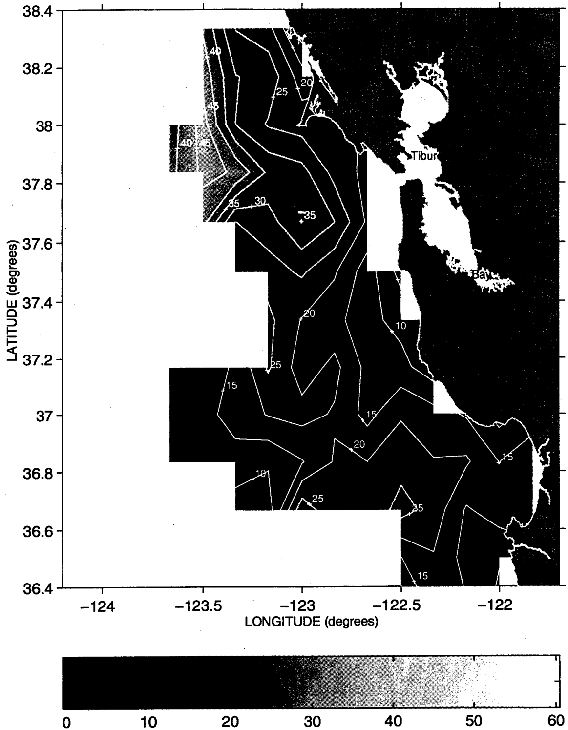
Mixed Layer Depth (meters) during Sweep 1, 1989
