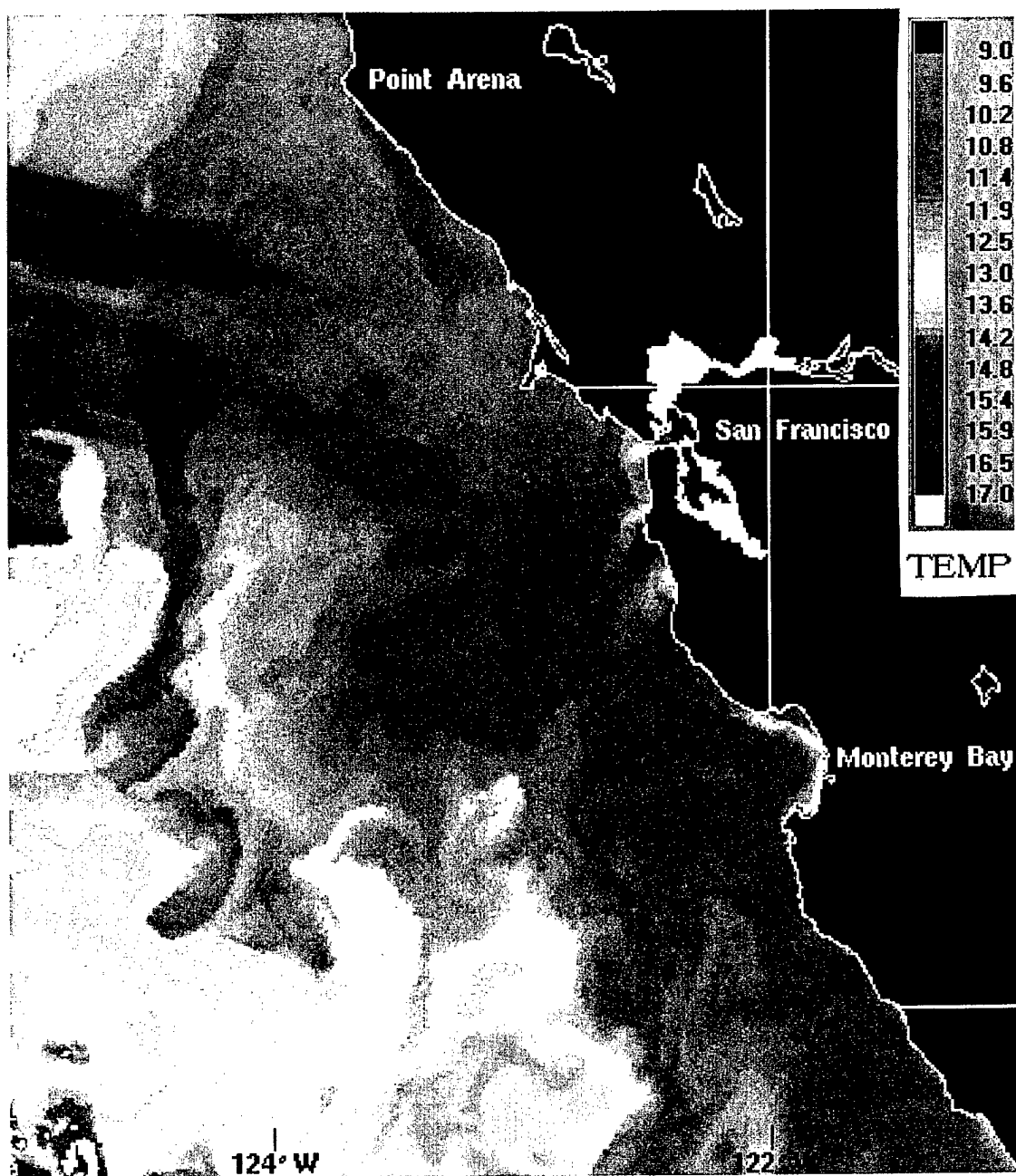
Figure 1. AVHRR Satellite Image of Sea Surface Temperature off Central California, June 10, 1996, Image Resolution is 1.1 km, Temperature Scale is in Degrees Celsius
