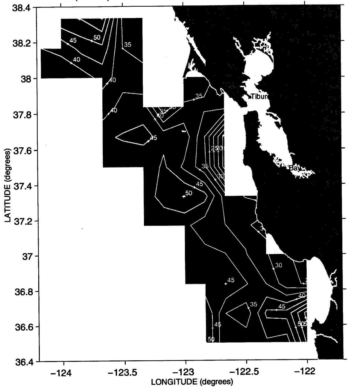
Thickness(meters) between the 25.8 and 26.2 isopycnals ~ Sweep 1, 1994
