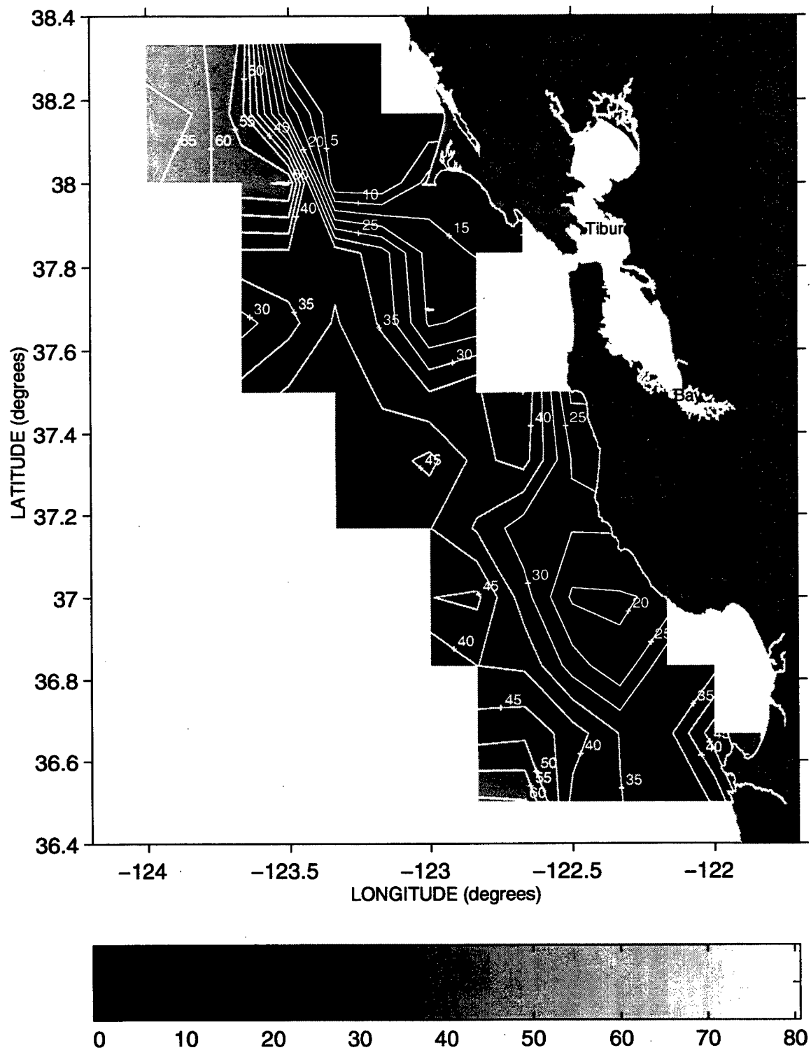
Figure 29. Depth of the 25.8 kg/m 3 isopycnal during sweep 1, 1996. Contour interval is 5 meters. 1996 was characterized as having a strong upwelling season.
