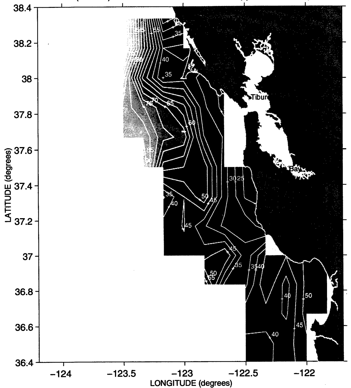
Thickness(meters) between the 25.8 and 26.2 isopycnals ~ Sweep 1, 1990
