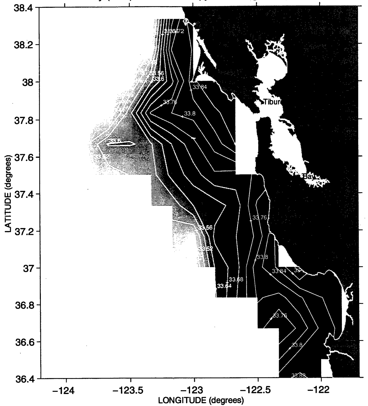
Salinity (PSS) at the 25.8 Isopycnal during Sweep 1, 1988
