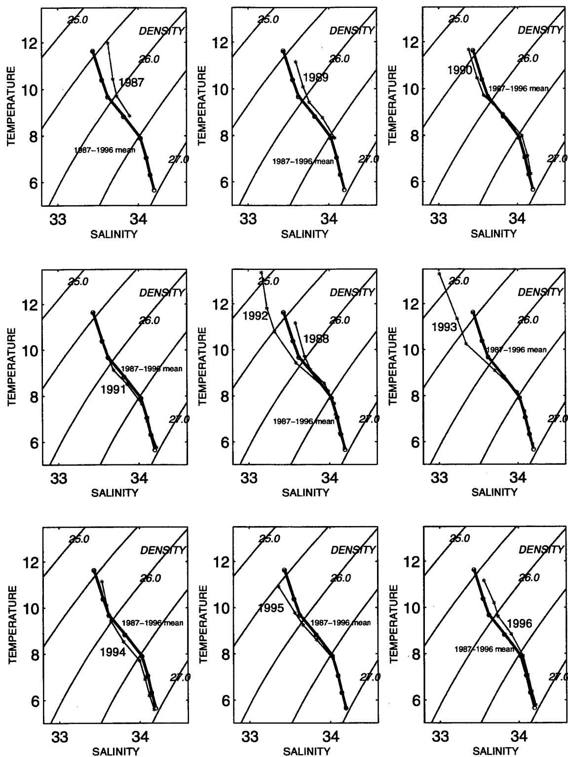
Figure 27. Temperature-Salinity diagrams for each of the annual May-June surveys, 1987-1996. The ten year mean values are plotted along with each of the yearly values.
