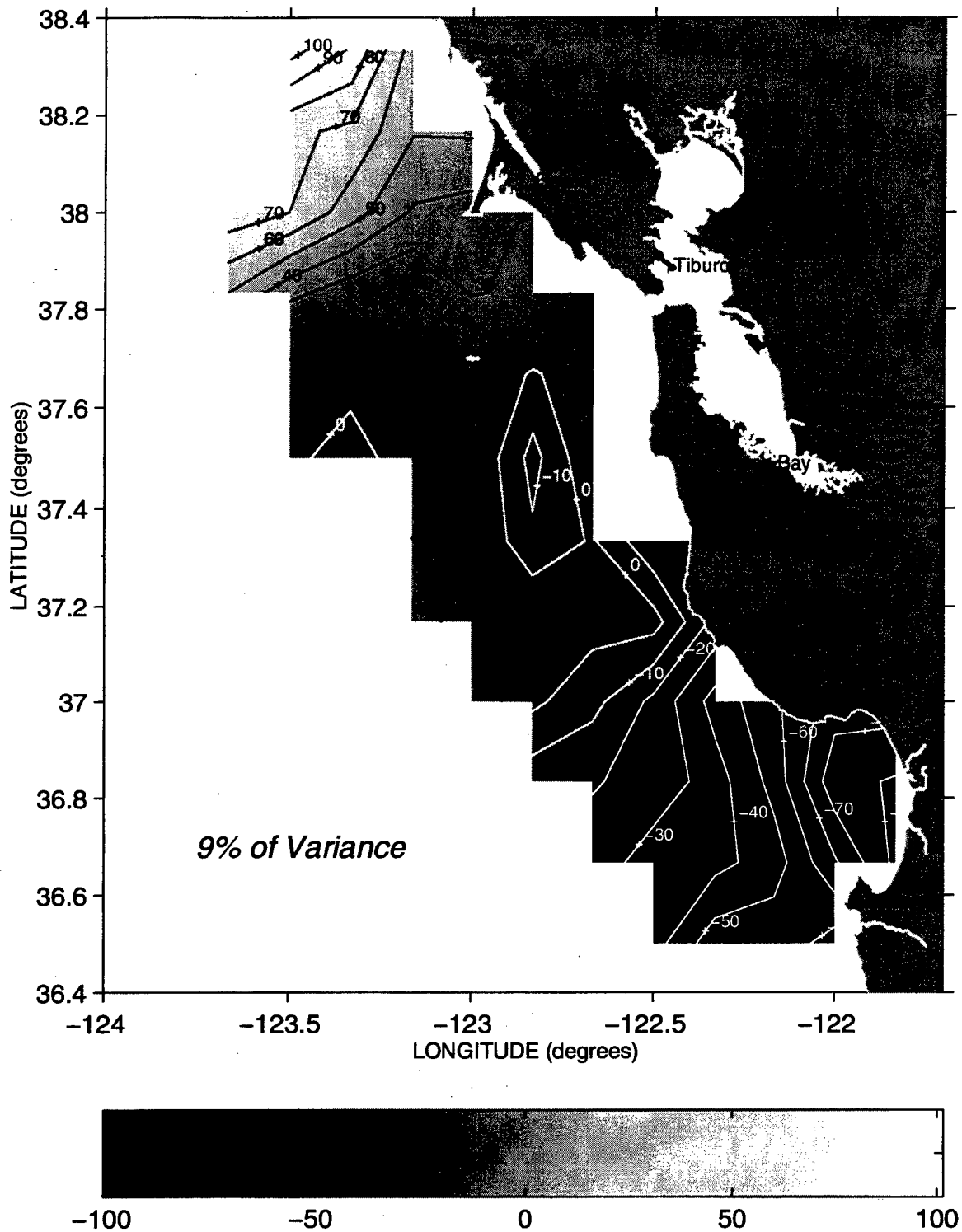
Figure 34. Zscore pattern of the second EOF mode for the 26.2 \text{ kg/m}^3 isopycnal depth. Contour interval is 10.
