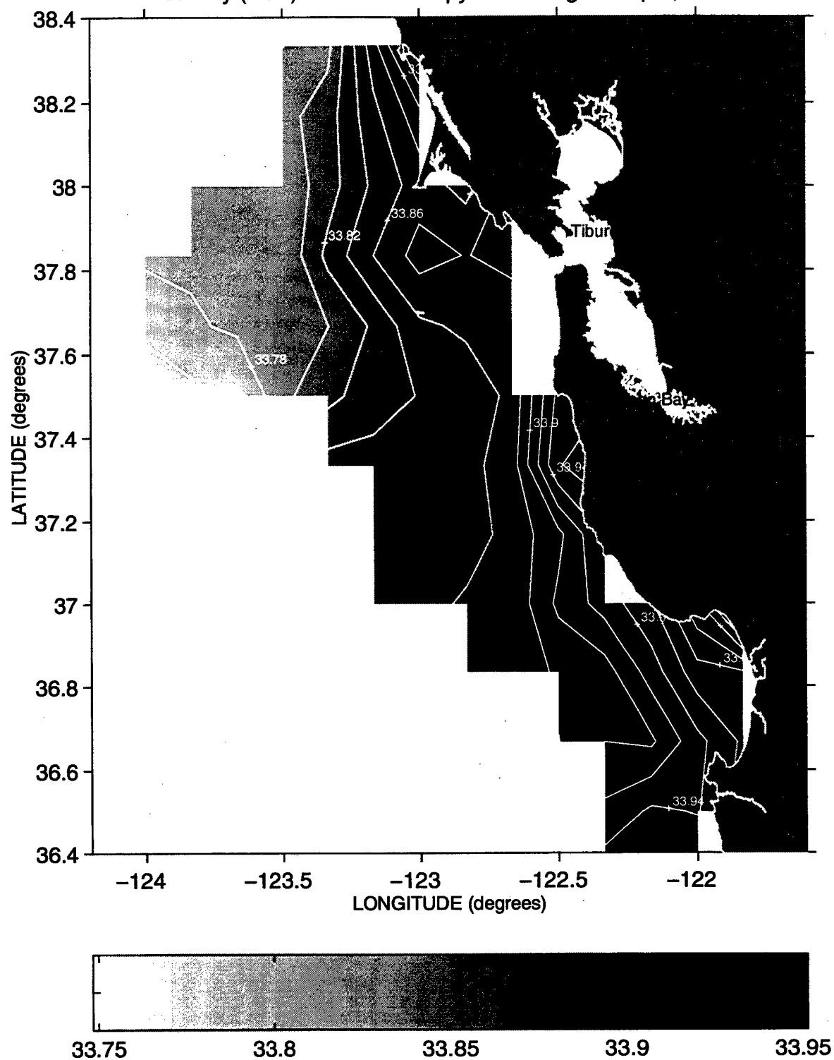
Salinity (PSS) at the 26.2 Isopycnal during Sweep 1, 1988
