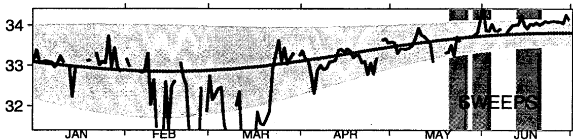
Surface Salinity ~ 1996
