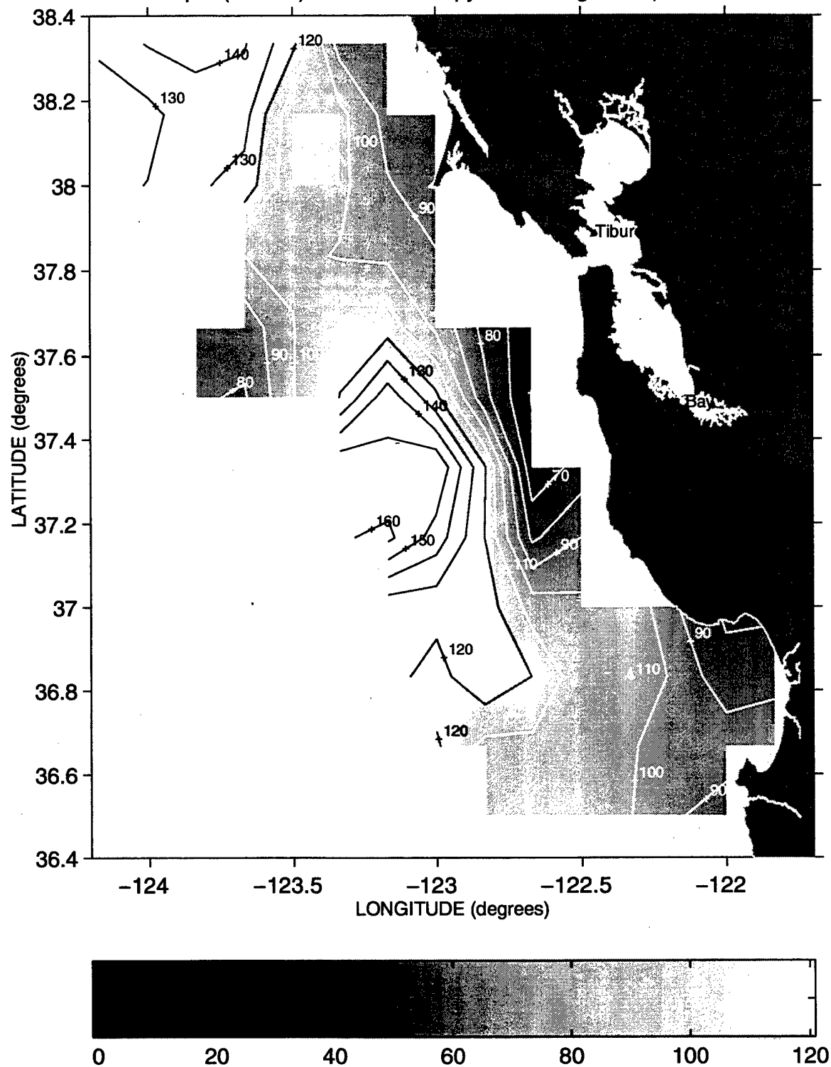
Depth (meters) of the 26.2 Isopycnal during Sweep 2, 1993
