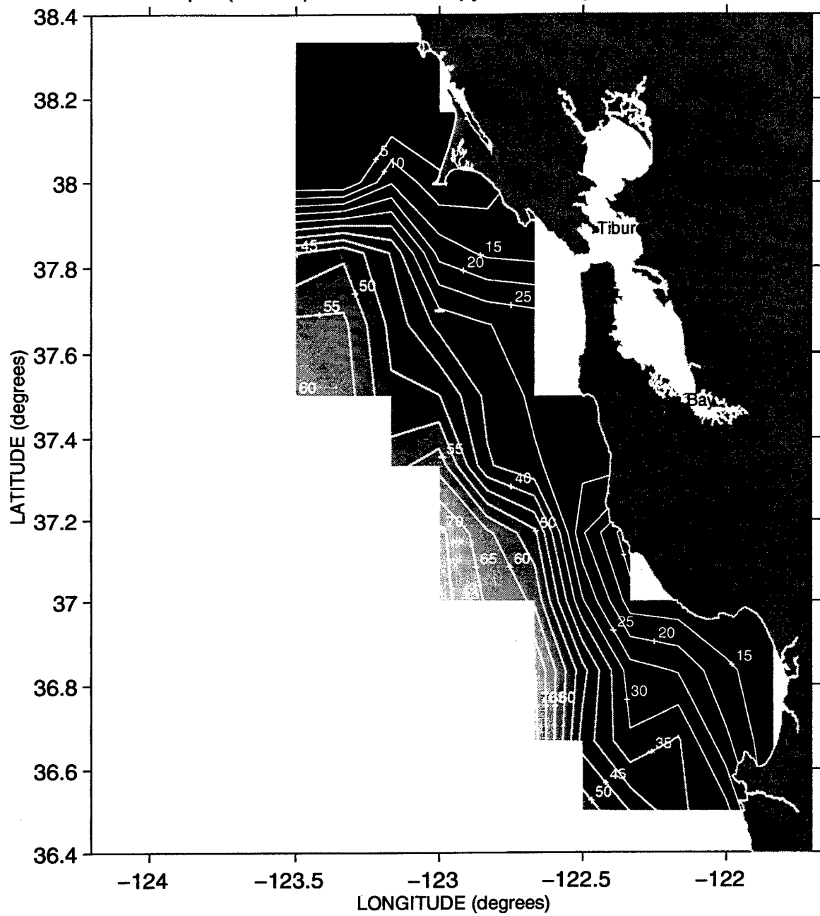
Depth (meters) of the 25.8 Isopycnal during Sweep 3, 1987
