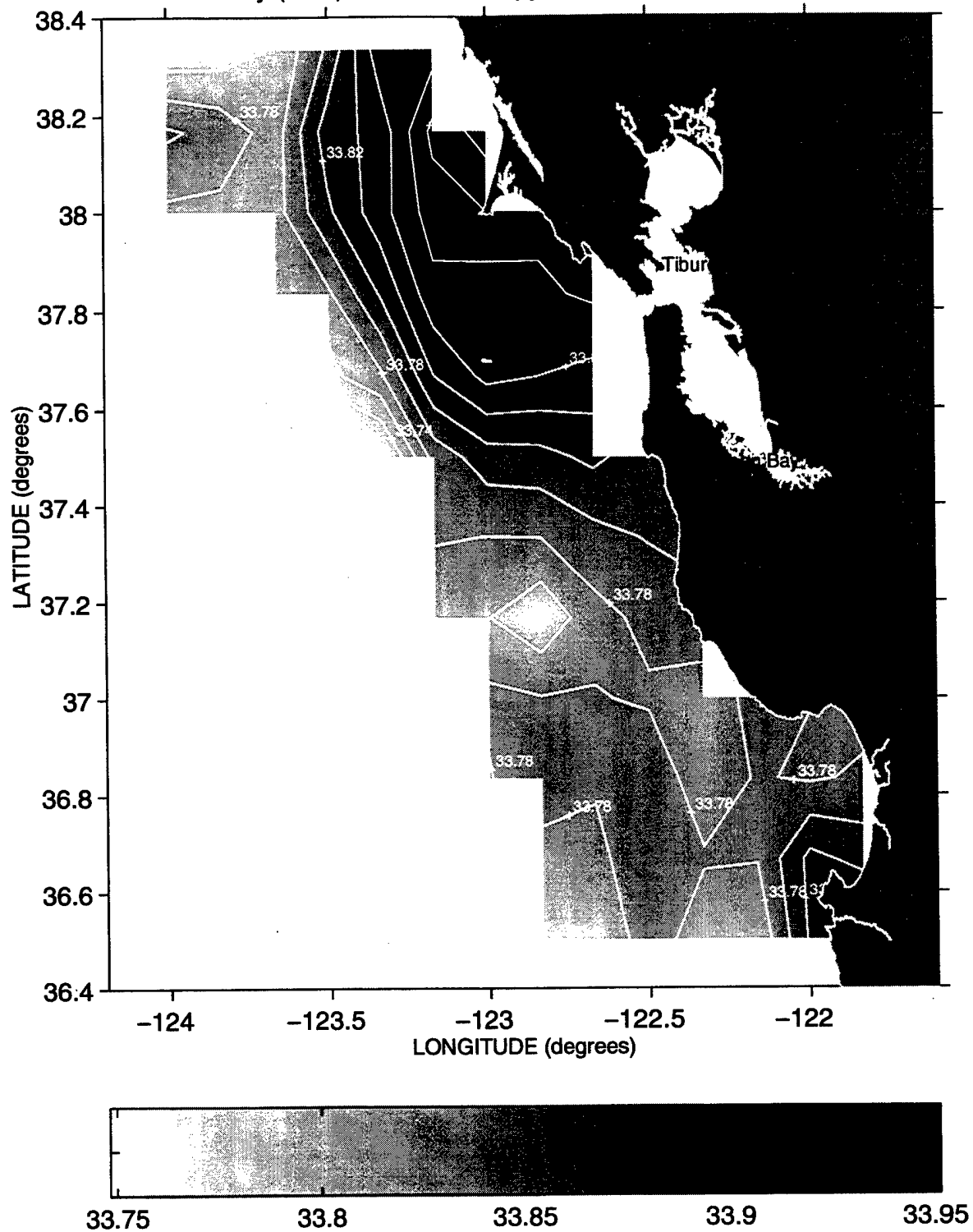
Salinity (PSS) at the 26.2 Isopycnal during Sweep 3, 1994
