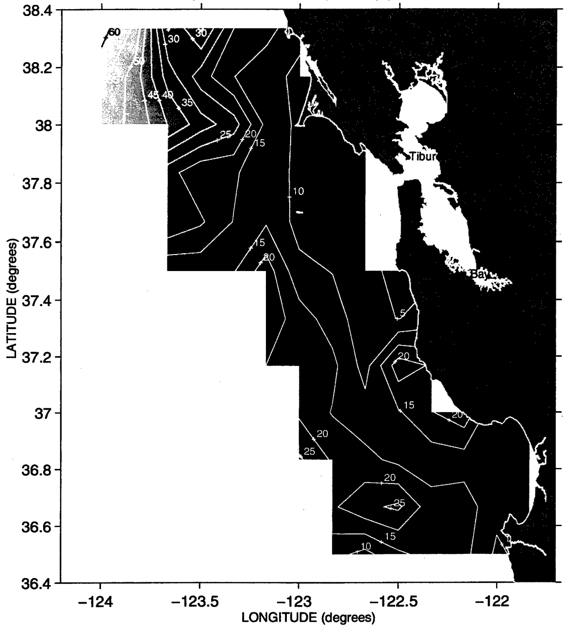
Mixed Layer Depth (meters) during Sweep 1, 1995
