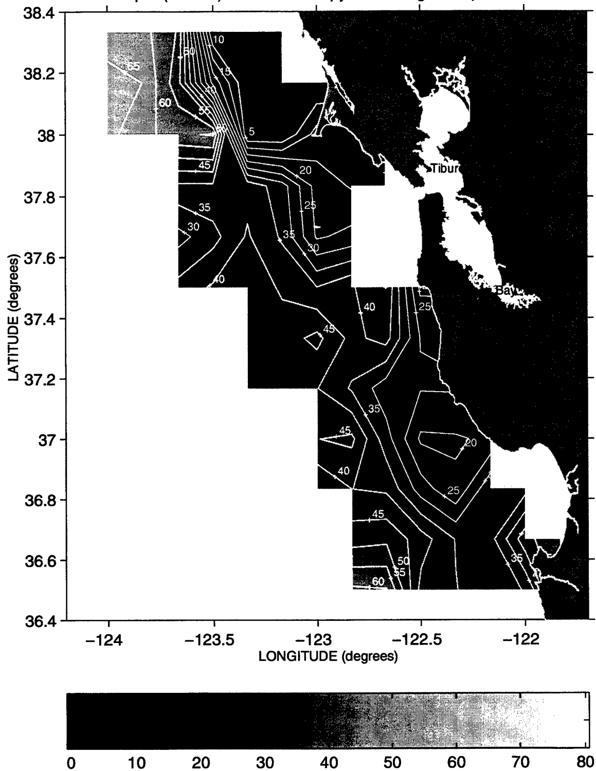
Depth (meters) of the 25.8 Isopycnal during Sweep 1, 1996
