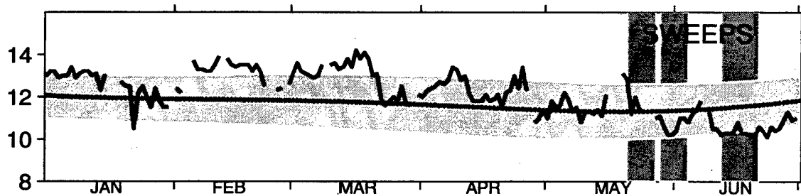
Surface Salinity ~ 1996
