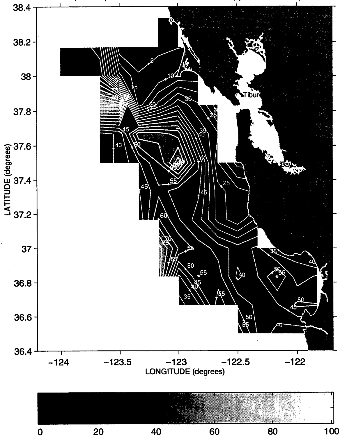
Thickness(meters) between the 25.8 and 26.2 isopycnals ~ Sweep 2, 1991
