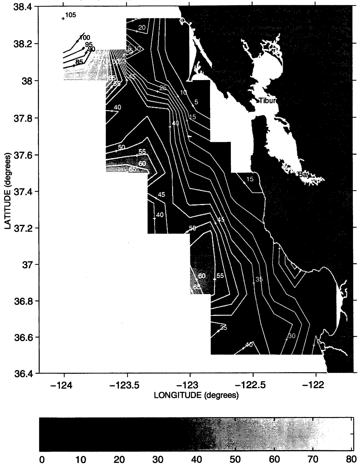
Depth (meters) of the 25.8 Isopycnal during Sweep 2, 1995
