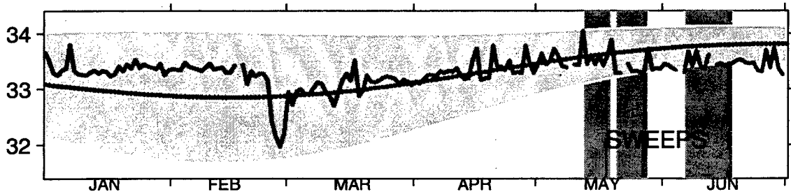
Surface Salinity ~ 1992
