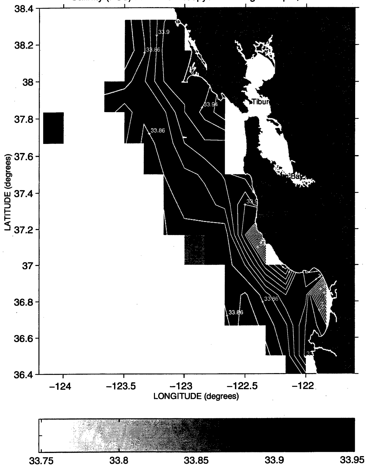
Salinity (PSS) at the 26.2 Isopycnal during Sweep 3, 1989
