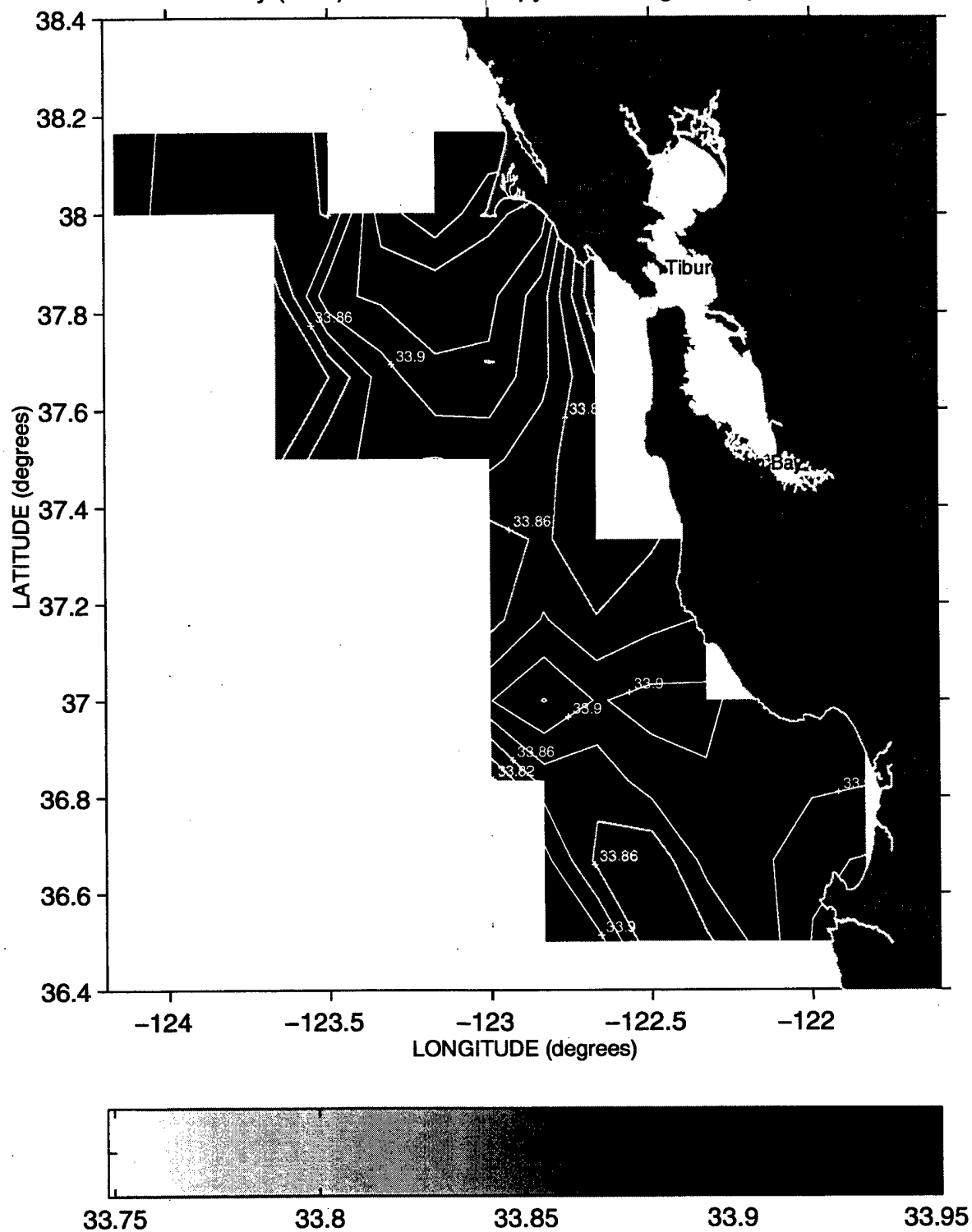
Salinity (PSS) at the 26.2 Isopycnal during Sweep 3, 1996
