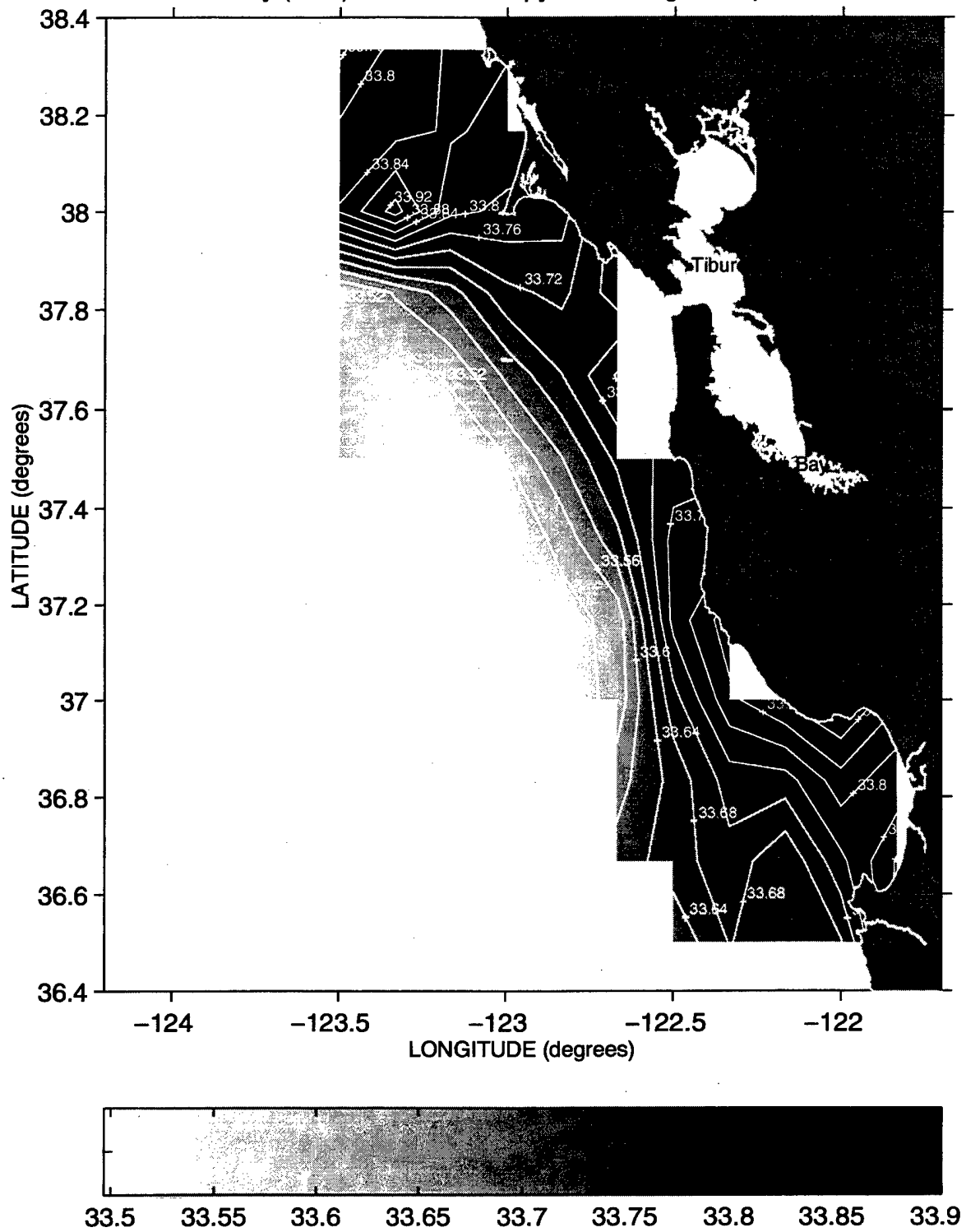
Salinity (PSS) at the 25.8 Isopycnal during Sweep 3, 1987
