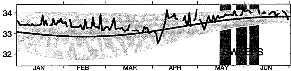
Sea Surface Temperature ~ 1992
