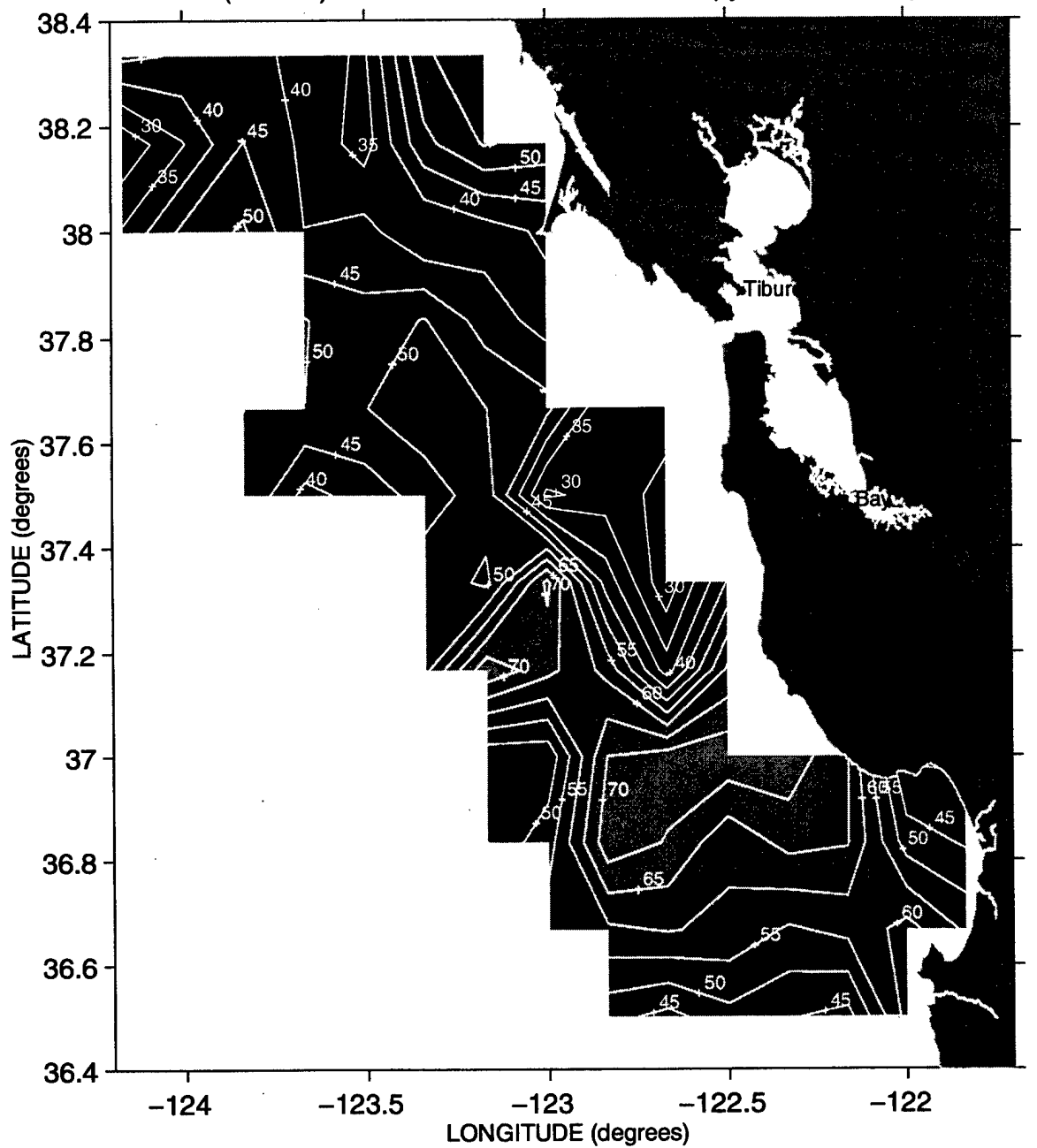
Thickness(meters) between the 25.8 and 26.2 isopycnals ~ Sweep 2, 1993
