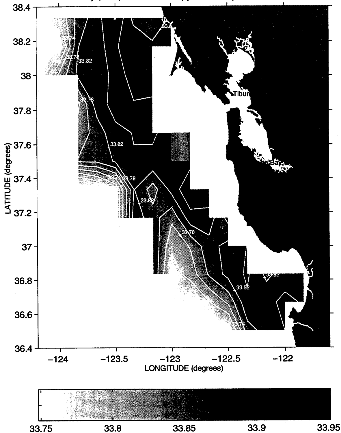
Salinity (PSS) at the 26.2 Isopycnal during Sweep 3, 1992
