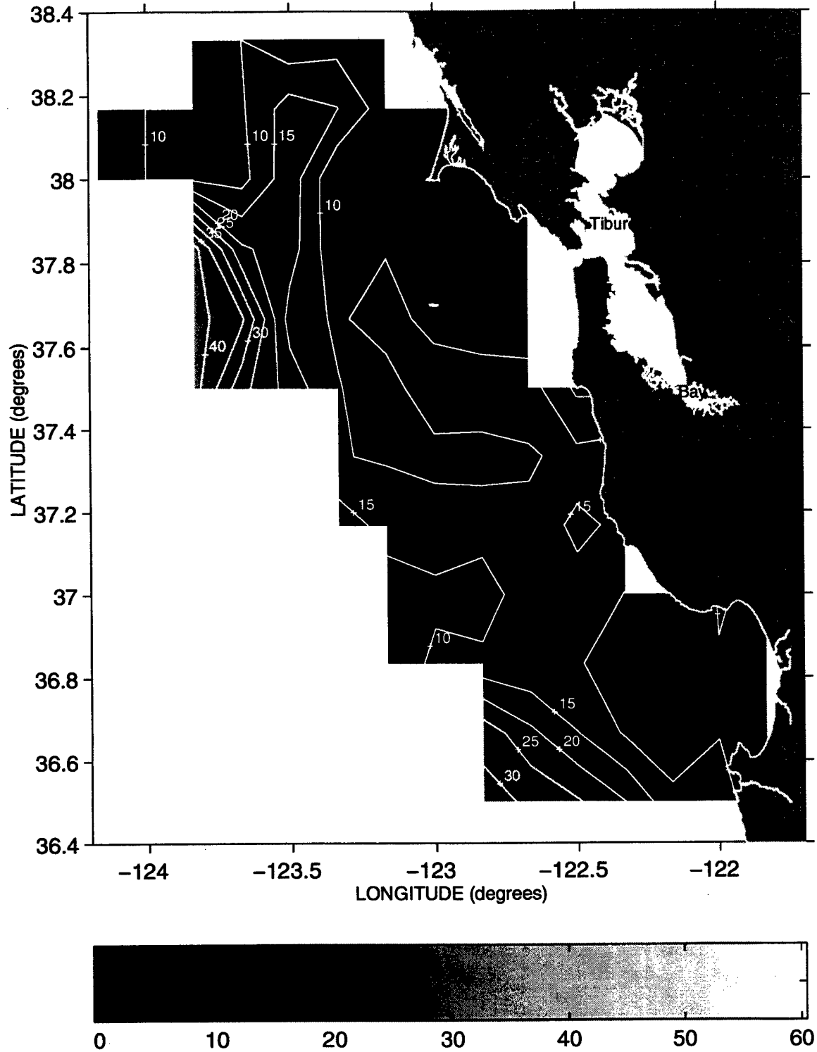
Mixed Layer Depth (meters) during Sweep 1, 1992
