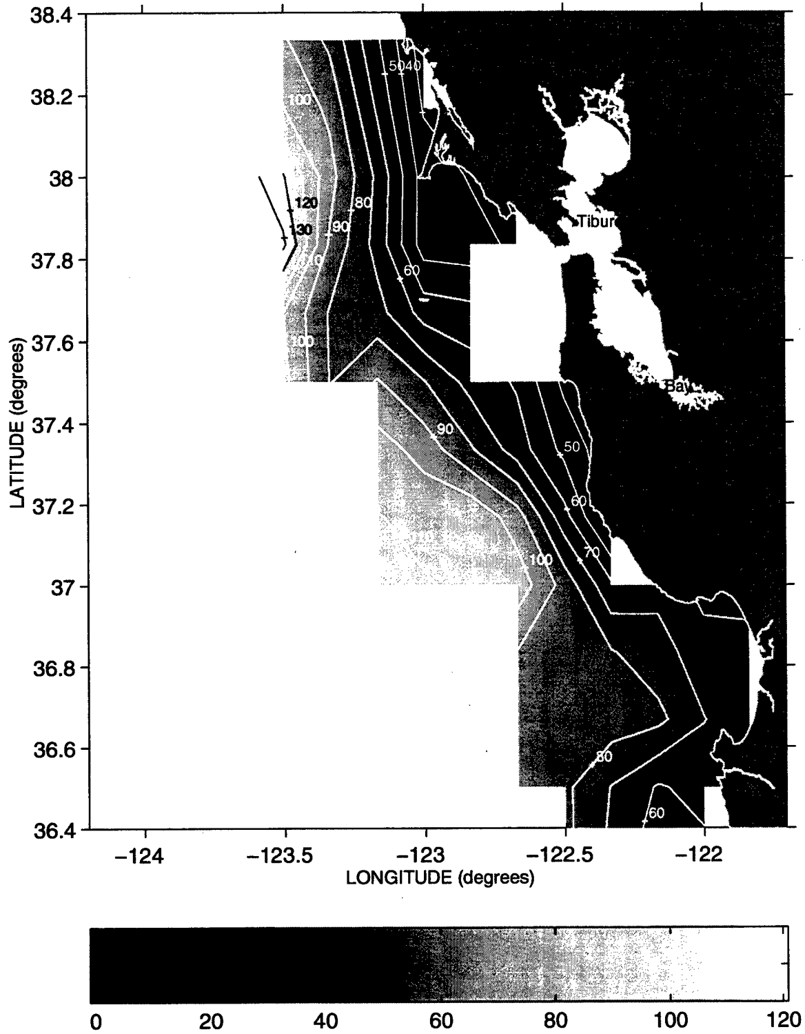
Depth (meters) of the 26.2 Isopycnal during Sweep 3, 1990
