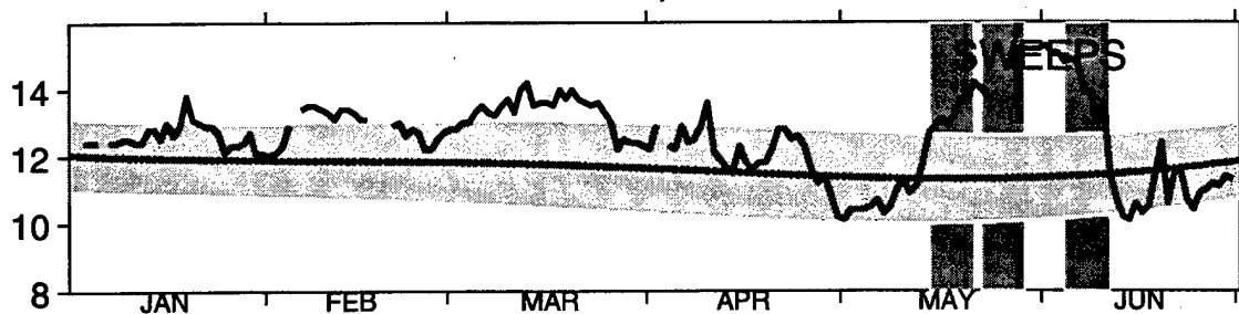
Surface Salinity ~ 1993
