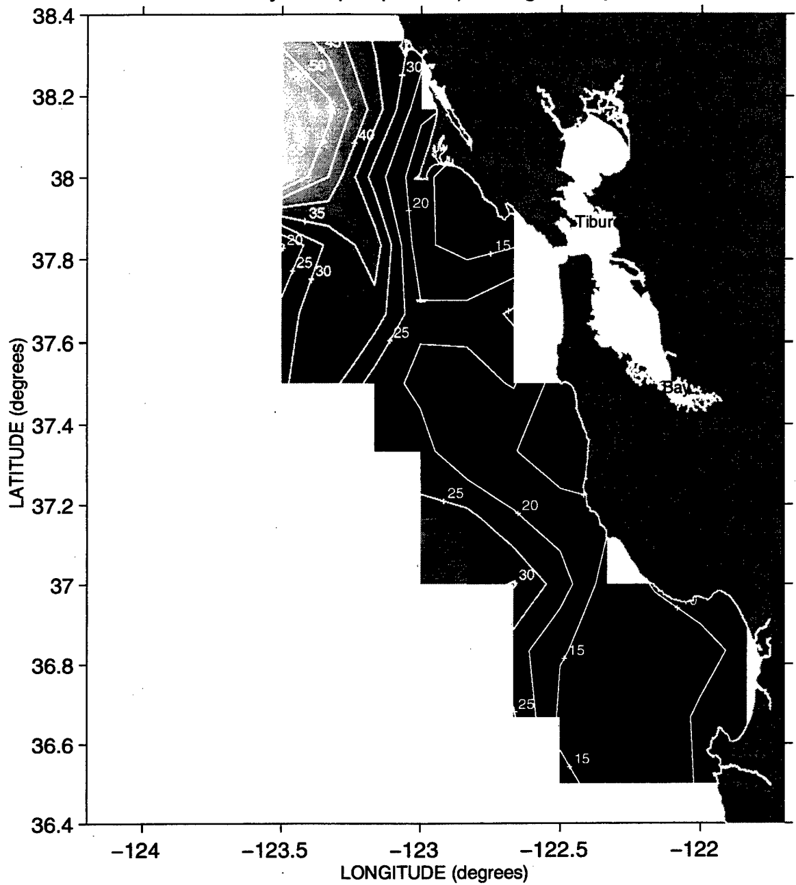
Mixed Layer Depth (meters) during Sweep 3, 1987
