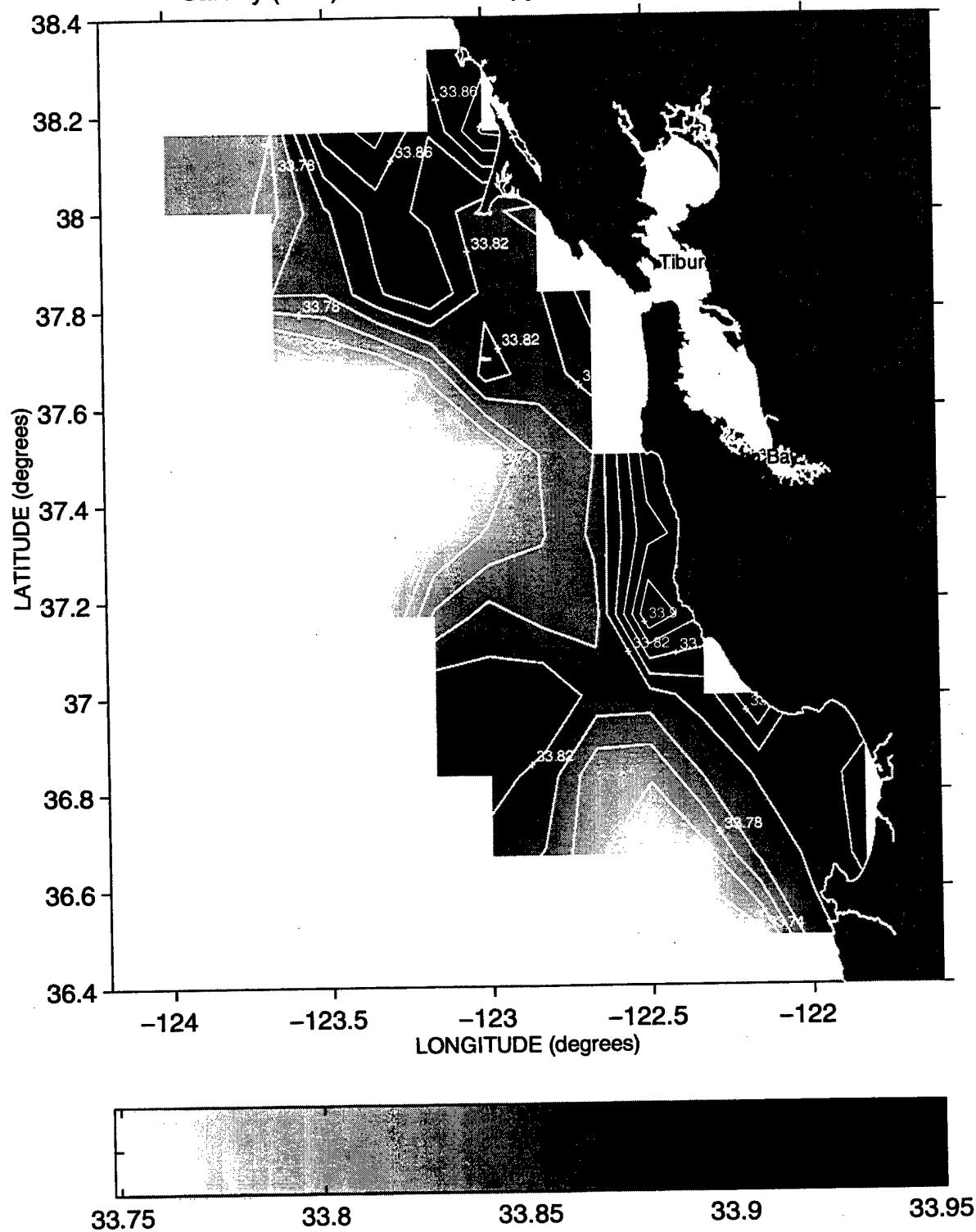
Salinity (PSS) at the 26.2 Isopycnal during Sweep 2, 1991
