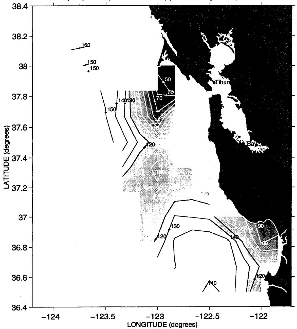
Depth (meters) of the 26.2 Isopycnal during Sweep 3, 1993
