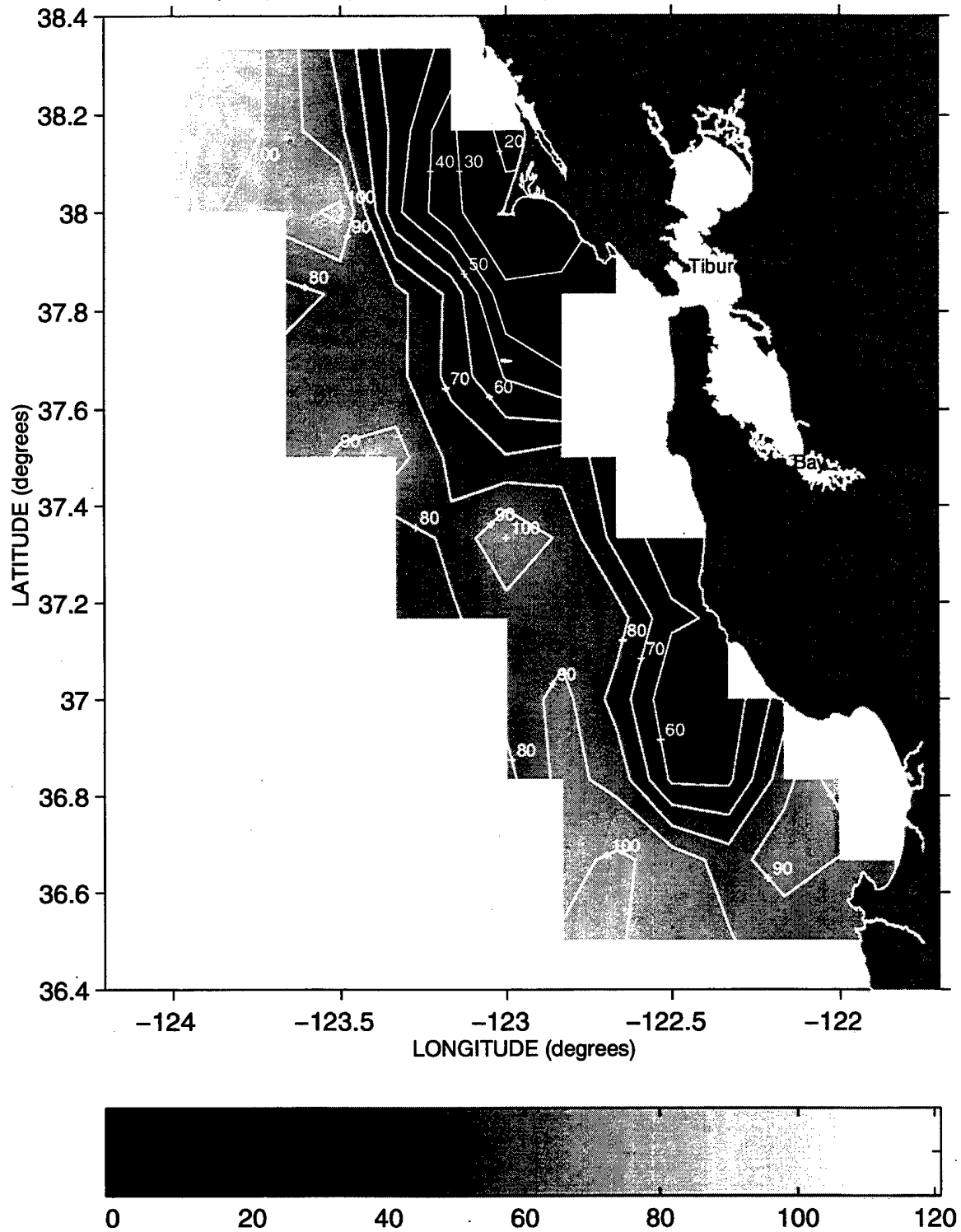
Depth (meters) of the 26.2 Isopycnal during Sweep 1, 1996
