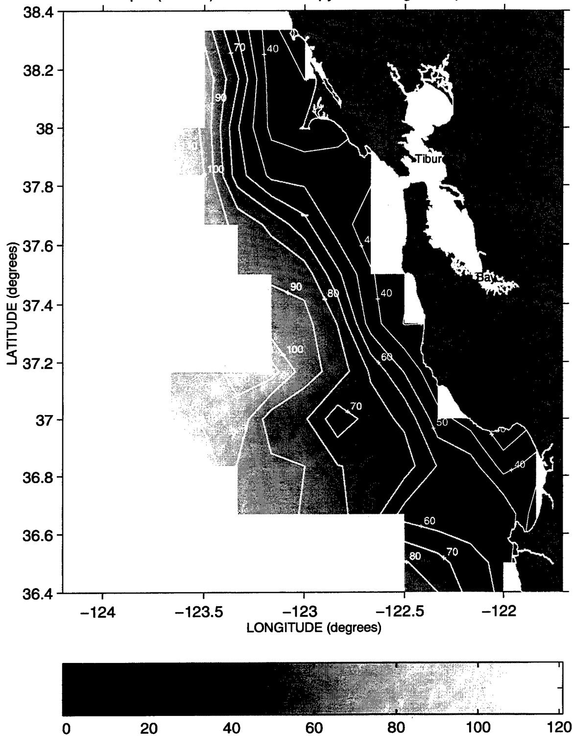
Depth (meters) of the 26.2 Isopycnal during Sweep 1, 1989
