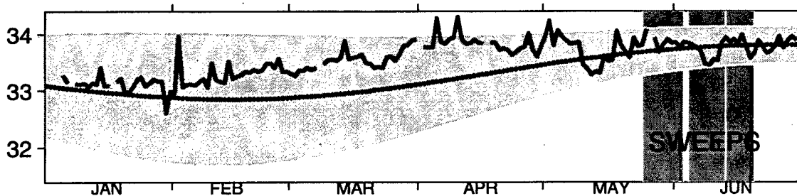
Surface Salinity ~ 1988
