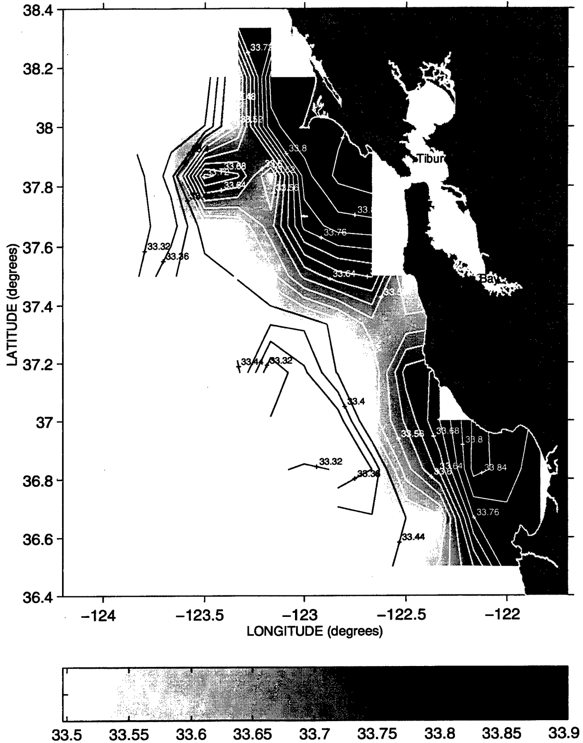
Salinity (PSS) at the 25.8 Isopycnal during Sweep 1, 1991
