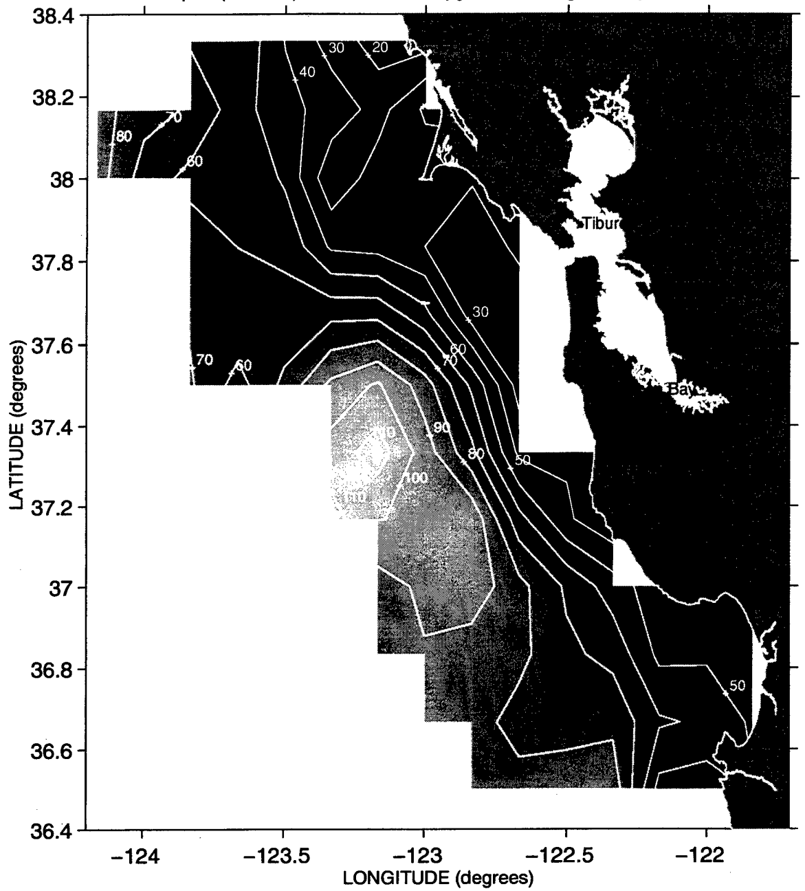
Depth (meters) of the 26.2 Isopycnal during Sweep 3, 1991
