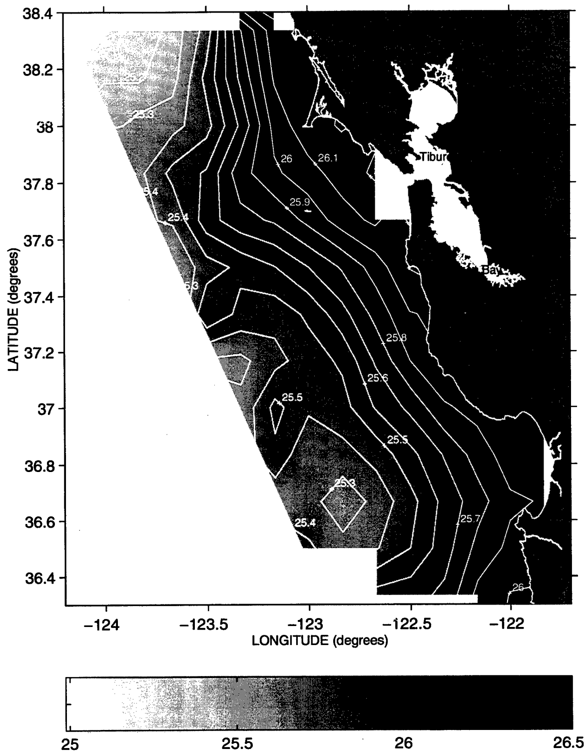
Figure 20. Mean potential density anomaly at 30 meters during May-June, 1987-1996. Contour interval is 0.1 kg/m 3 .
