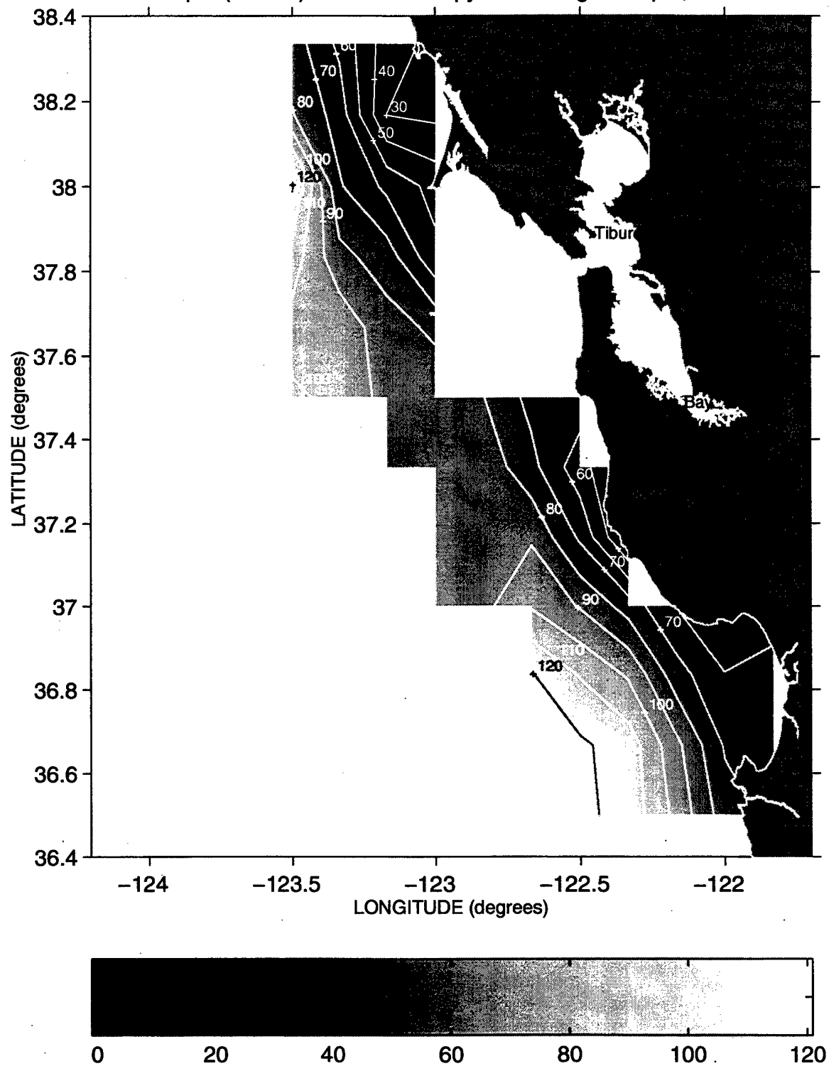
Depth (meters) of the 26.2 Isopycnal during Sweep 2, 1987
