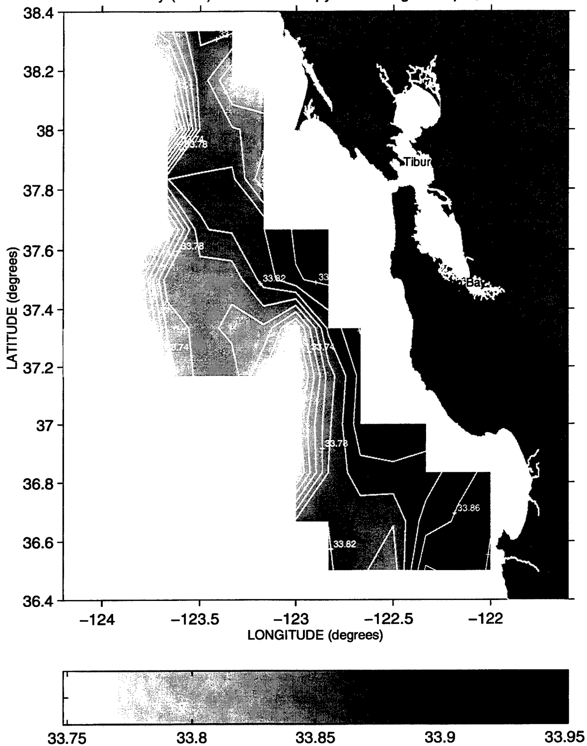
Salinity (PSS) at the 26.2 Isopycnal during Sweep 2, 1992
