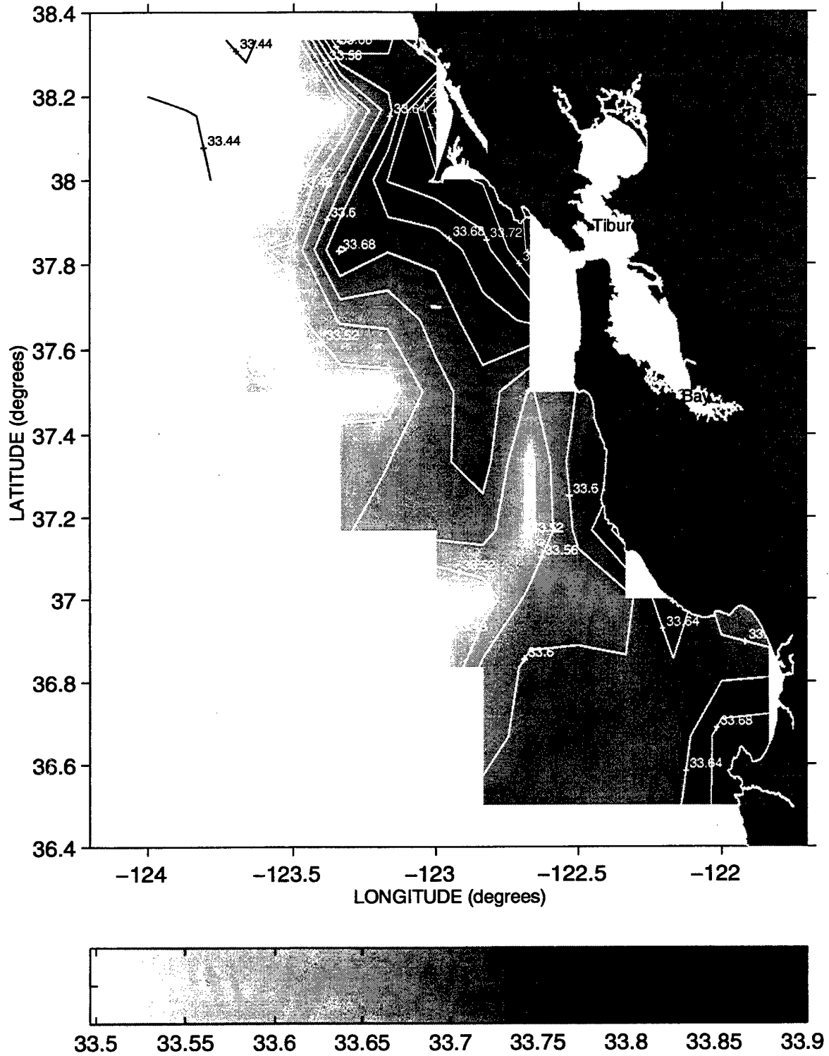
Salinity (PSS) at the 25.8 Isopycnal during Sweep 3, 1995
