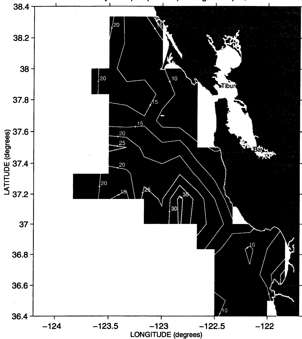
Mixed Layer Depth (meters) during Sweep 2, 1990
