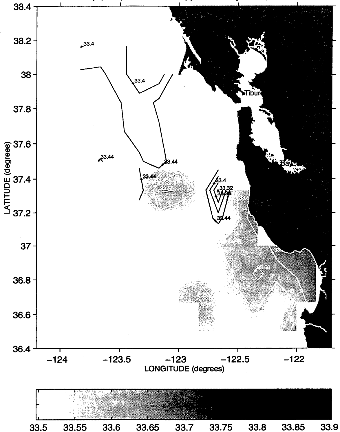
Salinity (PSS) at the 25.8 Isopycnal during Sweep 3, 1993
