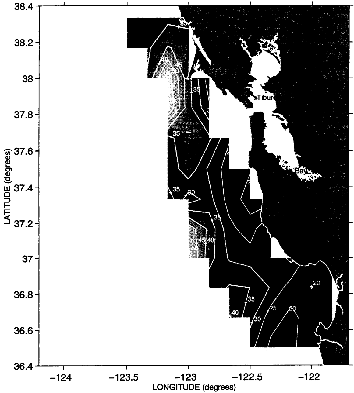
Mixed Layer Depth (meters) during Sweep 1, 1987
