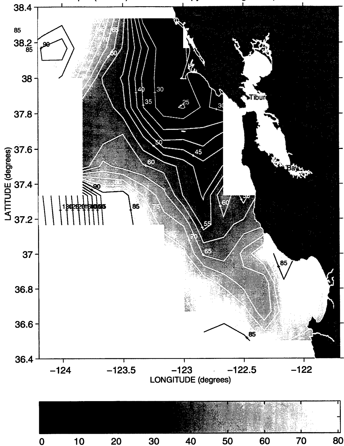
Depth (meters) of the 25.8 Isopycnal during Sweep 3, 1992
