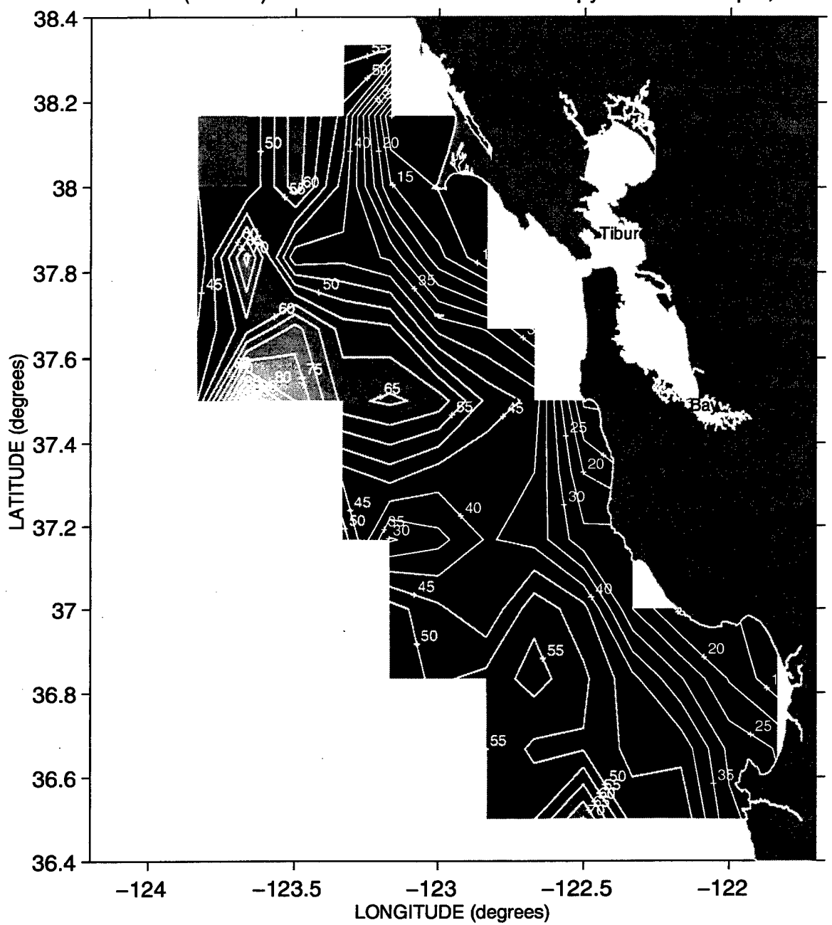
Thickness(meters) between the 25.8 and 26.2 isopycnals ~ Sweep 1, 1991
