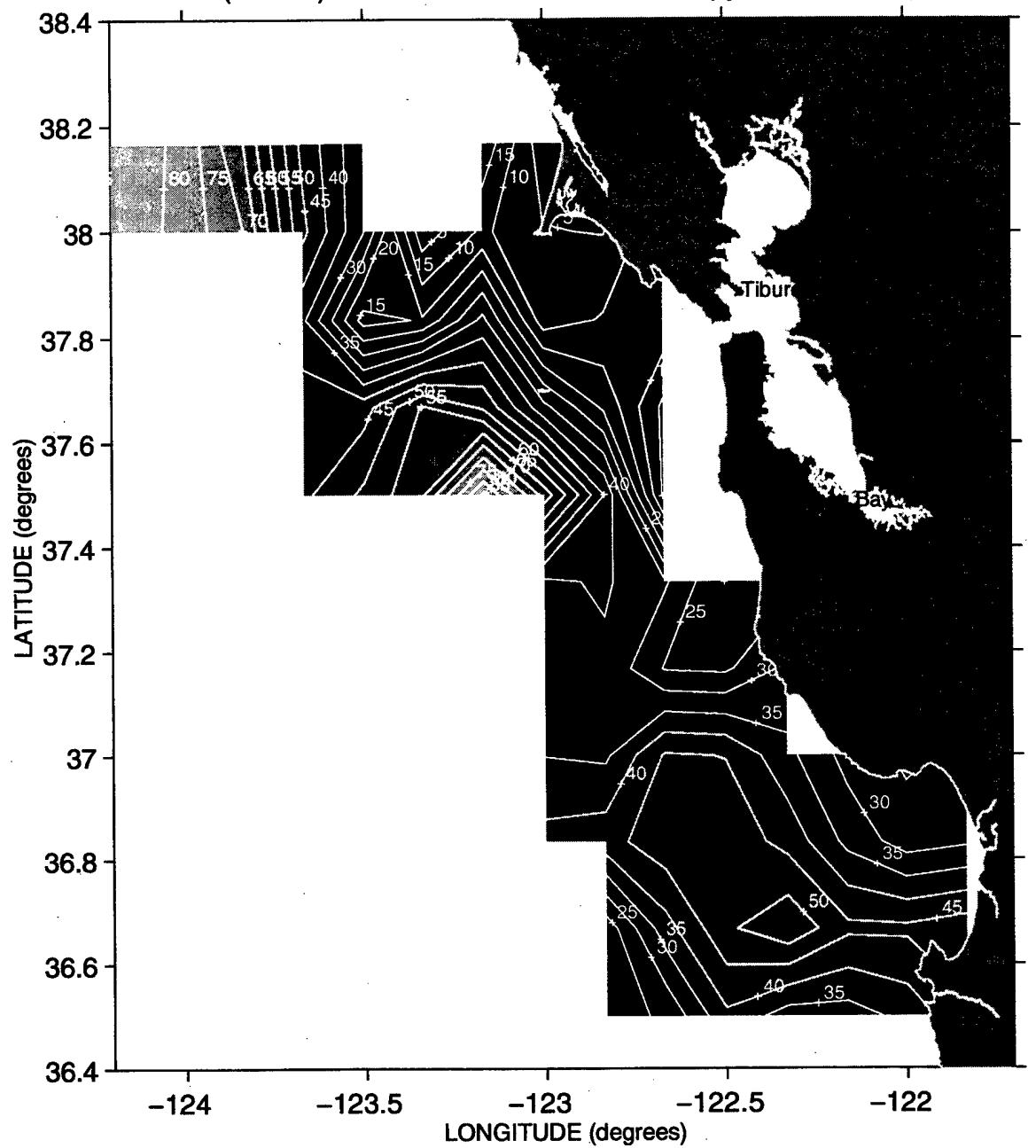
Thickness(meters) between the 25.8 and 26.2 isopycnals ~ Sweep 3, 1996
