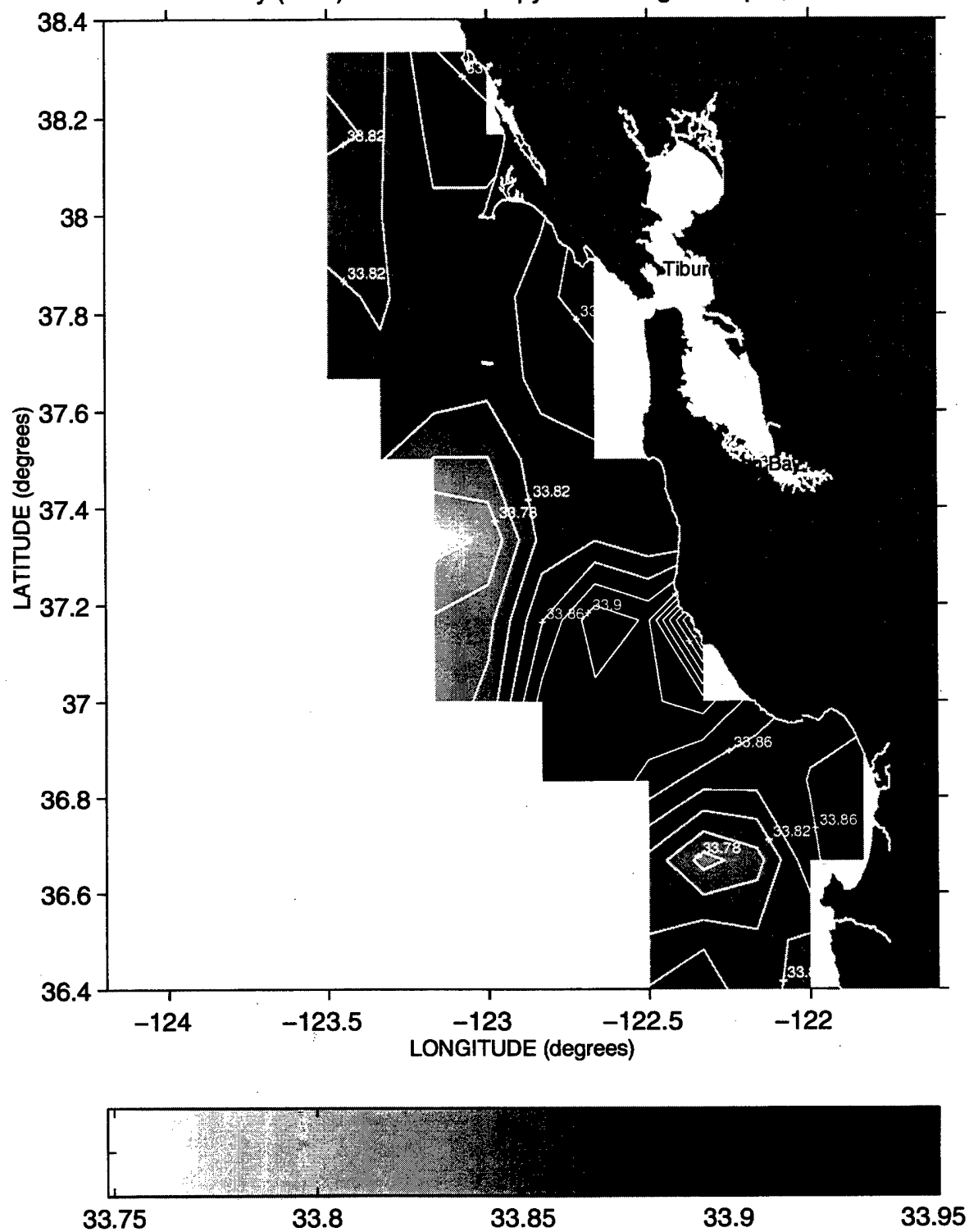
Salinity (PSS) at the 26.2 Isopycnal during Sweep 1, 1990
