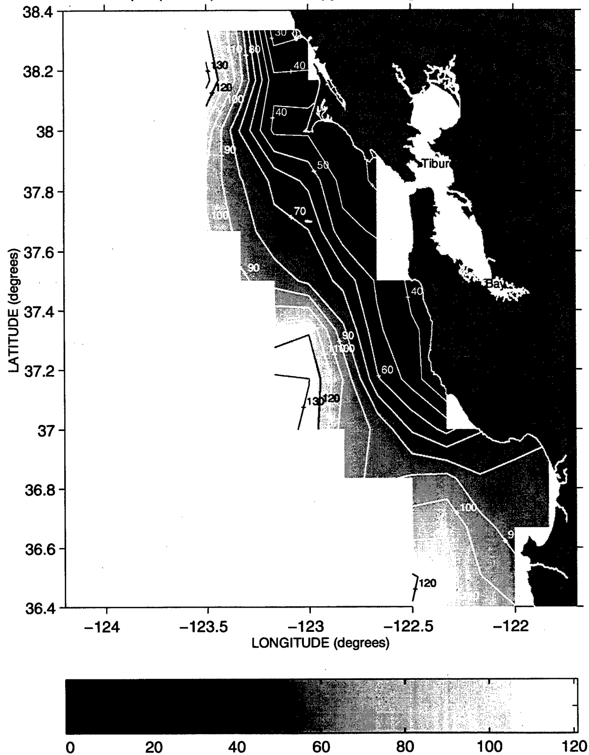
Depth (meters) of the 26.2 Isopycnal during Sweep 1, 1990
