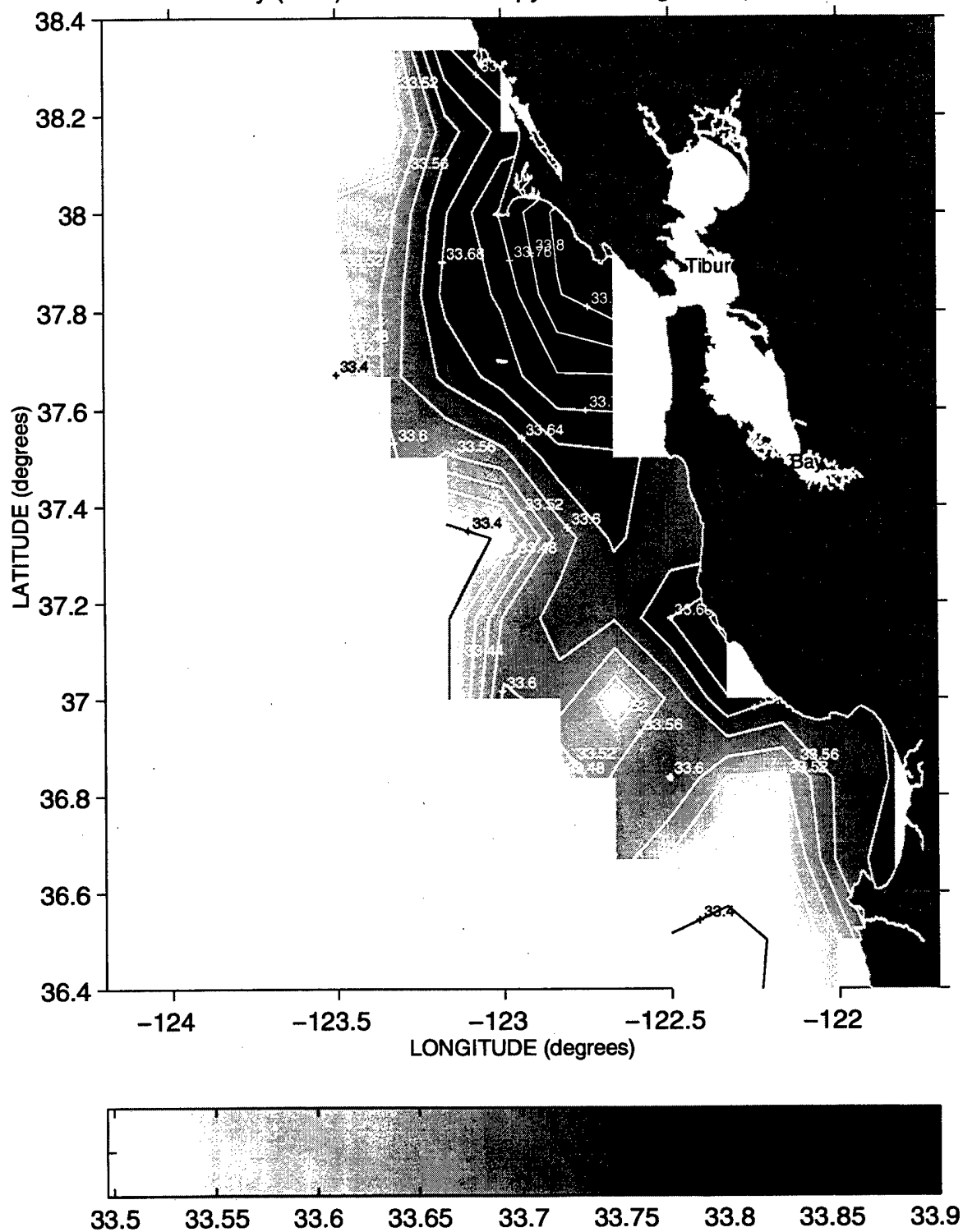
Salinity (PSS) at the 25.8 Isopycnal during Sweep 1, 1990
