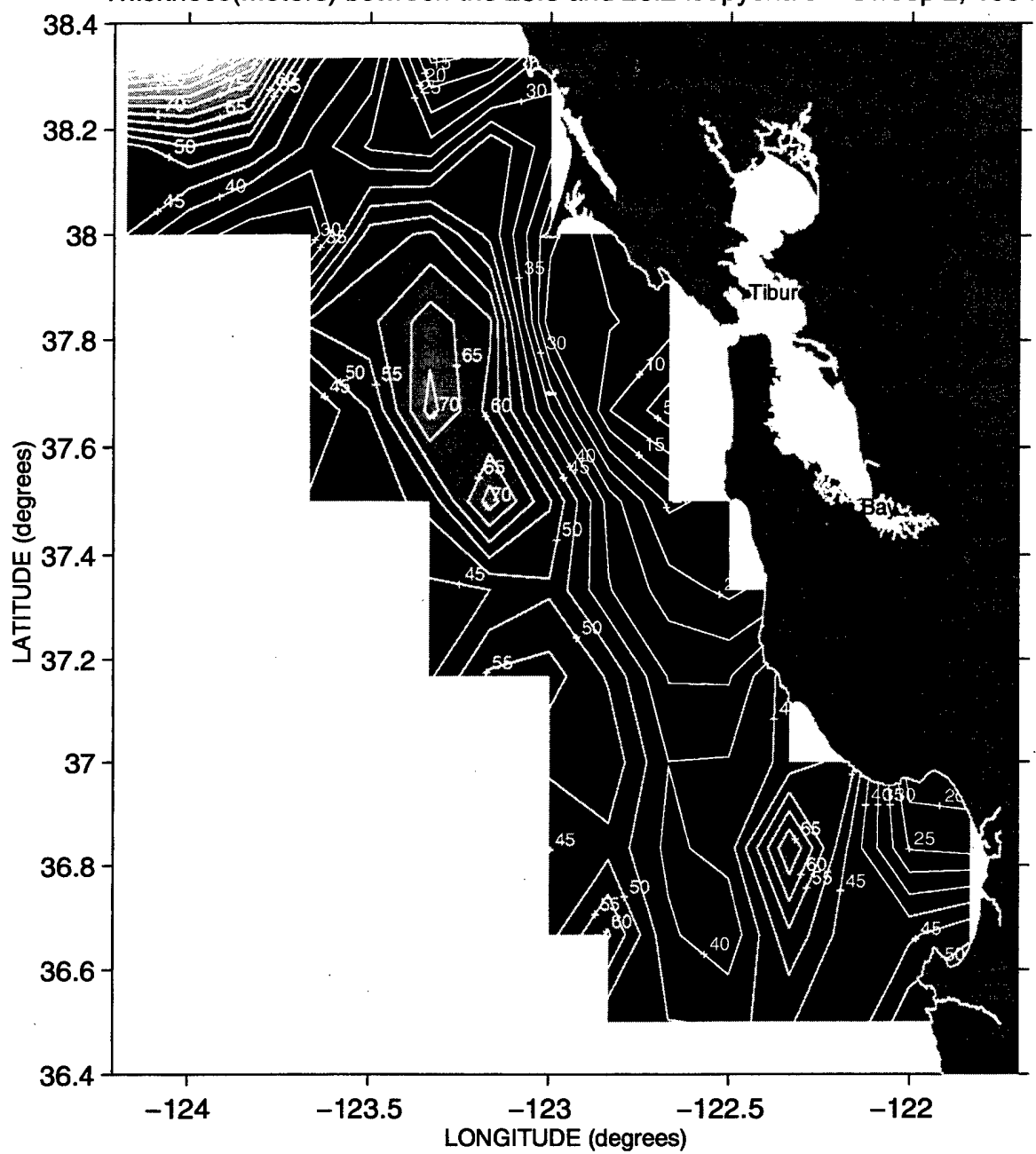
Thickness(meters) between the 25.8 and 26.2 isopycnals ~ Sweep 2, 1994
