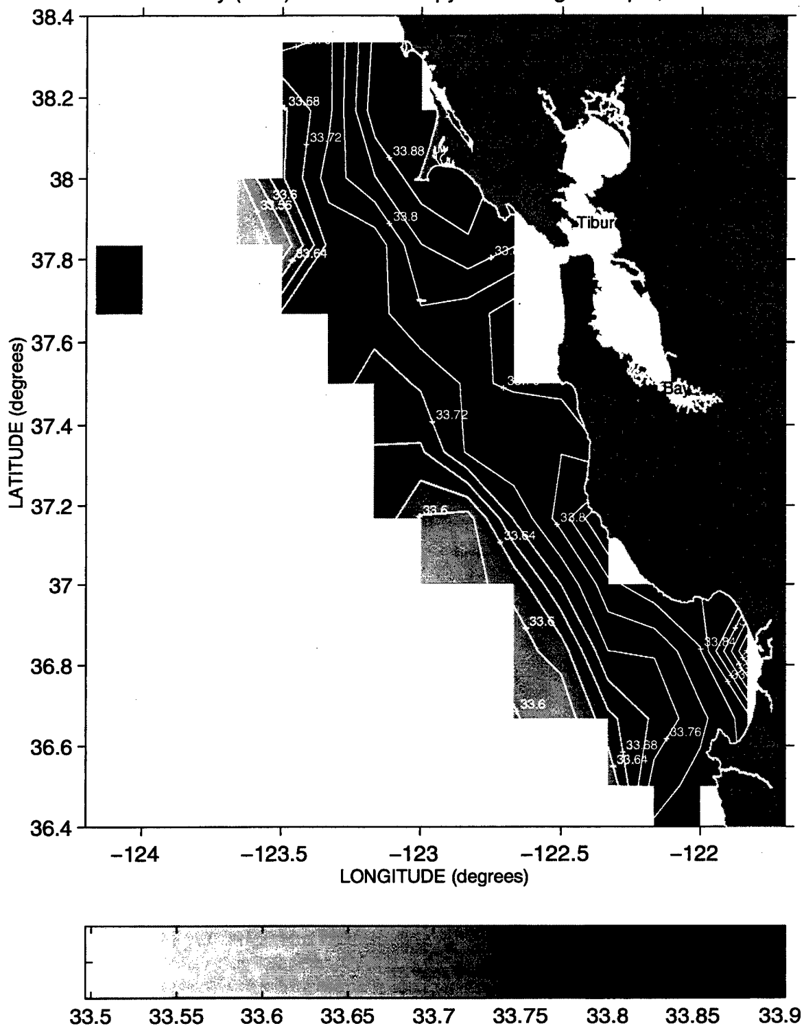
Salinity (PSS) at the 25.8 Isopycnal during Sweep 3, 1989
