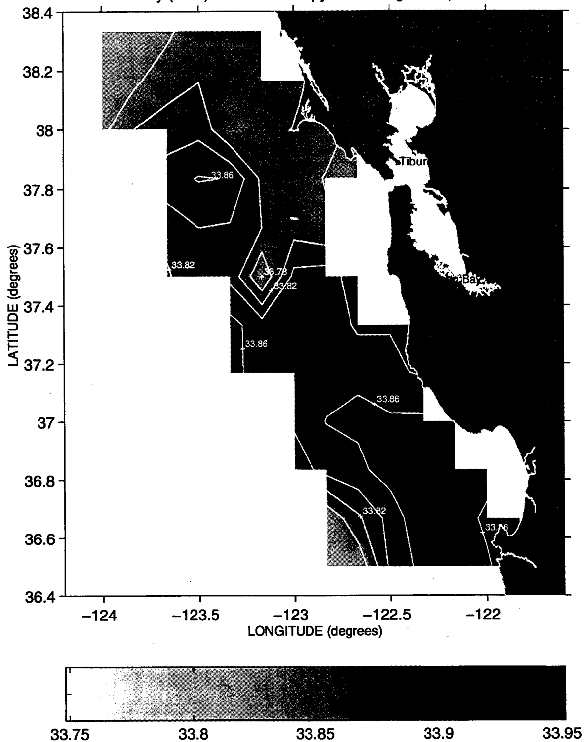
Salinity (PSS) at the 26.2 Isopycnal during Sweep 1, 1996
