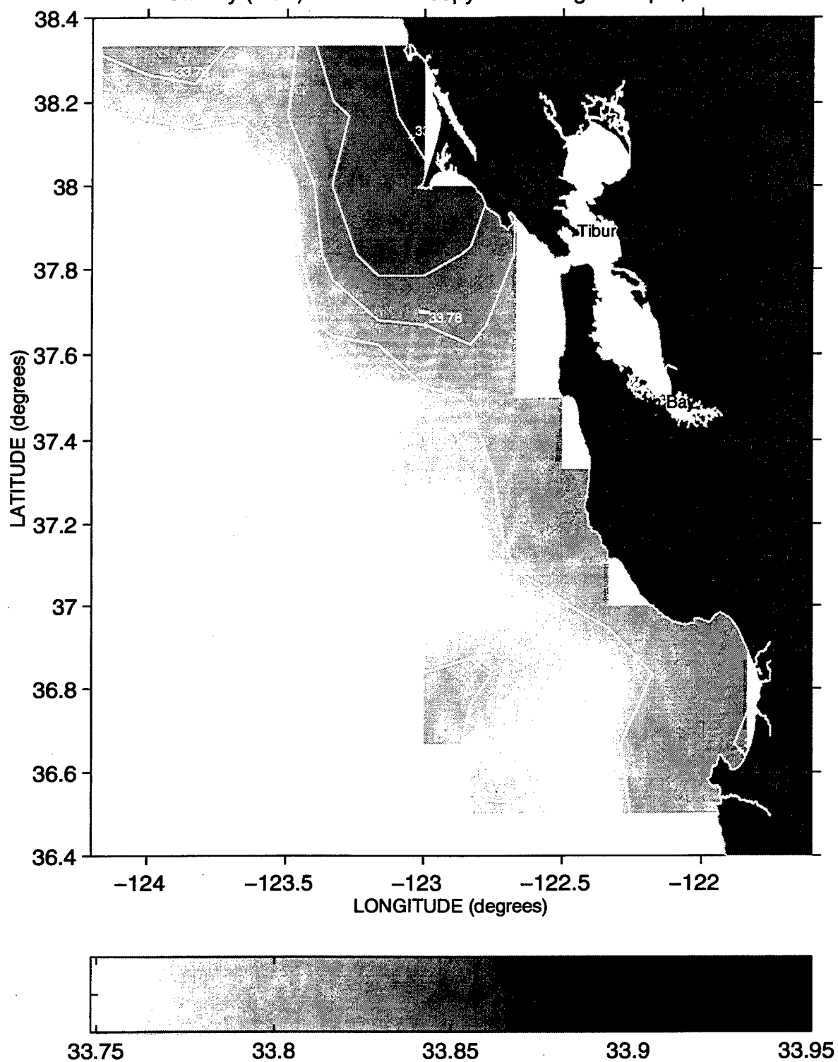
Salinity (PSS) at the 26.2 Isopycnal during Sweep 2, 1994
