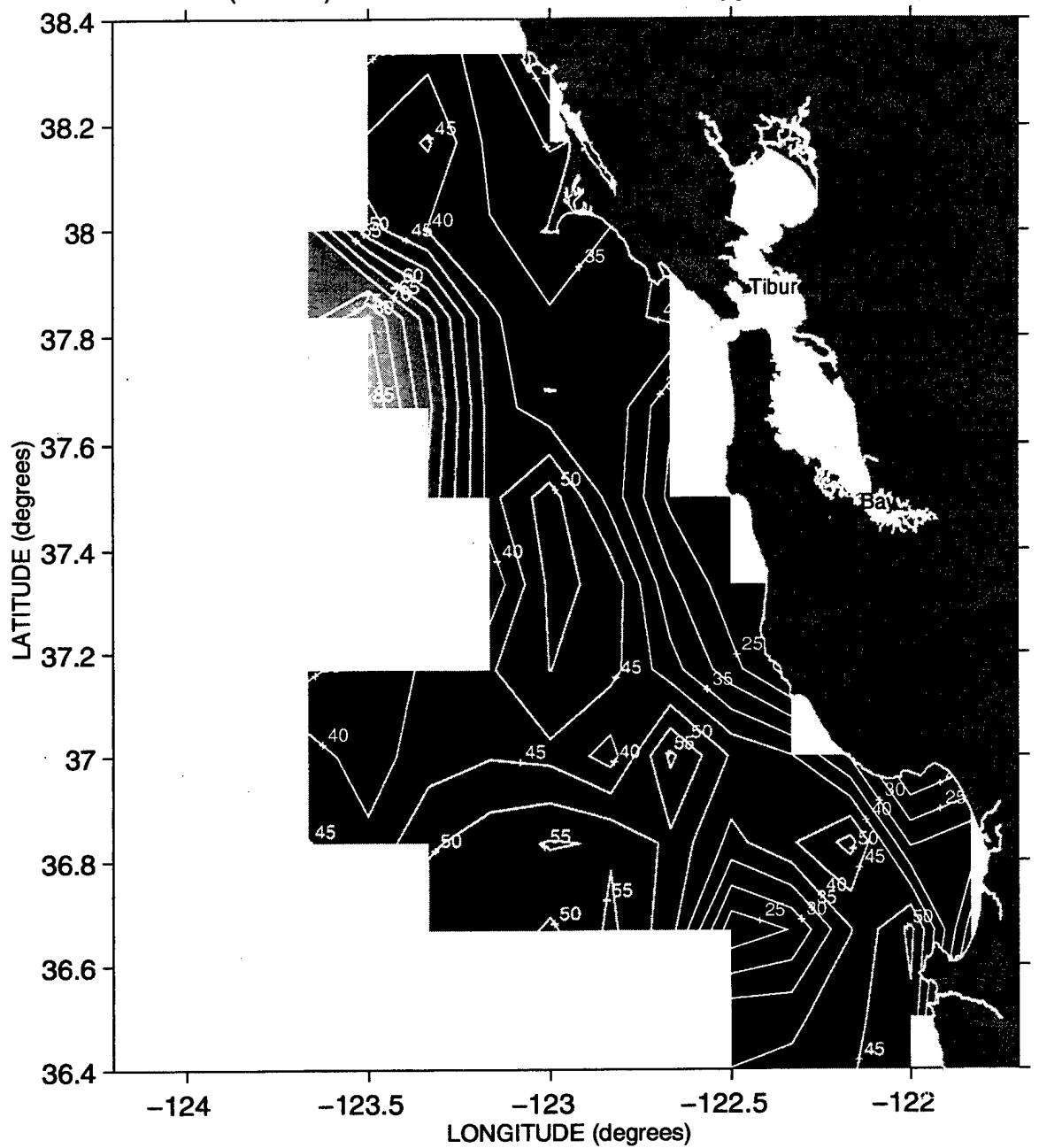
Thickness(meters) between the 25.8 and 26.2 isopycnals ~ Sweep 1, 1989
