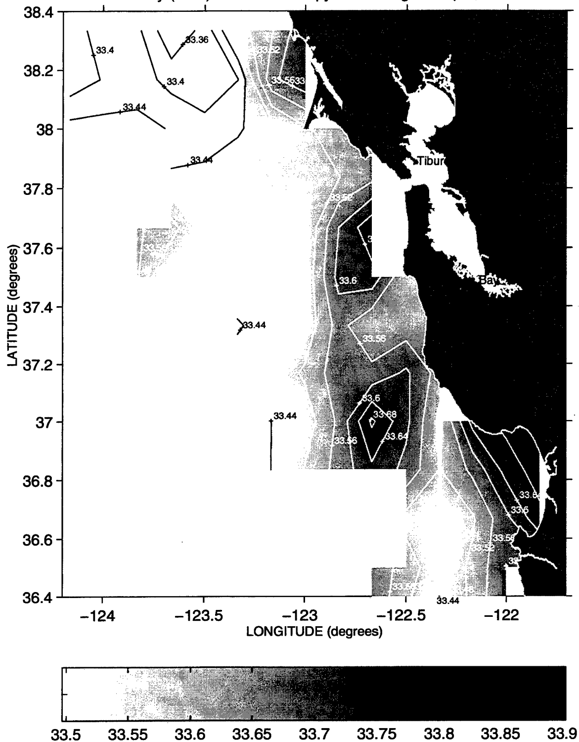
Salinity (PSS) at the 25.8 Isopycnal during Sweep 1, 1993
