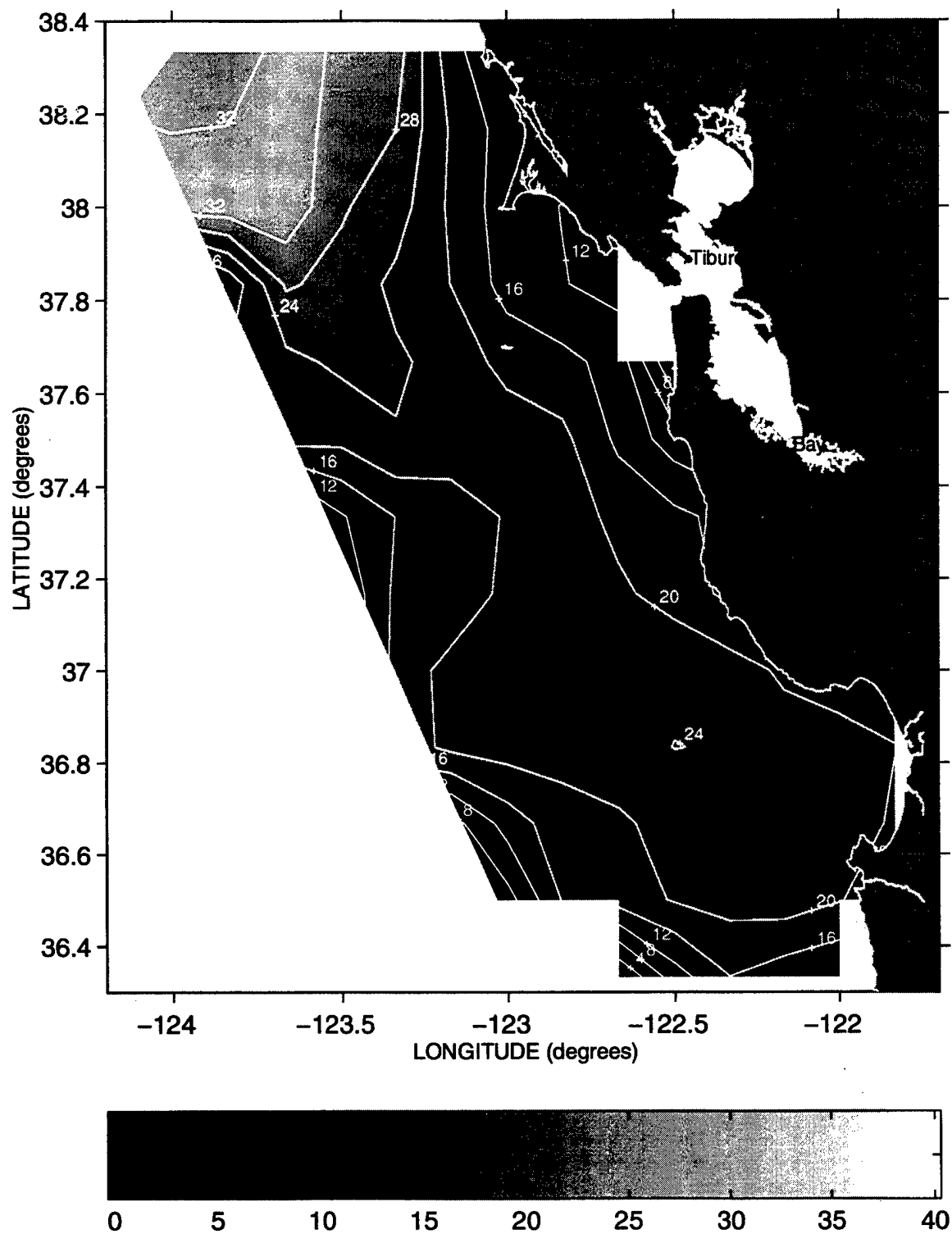
Figure 10. Standard deviations of the 25.8 kg/m 3 isopycnal depths during May-June, 1987-1996. Contour interval is 4 meters.
