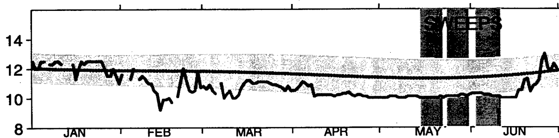
Surface Salinity ~ 1990
