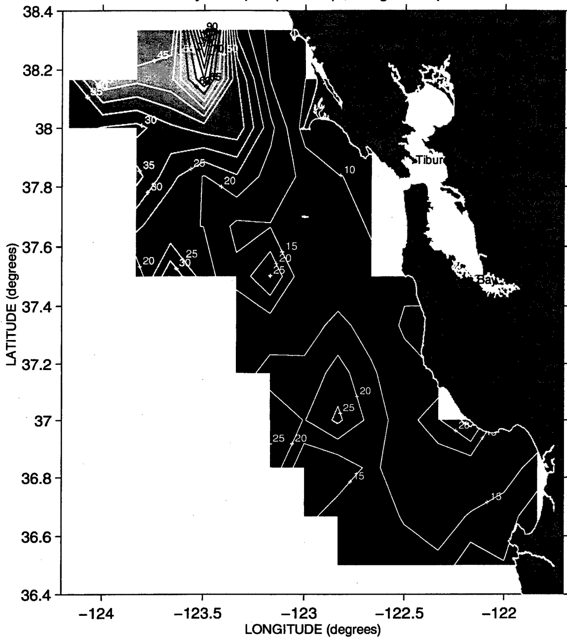
Mixed Layer Depth (meters) during Sweep 3, 1991
