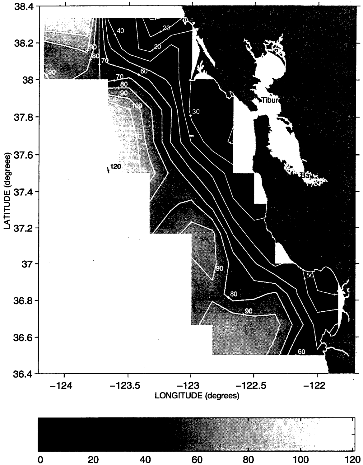
Depth (meters) of the 26.2 Isopycnal during Sweep 2, 1994
