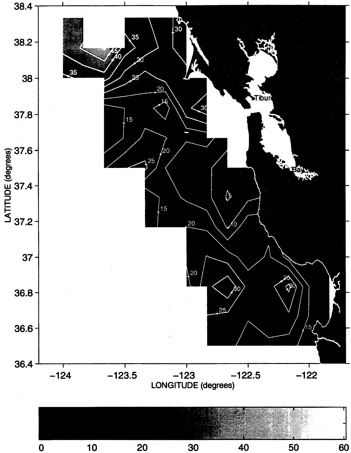
Mixed Layer Depth (meters) during Sweep 2, 1995
