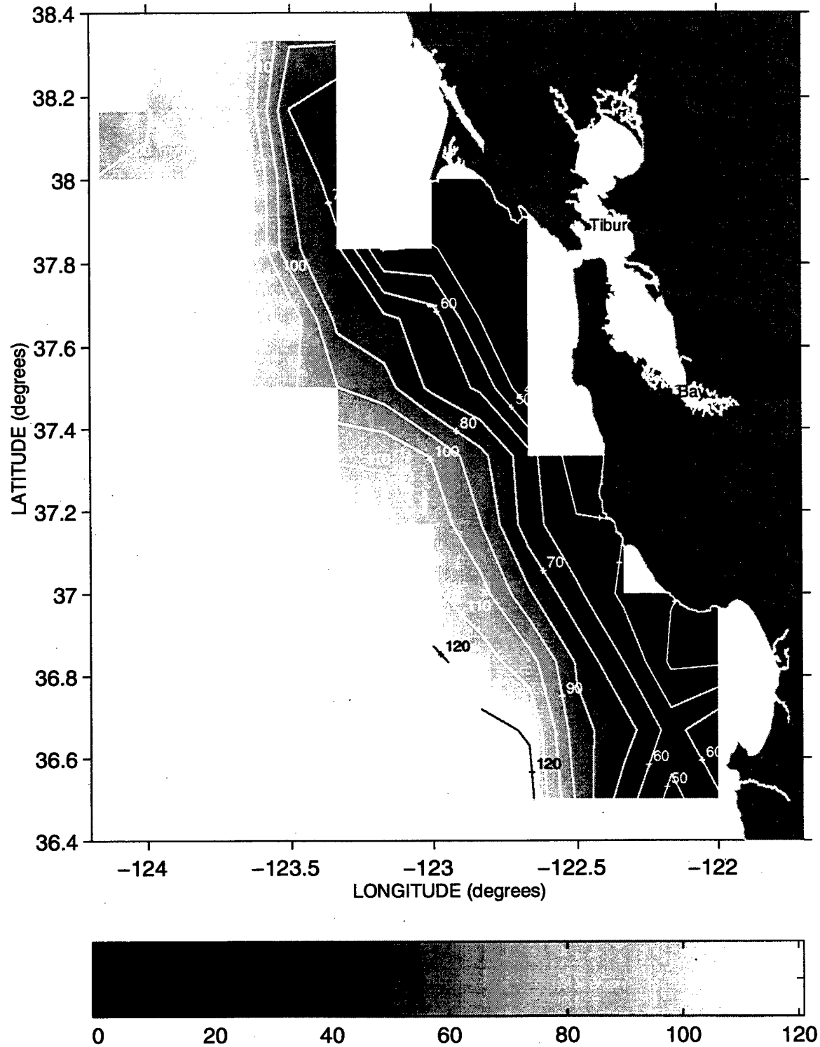
Depth (meters) of the 26.2 Isopycnal during Sweep 1, 1994
