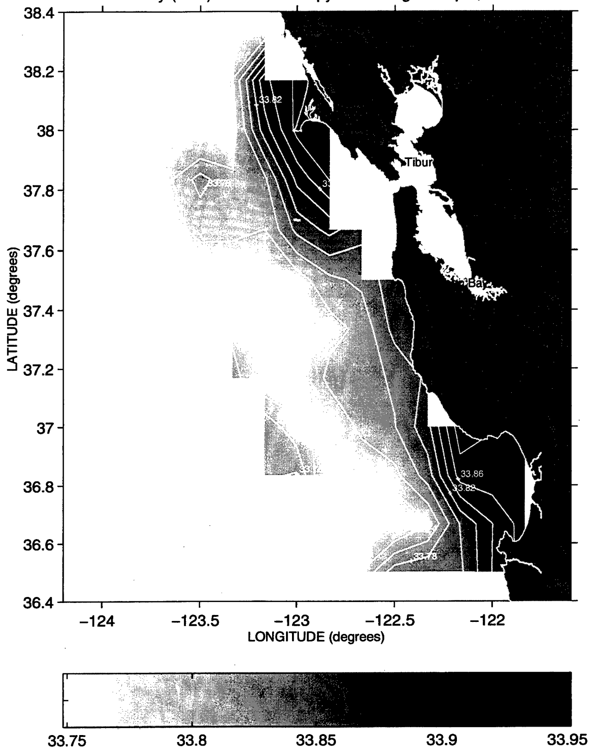
Salinity (PSS) at the 26.2 Isopycnal during Sweep 1, 1991
