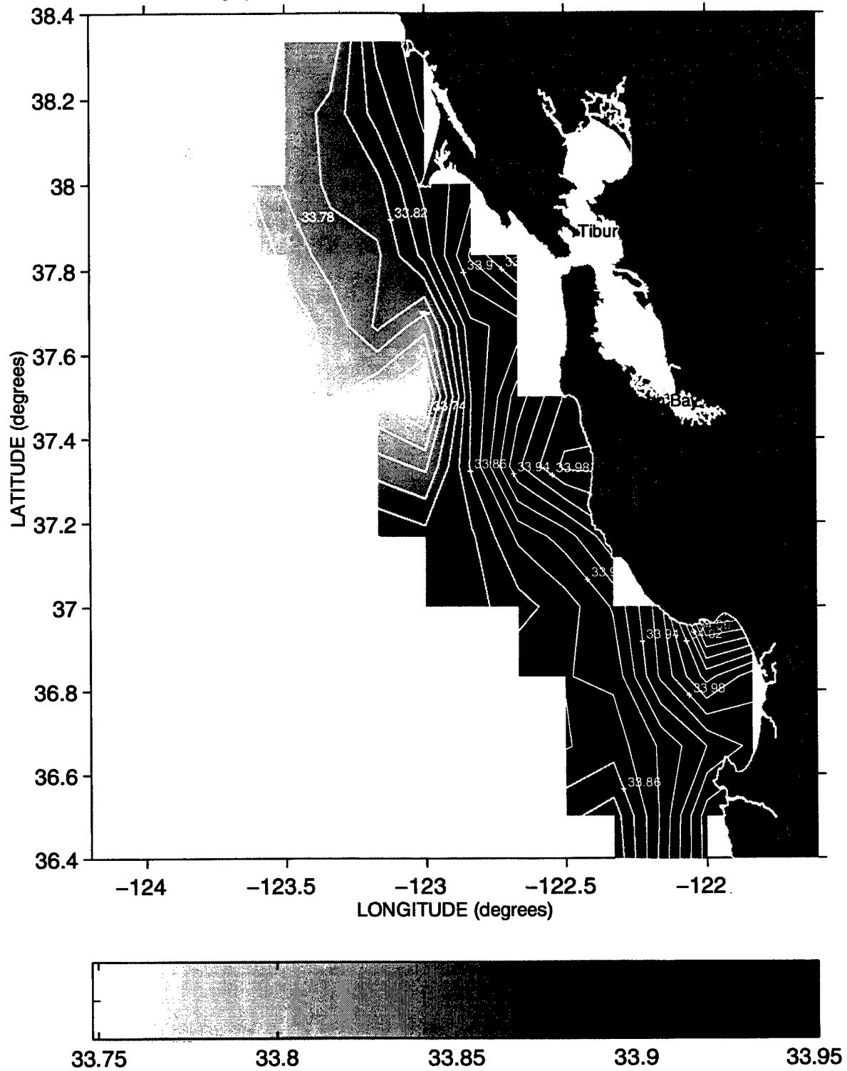
Salinity (PSS) at the 26.2 Isopycnal during Sweep 3, 1988
