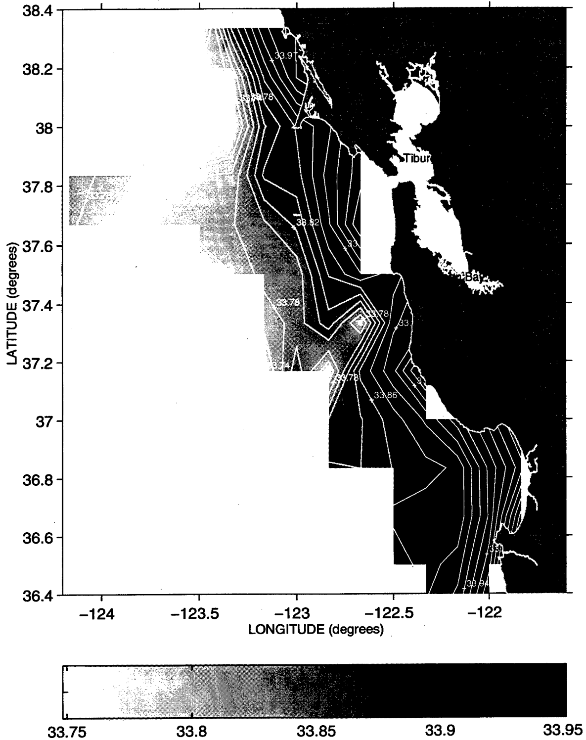
Salinity (PSS) at the 26.2 Isopycnal during Sweep 2, 1988
