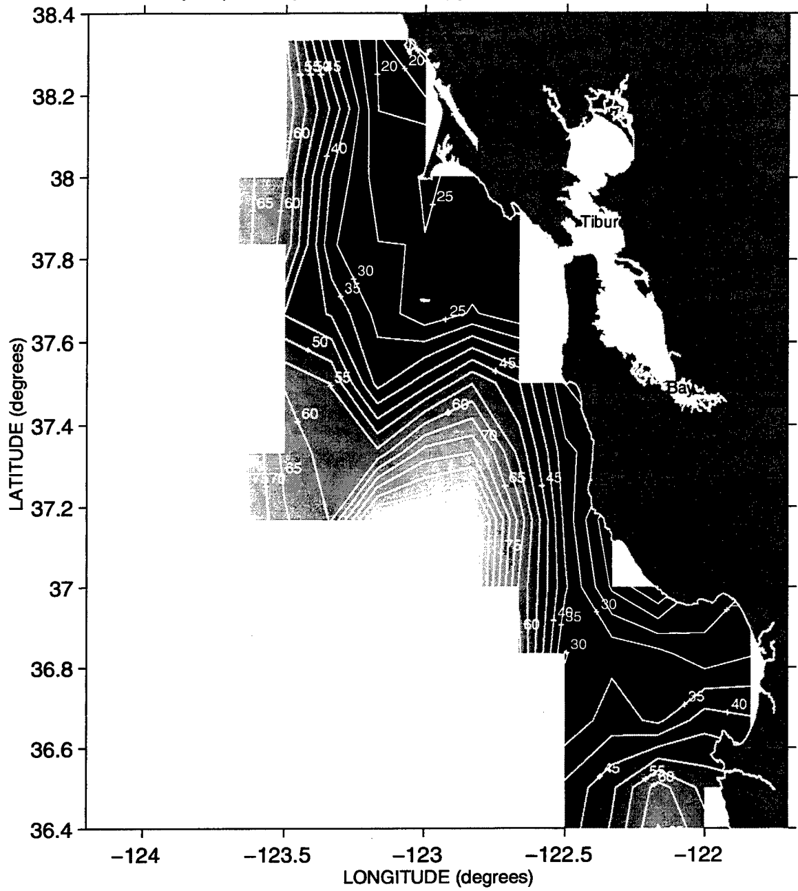
Depth (meters) of the 25.8 Isopycnal during Sweep 2, 1990
