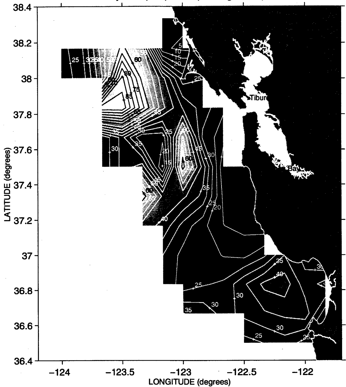
Mixed Layer Depth (meters) during Sweep 2, 1991
