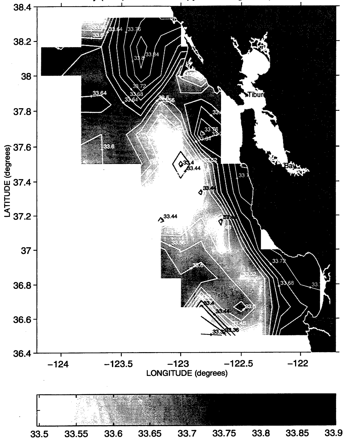
Salinity (PSS) at the 25.8 Isopycnal during Sweep 3, 1991
