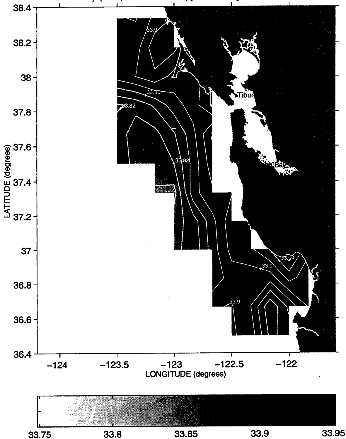
Salinity (PSS) at the 26.2 Isopycnal during Sweep 3, 1987
