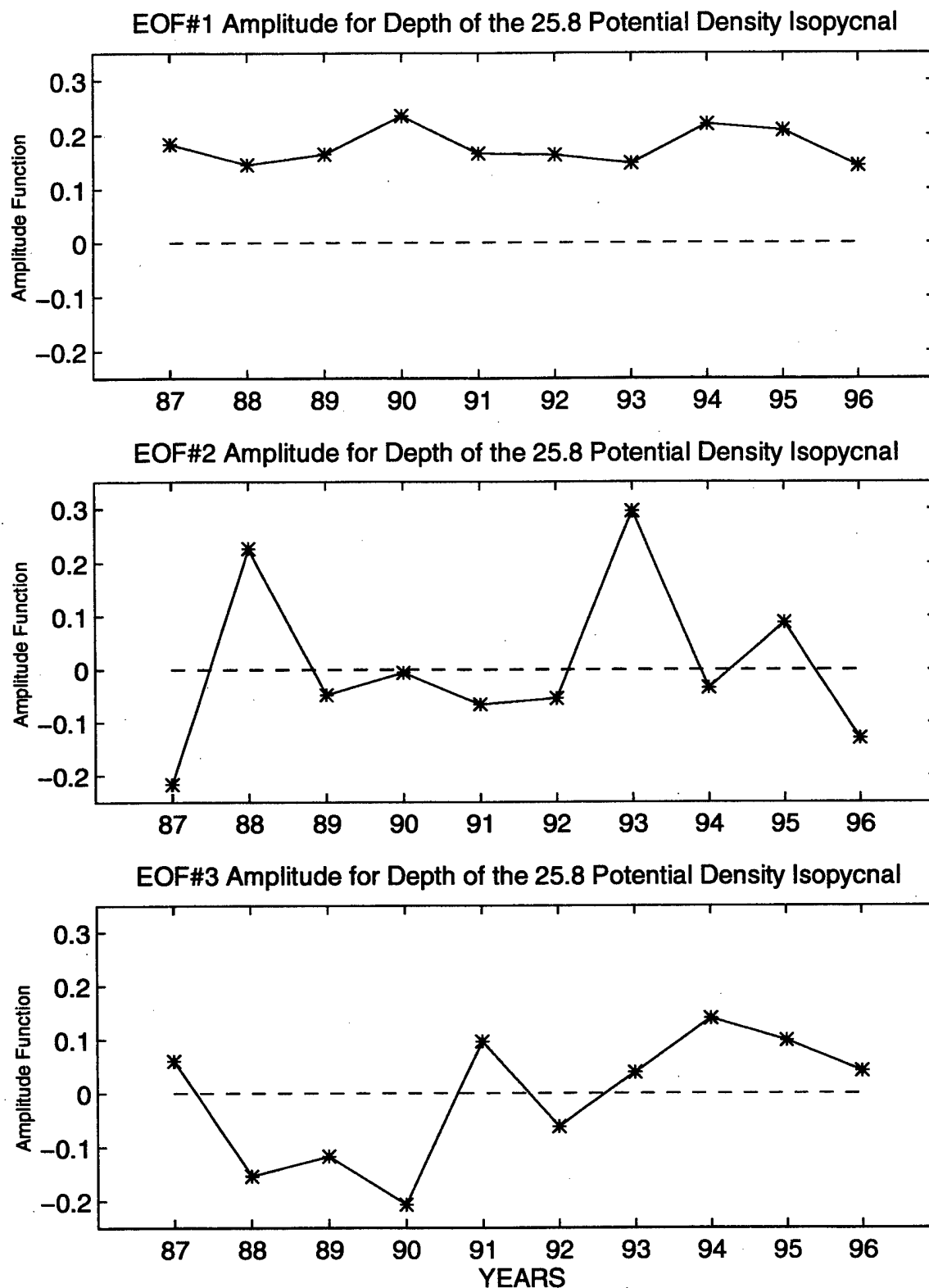
Figure 37. Temporal amplitudes of the first three EOF modes for the 25.8 kg/m 3 isopycnal depth.
