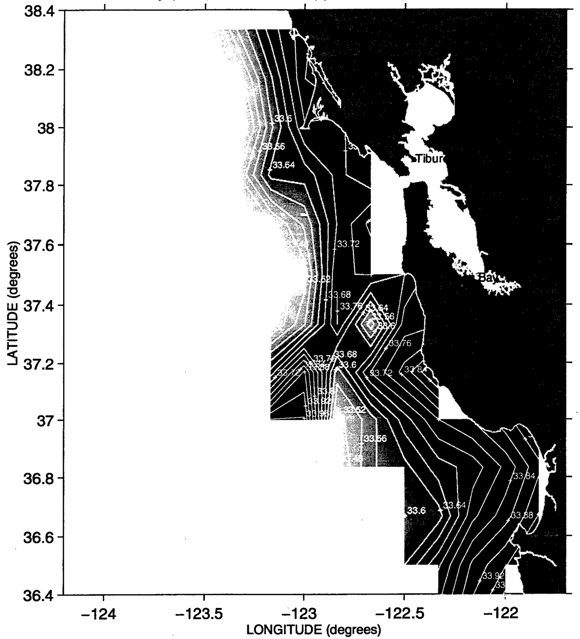
Salinity (PSS) at the 25.8 Isopycnal during Sweep 2, 1988
