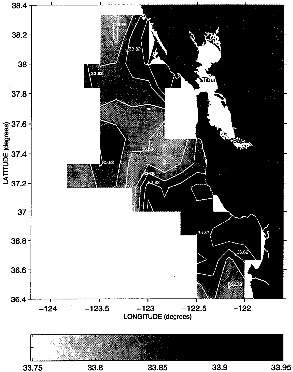
Salinity (PSS) at the 26.2 Isopycnal during Sweep 2, 1990
