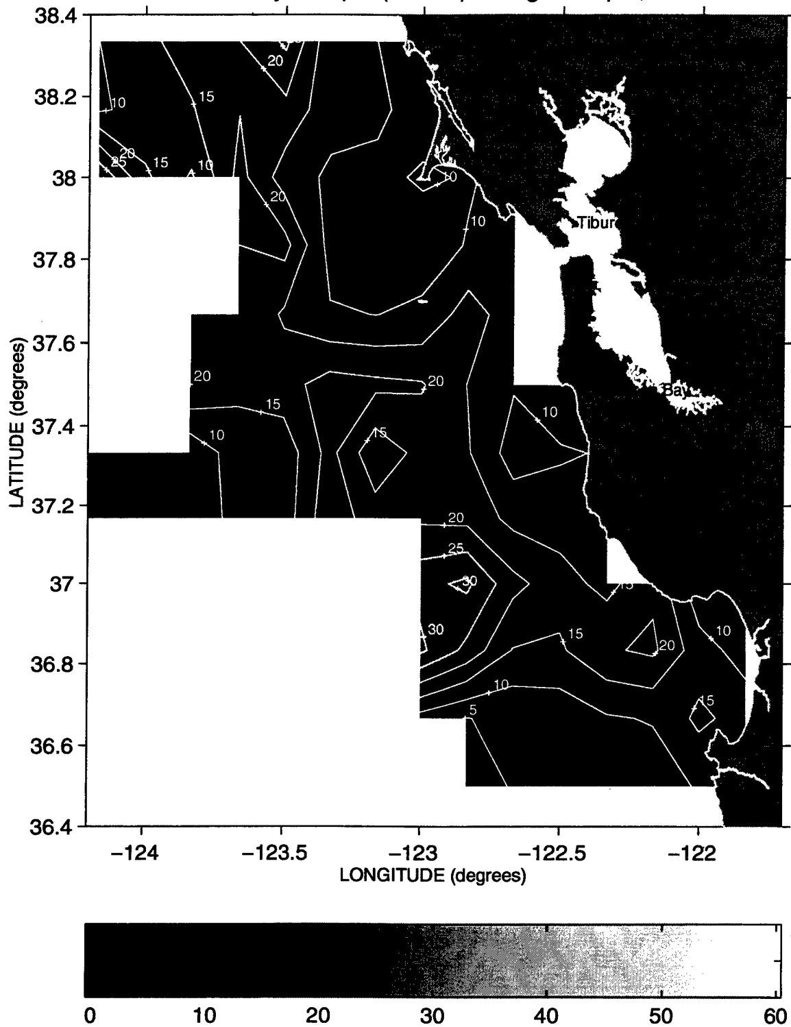
Mixed Layer Depth (meters) during Sweep 2, 1992
