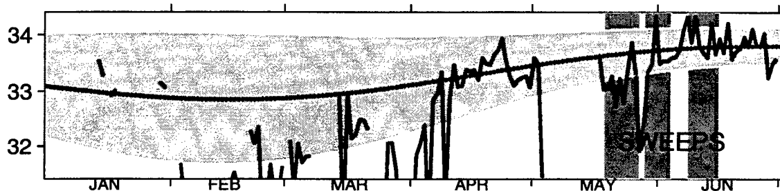
Sea Surface Temperature ~ 1996
