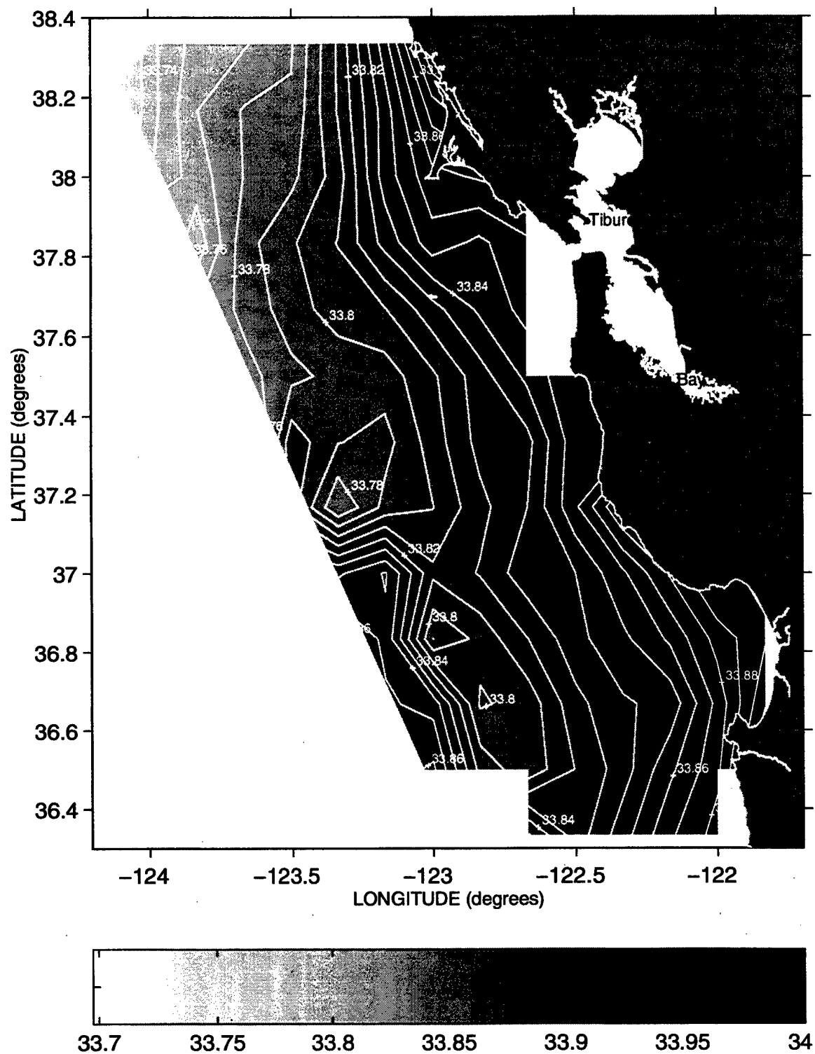
Figure 13. Mean Salinity (PSS) on the 26.2 \text{ kg/m}^3 isopycnal during May-June, 1987-1996. Contour interval is 0.01.
