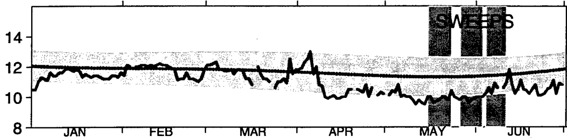
Surface Salinity ~ 1991
