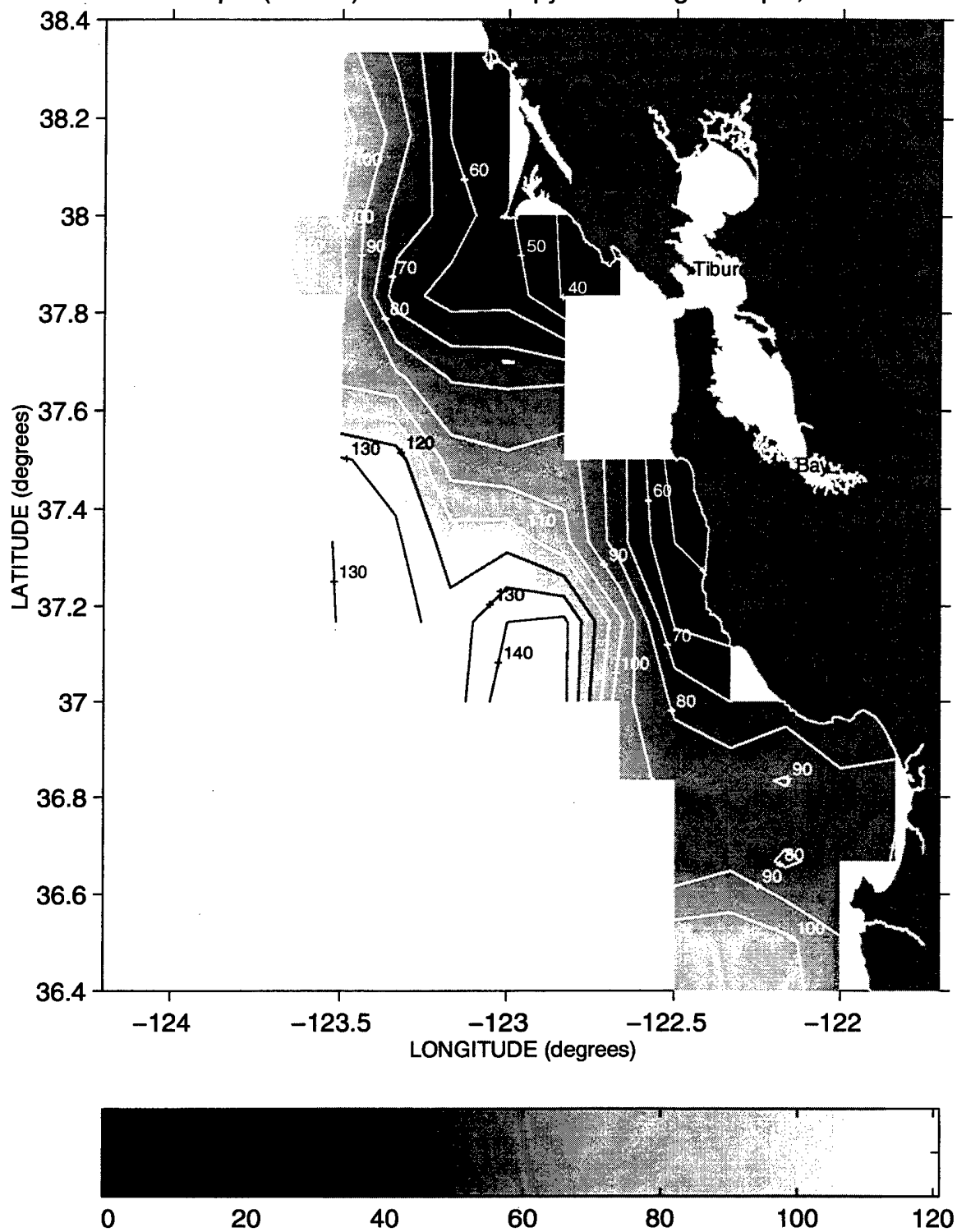
Depth (meters) of the 26.2 Isopycnal during Sweep 2, 1990
