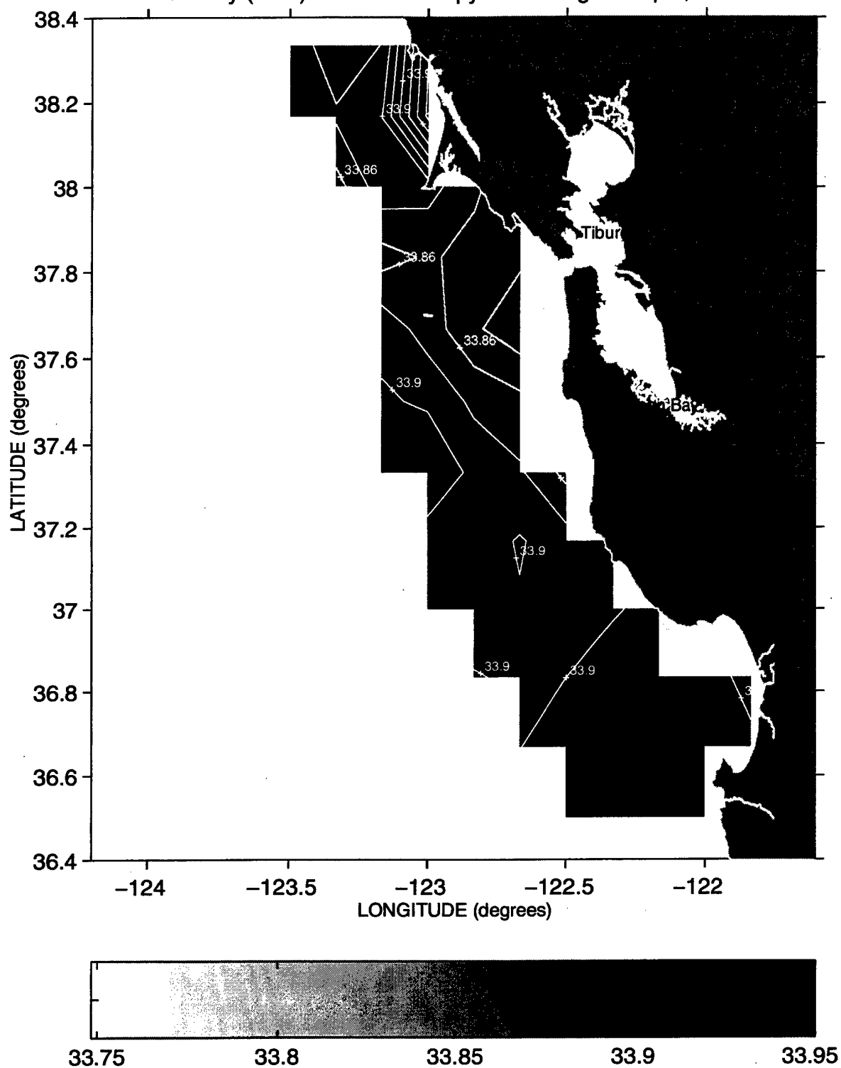
Salinity (PSS) at the 26.2 Isopycnal during Sweep 1, 1987
