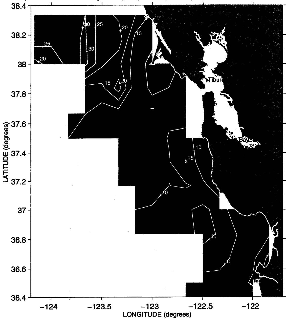
Mixed Layer Depth (meters) during Sweep 1, 1993
