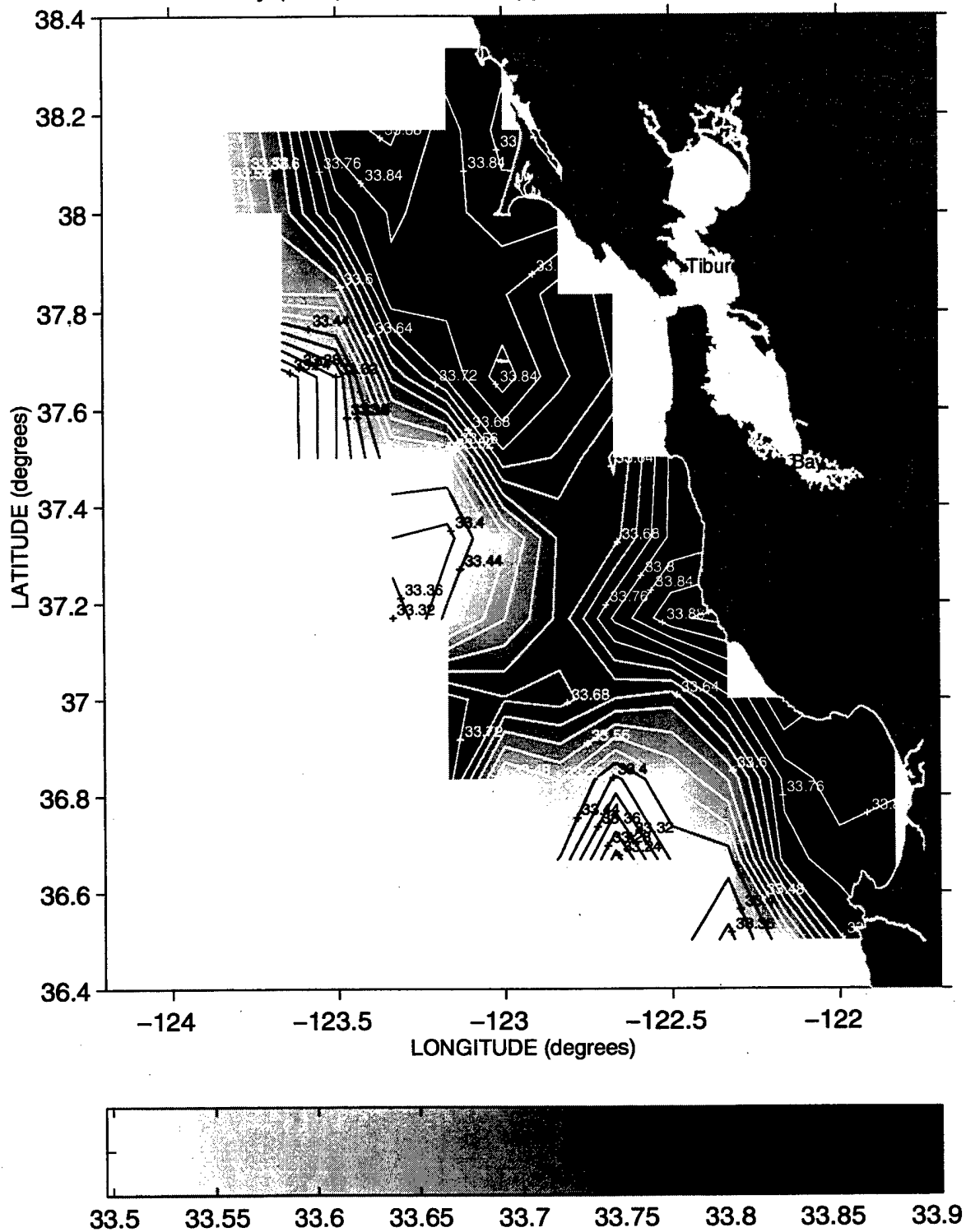
Salinity (PSS) at the 25.8 Isopycnal during Sweep 2, 1991
