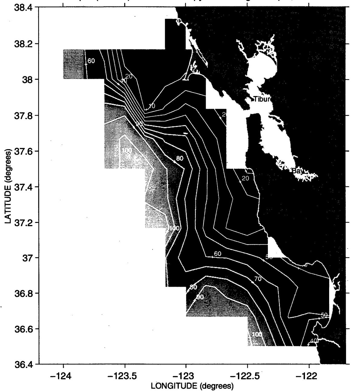
Depth (meters) of the 26.2 Isopycnal during Sweep 2, 1991
