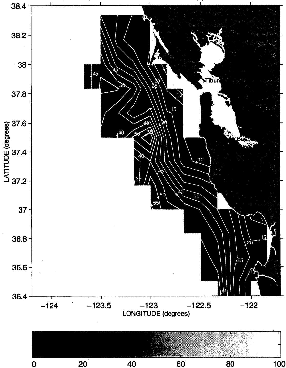
Thickness(meters) between the 25.8 and 26.2 isopycnals ~ Sweep 3, 1988
