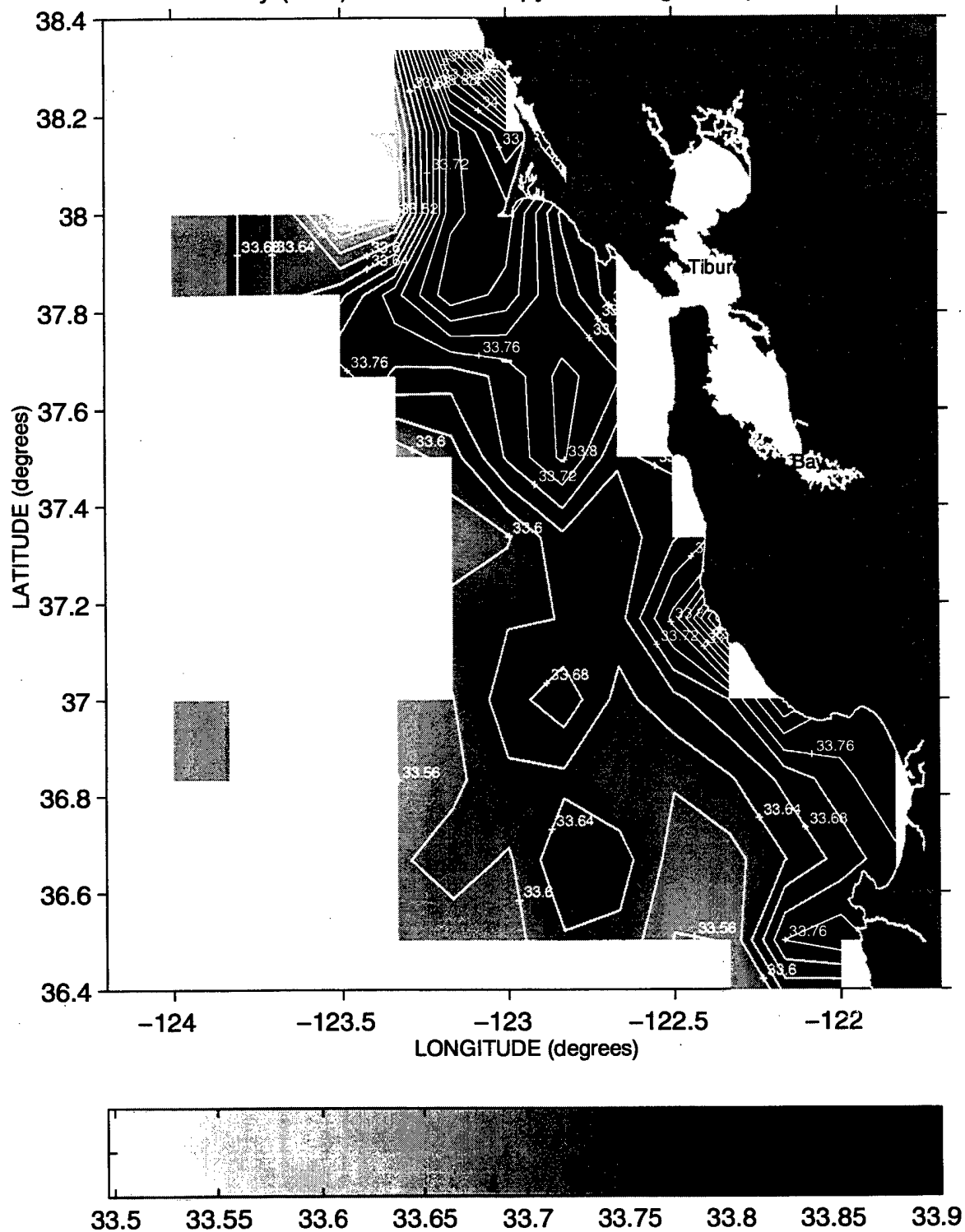
Salinity (PSS) at the 25.8 Isopycnal during Sweep 2, 1989
