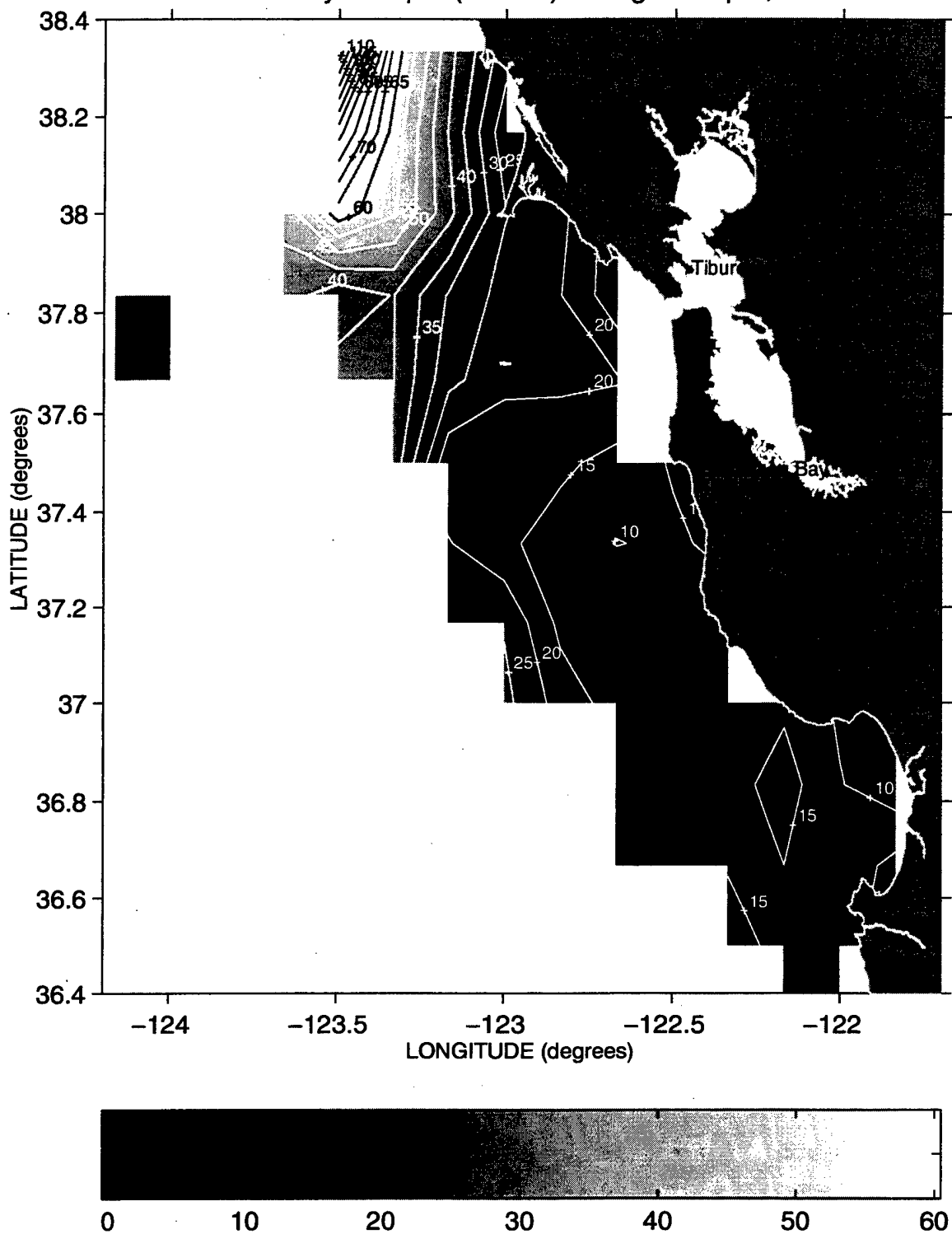
Mixed Layer Depth (meters) during Sweep 3, 1989
