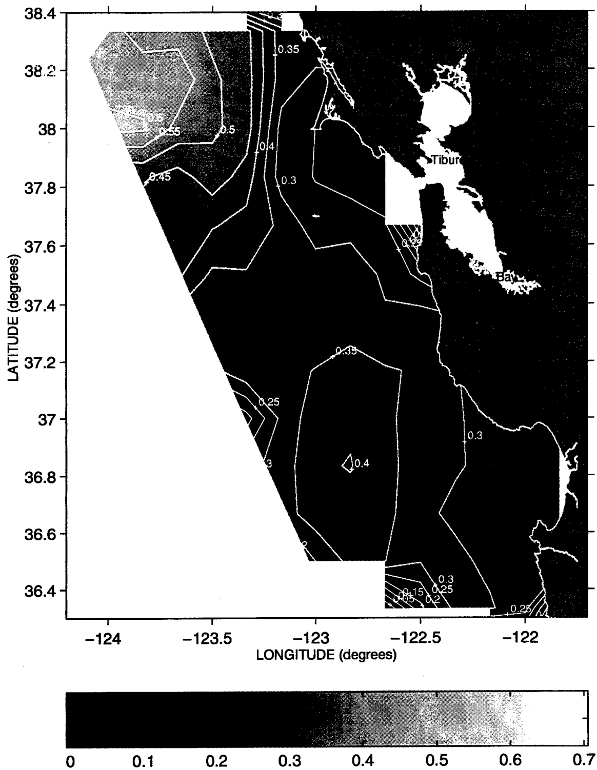
Figure 21. Standard deviations of potential density anomaly at 30 meters during May-June, 1987-1996. Contour interval is 0.05 kg/m 3 .
