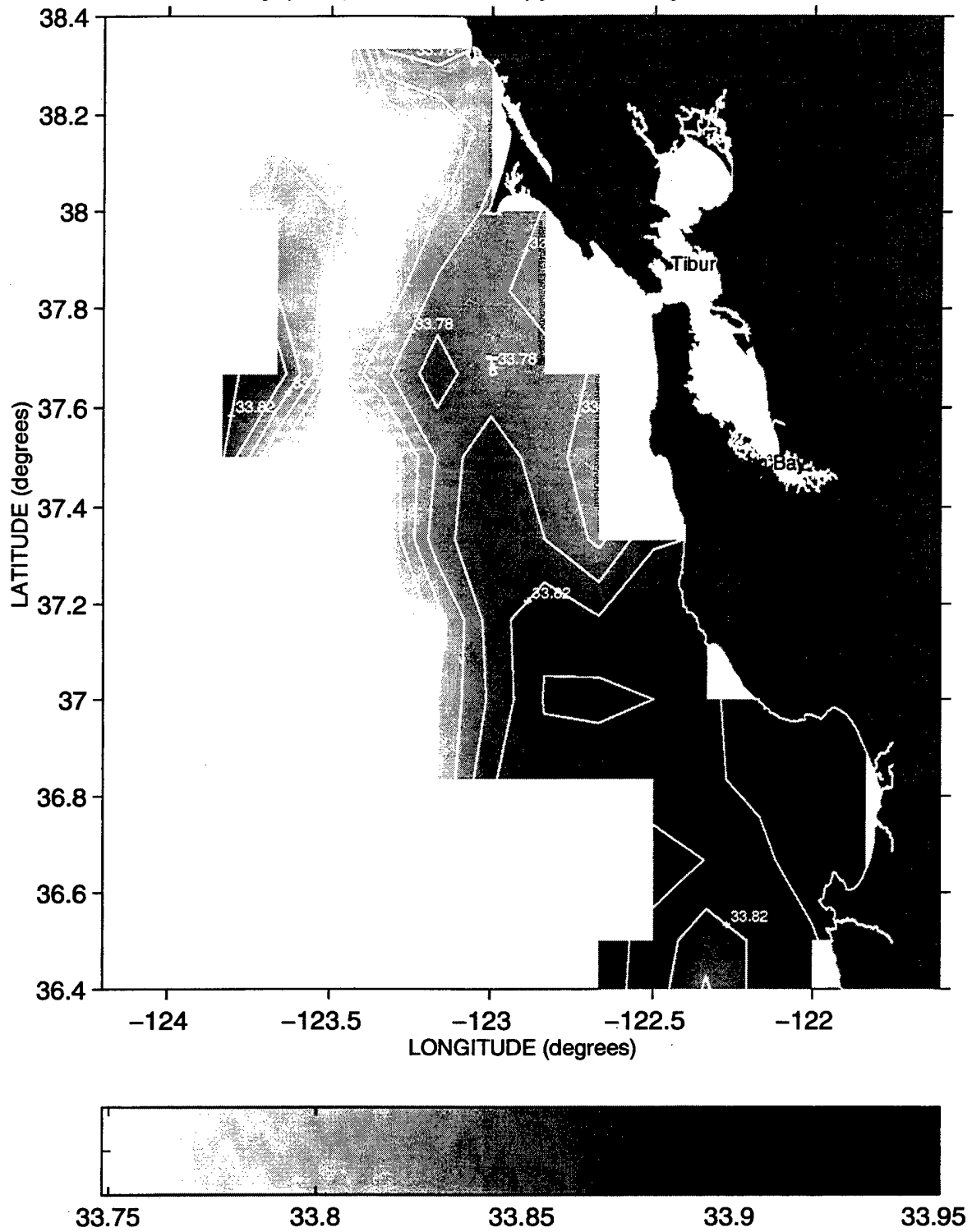
Salinity (PSS) at the 26.2 Isopycnal during Sweep 1, 1993
