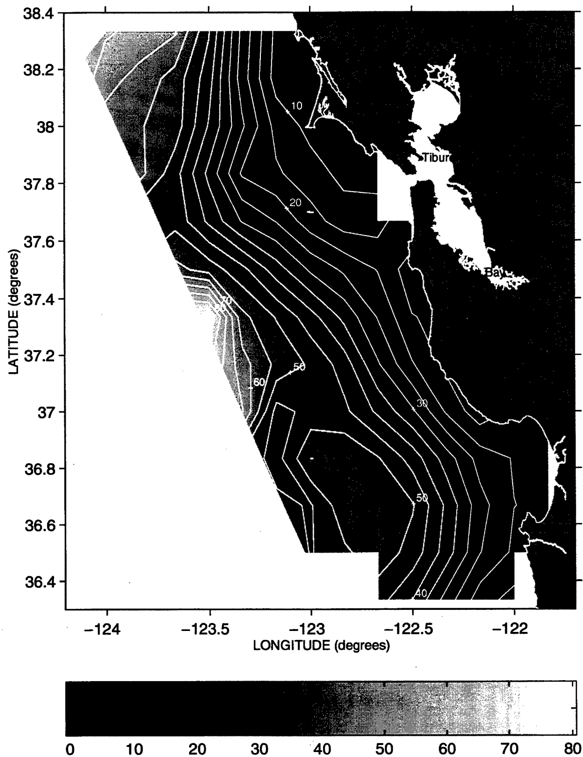
Figure 8. Mean depths of the 25.8 kg/m 3 isopycnal during May-June, 1987-1996. Contour interval is 5 meters.
