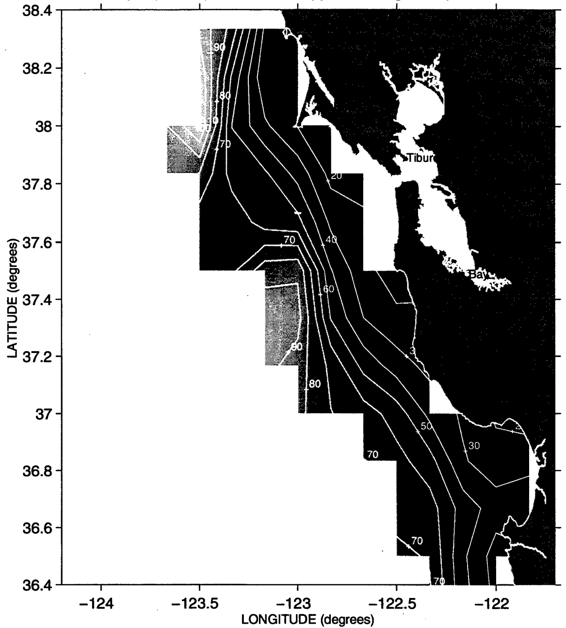
Depth (meters) of the 26.2 Isopycnal during Sweep 3, 1988
