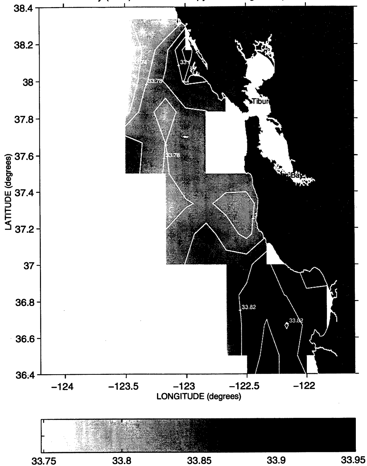
Salinity (PSS) at the 26.2 Isopycnal during Sweep 3, 1990
