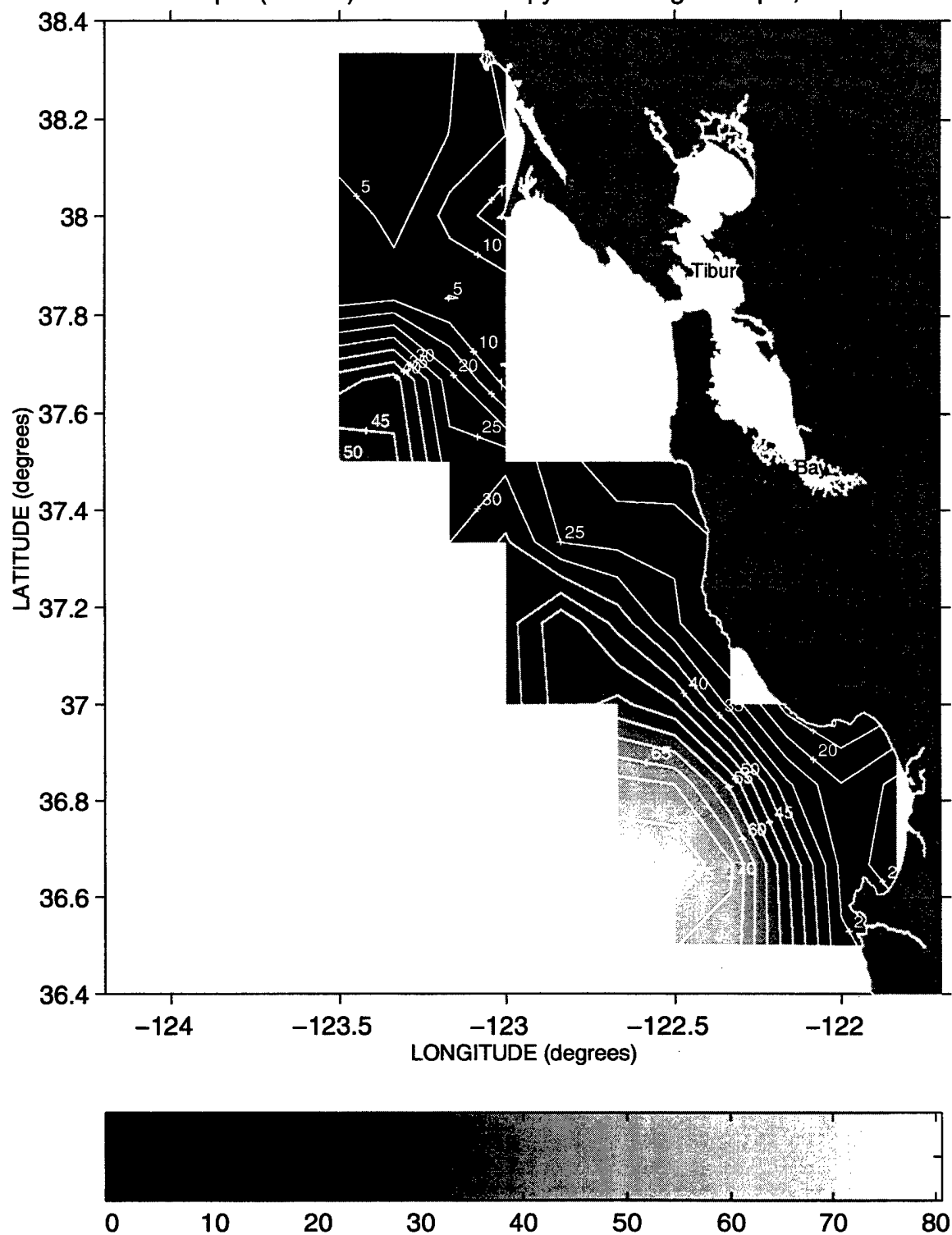
Depth (meters) of the 25.8 Isopycnal during Sweep 2, 1987
