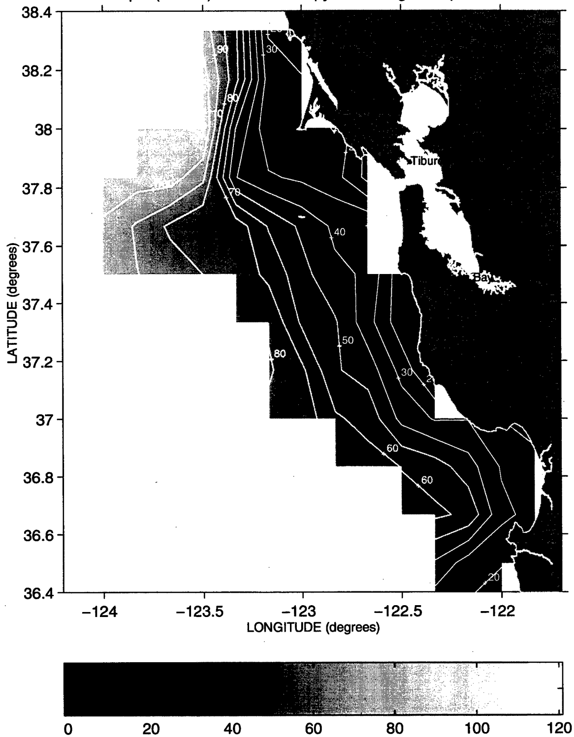
Depth (meters) of the 26.2 Isopycnal during Sweep 1, 1988
