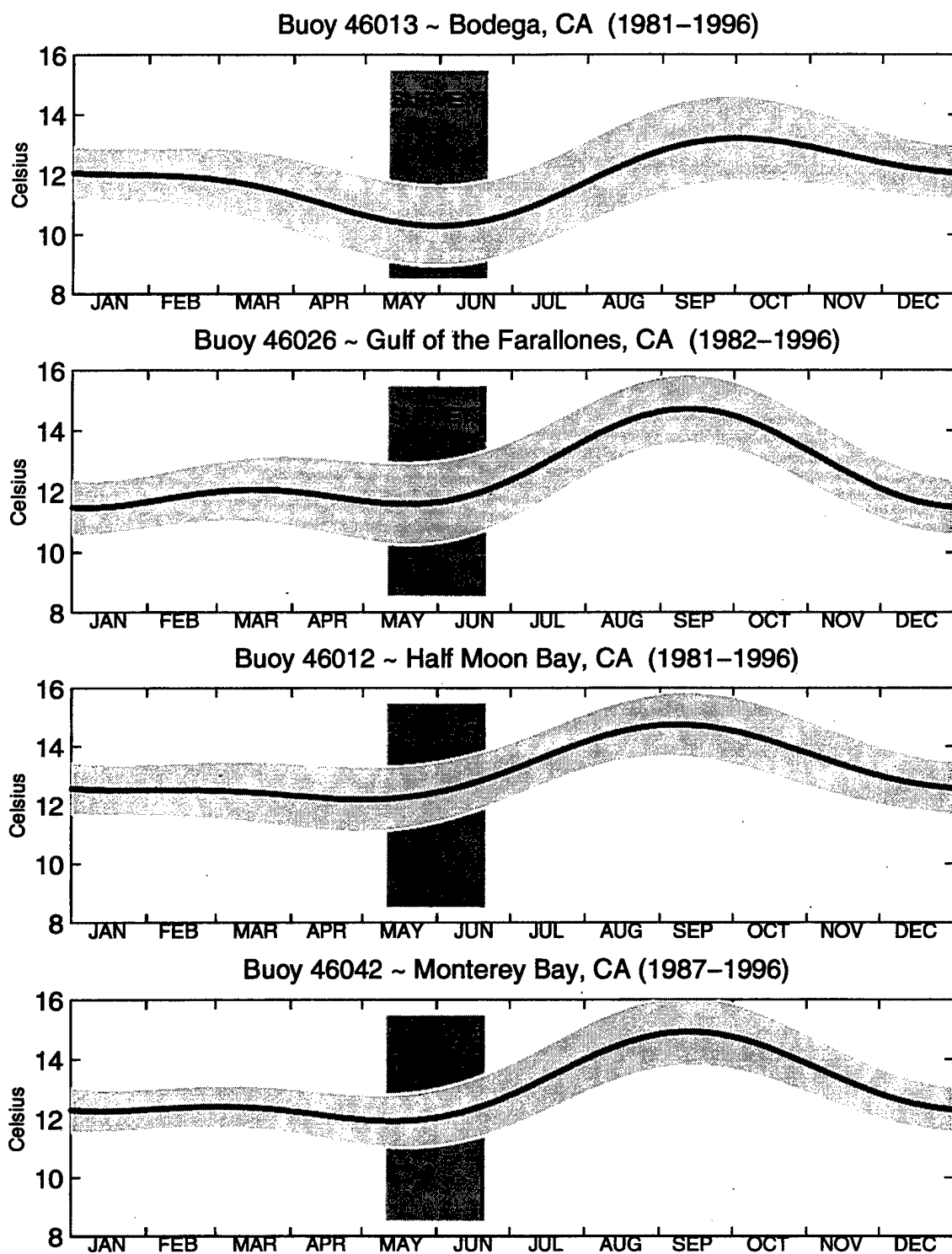
Figure 5. SST climatologies from NOAA Buoys. The bold curve denotes the harmonic fits to the daily data. The light gray shaded area around the bold curve is plus and minus one standard error. The dark gray shaded area denotes the survey period.
