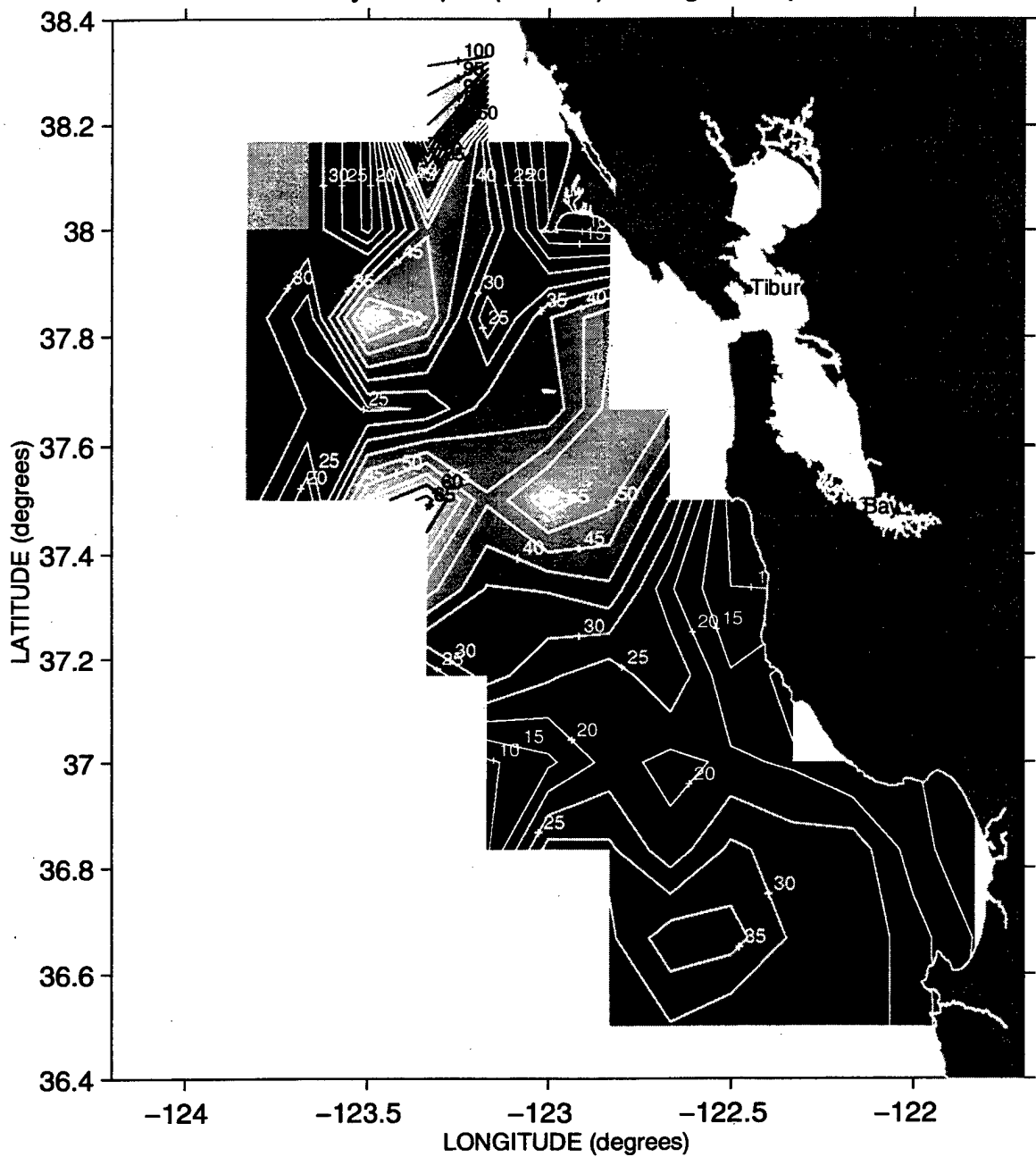
Mixed Layer Depth (meters) during Sweep 1, 1991
