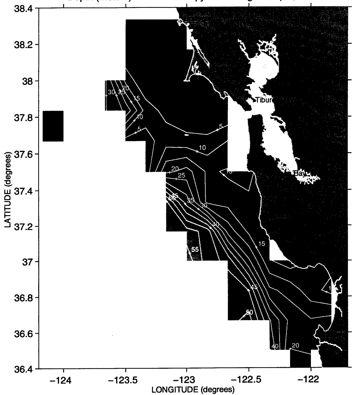
Depth (meters) of the 25.8 Isopycnal during Sweep 3, 1989
