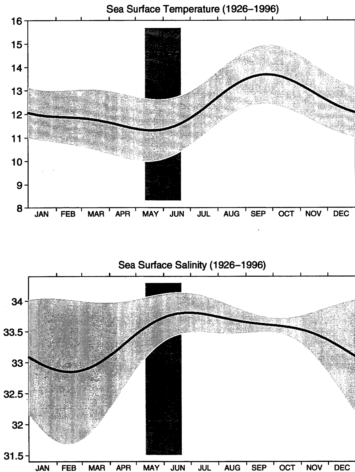
Figure 6. SST and SSS climatologies at Southeast Farallon Island. The bold curve denotes the fits to the daily data. The light gray shaded area around the bold curve is plus and minus one standard error. The dark gray shaded area is the survey period.
