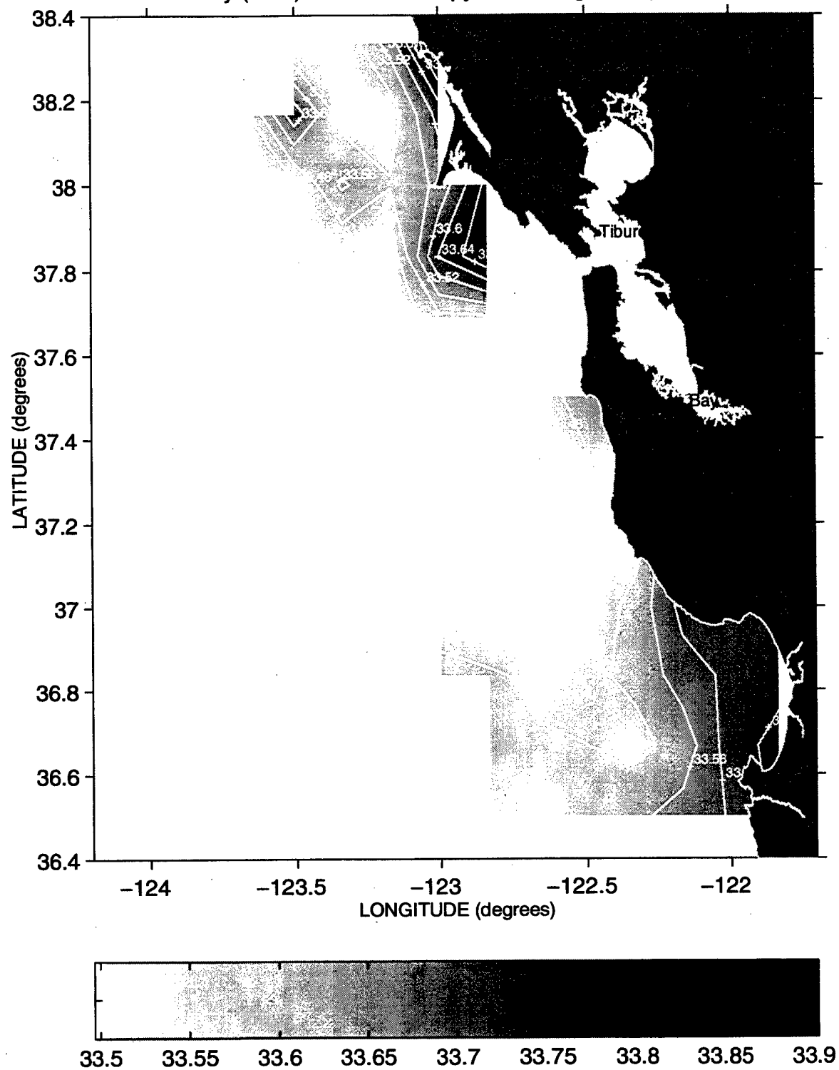
Salinity (PSS) at the 25.8 Isopycnal during Sweep 2, 1995
