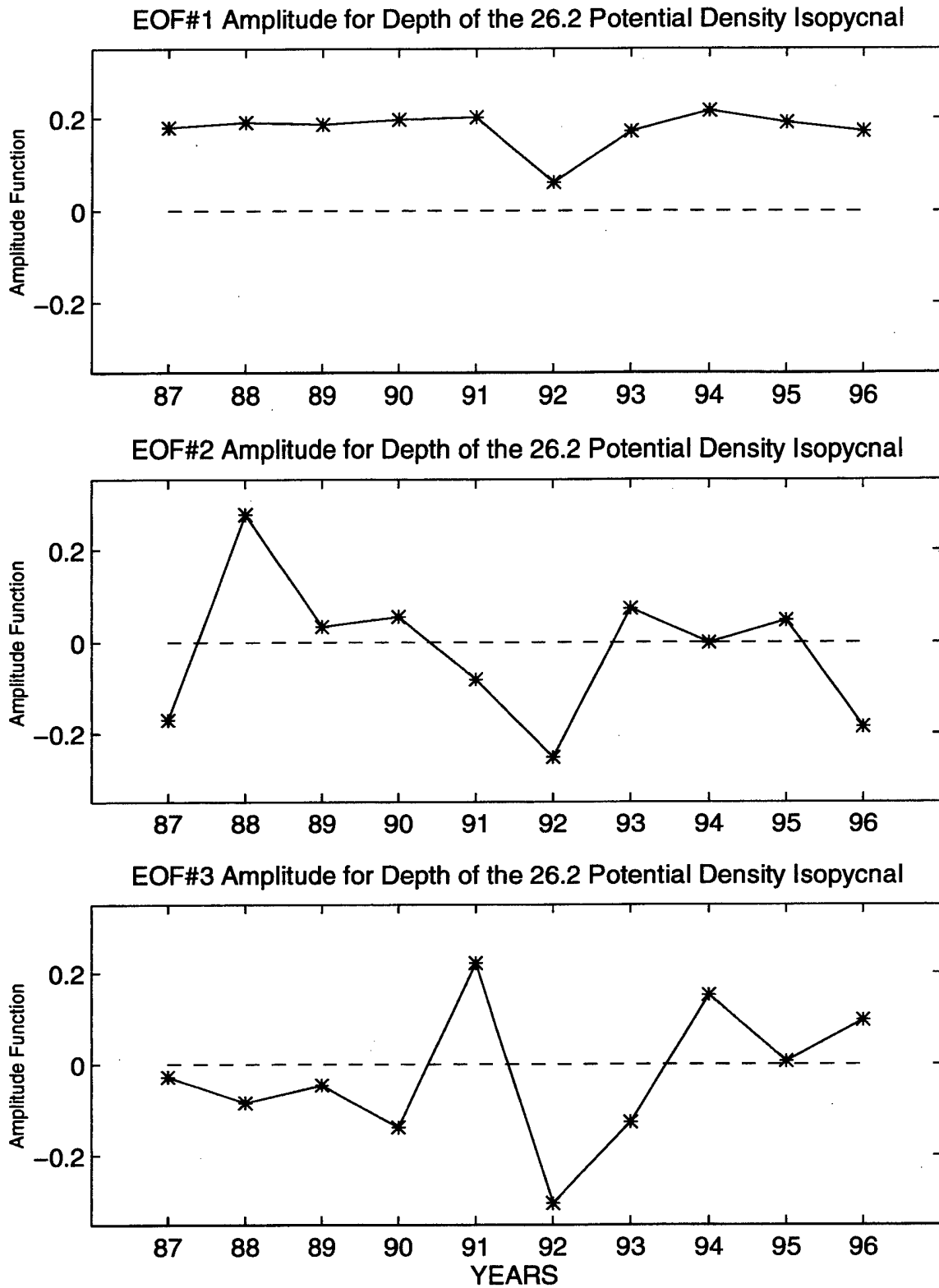
Figure 38. Temporal amplitudes of the first three EOF modes for the 26.2 kg/m 3 isopycnal depth.
