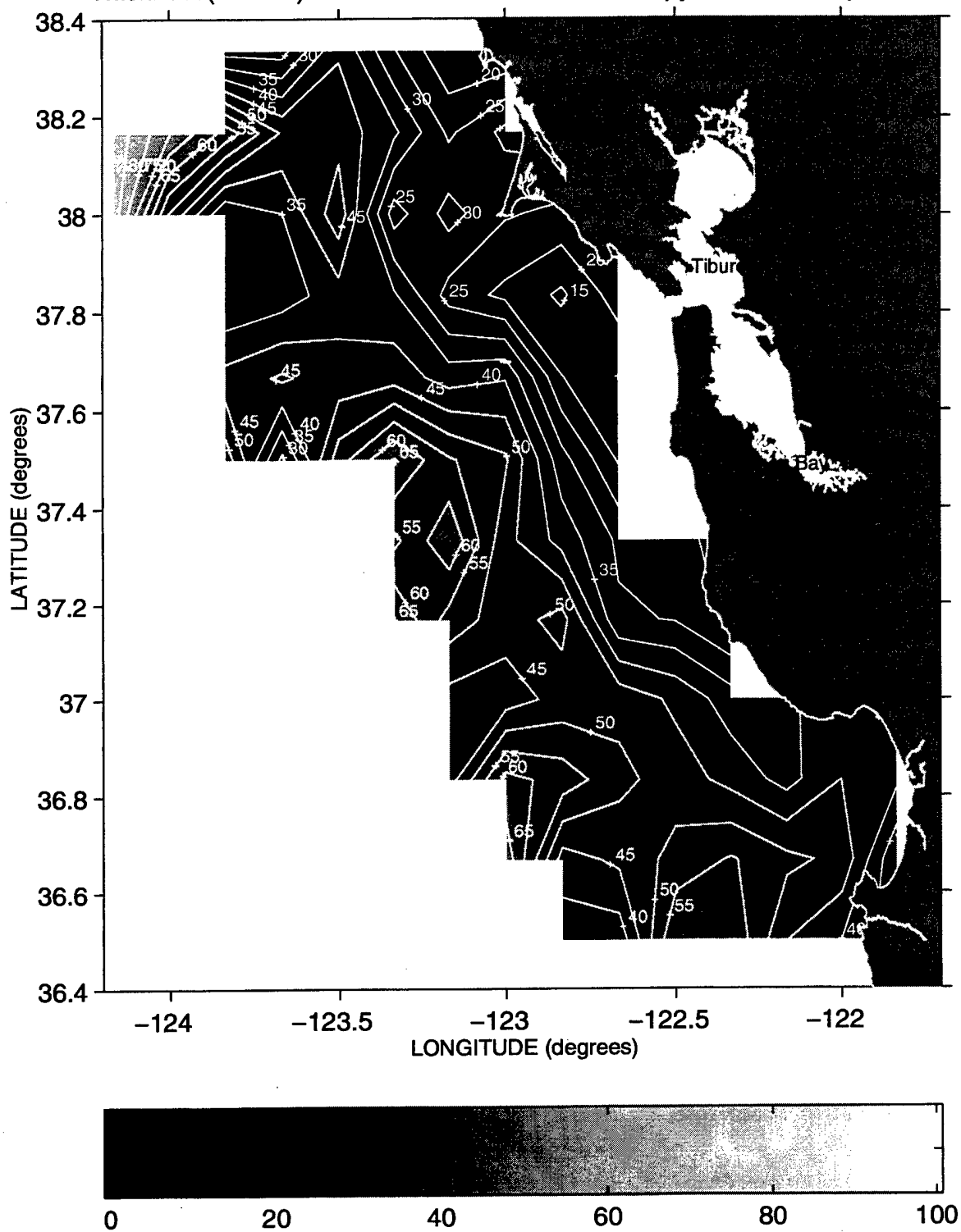
Thickness(meters) between the 25.8 and 26.2 isopycnals ~ Sweep 3, 1991
