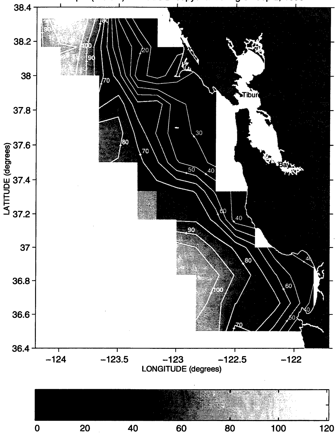
Depth (meters) of the 26.2 Isopycnal during Sweep 2, 1996
