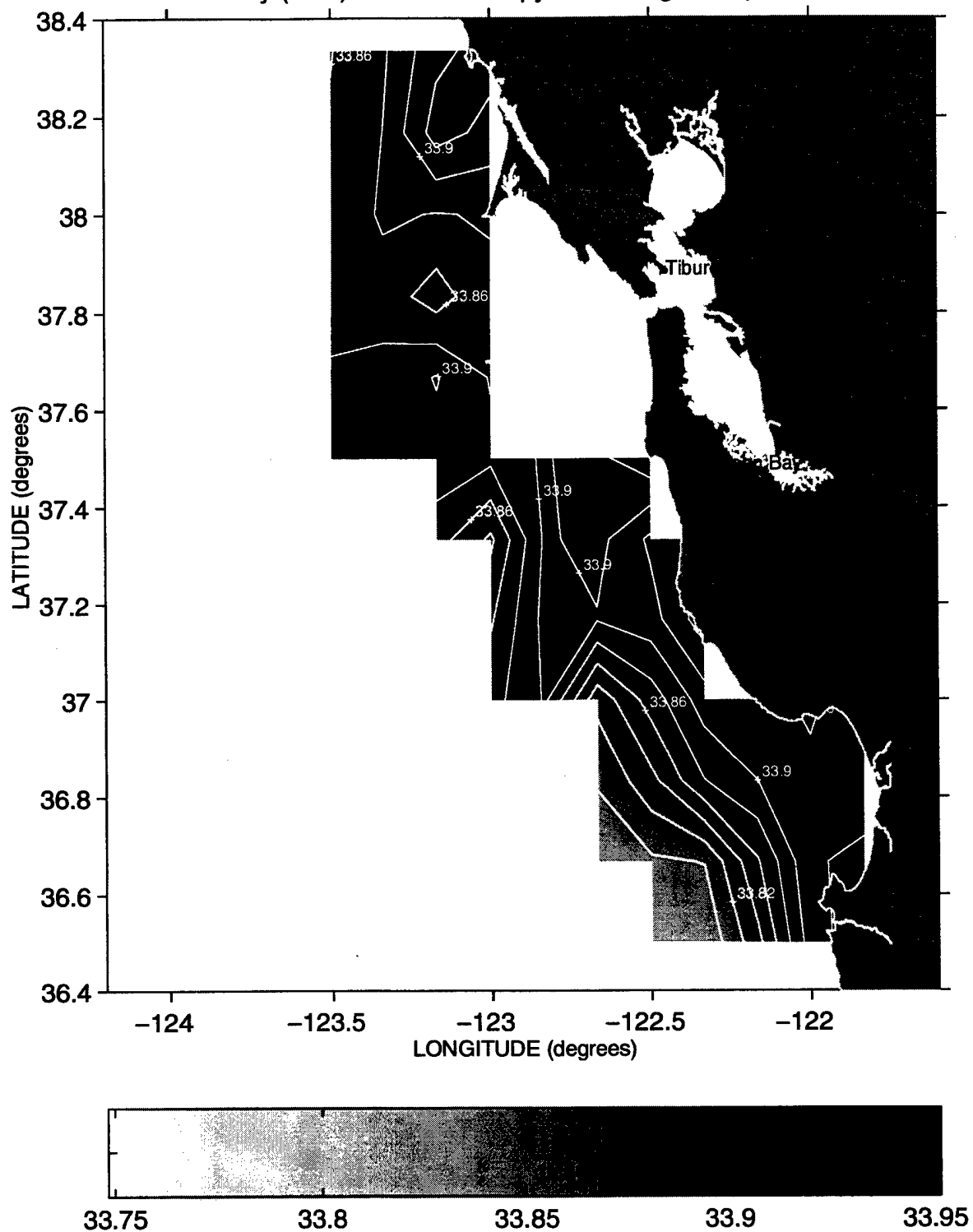
Salinity (PSS) at the 26.2 Isopycnal during Sweep 2, 1987
