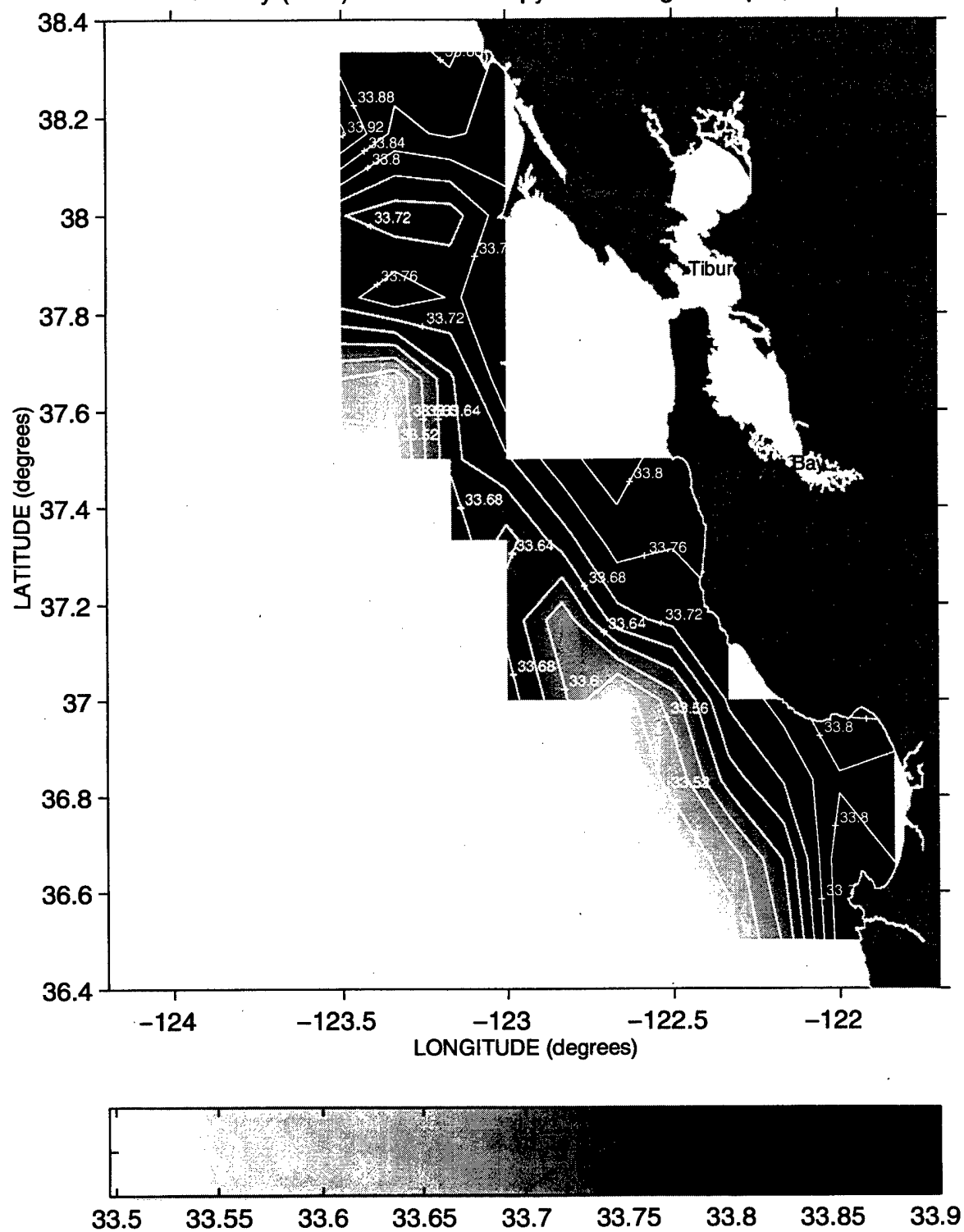
Salinity (PSS) at the 25.8 Isopycnal during Sweep 2, 1987
