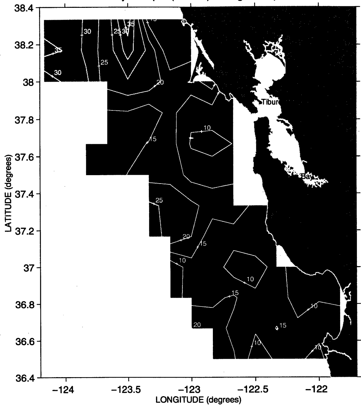
Mixed Layer Depth (meters) during Sweep 2, 1993
