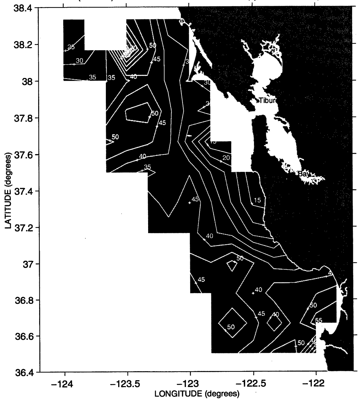
Thickness(meters) between the 25.8 and 26.2 isopycnals ~ Sweep 2, 1995
