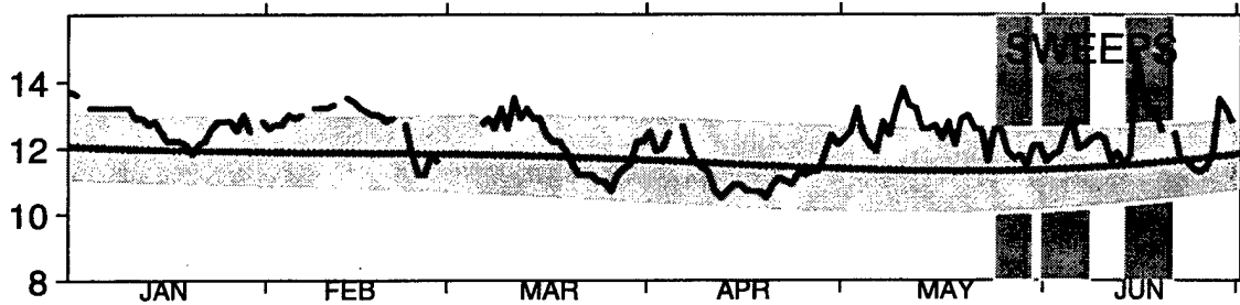
Surface Salinity ~ 1987
