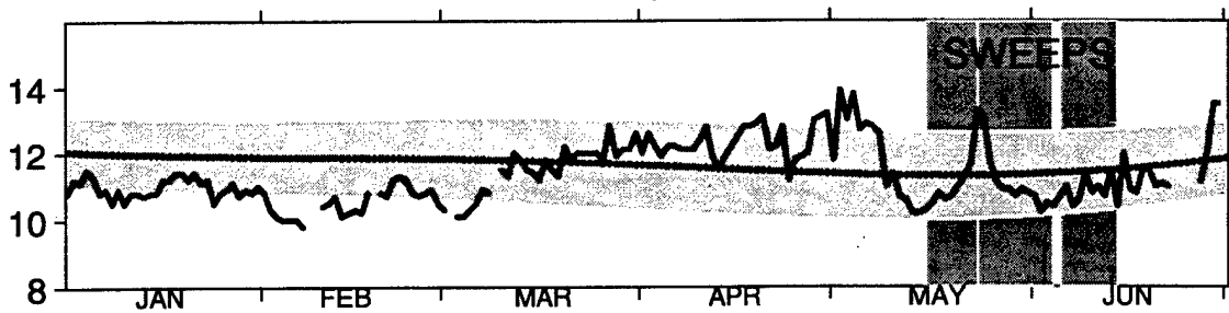
Surface Salinity ~ 1989
