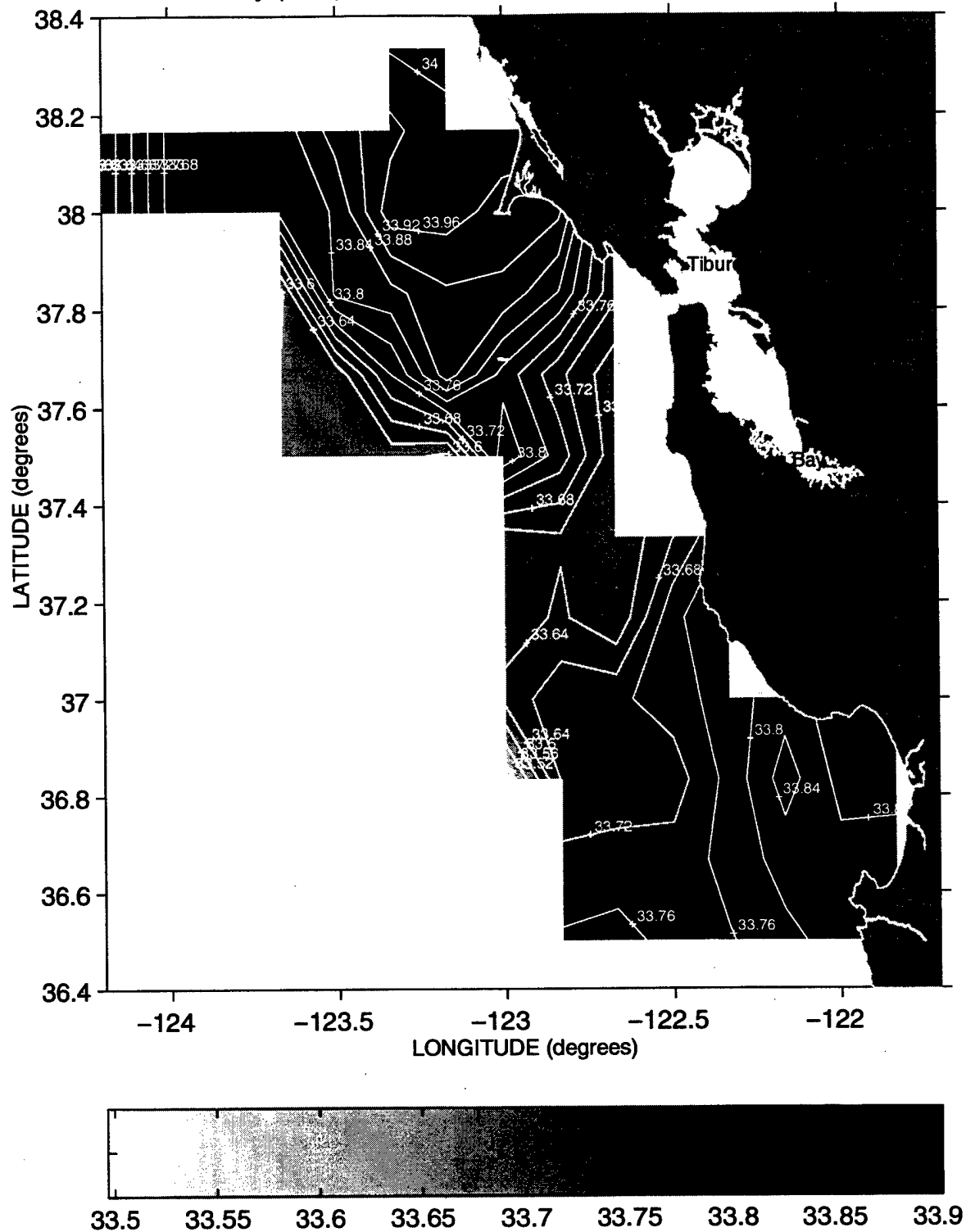
Salinity (PSS) at the 25.8 Isopycnal during Sweep 3, 1996
