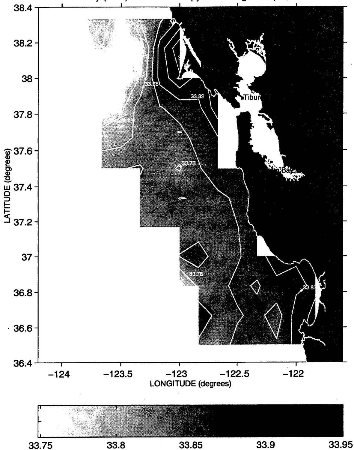
Salinity (PSS) at the 26.2 Isopycnal during Sweep 3, 1995
