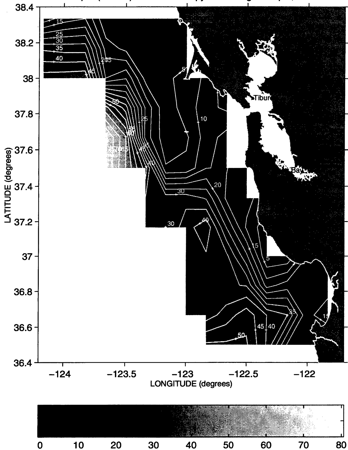
Depth (meters) of the 25.8 Isopycnal during Sweep 2, 1994
