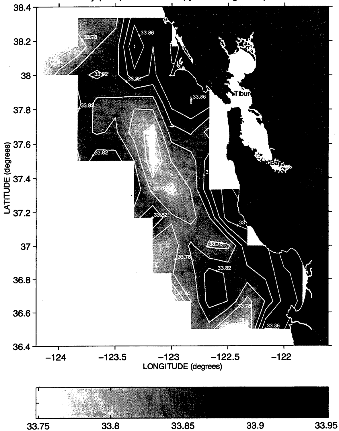
Salinity (PSS) at the 26.2 Isopycnal during Sweep 3, 1991
