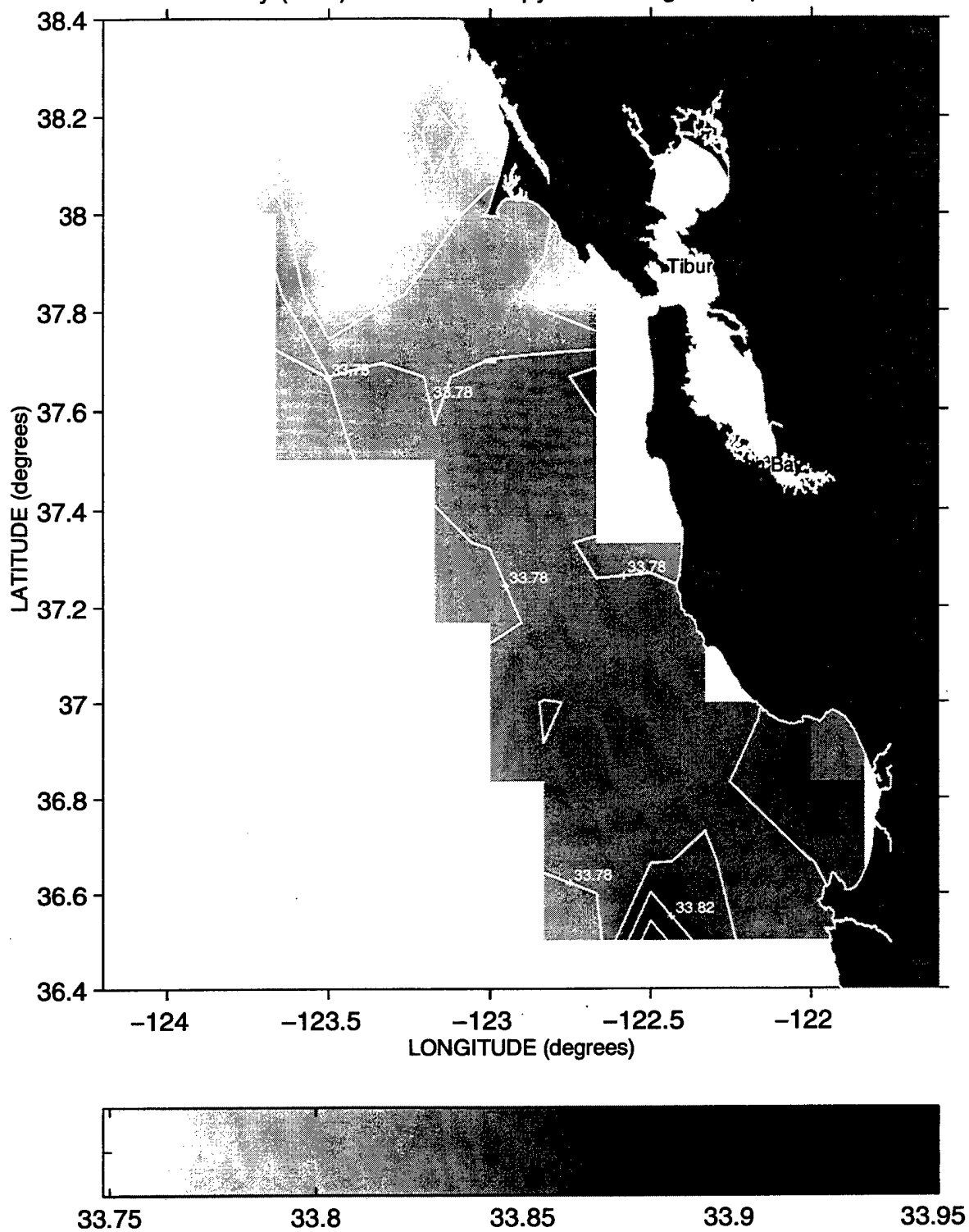
Salinity (PSS) at the 26.2 Isopycnal during Sweep 1, 1995
