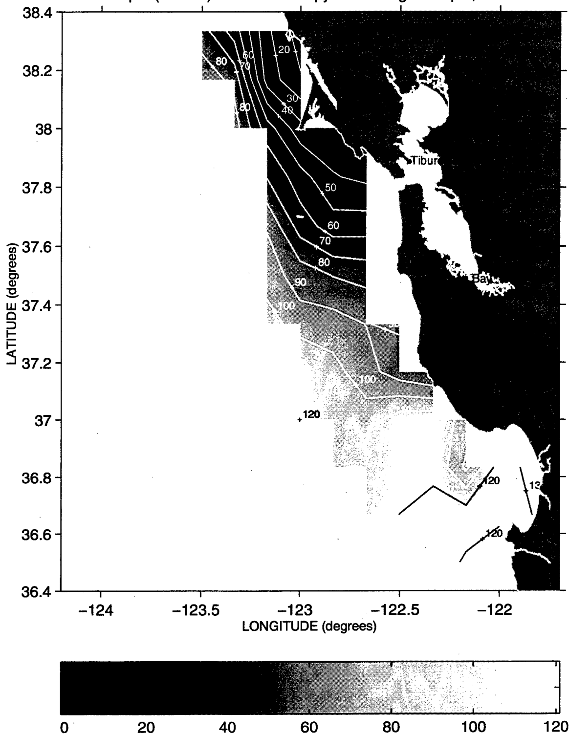
Depth (meters) of the 26.2 Isopycnal during Sweep 1, 1987
