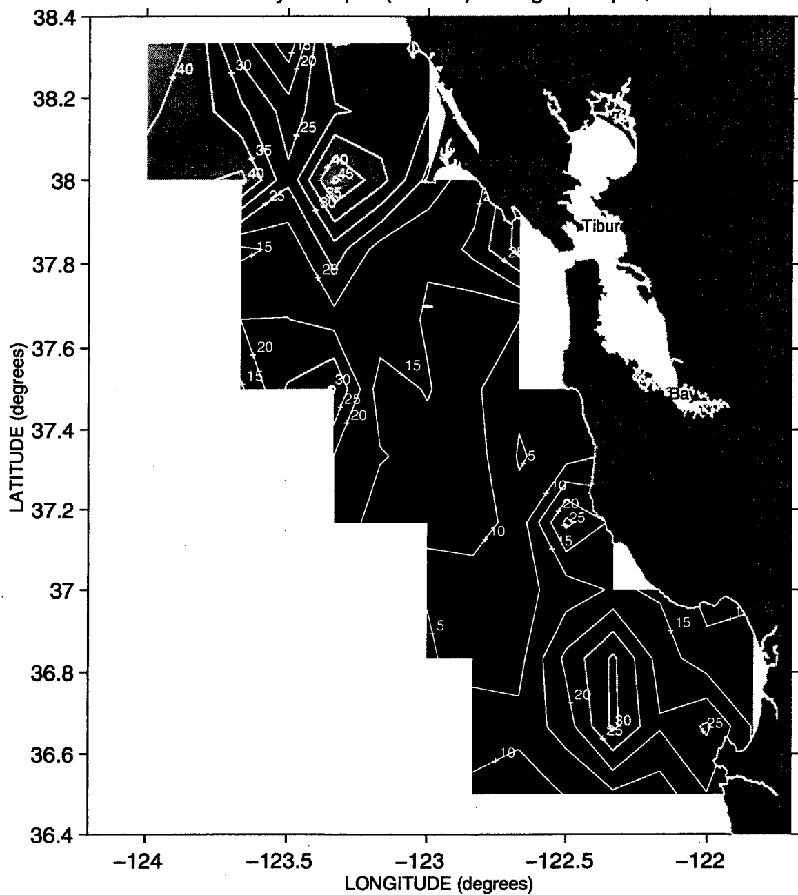
Mixed Layer Depth (meters) during Sweep 3, 1995
