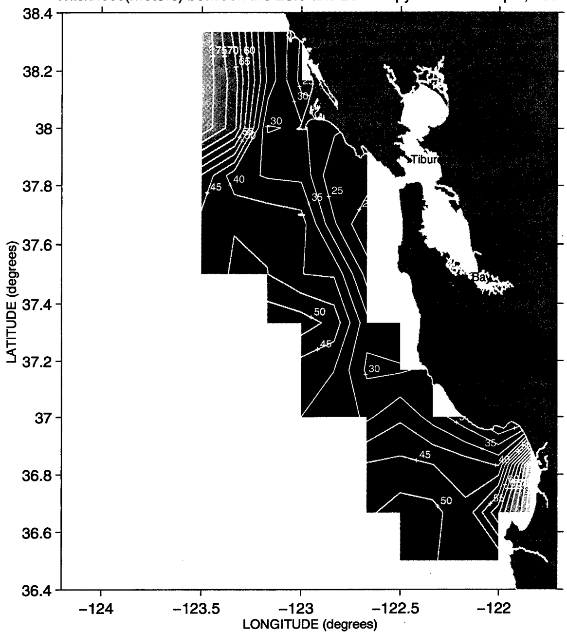
Thickness(meters) between the 25.8 and 26.2 isopycnals ~ Sweep 3, 1987
