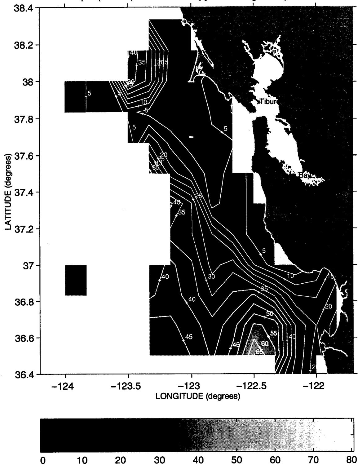
Depth (meters) of the 25.8 Isopycnal during Sweep 2, 1989
