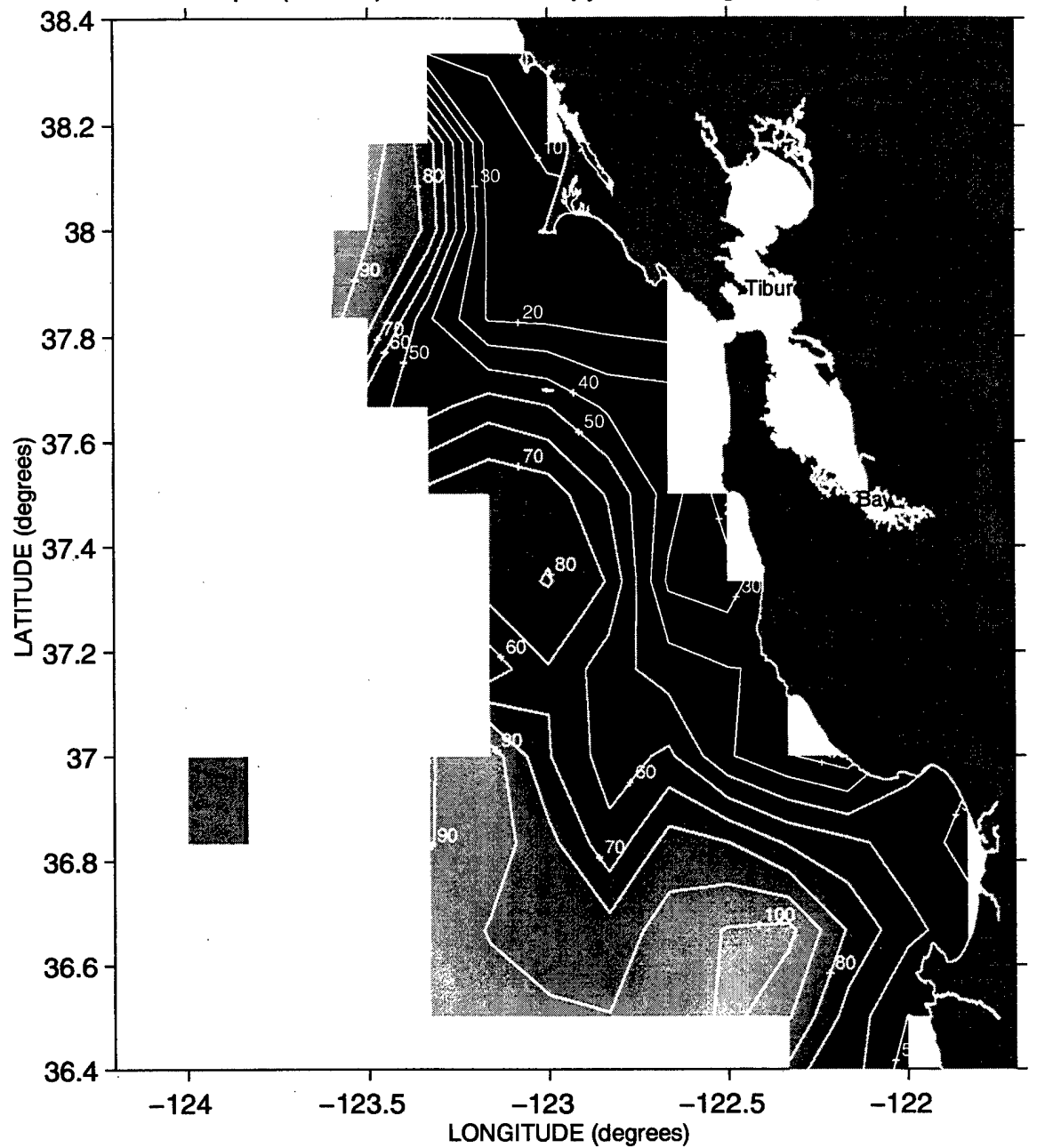
Depth (meters) of the 26.2 Isopycnal during Sweep 2, 1989
