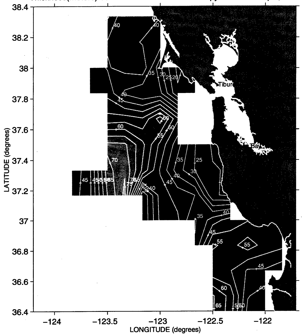
Thickness(meters) between the 25.8 and 26.2 isopycnals ~ Sweep 2, 1990
