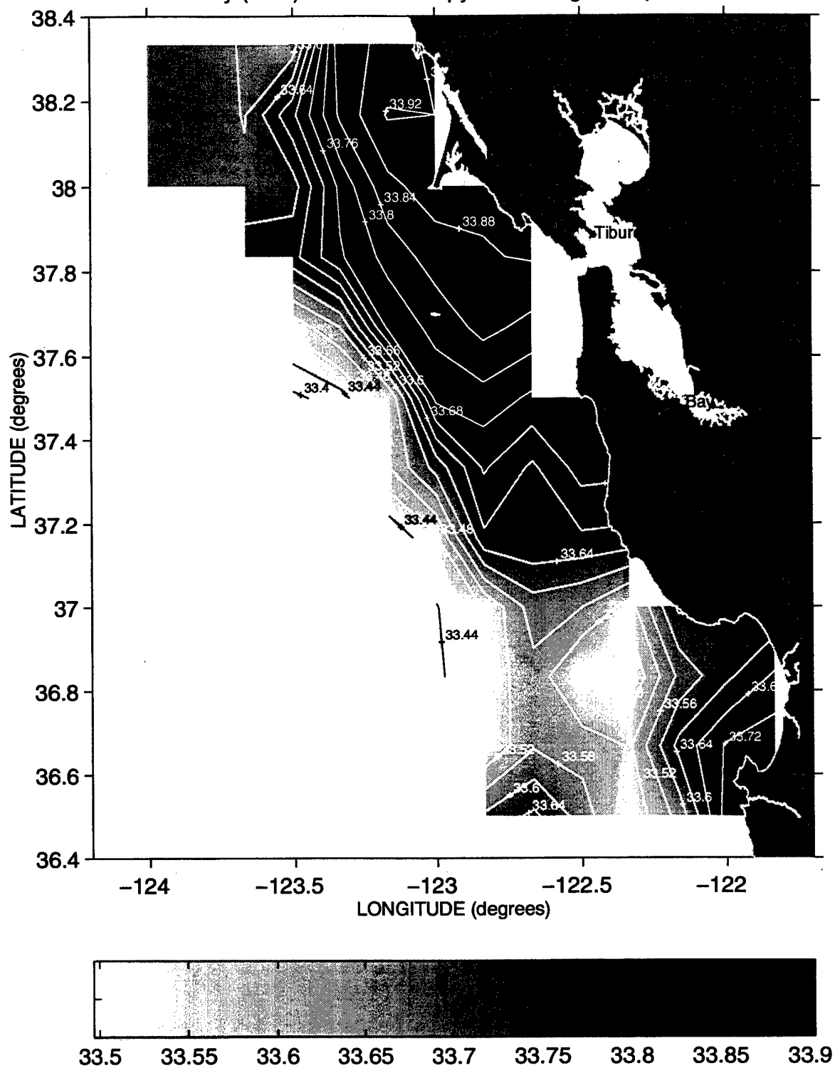
Salinity (PSS) at the 25.8 Isopycnal during Sweep 3, 1994
