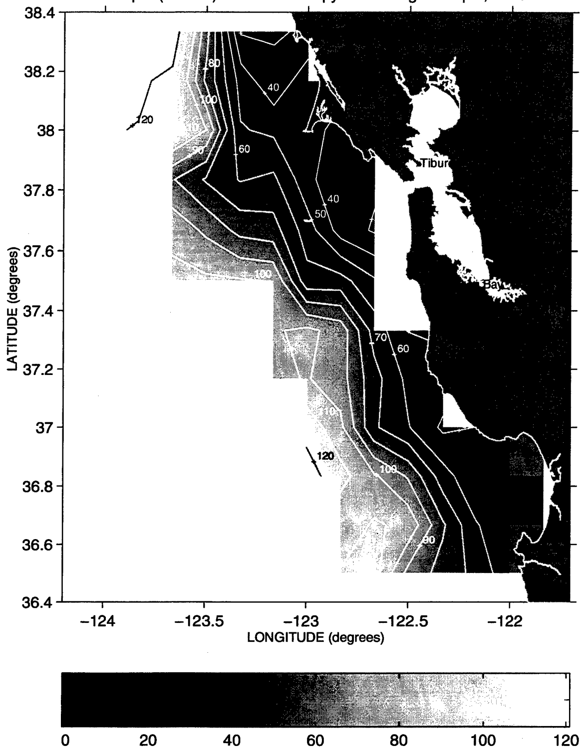
Depth (meters) of the 26.2 Isopycnal during Sweep 1, 1995
