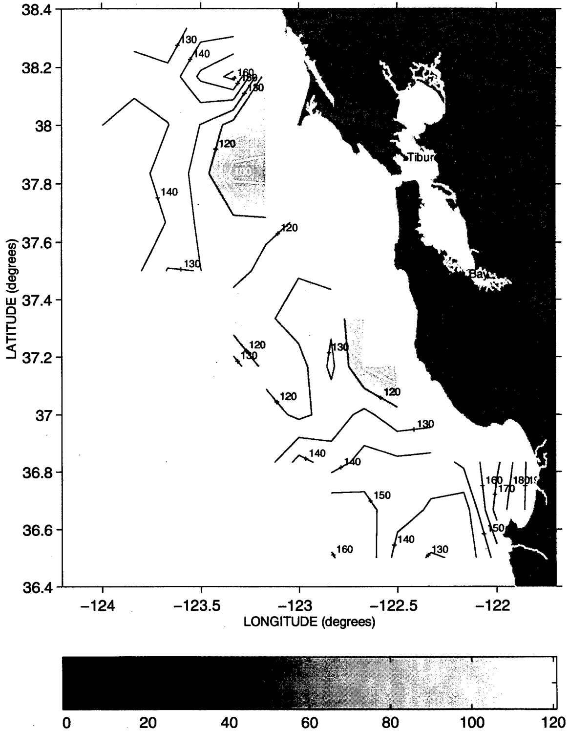
Depth (meters) of the 26.2 Isopycnal during Sweep 1, 1992
