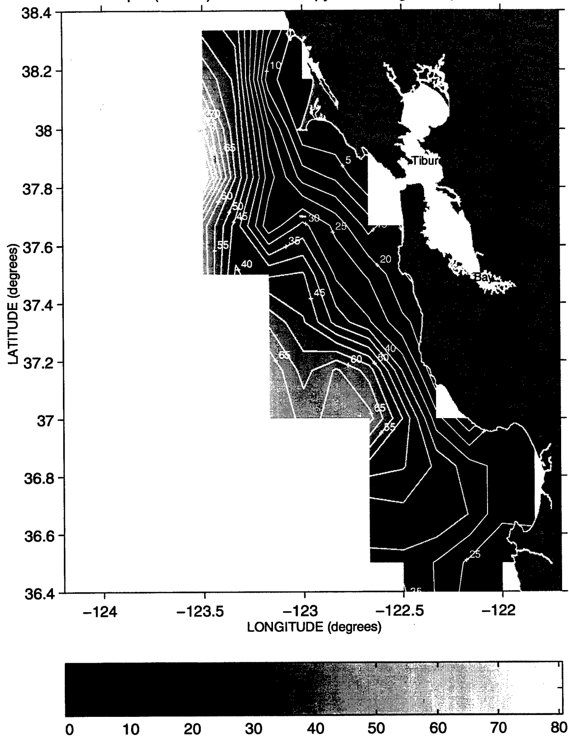
Depth (meters) of the 25.8 Isopycnal during Sweep 3, 1990
