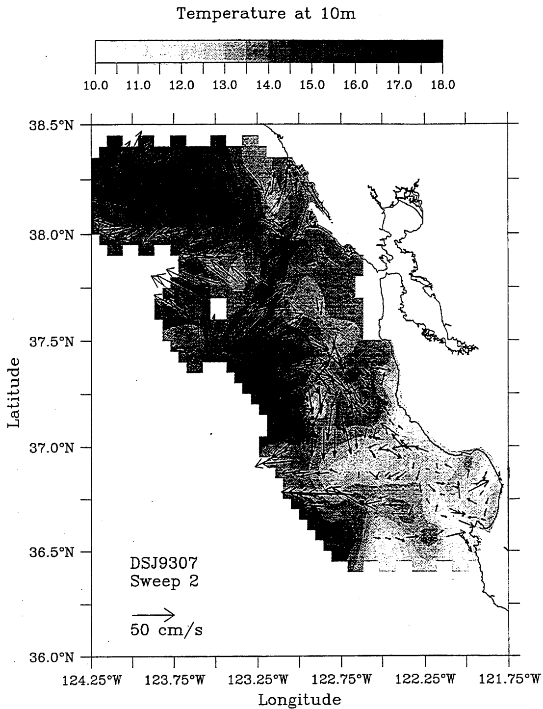
Figure 48. ADCP velocity vectors between 15-30 m and temperature (Celsius) at 10 m during sweep 2, 1993. Adapted from Parker (1996).
