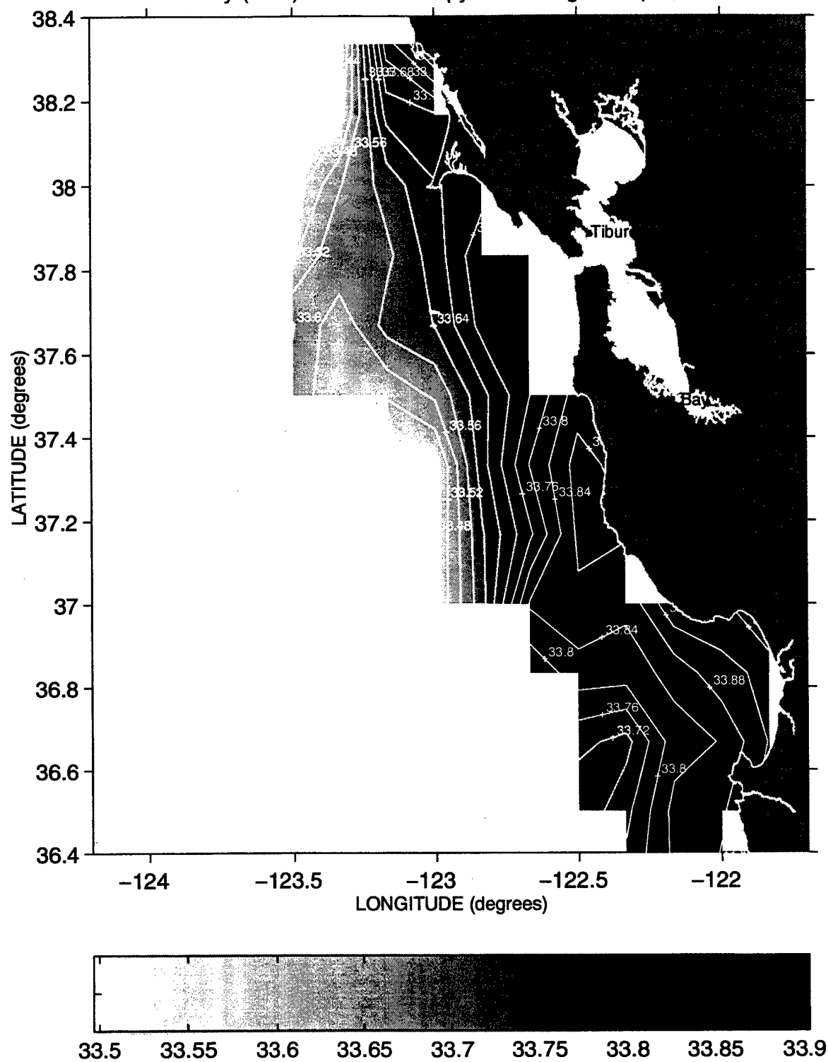
Salinity (PSS) at the 25.8 Isopycnal during Sweep 3, 1988
