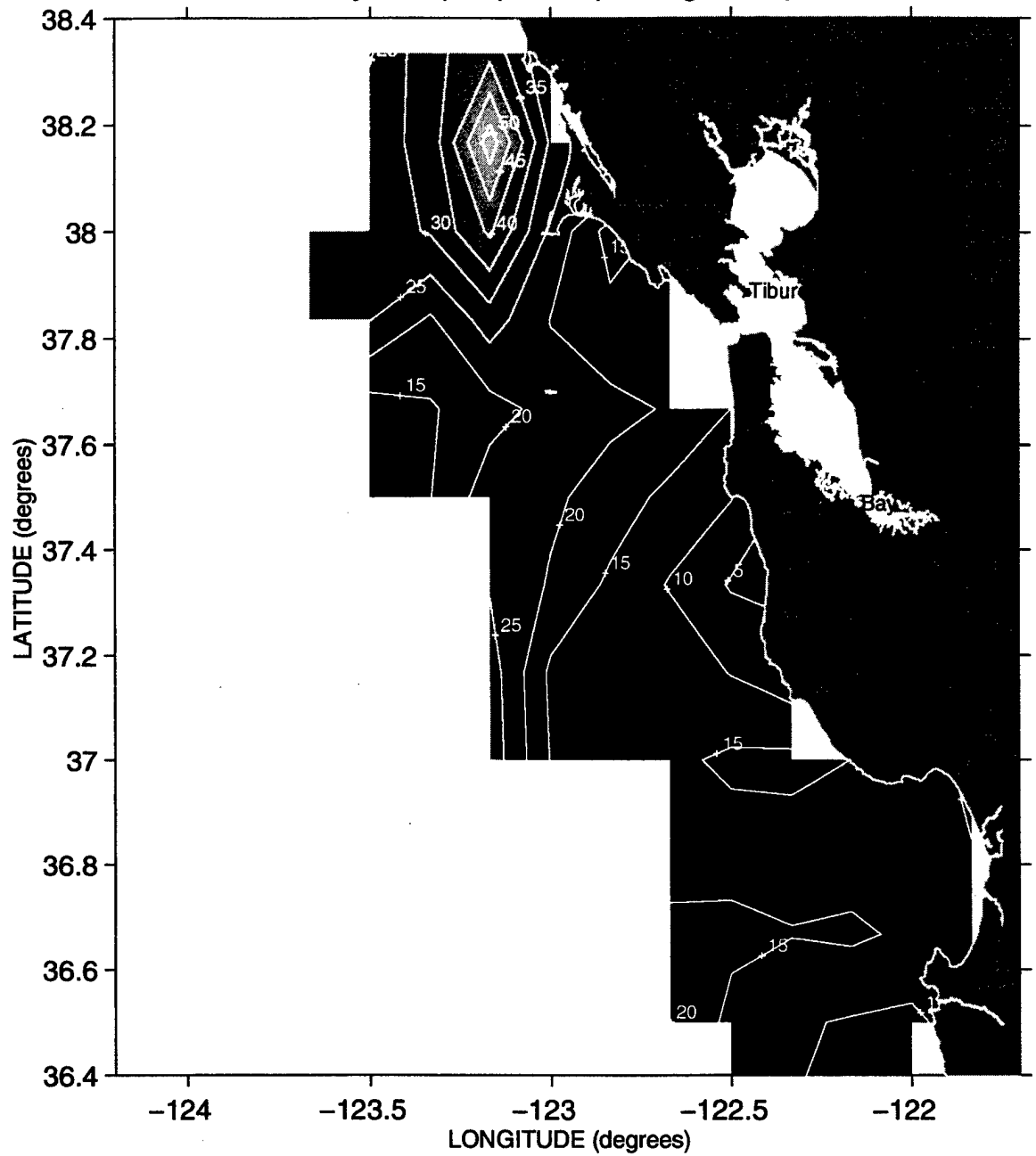
Mixed Layer Depth (meters) during Sweep 3, 1990
