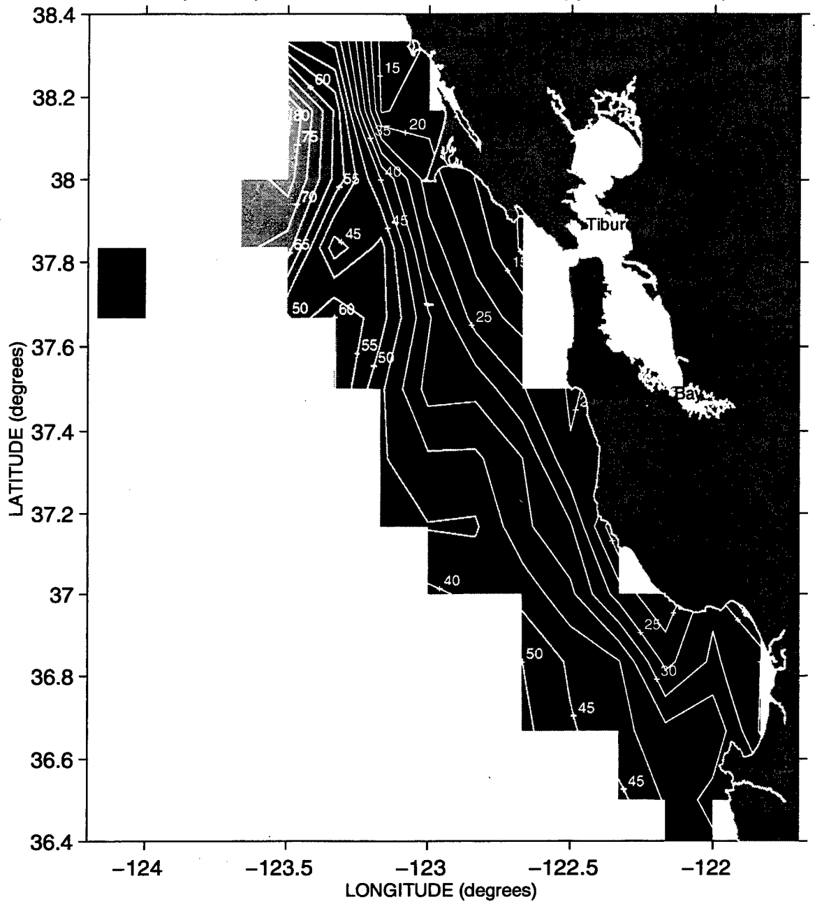
Thickness(meters) between the 25.8 and 26.2 isopycnals ~ Sweep 3, 1989
