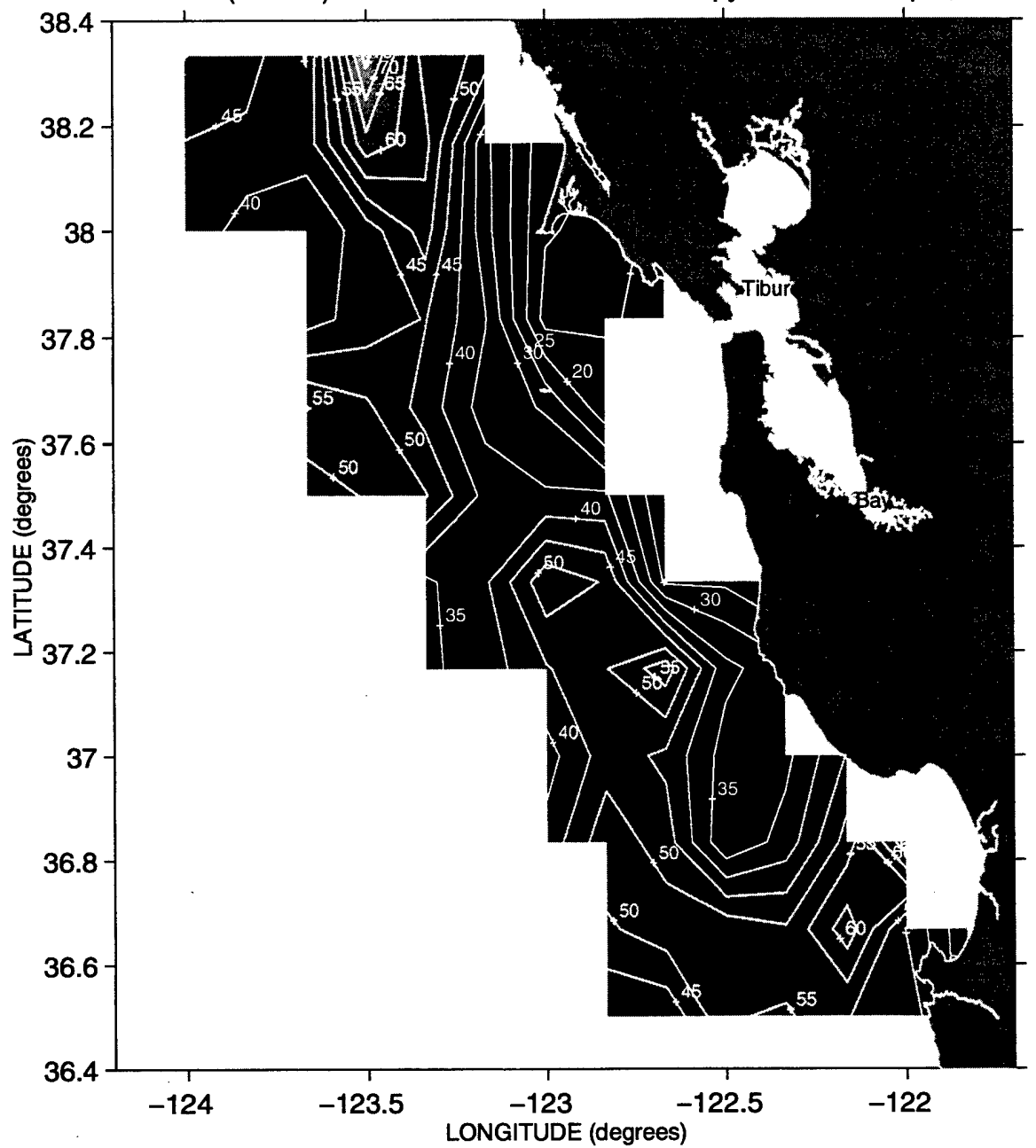
Thickness(meters) between the 25.8 and 26.2 isopycnals ~ Sweep 1, 1996
