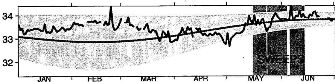
Sea Surface Temperature ~ 1990
