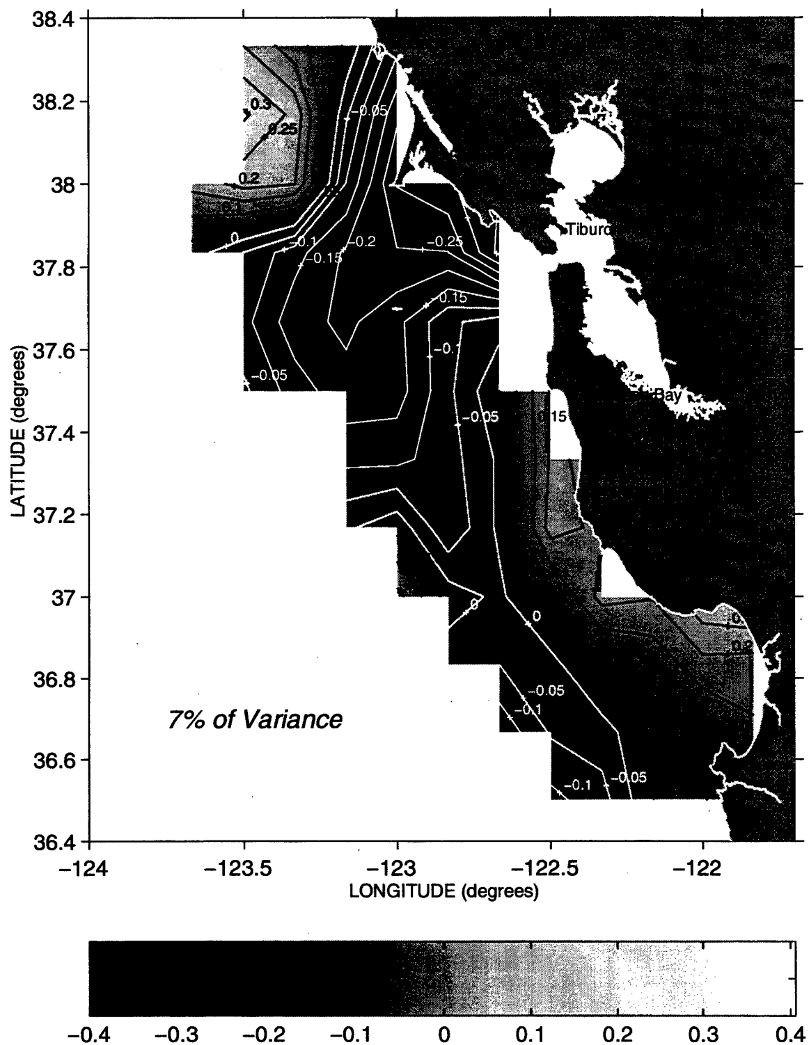
Figure 43. Zscore pattern of the third EOF for salinity on the 25.8 \text{ kg/m}^3 isopycnal. Contour interval is 0.05.
