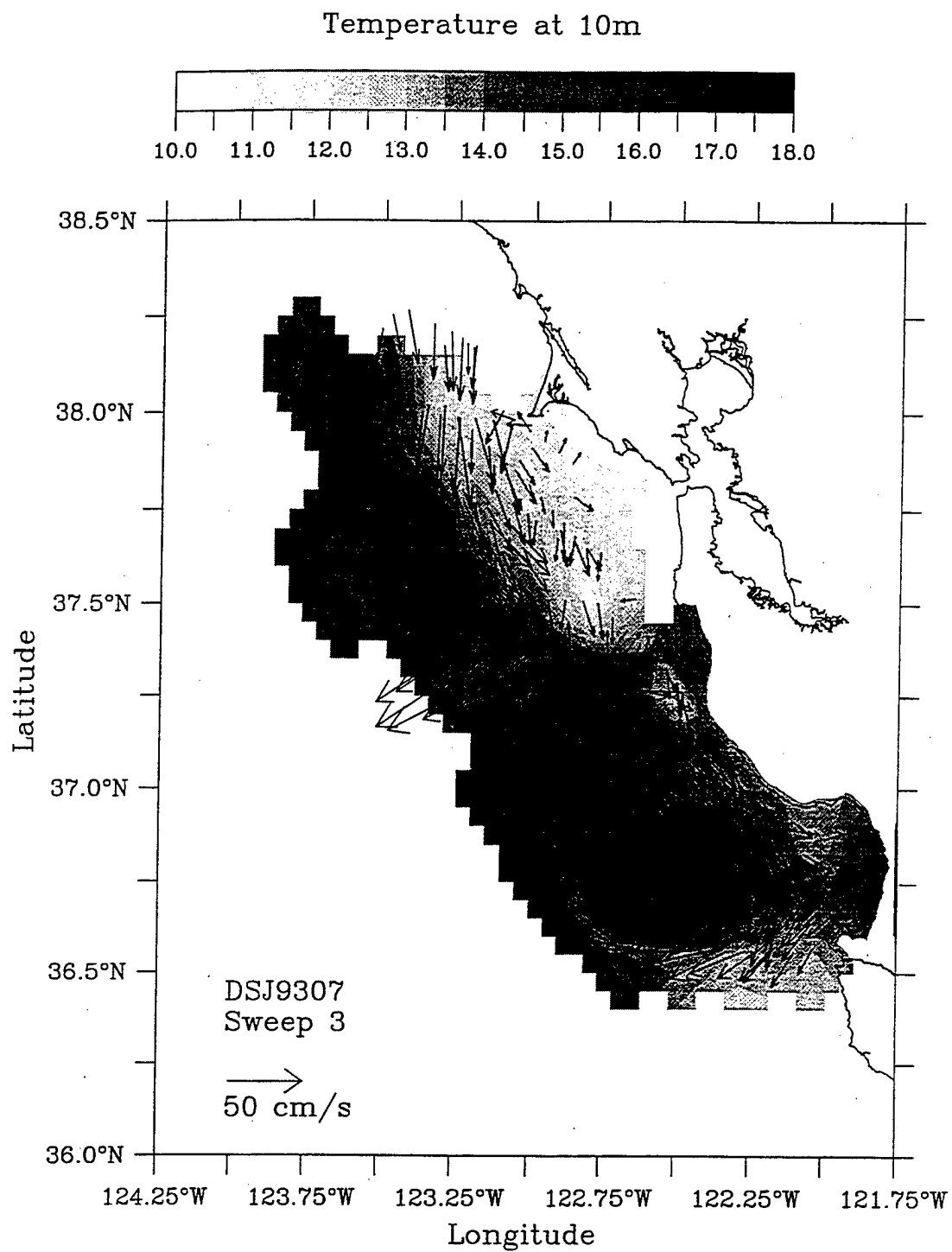
Figure 49. ADCP velocity vectors between 15-30 m and temperature (Celsius) at 10 m during sweep 3, 1993. Adapted from Parker (1996).
