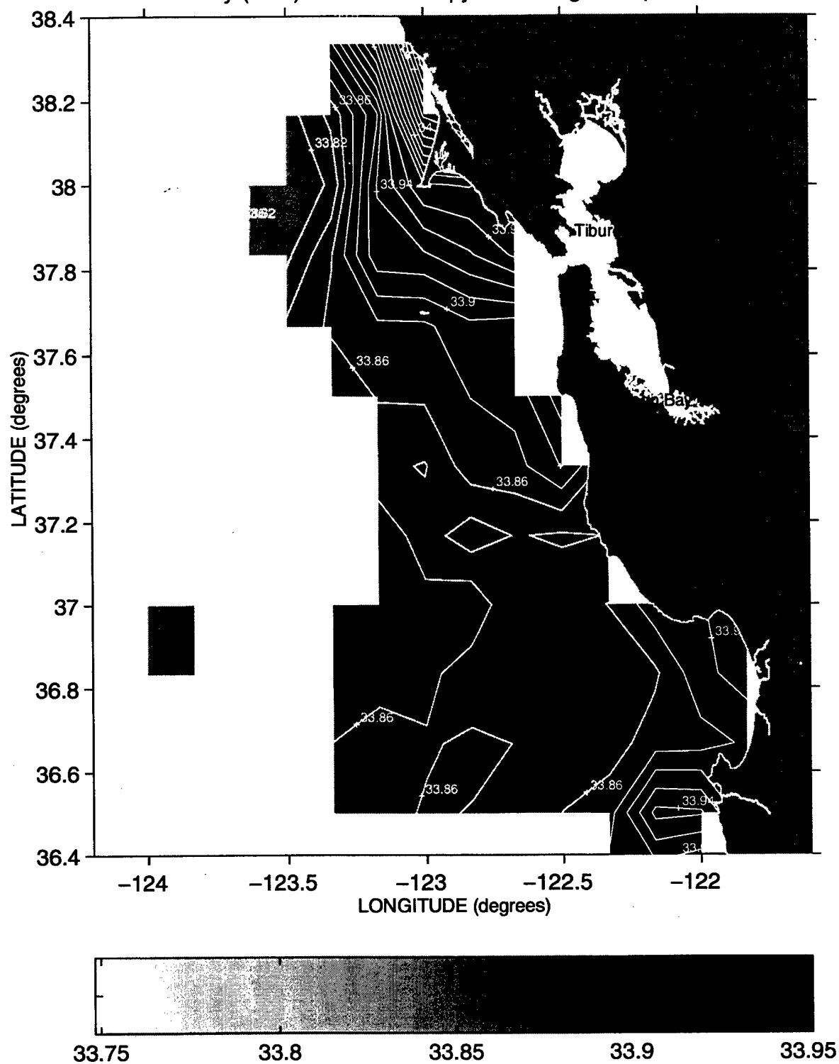
Salinity (PSS) at the 26.2 Isopycnal during Sweep 2, 1989
