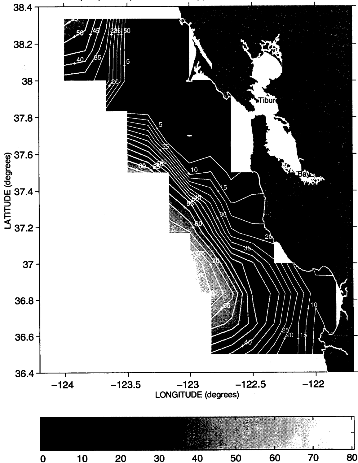
Depth (meters) of the 25.8 Isopycnal during Sweep 3, 1994
