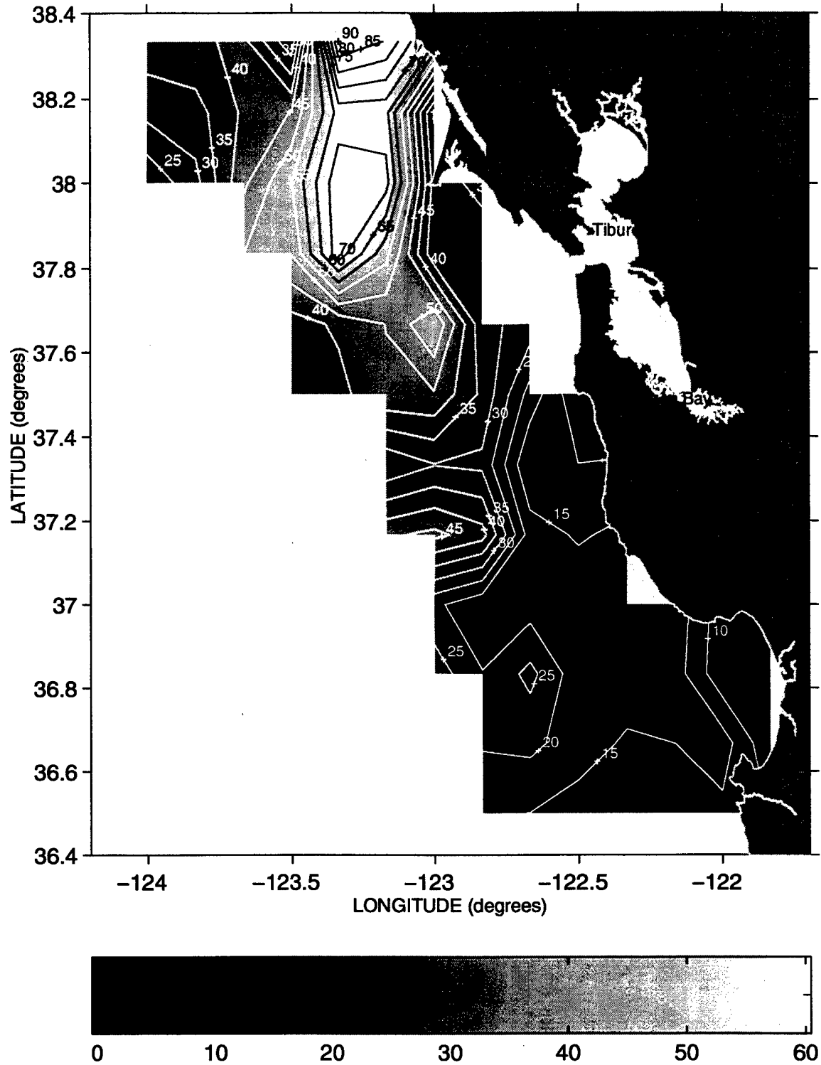
Mixed Layer Depth (meters) during Sweep 3, 1994
