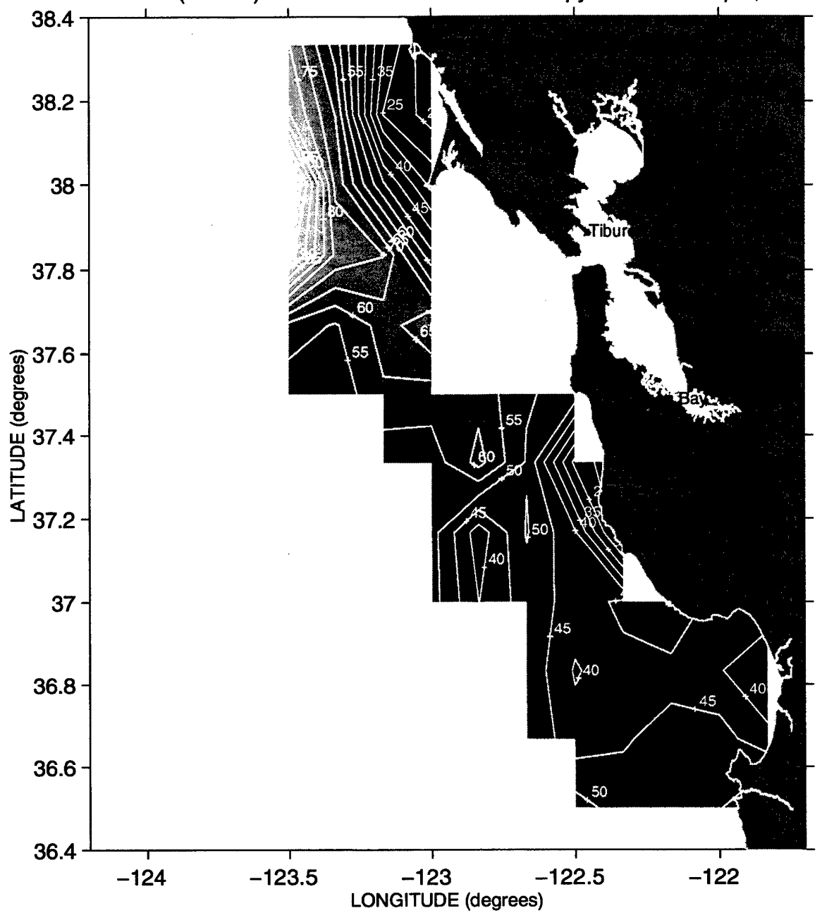
Thickness(meters) between the 25.8 and 26.2 isopycnals ~ Sweep 2, 1987
