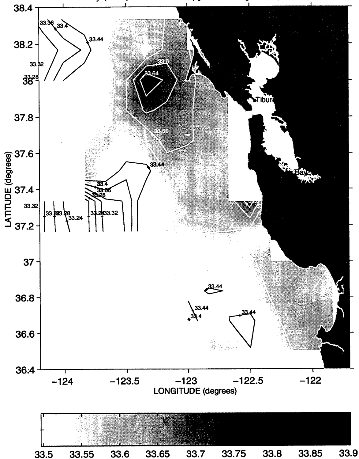
Salinity (PSS) at the 25.8 Isopycnal during Sweep 3, 1992
