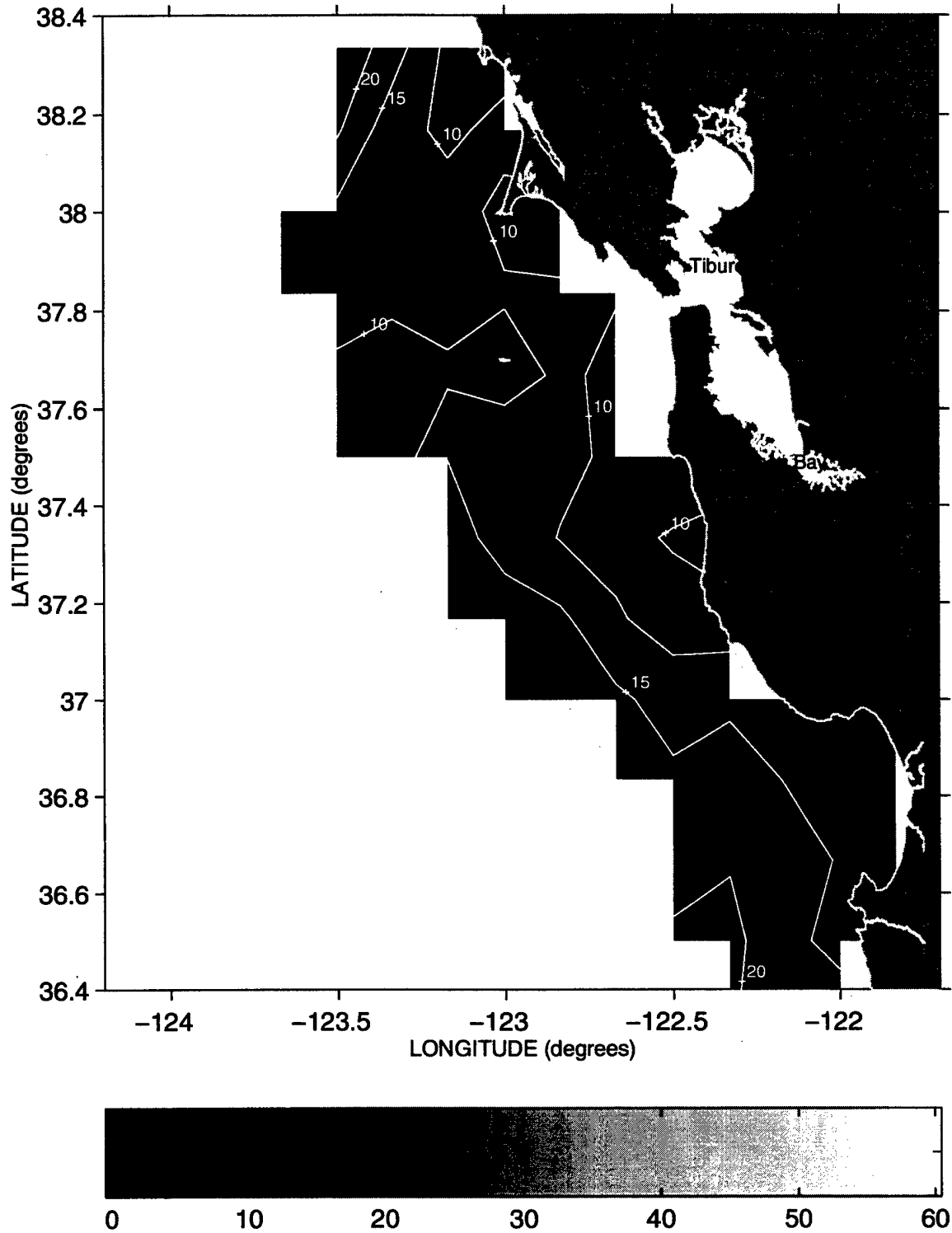
Mixed Layer Depth (meters) during Sweep 3, 1988
