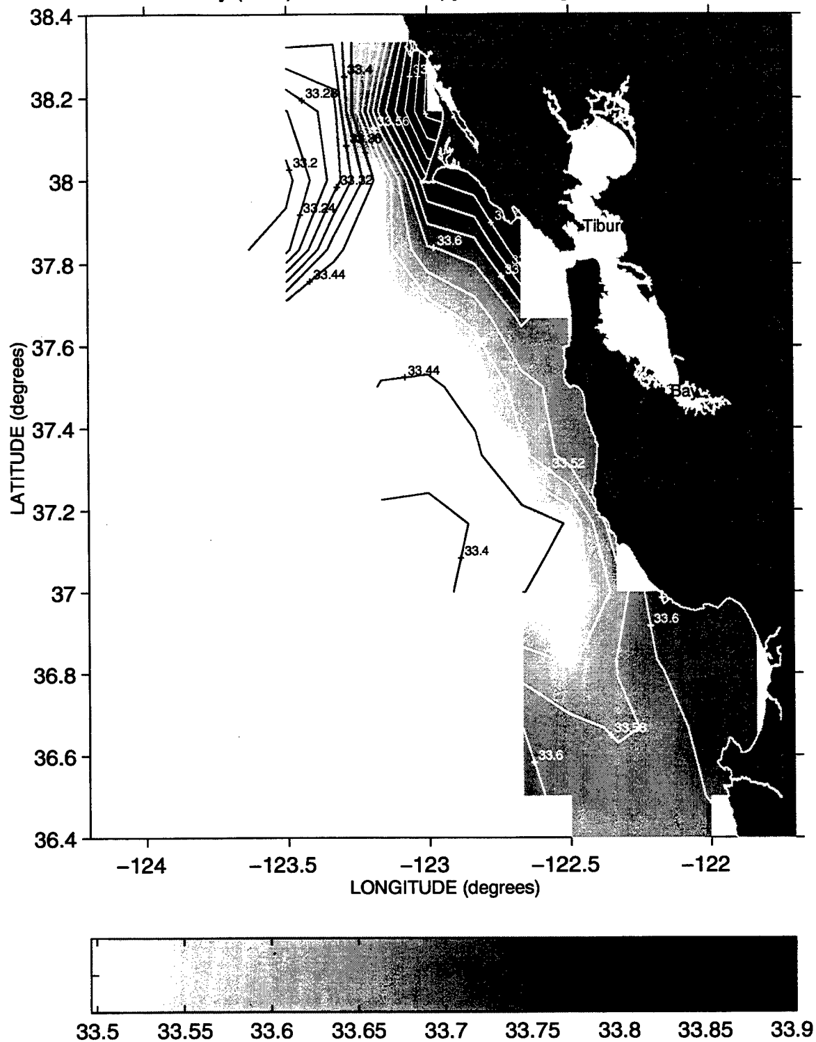
Salinity (PSS) at the 25.8 Isopycnal during Sweep 3, 1990
