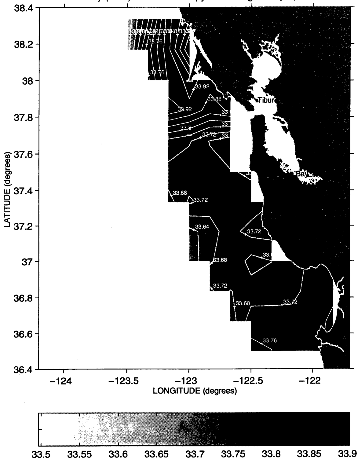
Salinity (PSS) at the 25.8 Isopycnal during Sweep 1, 1987
