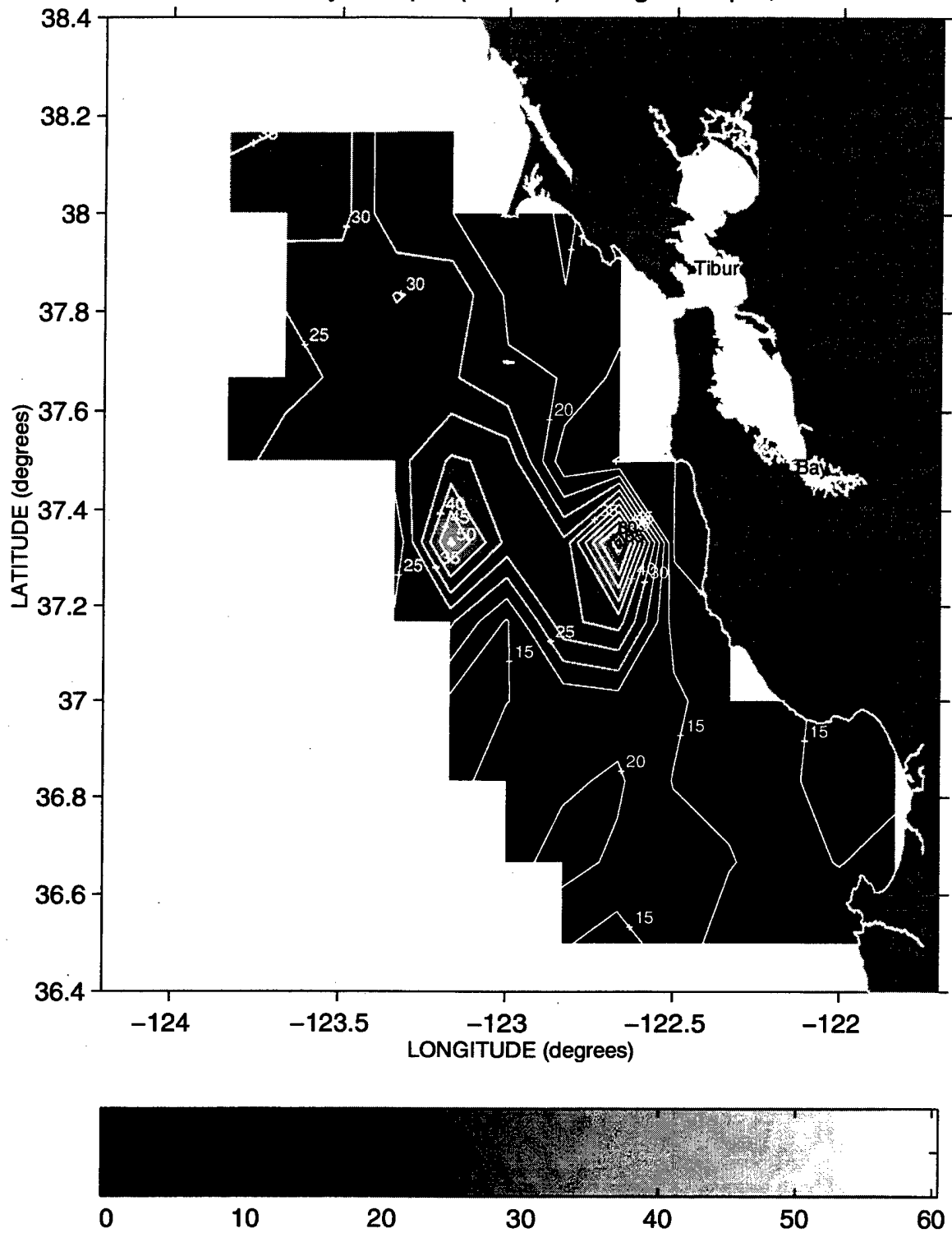
Mixed Layer Depth (meters) during Sweep 3, 1993
