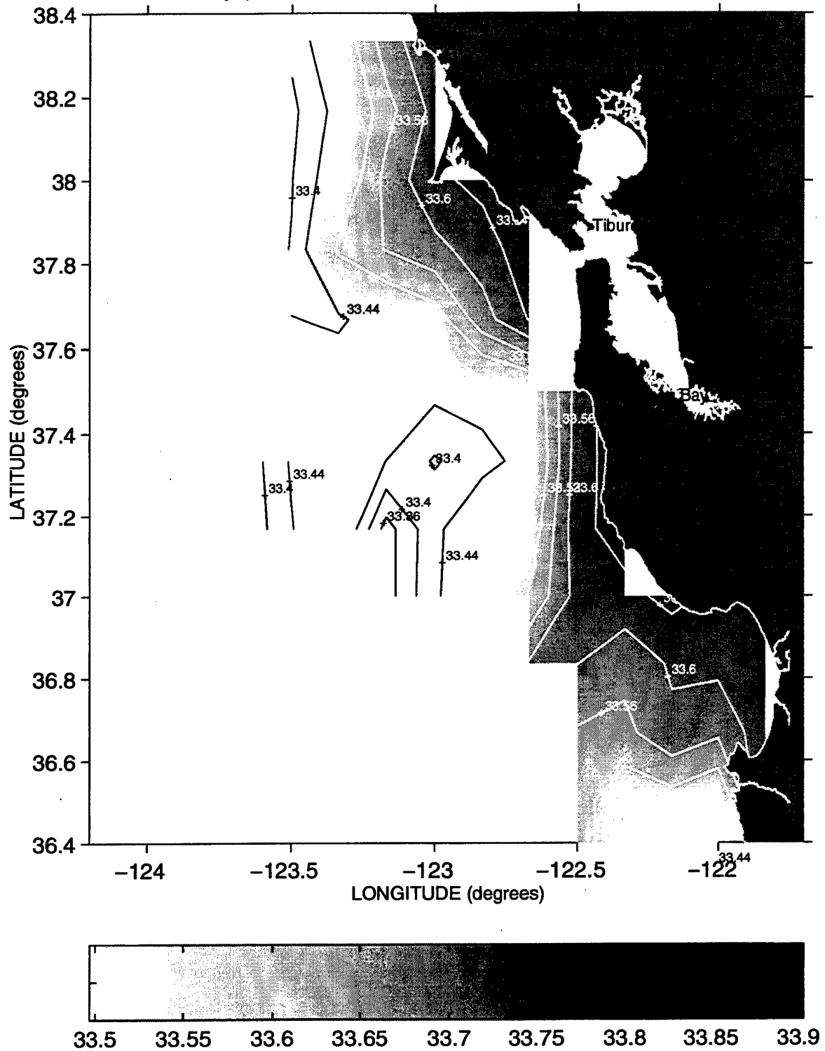
Salinity (PSS) at the 25.8 Isopycnal during Sweep 2, 1990
