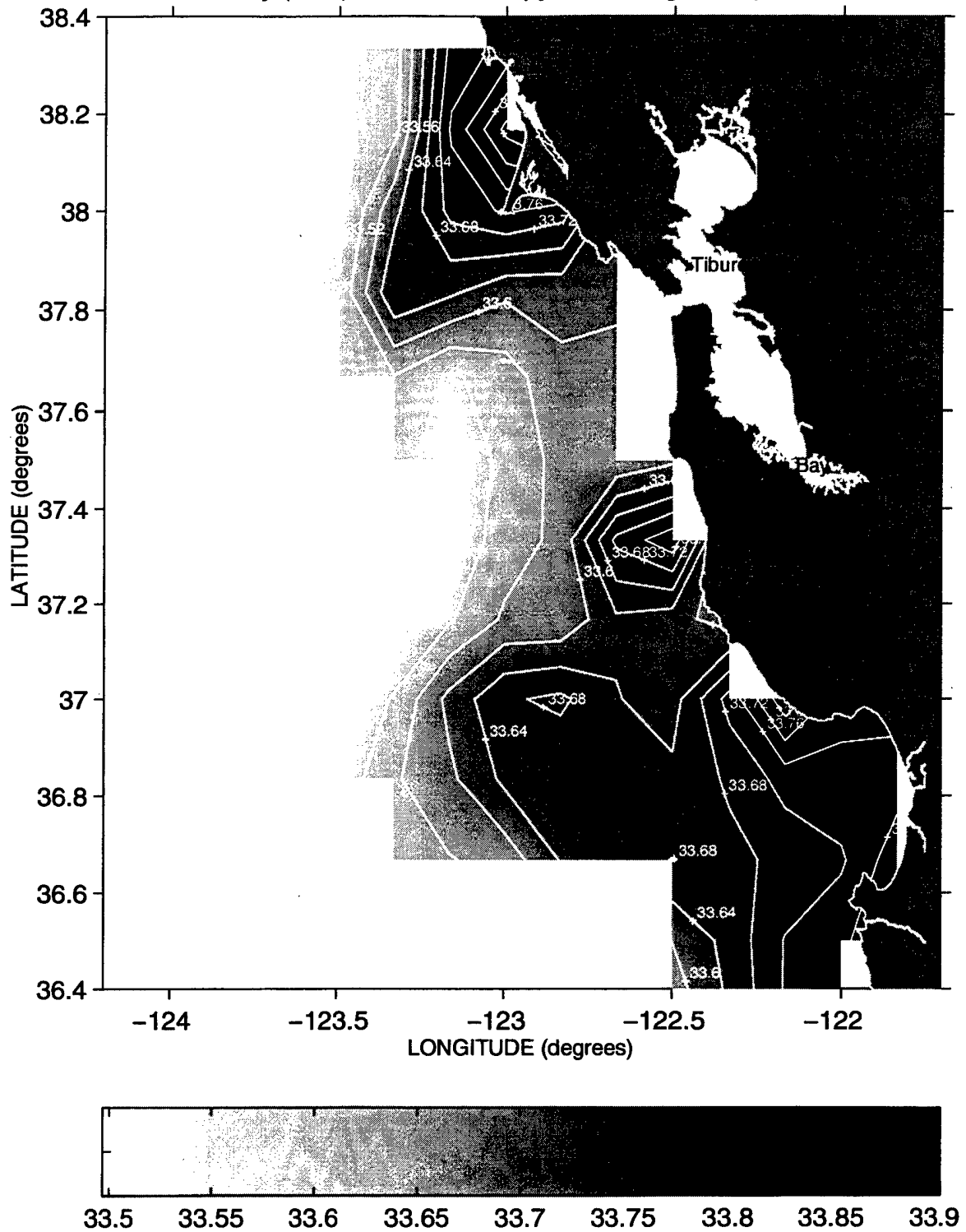
Salinity (PSS) at the 25.8 Isopycnal during Sweep 1, 1989
