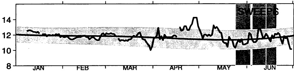
Surface Salinity ~ 1988
