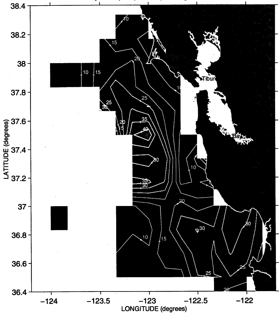
Mixed Layer Depth (meters) during Sweep 2, 1989
