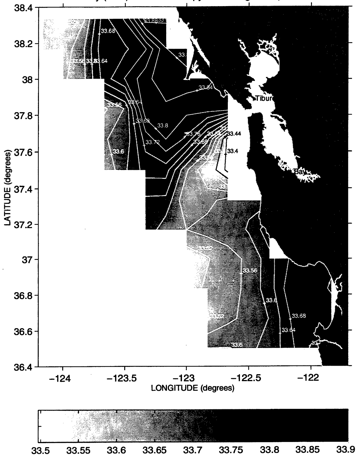
Salinity (PSS) at the 25.8 Isopycnal during Sweep 2, 1996
