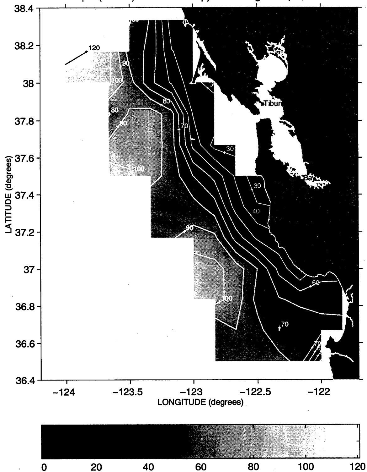
Depth (meters) of the 26.2 Isopycnal during Sweep 2, 1995
