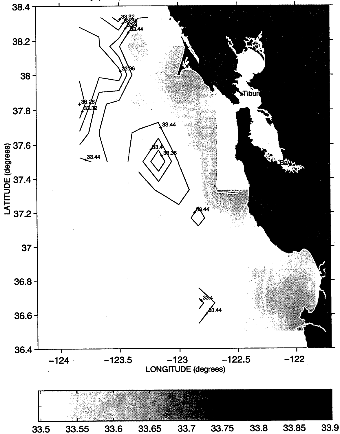
Salinity (PSS) at the 25.8 Isopycnal during Sweep 1, 1992
