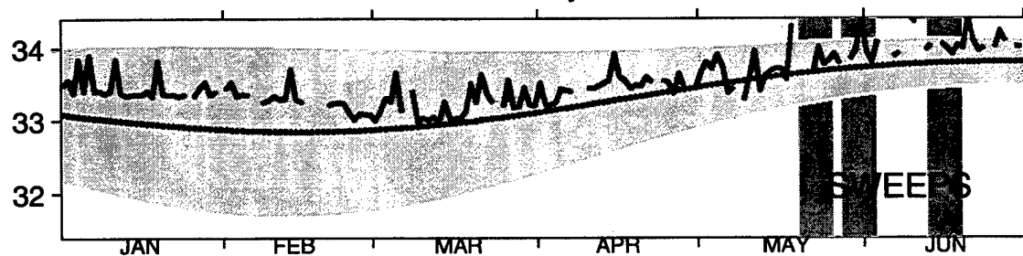
Surface Salinity ~ 1994
