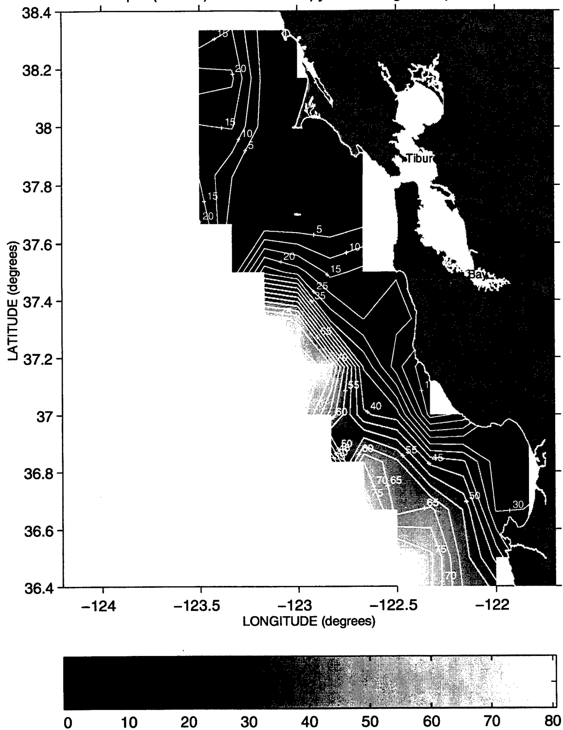
Depth (meters) of the 25.8 Isopycnal during Sweep 1, 1990
