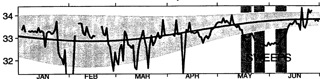
Sea Surface Temperature ~ 1994
