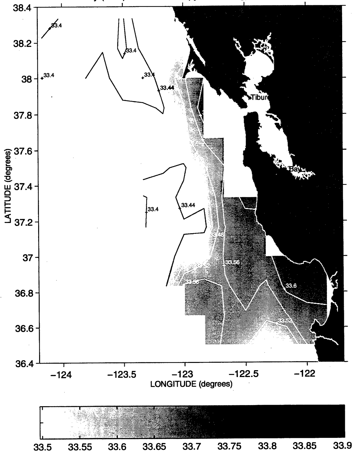
Salinity (PSS) at the 25.8 Isopycnal during Sweep 2, 1993
