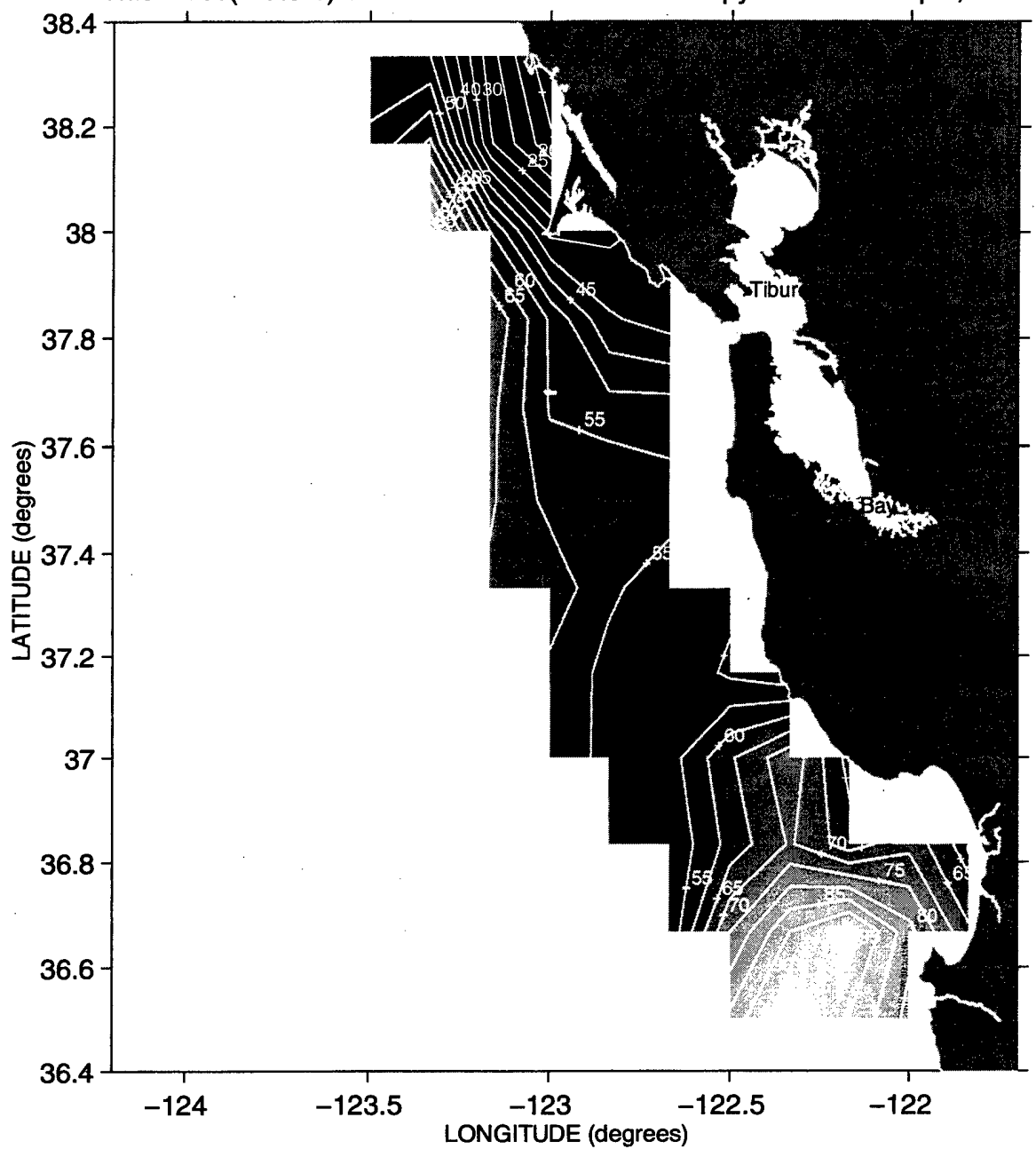
Thickness(meters) between the 25.8 and 26.2 isopycnals ~ Sweep 1, 1987
