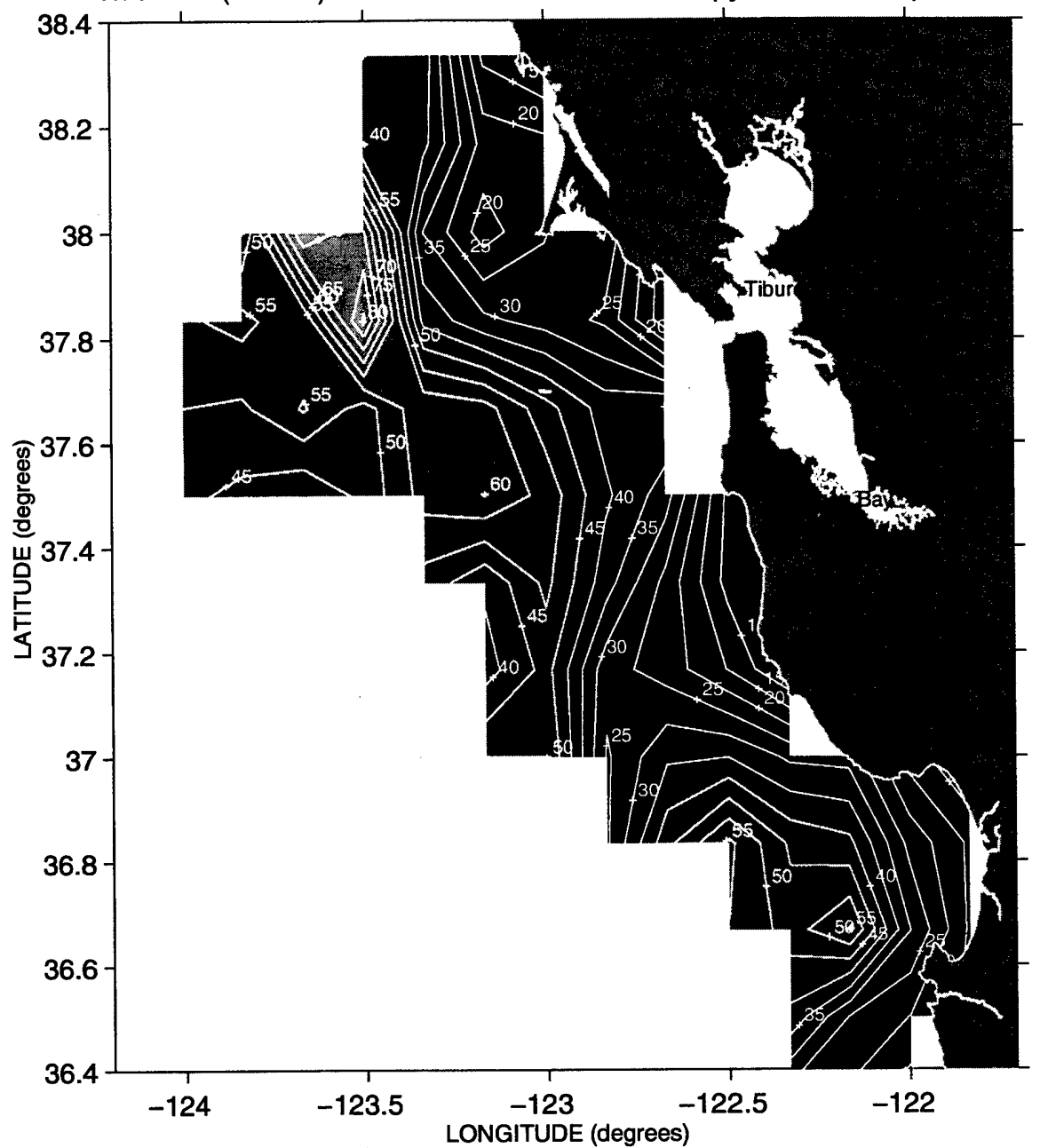
Thickness(meters) between the 25.8 and 26.2 isopycnals ~ Sweep 1, 1988
