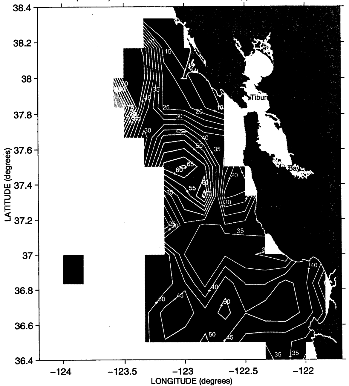
Thickness(meters) between the 25.8 and 26.2 isopycnals ~ Sweep 2, 1989
