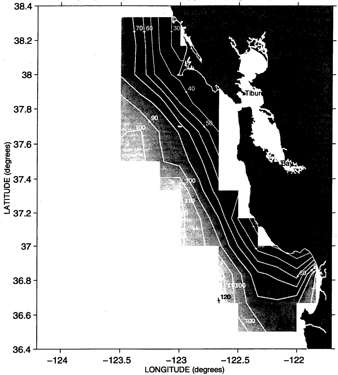
Depth (meters) of the 26.2 Isopycnal during Sweep 3, 1987
