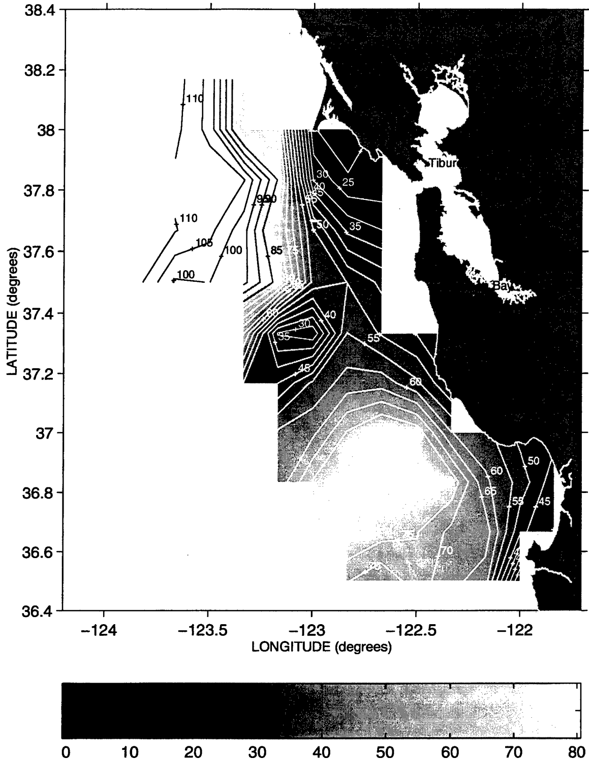
Depth (meters) of the 25.8 Isopycnal during Sweep 3, 1993
