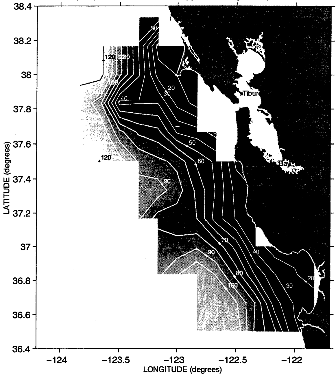
Depth (meters) of the 26.2 Isopycnal during Sweep 1, 1991
