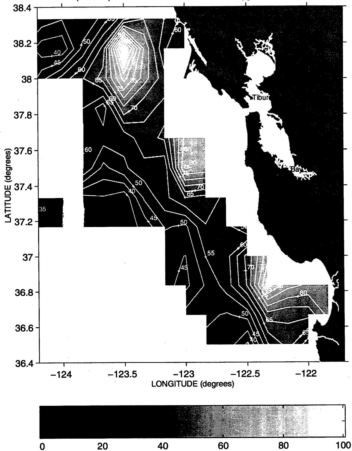
Thickness(meters) between the 25.8 and 26.2 isopycnals ~ Sweep 3, 1992
