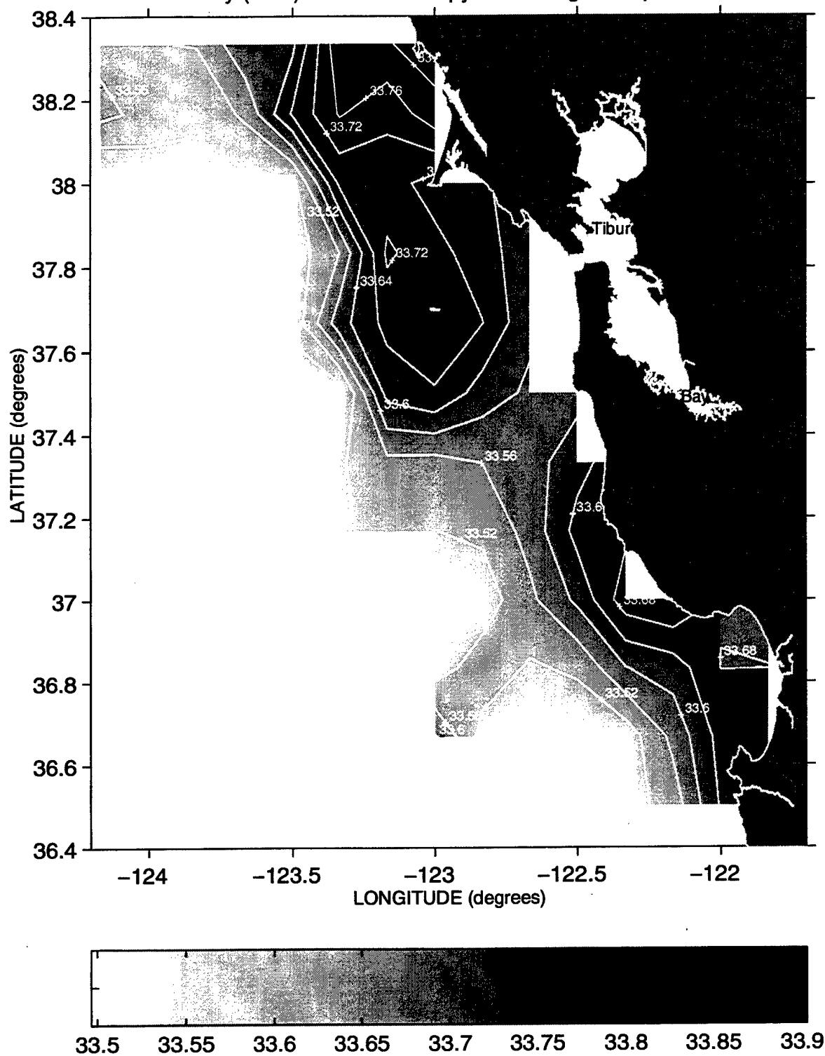
Salinity (PSS) at the 25.8 Isopycnal during Sweep 2, 1994
