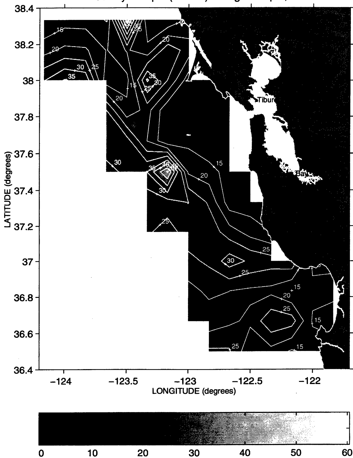
Mixed Layer Depth (meters) during Sweep 2, 1994
