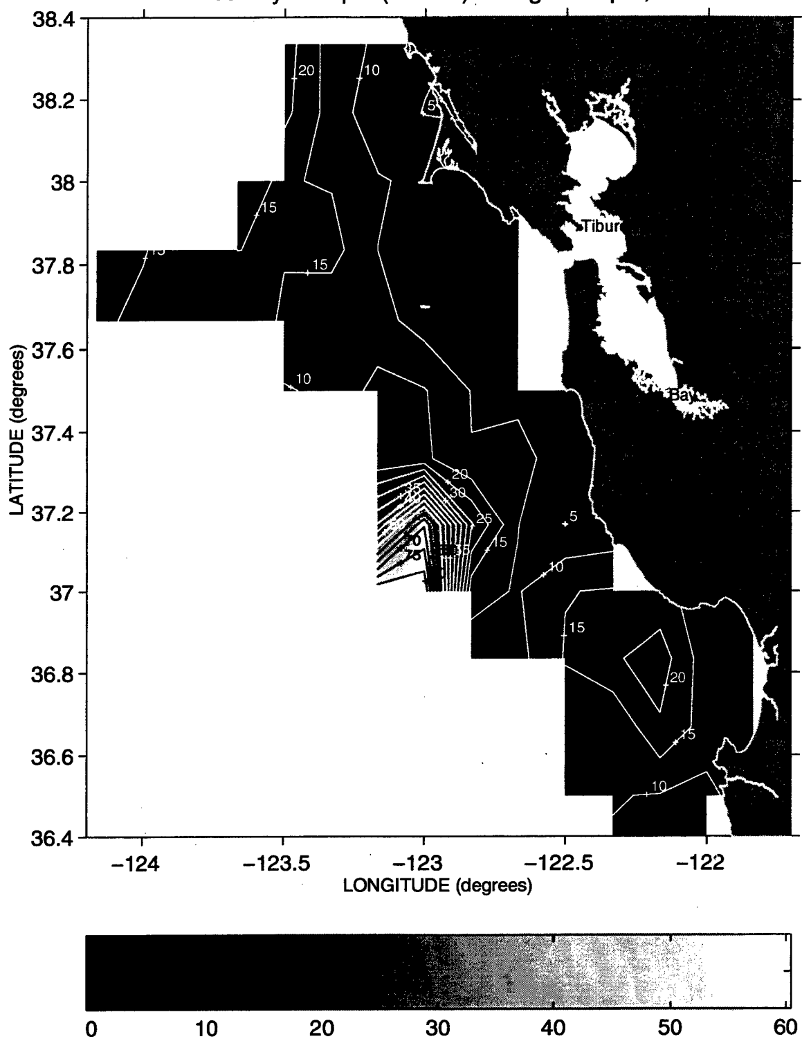
Mixed Layer Depth (meters) during Sweep 2, 1988
