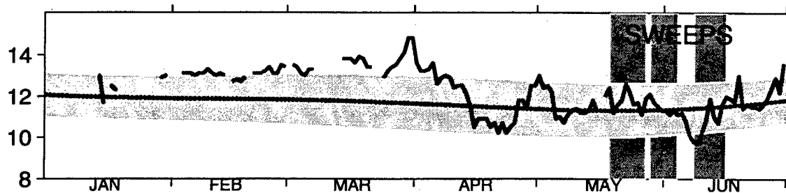
Surface Salinity ~ 1995
