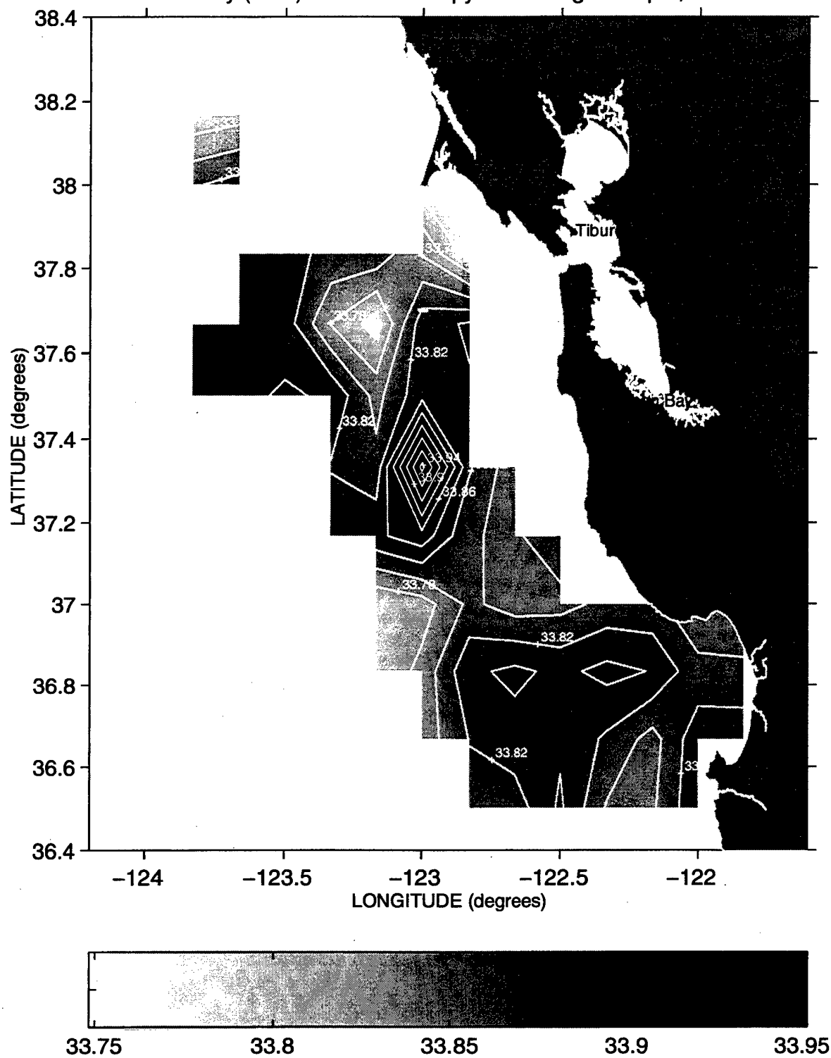
Salinity (PSS) at the 26.2 Isopycnal during Sweep 3, 1993
