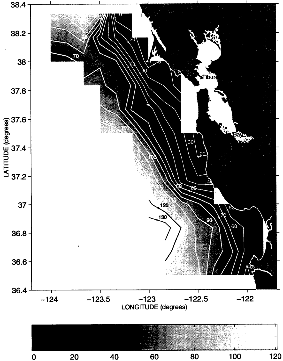
Depth (meters) of the 26.2 Isopycnal during Sweep 3, 1994
