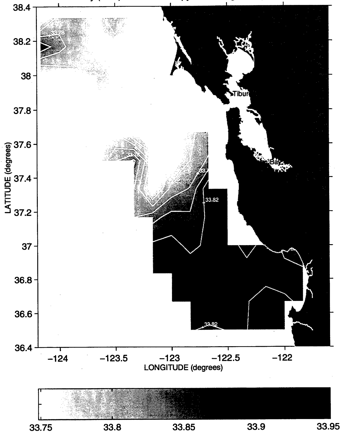
Salinity (PSS) at the 26.2 Isopycnal during Sweep 2, 1993
