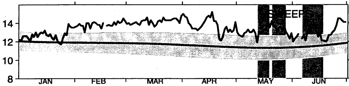
Surface Salinity ~ 1992
