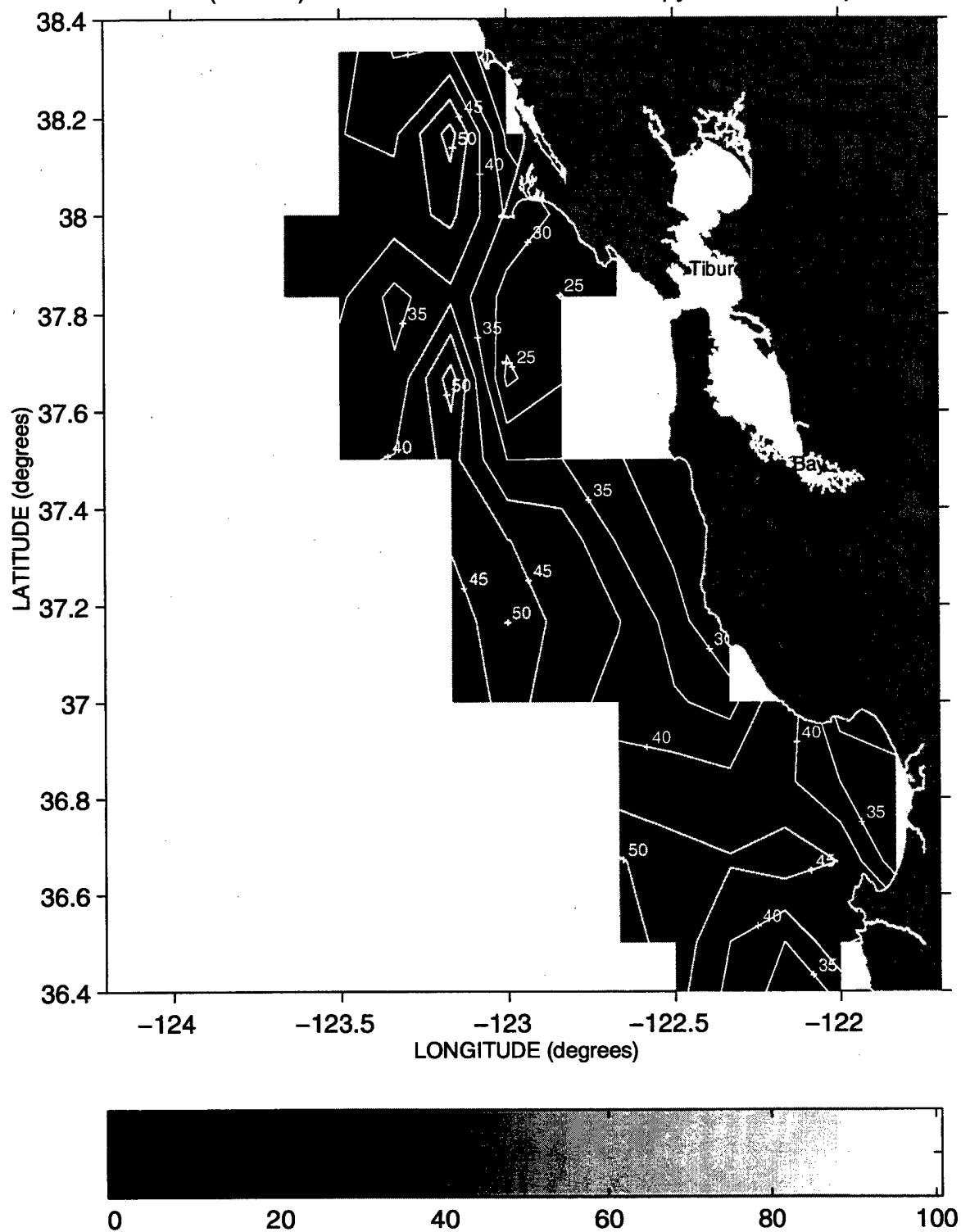
Thickness(meters) between the 25.8 and 26.2 isopycnals ~ Sweep 3, 1990
