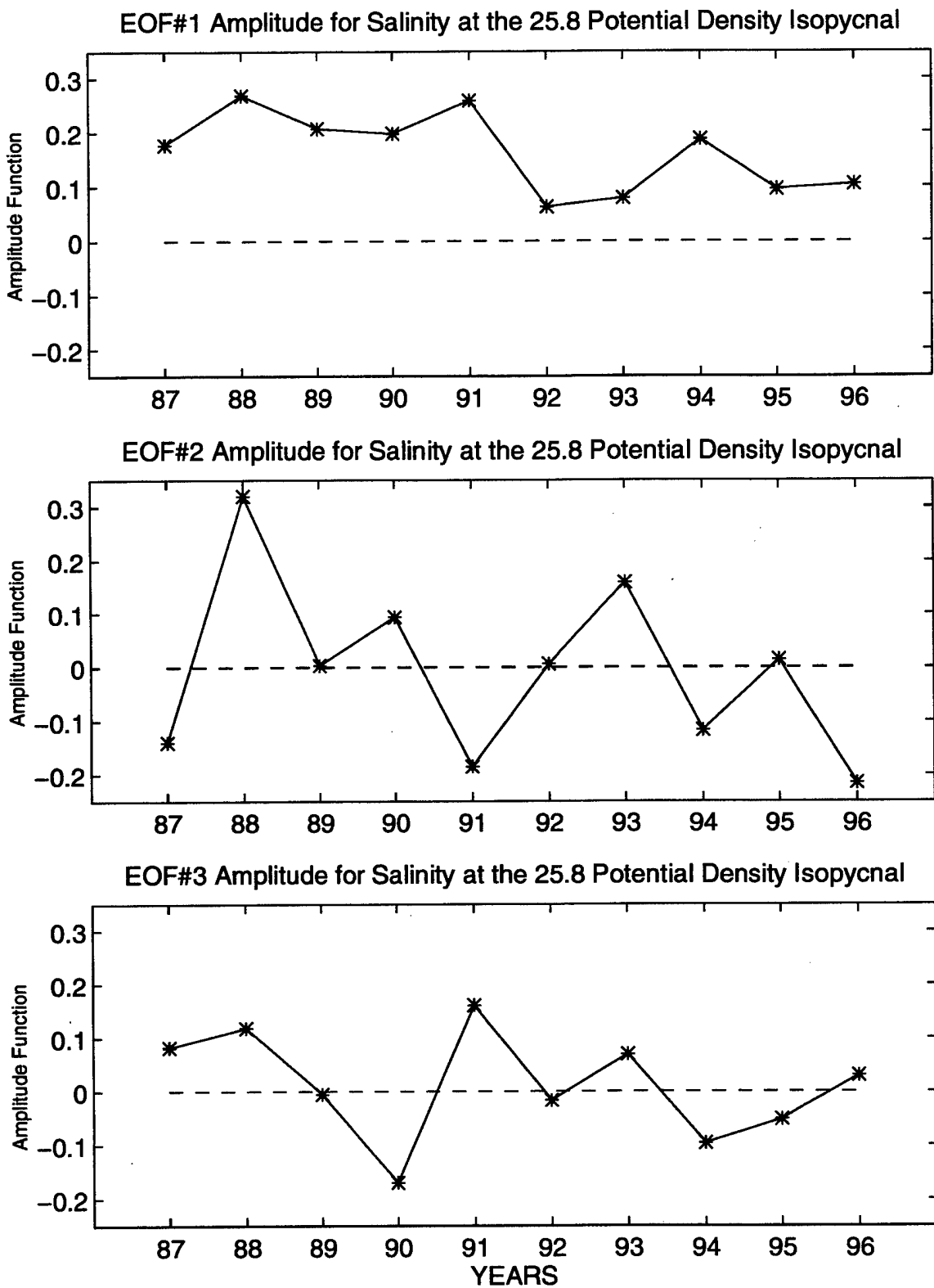
Figure 45. Temporal amplitudes of the first three EOFs for salinity on the 25.8 kg/m 3 isopycnal.
