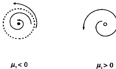
Figure 6. Subcritical Hopf Bifurcation
