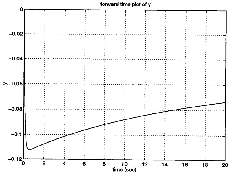
Figure 15. Simulation: y Dynamics for \mu = 0 (Feedback ON)
