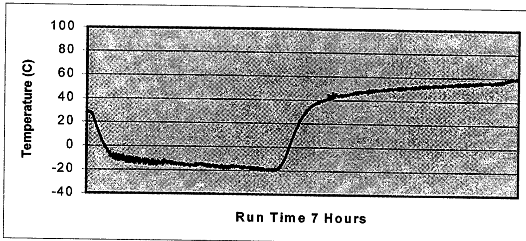
Figure 6.16 MSU #1 Thermal Vacuum Run #1
