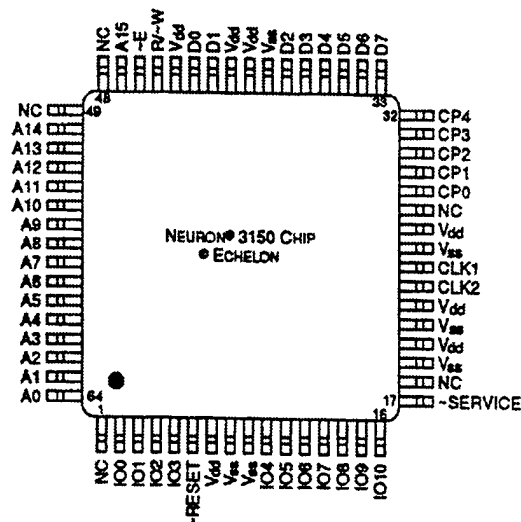
Figure 4.1 Neuron Chip Plan View (Echelon, Neuron Chip Data Book)
