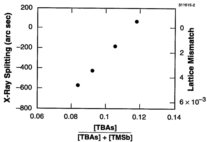
Figure 2-4. Lattice mismatch of GaInAsSb grown at 575°C as a function of TBAAs fraction in the gas phase.
