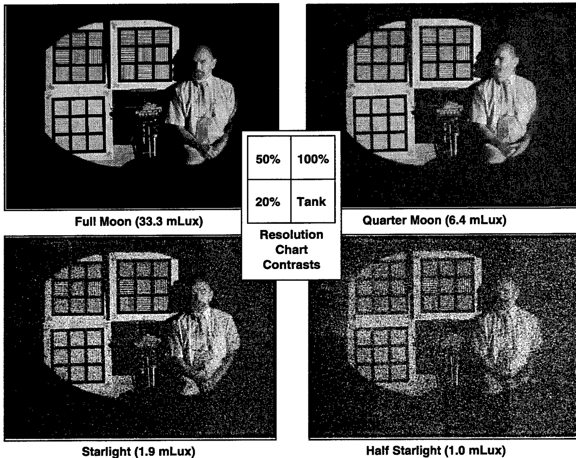
Figure 5-3. Contrast resolution chart images from the 640 \times 480 -pixel CCD camera for lighting conditions ranging from full moon to half starlight. The camera is operating at 30 frames per second and the lens used in obtaining the images had an f -number of 1.4.
