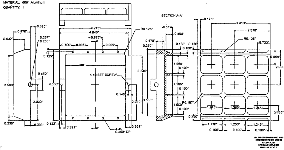
Figure 5: Scanning Mirror Holder.
