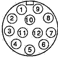
Figure 23: Camera P12, 12 Pin Connector. From Pulnix (1996).
