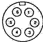
Figure 22: Camera P6, Six Pin Connector. From Pulnix (1996).
