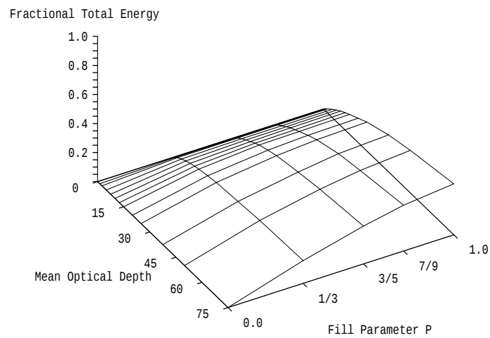
Figure 25. Fractional flux escaping from volume top for 30^\circ incident direct radiation as a function of the P parameter and mean single-axis optical depth.
