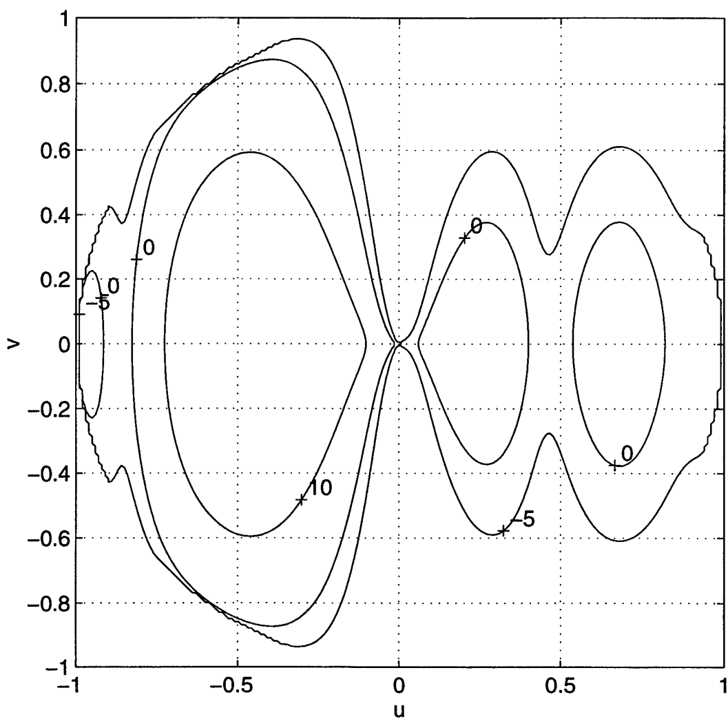
Figure 31. Contour plot (in dB) in direction cosine space for the beam steered to \theta = -25^\circ for the geometry of Figure 7.
