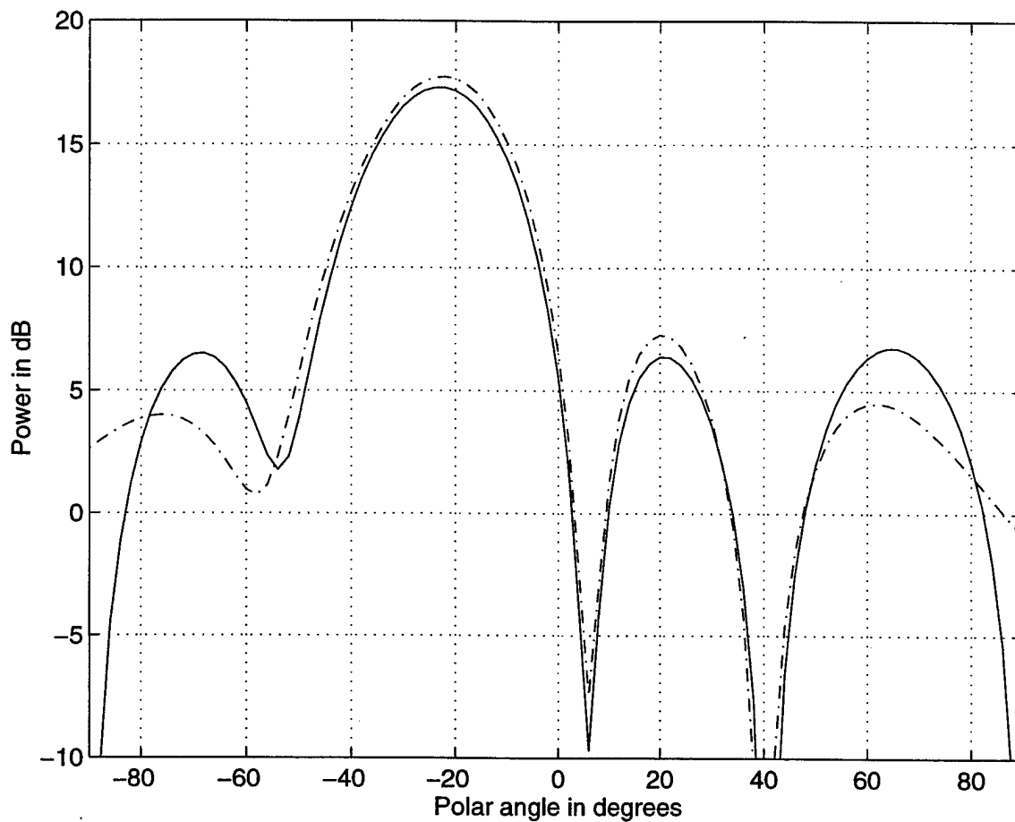
Figure 23. Radiation patterns for five elements ( d=0.35 wavelength) and the beam steered to -25 degrees. Solid line: over an infinite ground plane; Dash-dotted line: over a finite ground plane ( \phi=0^\circ ).
