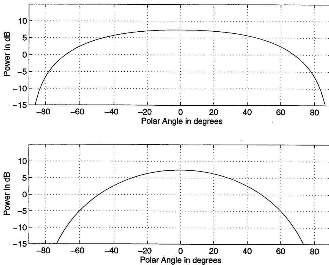
Figure 9. Radiation pattern for single dipole over infinite ground plane obtained from patch (top: \phi = 0^\circ ; bottom: \phi = 90^\circ ).
