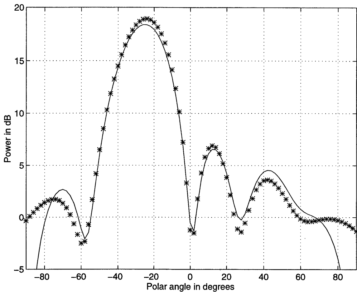
Figure 20. Radiation pattern for five elements with the beam steered to -25 degrees. Solid line: over infinite ground plane; crosses: over finite ground plane ( \phi = 0^\circ ).
