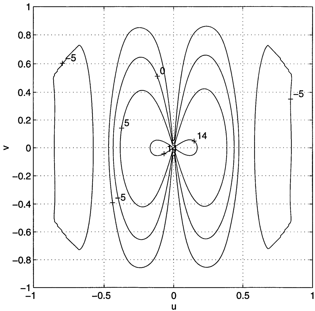
Figure 39. Radiation pattern in direction cosine space (contour plot in dB) for the geometry of Figure 35.
