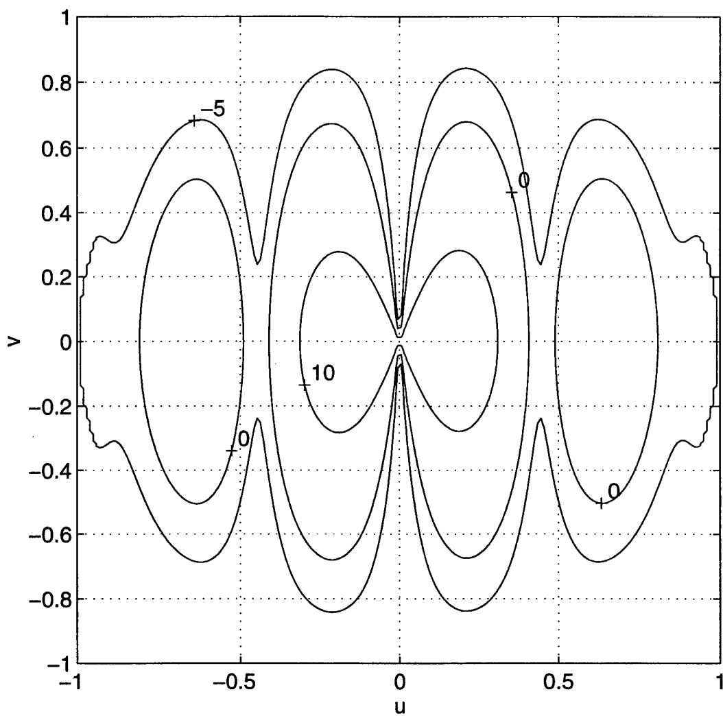
Figure 27. Radiation pattern in direction cosine space (contour plot in dB) for the geometry of Figure 7.
