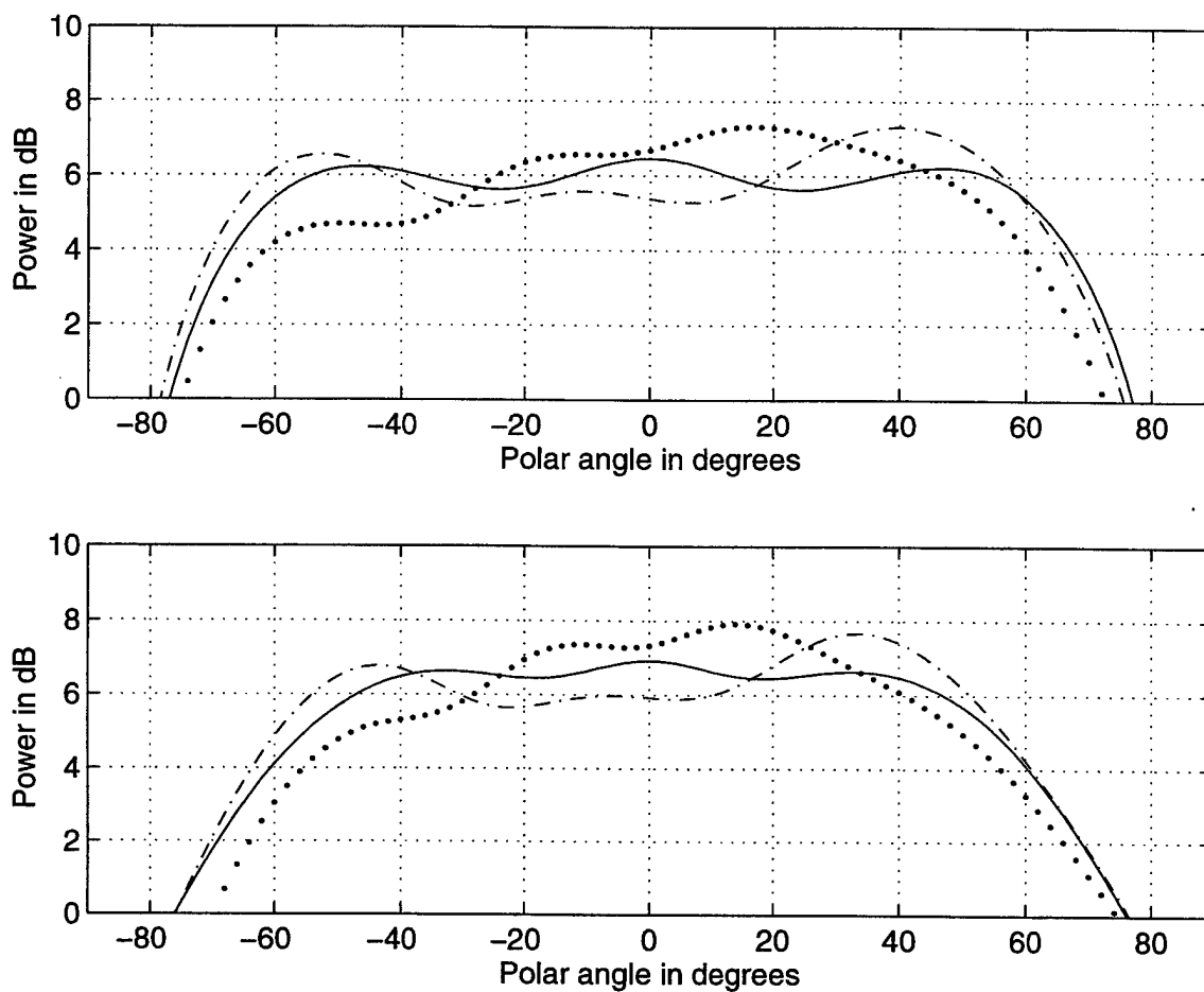
Figure 22. Top: element factors for five elements over an infinite ground plane as in Figure 19. Bottom: element factors for five elements over a finite ground plane as in Figure 7. Solid line: element 3, dash-dotted line: element 2, dotted line: element 1. The distance between the elements is 0.35 wavelength ( \phi = 0^\circ ).
