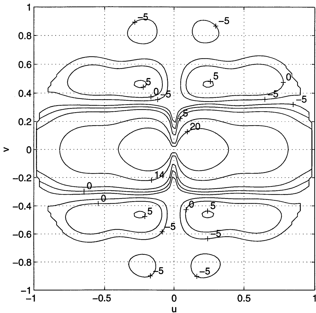
Figure 55. Contour plot (in dB) of the radiation pattern for the geometry of Figure 52.
