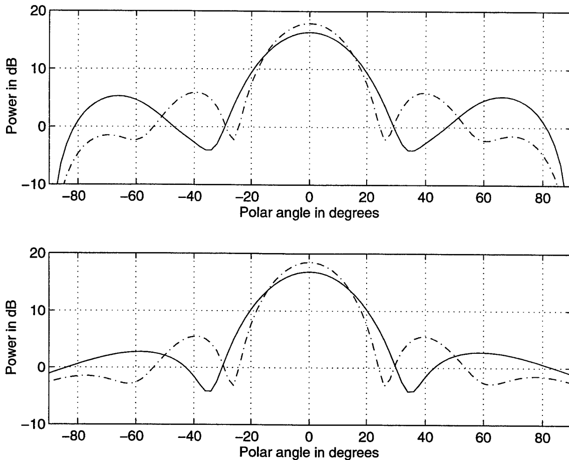
Figure 21. Radiation pattern for five elements when the distance between the elements is d=0.35\lambda (solid line) in comparison with the original geometry where d=0.4\lambda (Dash-dotted line). Top: infinite ground plane. Bottom: finite ground plane ( \phi=0^\circ ).
