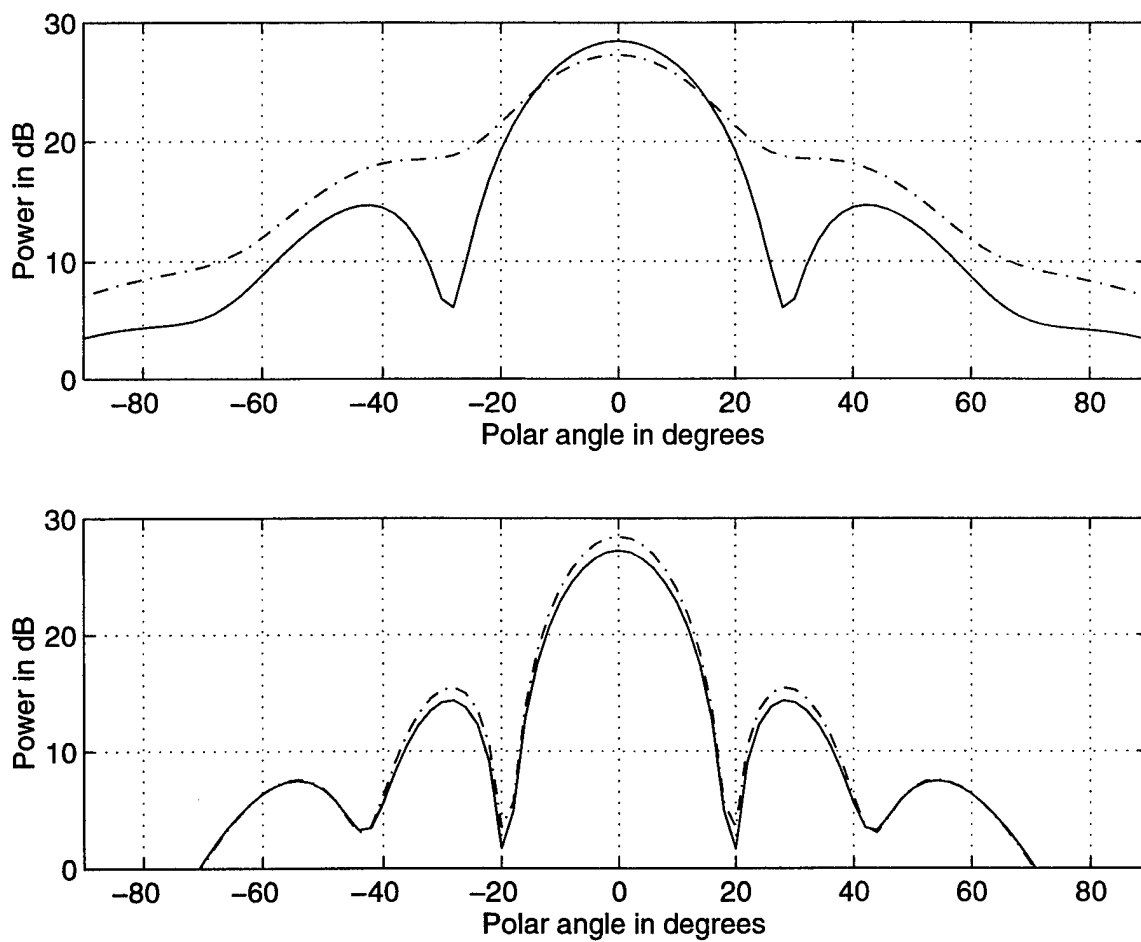
Figure 53. Radiation patterns for the five by five array with flat (solid line) and curved (dash-dotted line) geometry. Top: \phi -polarization for \phi = 0^\circ . Bottom: \theta -polarization for \phi = 90^\circ .
