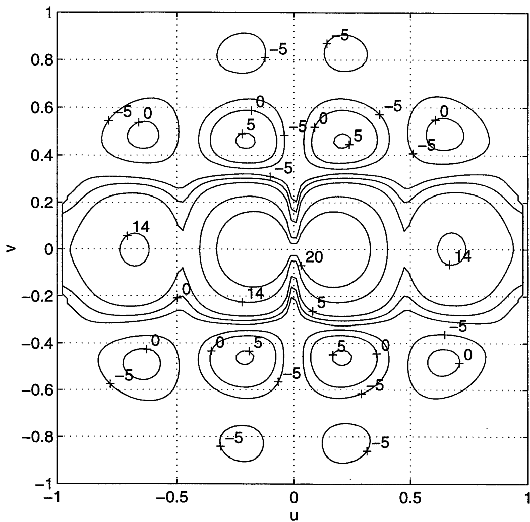
Figure 54. Contour plot (in dB) of the radiation pattern for the geometry of Figure 48.
