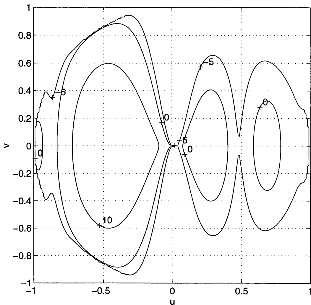
Figure 32. Contour plot (in dB) in direction cosine space for beam steered to \theta = -25^\circ for the geometry of Figure 24.
