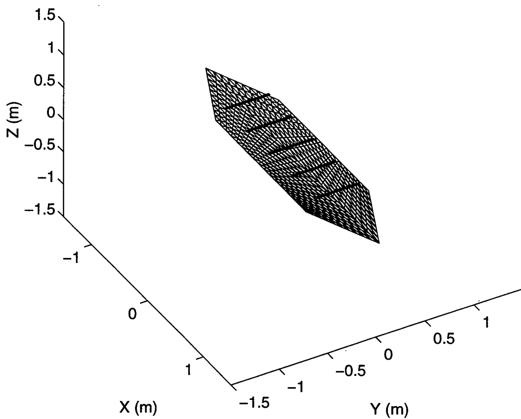
Figure 35. Geometry similar to Figure 24 with the ground plane edges extending 0.1 wavelength beyond the dipole edge.
