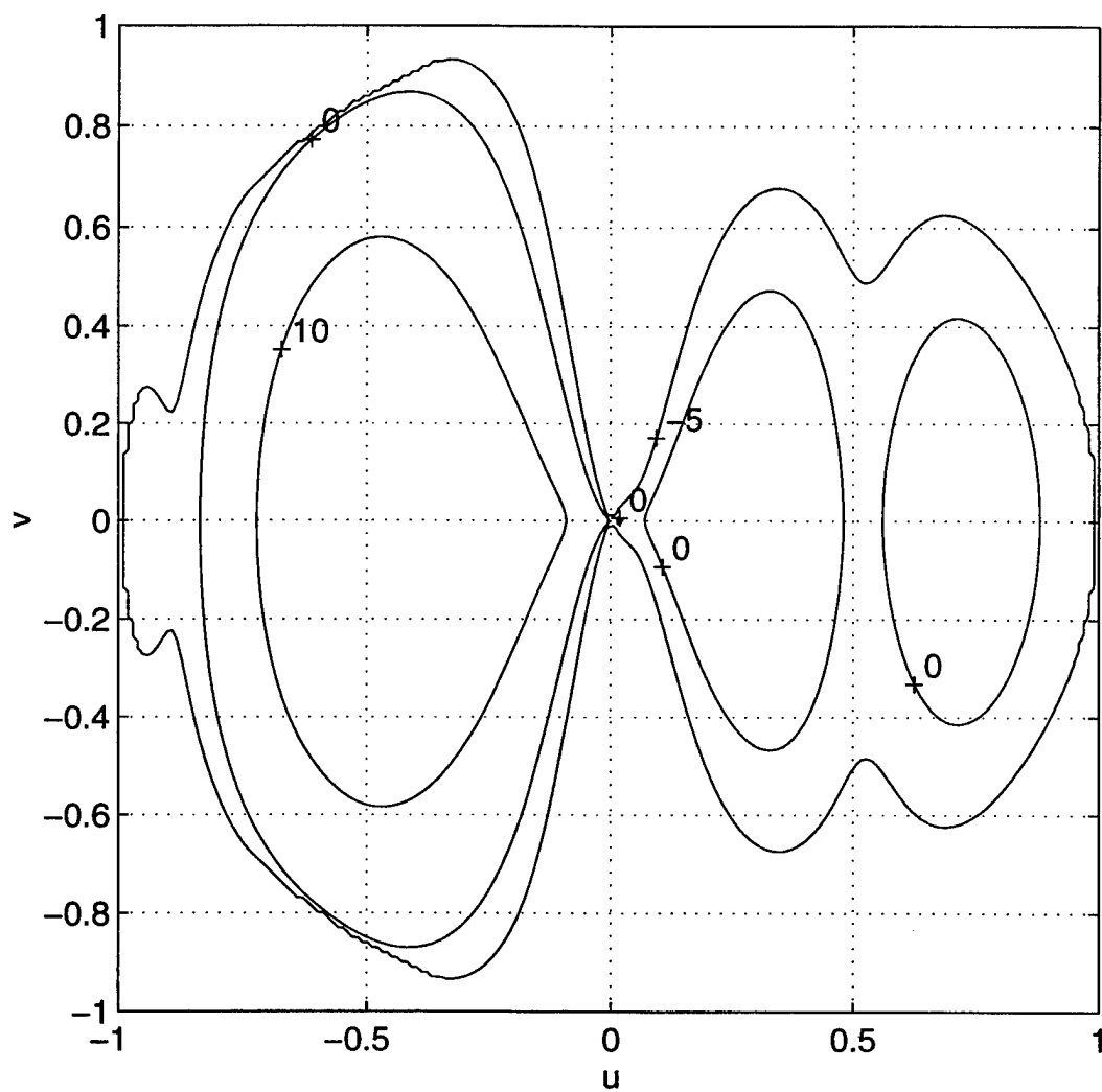
Figure 33. Contour plot (in dB) in direction cosine space for the beam pattern steered at \theta = -25^\circ for the geometry of Figure 25.
