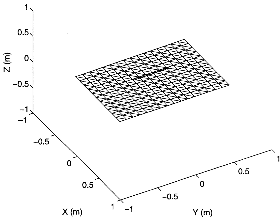
Figure 10. Single dipole over finite ground plane.
