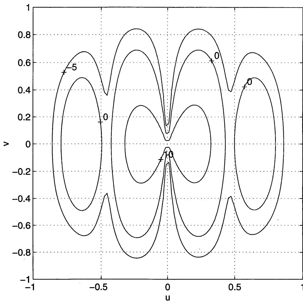
Figure 29. Radiation pattern in direction cosine space (contour plot in dB) for the geometry of Figure 25.
