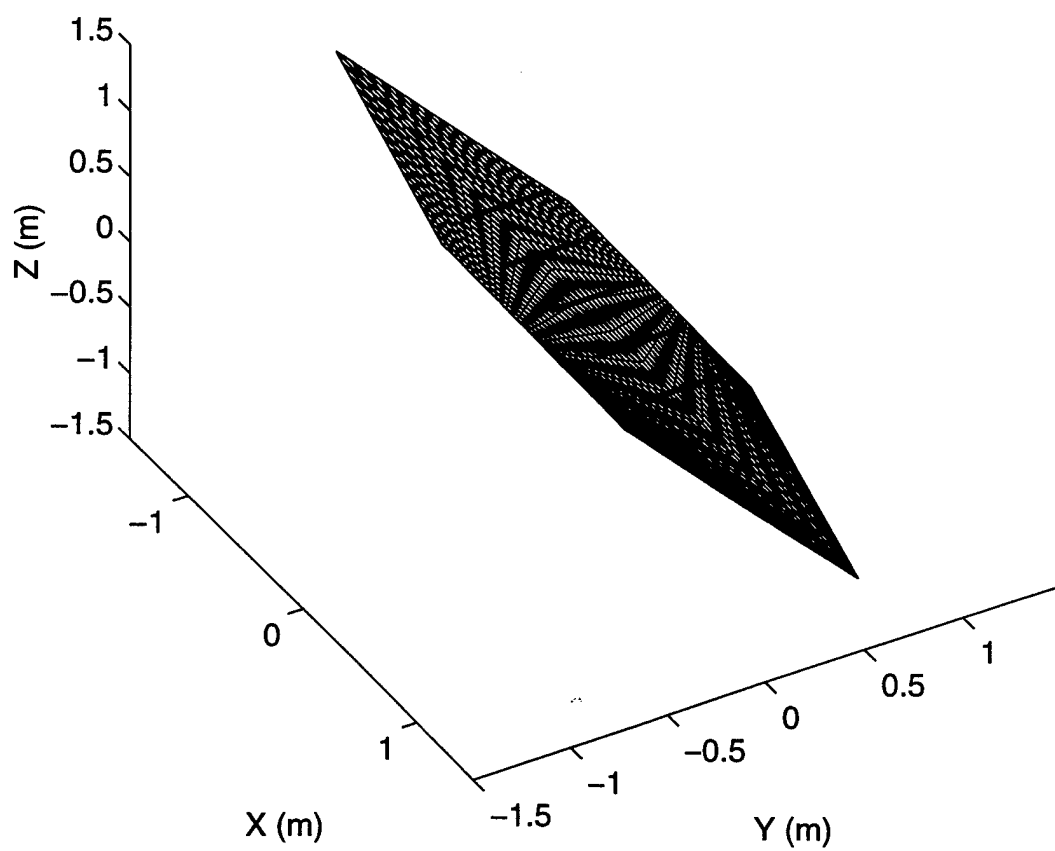
Figure 36. Geometry similar to Figure 25 with the ground plane edges extending 0.1 wavelength beyond the dipole edge.
