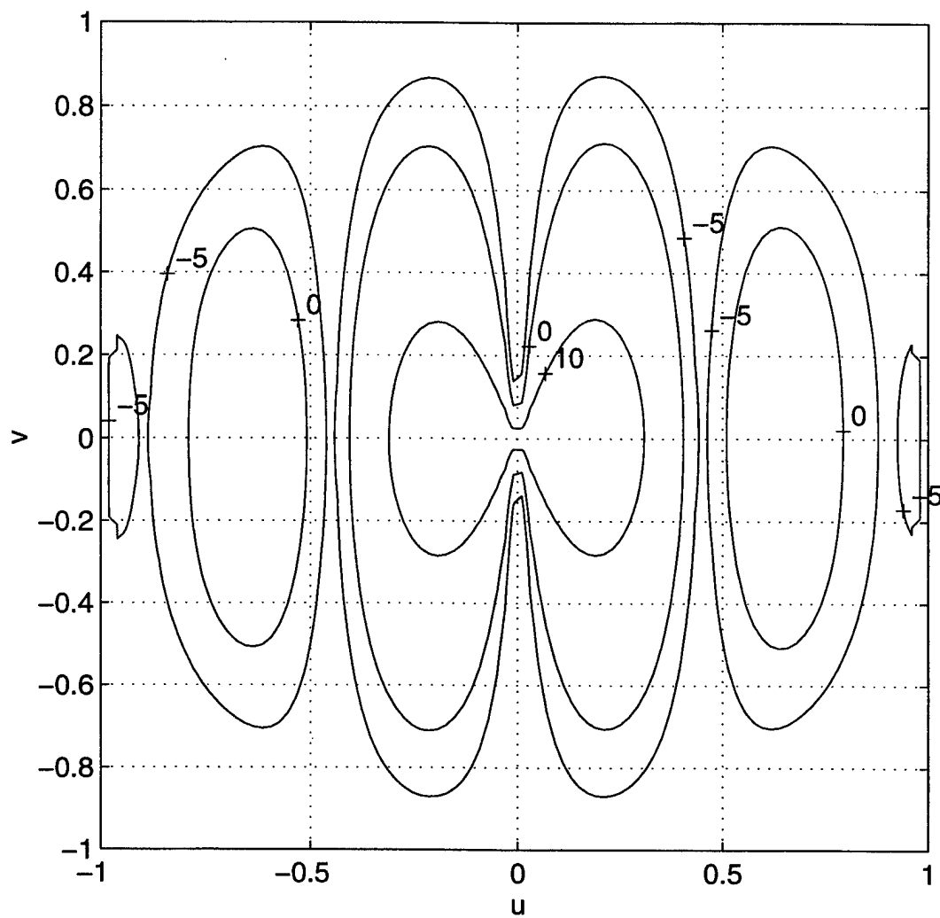
Figure 28. Radiation pattern in direction cosine space (contour plot in dB) for the geometry of Figure 24.
