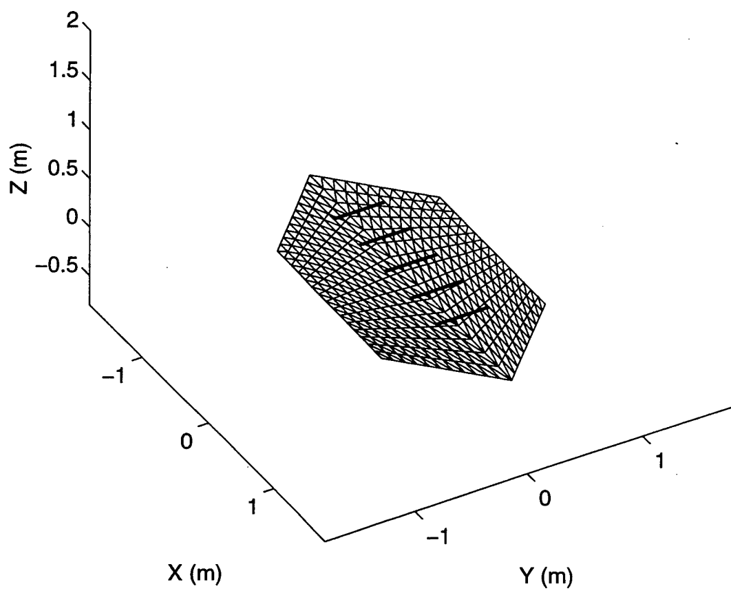
Figure 24. Shaped ground plane with triangular edges of height 0.5 wavelength.
