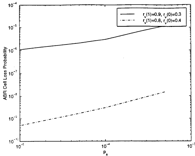
Figure 5: ABR cell loss probability vs. p_s for various VBR arrival rates
