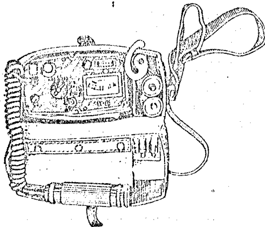
Figure 5.1 IT-65 intensity meter in carrying case
