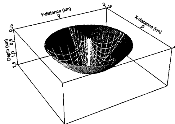
Figure 4. The rays (white) of linear slotted model have a parabolic shape. The grey surface is the caustic surface of the ray equations for this model.
