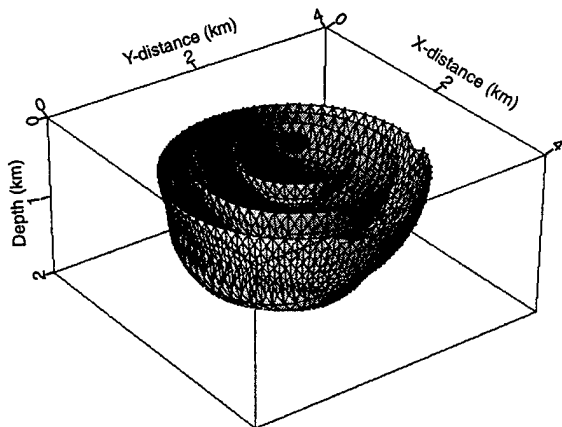
Figure 6. Triangulated wavefronts for smoothed salt dome model at t = 0.1, 0.4, 0.65, and 0.9s . The source is located at the center of the up surface.
