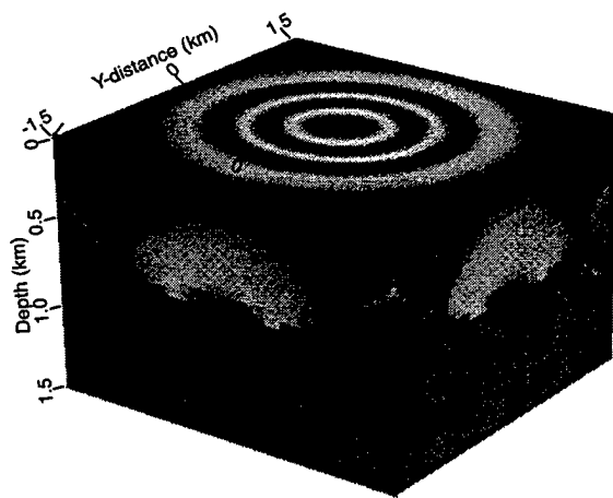
Figure 3. 3D wave field of a linear slotted model using WF construction method. The grey part is the shadow zone.
