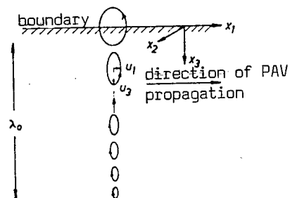
Figure 1. Illustrated motion of particles in an acoustic surface wave u_1 , u_3 are components of the displacement vector
