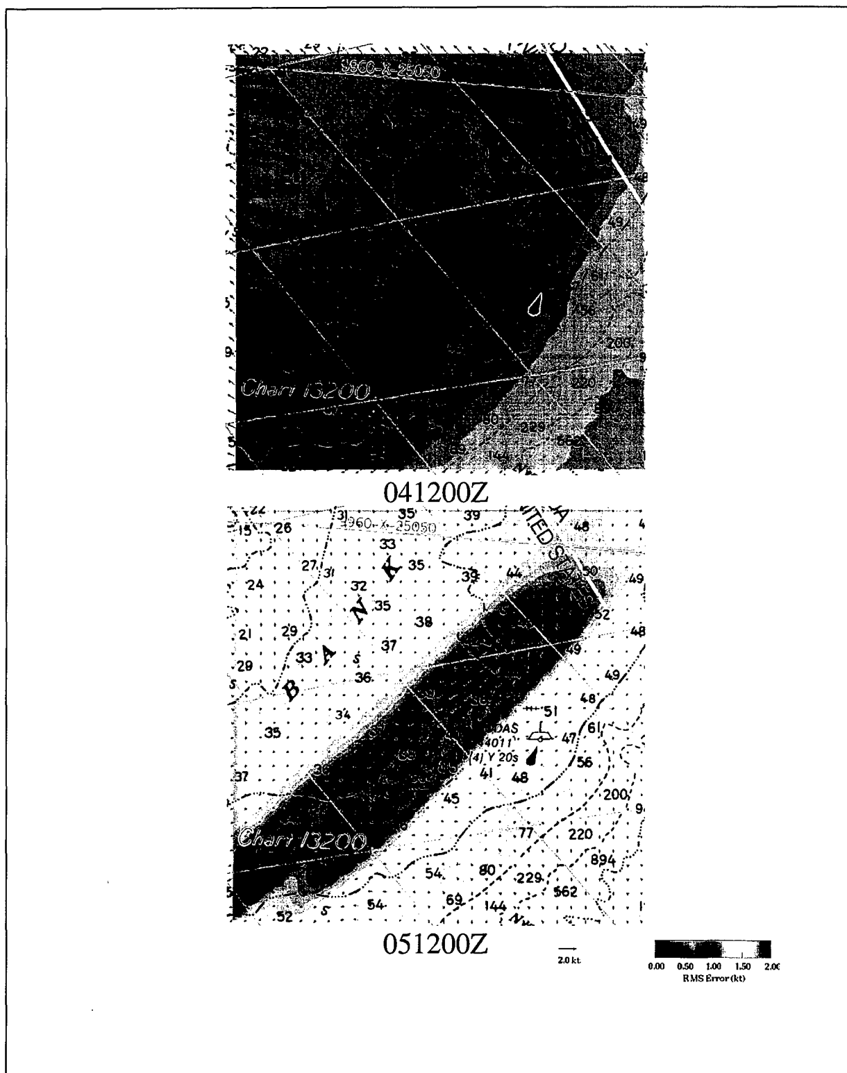
Figure 5-7. OPS Current Field Estimate, 041200Z - 051200Z JUN 96
