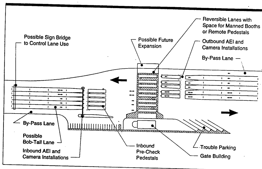
Figure 9. State-of-the-art rail facility gate. [Ref. 49]
