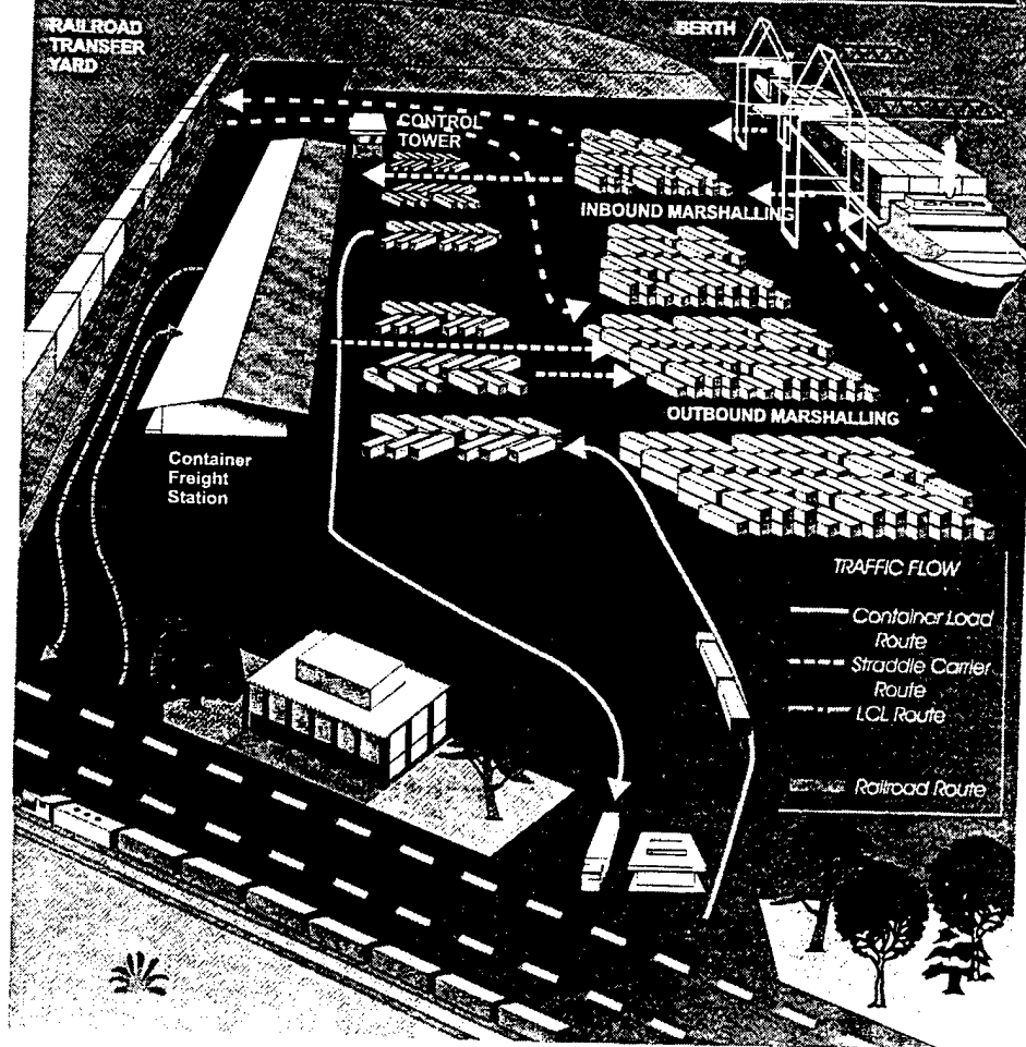
Figure 12. Organization of and traffic flow through a fixed-port container transfer facility. [Ref. 27]
