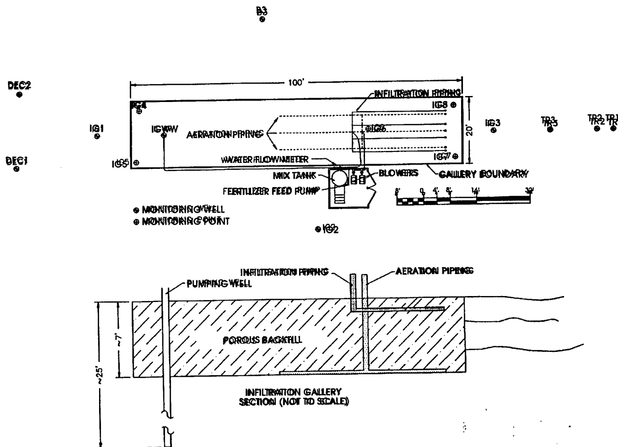
Figure 6. Infiltration gallery and monitoring wells (1 ft = 0.3048 m).
