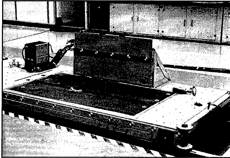
Figure 3. CAMI Test Sled Setup
