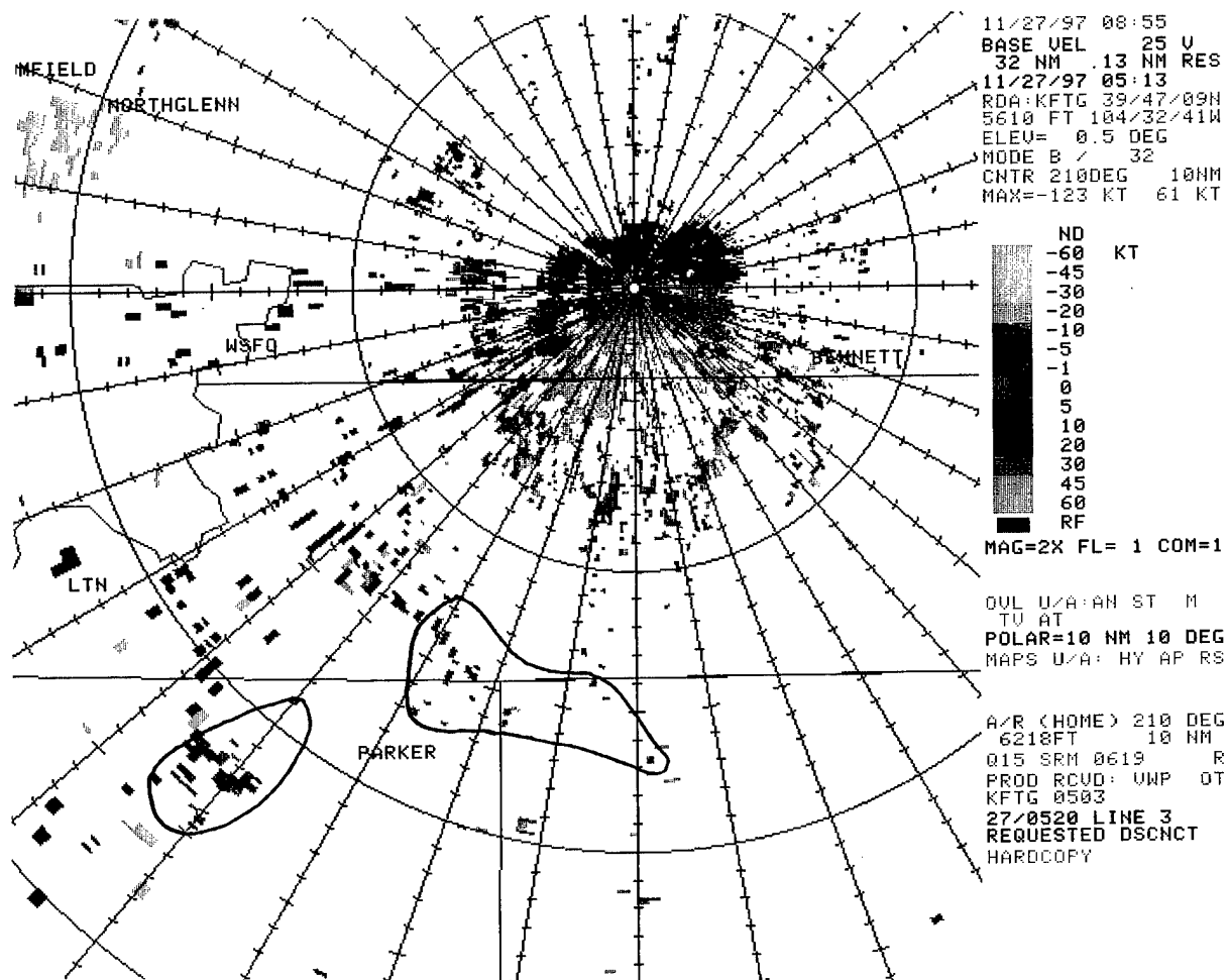
Fig. 7. Impact of Ground Contaminated Data on the Base Velocity Product of the Denver WSR-88D. Regions of anomalously small velocity magnitudes are circled. Range rings are positioned at intervals of 10 nm from the radar dish with radials drawn every 10°. The default range used by the VAD algorithm is 16.2 nm (30 km).
