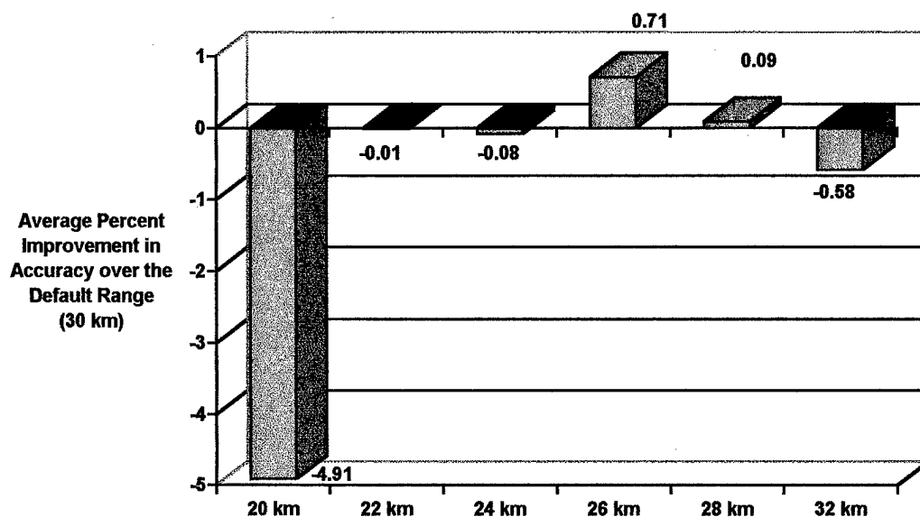
Fig. 8. Skill Scores for Alternative Ranges Obtained Using Profiler Data for Verification (Averaged over All Seasons for Atmospheres which Were Superrefractive at the Surface )
