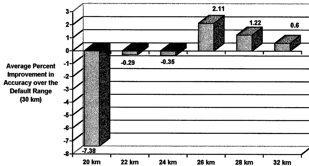
Fig. 16. Skill Scores for Alternative Ranges Obtained Using Profiler Data as Verification (Averaged over All Atmospheric Refractivity States for the Winter Season )
